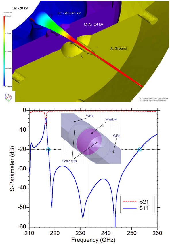
Figure 3. (top) Gun design in MICHELLE. (bottom) Simulation of pillbox resonant window structure for the input predicting over 30 \text{ GHz} BW at -20 \text{ dB} S_{11} .
