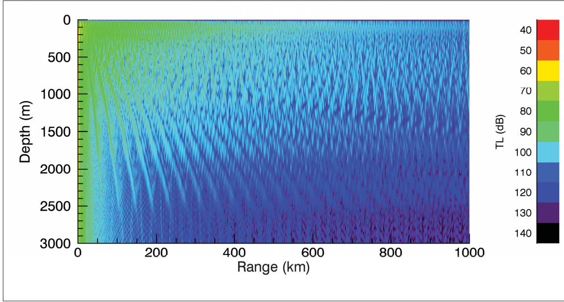
Figure 8: Full field transmission loss in Arctic environment at 50 Hz for a source at 50 m depth.
