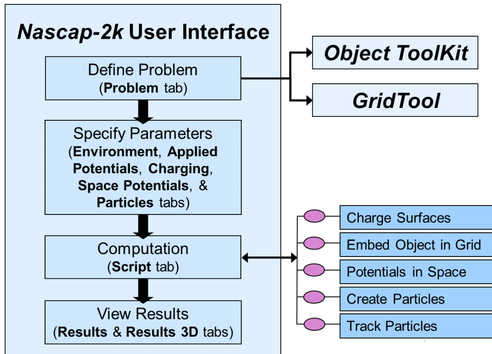
Figure 2. Nascap-2k Structure
