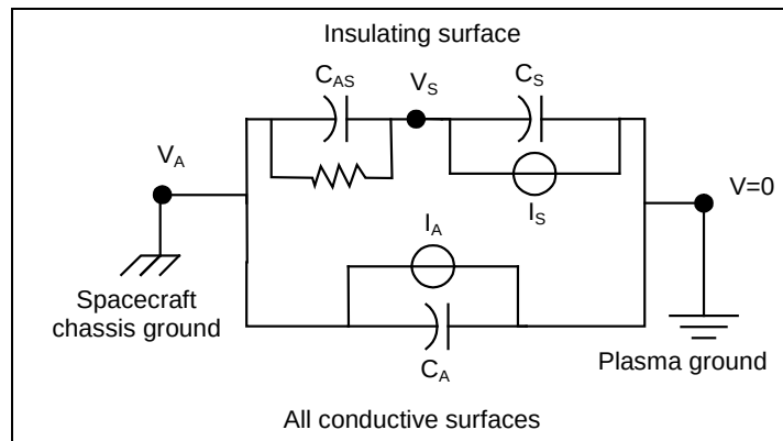
Figure 19. Circuit Model of a Spacecraft with One Insulating Surface Element
