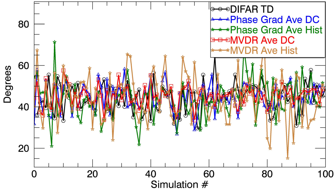
Figure 7: Estimates of the DOA from all algorithms for 100 simulations, with SNR -3 dB and the true DOA at 45°.
