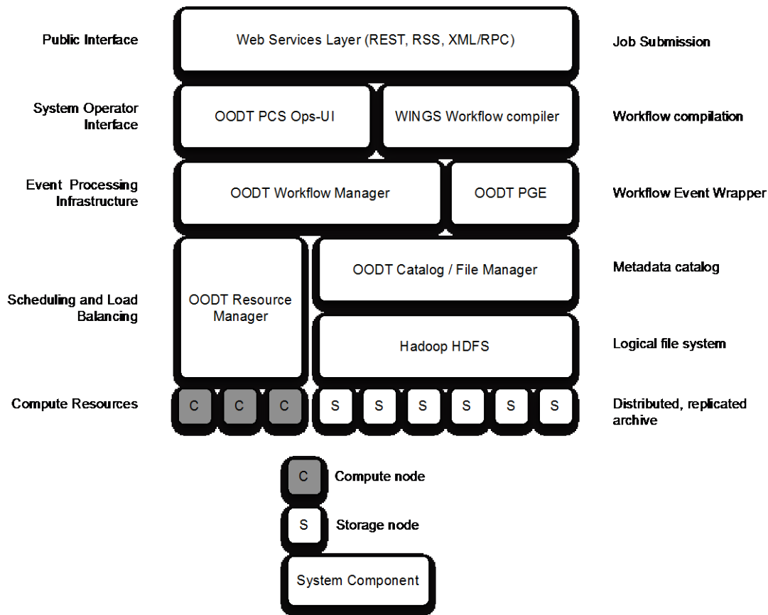
Figure 6: Architecture “To-Be” Goal for XDATA Incorporation of OODT and WINGS
