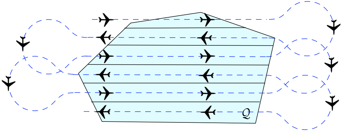
Figure 4. Depiction of the Strip Loitering policy. The segment providing closure of the loitering path (returning the UAVs from the end of the last strip to the beginning of the first strip) is not shown here for clarity of the drawing.
