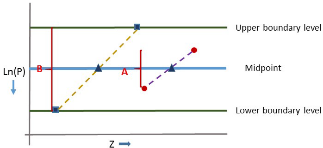
Fig. 2 Schematic chart illustrating the linear interpolation of height in terms of \ln(P) for 2 cases where the solid triangles represent the interpolated values. The first (A) is an example of interpolation between 2 data points that lie within the layer (solid circles). The second (B) is an example of interpolation between boundary levels (solid squares) where there are no data levels within the layer. Intermediate cases can occur where a data level is within the layer above or below the midpoint.
