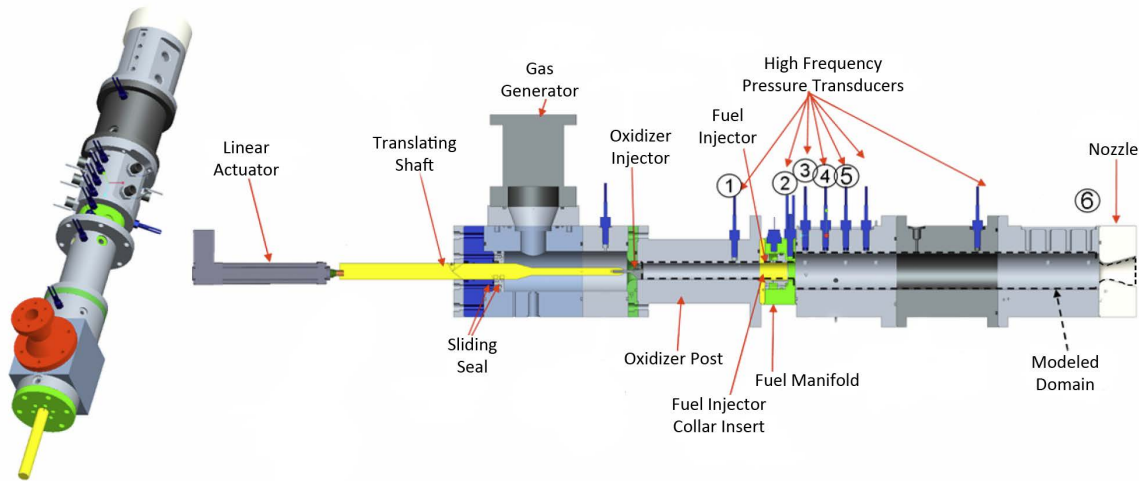
Figure 1: Experimental configuration of the CVRC experiment.
