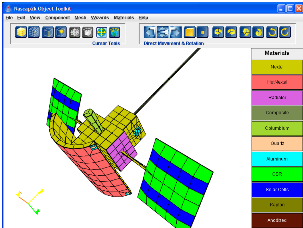
Figure 72. Object Toolkit Model of the MESSENGER Spacecraft.
