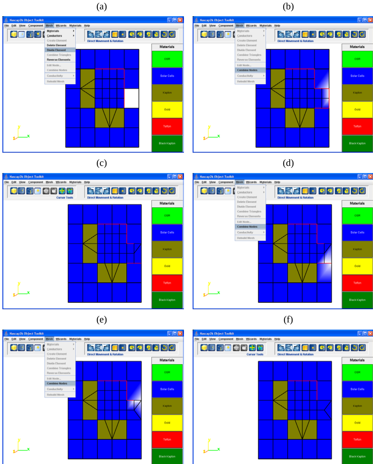
Figure 28. Resolving Incompatibilities by Dividing an Element Using “Divide Element” and “Combine Nodes” to Create Two Quadrilaterals and a Triangle in Place of the Original Single Element.
