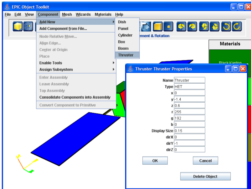
Figure 128. Thruster Definition for EPIC Object. Thruster Is Located at (0.0, -1.4, 0.6) and Is Pointed in the -Y Direction.
