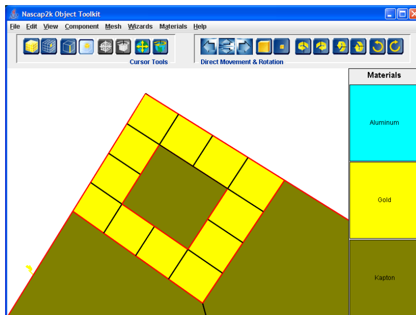
Figure 90. New Element Created after Consolidation and Then Selecting Four Nodes and Requesting “Create Element.”
