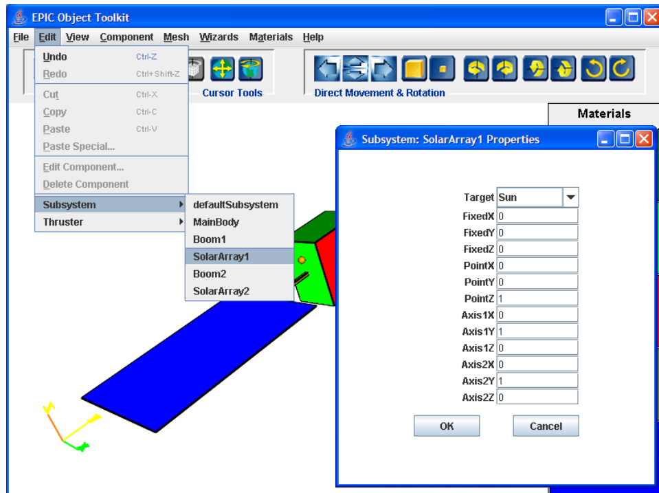
Figure 130. Setting SolarArray1 to Track the Sun. The Fixed Point Is (0.0, 0.0, 0.0). The Pointing Vector Is (0.0, 0.0, 1.0). The First Axis Is (0.0, 1.0, 0.0) and the Second Axis Is the Same.
