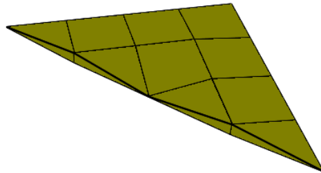
Figure 103. Adding Additional Triangular Elements to Fill in the Final Holes.
