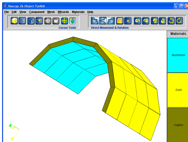
Figure 84. Hemispherical Sunshade.
