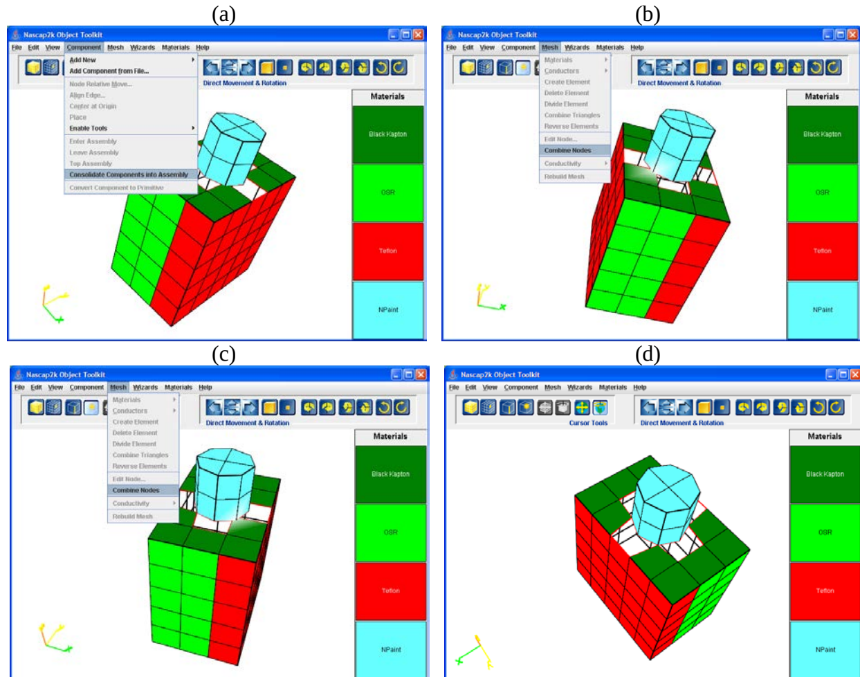
Figure 60. Moving the Nodes of the Body That Are Near the Nodes of the Cylinder to Be Coincident with the Nodes of the Cylinder. The Outlines of Elements with Normals Facing into the Screen Are Seen.
