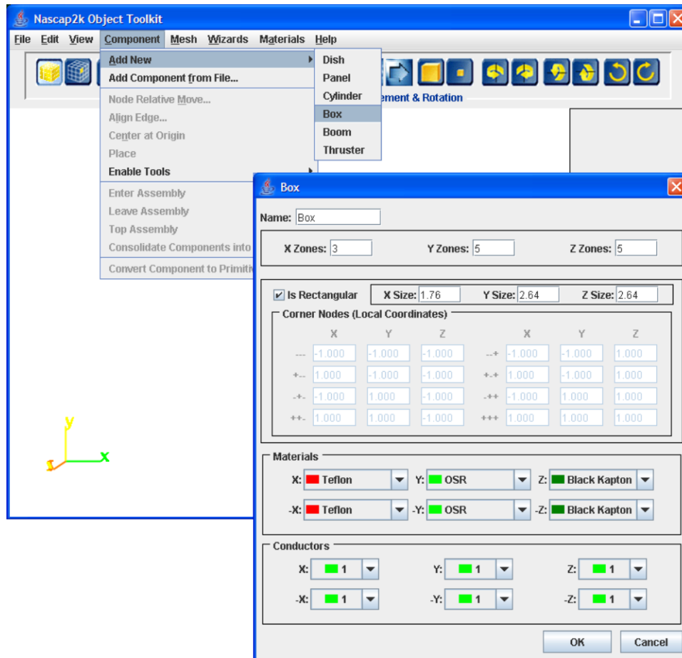
Figure 53. Defining a Box to Form the Body of the Spacecraft. The Box is 1.76 m by 2.64 m by 2.64 m in Size. Three Elements in the X Direction, and Five Elements in Each of the Other Two Directions. The \pm X Sides Are Teflon. The \pm Y Sides Are OSR. The \pm Z Sides Are Black Kapton.
