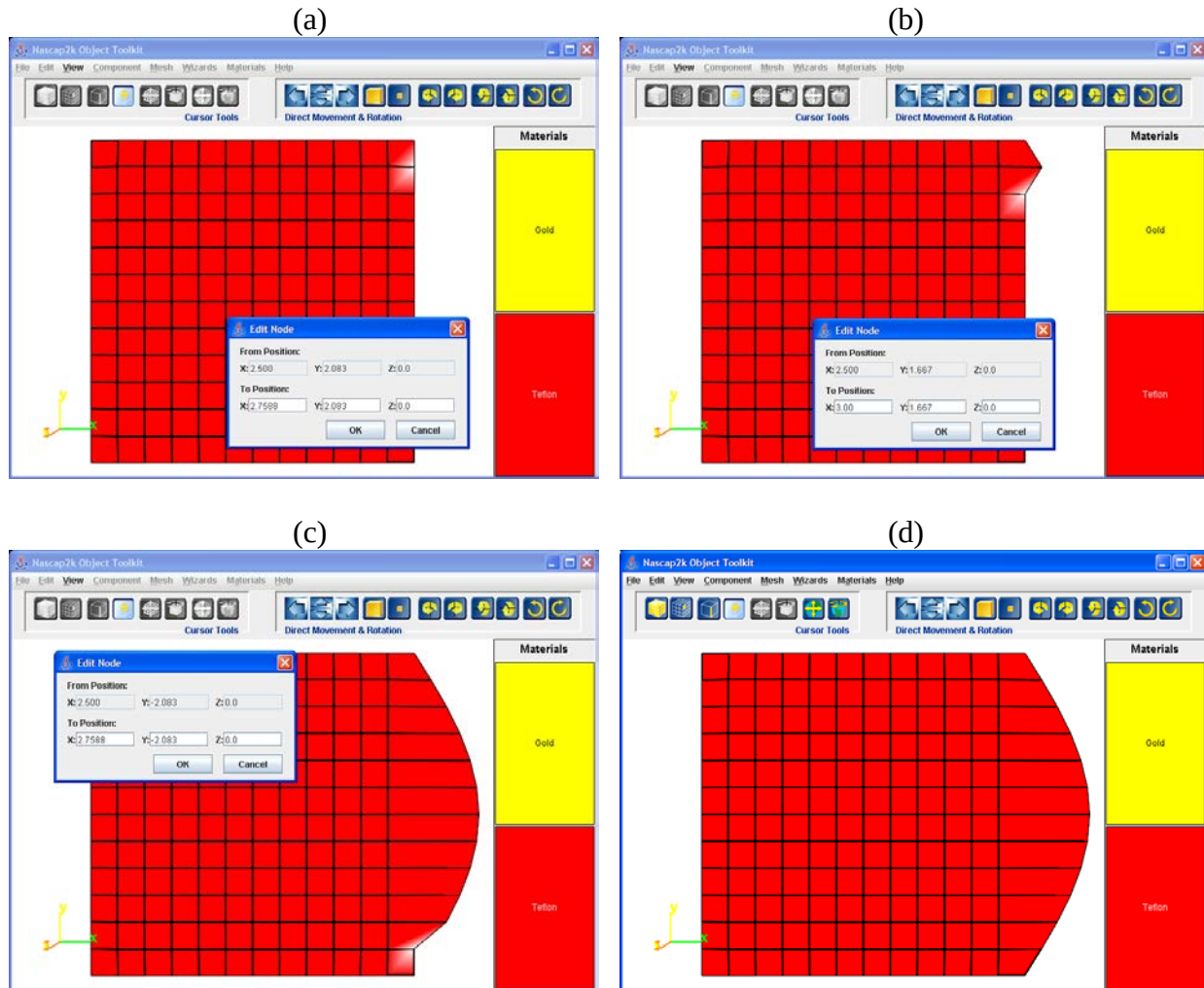
Figure 32. Changing the Edge of a Panel from a Straight Edge to a Cosine Curve by Repeated Use of “Edit Node” on the Mesh Menu.
