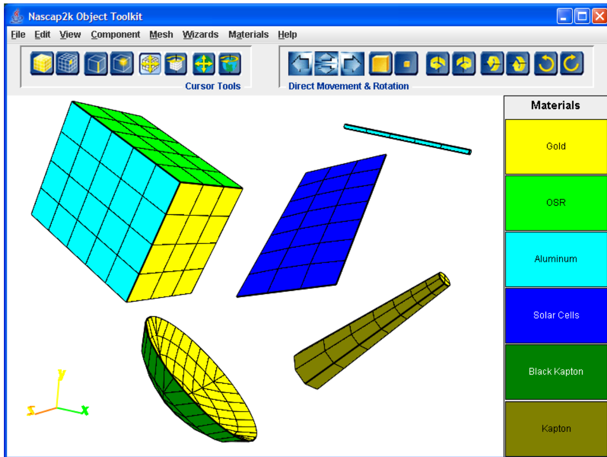
Figure 4. Object Toolkit Screen Showing the Five Standard Components.
