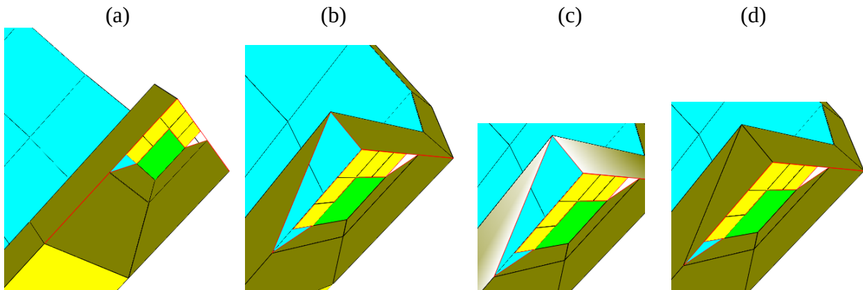
Figure 92. Replacing the Existing Side Element with Two New Elements, a Quadrilateral and a Triangle. The Outlines of Elements with Normals Facing into the Screen Are Seen.
