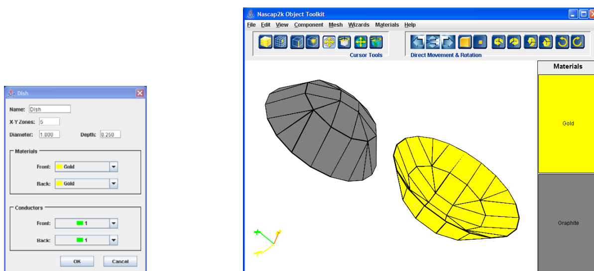
Figure 11. Definition of a Dish. The Screen on the Right Shows Two Dishes Viewed from Different Directions.
