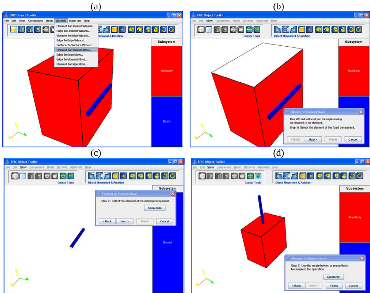
Figure 122. Placing the Boom Next to the Box Using the “Element to Element Move Wizard.”
