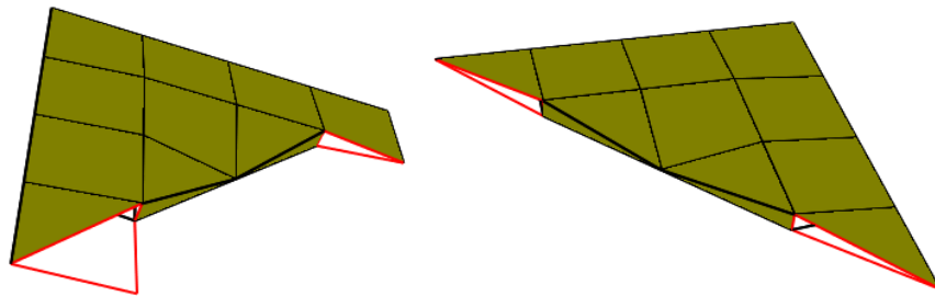
Figure 102. Replacing Each of the Square Elements in the Corners with a Triangular One, One at a Time. The Outlines of Elements with Normals Facing into the Screen Are Seen.
