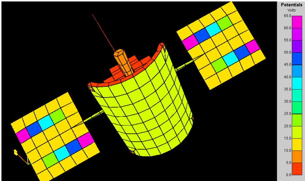
Figure 2. Nascap-2k Model of the MESSENGER Spacecraft, Showing Biased Solar Array Surfaces.
