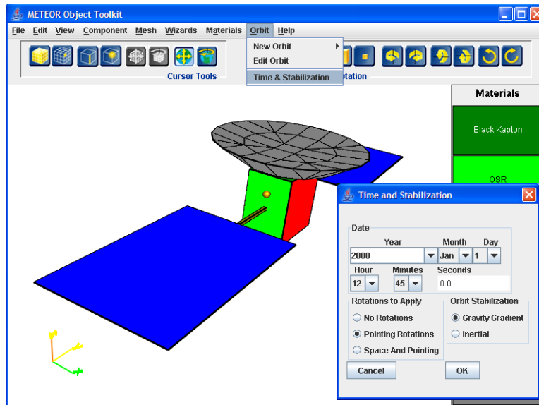
Figure 134. Applying Pointing Rotations Using the Time and Stabilization Dialog Box.
