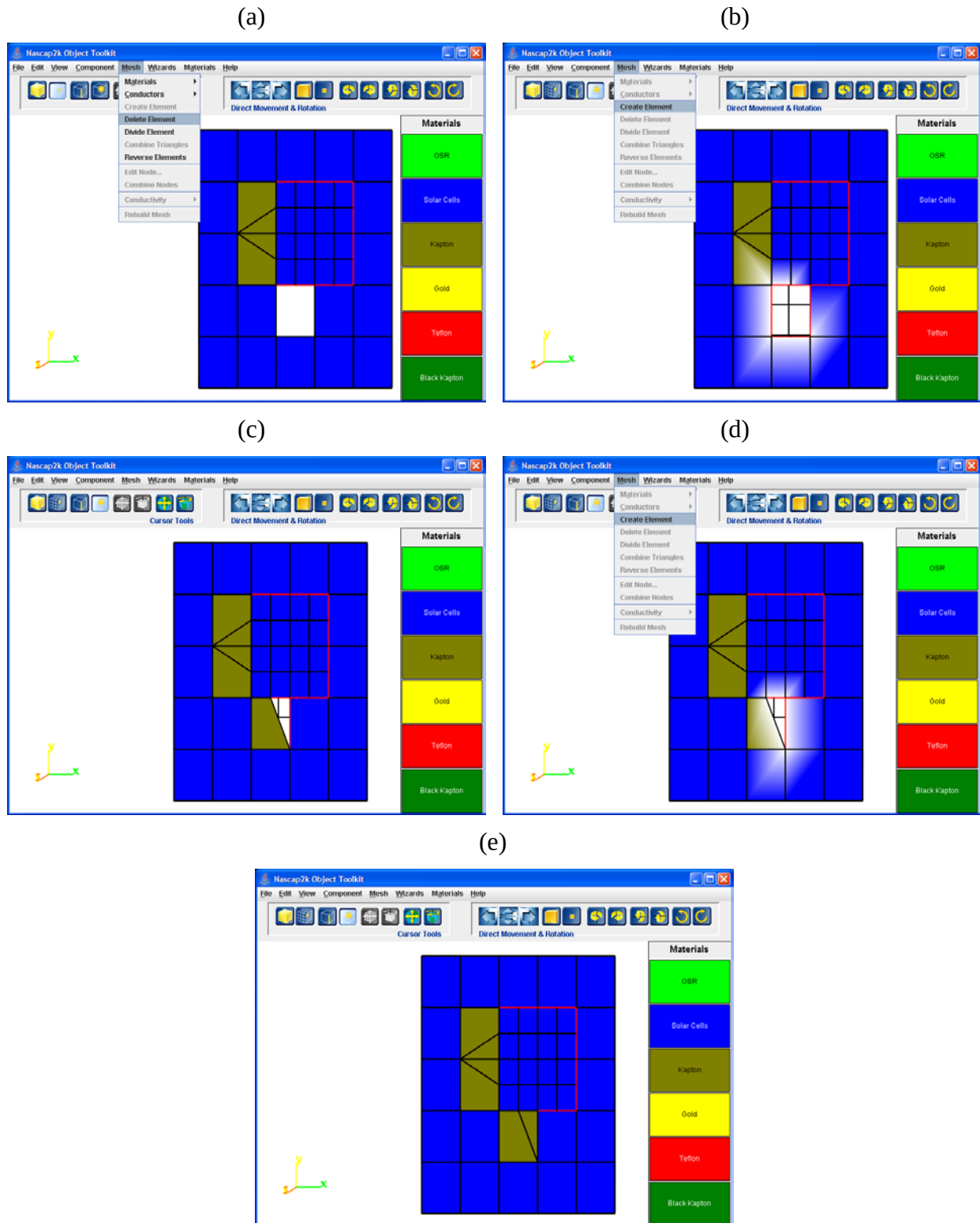
Figure 26. Deleting an Element Using “Delete Element” and Replacing It with a Quadrilateral and a Triangle by Selecting Nodes and Using “Create Element” on the Mesh Menu. In b, c, and d, the Outlines of Elements on the Far Side with Normals Facing into the Screen Are Seen.
