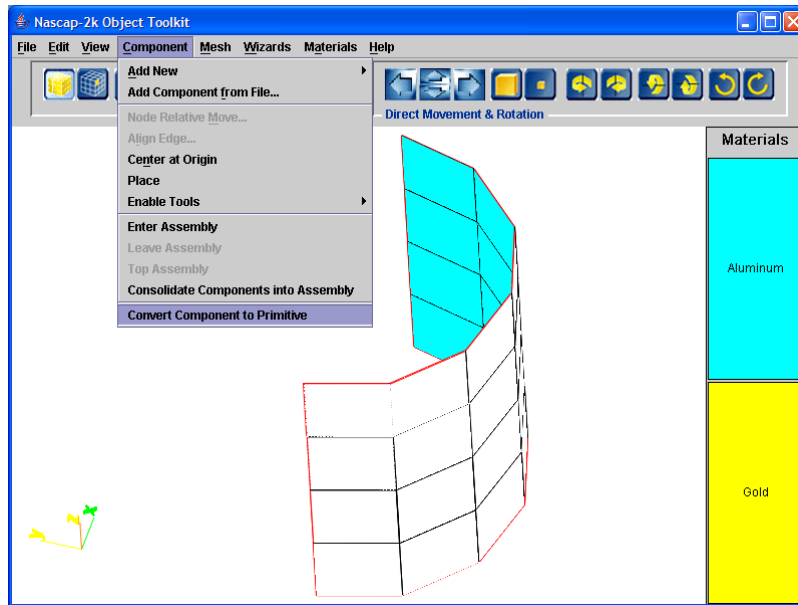
Figure 80. Converting the Outer Surface to a Primitive. The Outlines of Elements with Normals Facing into the Screen Are Seen.
