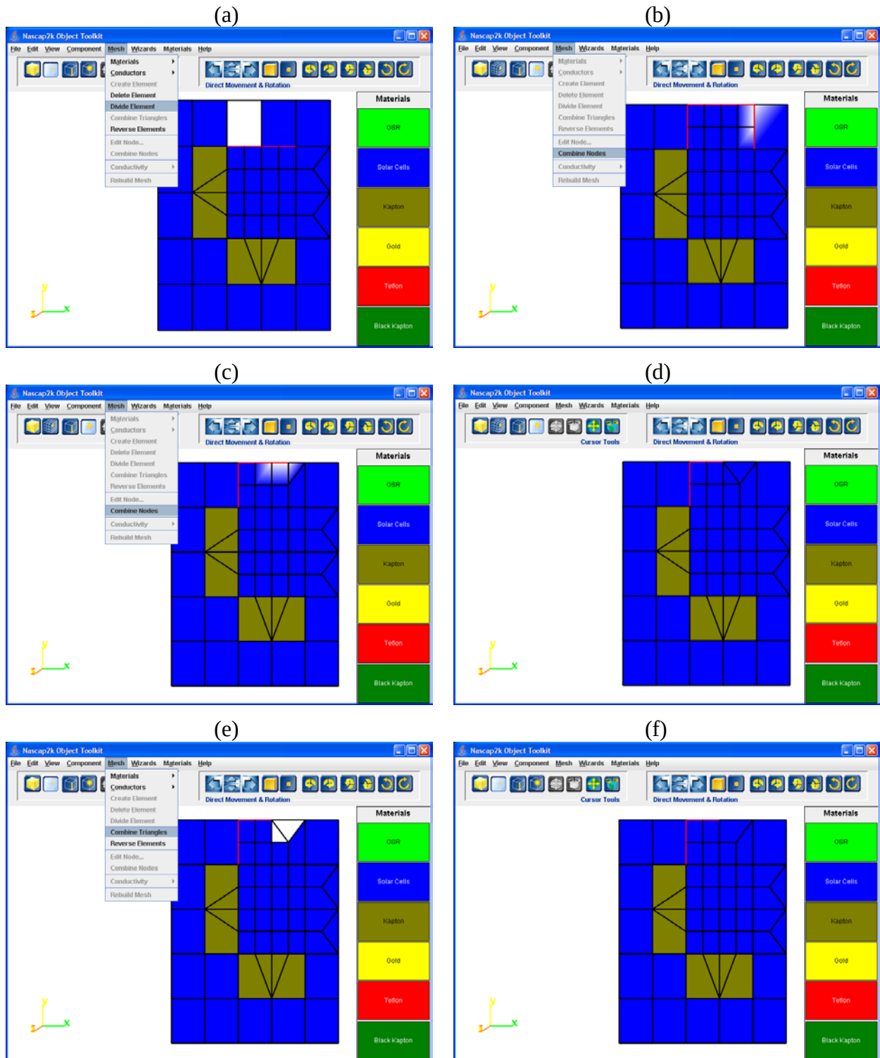
Figure 29. Resolving Incompatibilities by Dividing an Element, Combining Nodes Twice to Create Two Quadrilaterals and Two Triangles, and, Finally, Combining the Two Triangles into a Single Quadrilateral to Give Three Quadrilaterals in Place of the Original Single Element. In e, the Outlines of Elements on the Far Side with Normals Facing into the Screen Are Seen.
