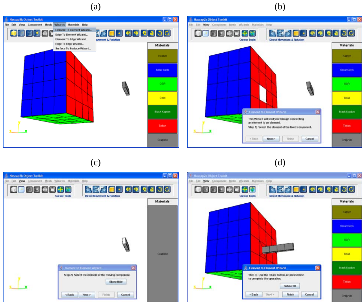
Figure 18. Moving, Aligning, and Grouping Two Components Using the “Element to Element Wizard.” The Four Trapezoidal Elements Belong to the Weld. In the Third Frame, the Fixed Component Is Automatically Hidden.
