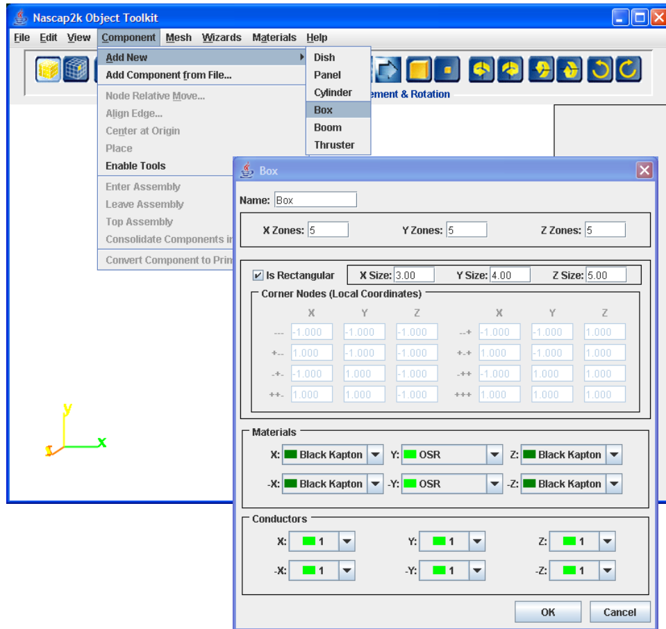
Figure 41. Dialog Box for Creating a Box 3.0 m by 4.0 m by 5.0 m in Size and Five Elements in Each Direction. The \pm Y Sides Are Defined to Be Material OSR and the Other Sides Are Black Kapton.
