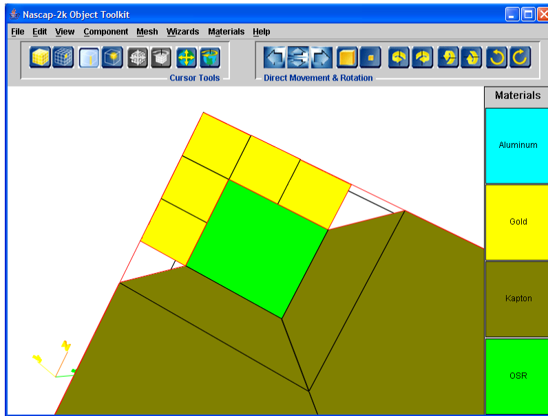
Figure 91. Result after Deleting Seven Small Elements and Replacing Them with Two Compatible, Larger Ones. The Outlines of Elements with Normals Facing into the Screen Are Seen.
