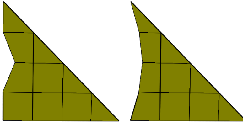
Figure 104. Moving Each Node to Form the Curved Edge by Going to the Mesh Menu and Choosing “Move Node.”
