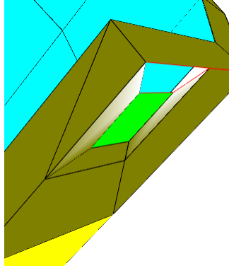
Figure 93. Replacing the Small Elements with Larger Compatible Ones to Form the DSAD Frame. The Outlines of Elements with Normals Facing into the Screen Are Seen.
