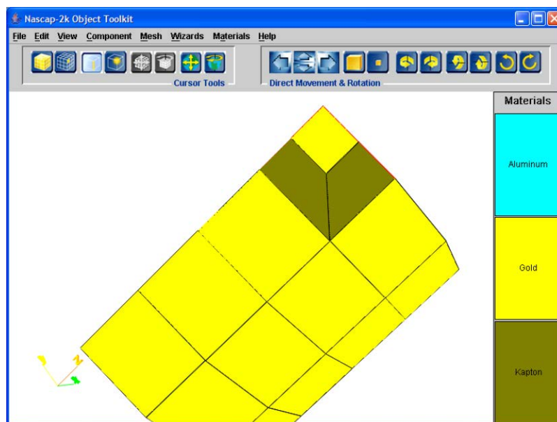
Figure 86. Result after Deleting Three Elements and Replacing Them with Two to Eliminate the Incompatibility along the Face of the Sunshade. Incompatible Elements Remain along the Edge.
