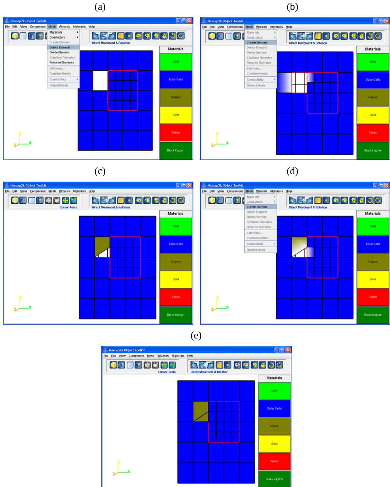
Figure 25. Deleting an Element Using “Delete Element” and Replacing It with a Quadrilateral and a Triangle by Selecting Edges and Using “Create Element” on the Mesh Menu. In b, c, and d, the Outlines of Elements on the Far Side with Normals Facing into the Screen Are Seen.
