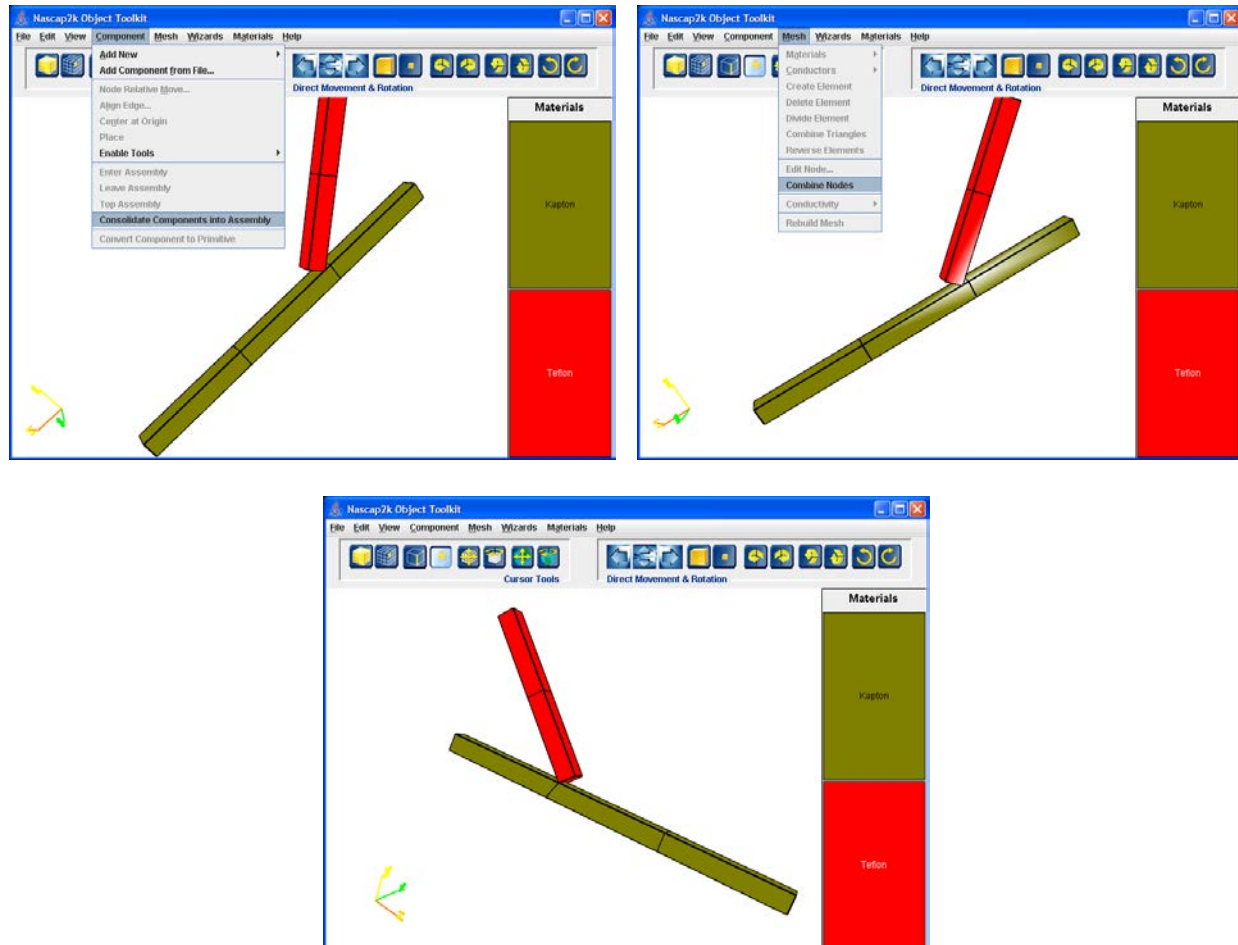
Figure 110. Consolidating Booms into a Single Assembly and Moving Nodes to Coincide.
