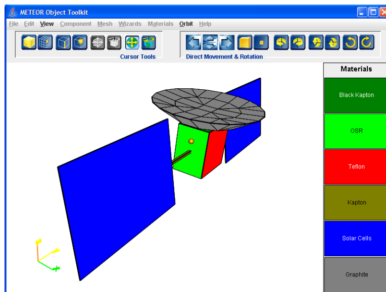
Figure 135. EPIC Object with Rotated Solar Arrays.
