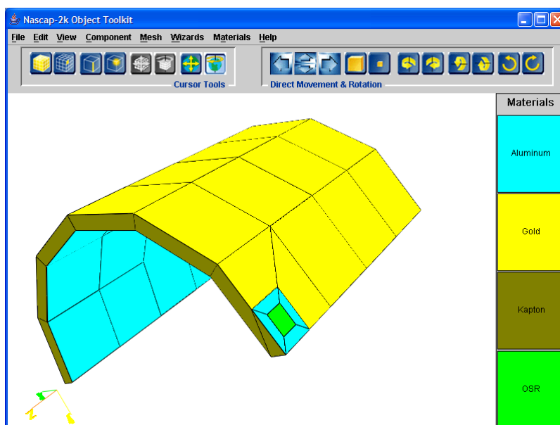
Figure 73. Simplified MESSENGER Sunshade, Including DSAD Instrument, to Be Built in this Example.
