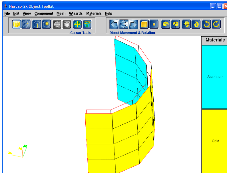
Figure 82. Resulting Inner and Outer Surfaces of the Sunshade. The Outlines of Elements with Normals Facing into the Screen Are Seen.
