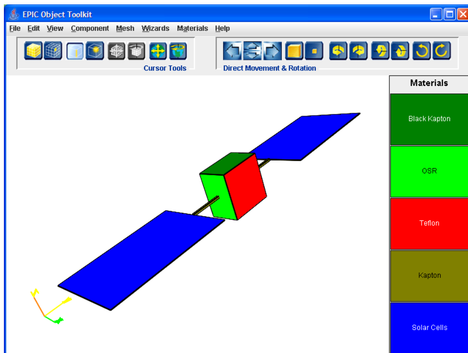
Figure 127. EPIC Object Colored by Material Name.
