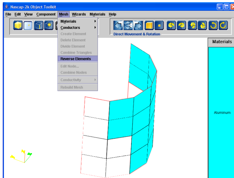
Figure 78. Reversing the Normal of the Elements. In the Figure, Some of the Distant Elements Have Already Been Reversed and Some of the Near Ones Have Been Selected and Are About to Be Reversed. The Outlines of Elements with Normals Facing into the Screen Are Seen.
