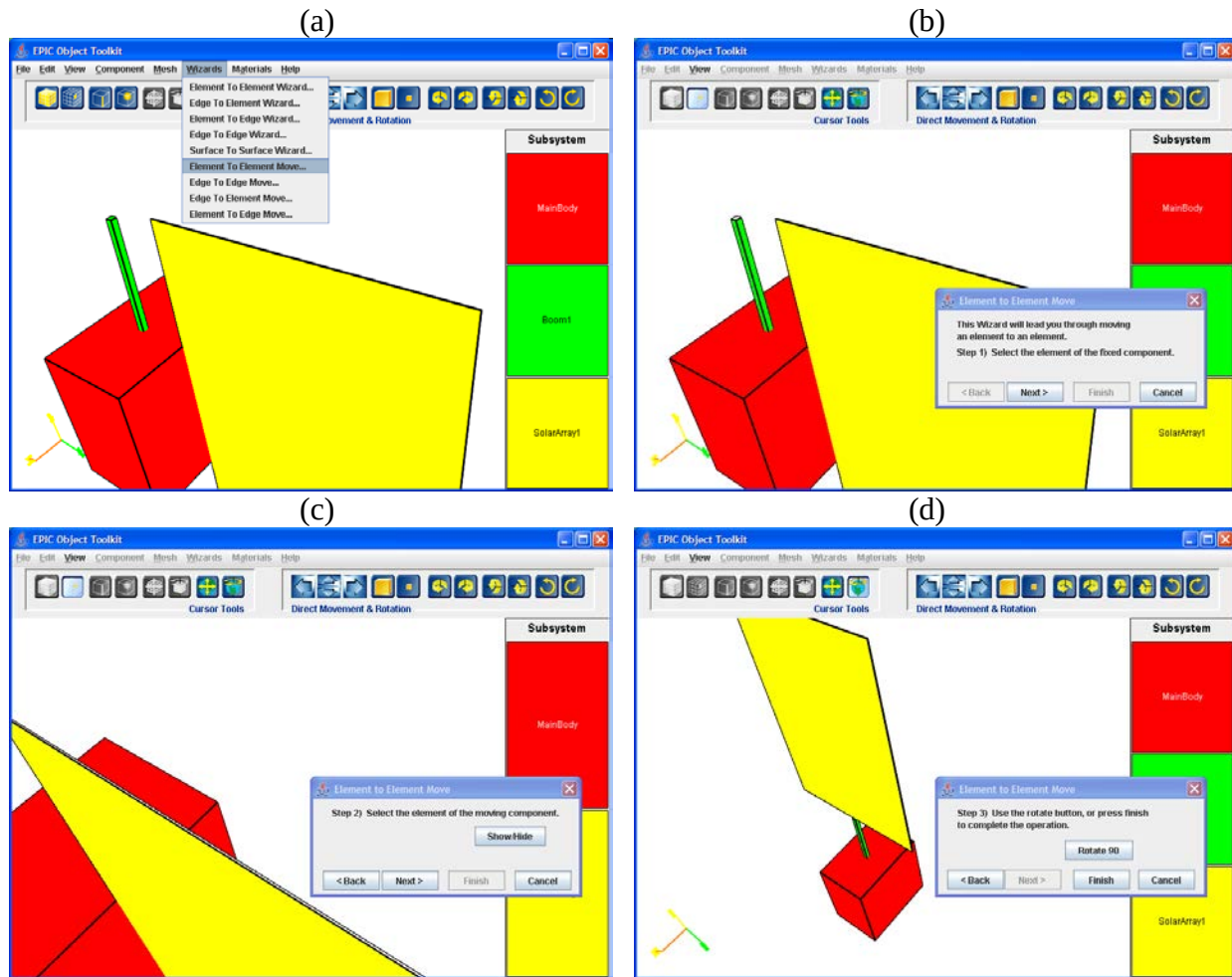
Figure 125. Placing the Solar Array at the End of the Boom Using the “Element to Element Move Wizard.”
