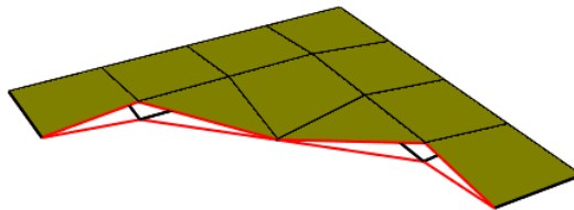
Figure 100. Closing the Open Edge in the Center By Going to the Mesh Menu and Choosing “Combine Nodes.” The Outlines of Elements with Normals Facing into the Screen Are Seen.
