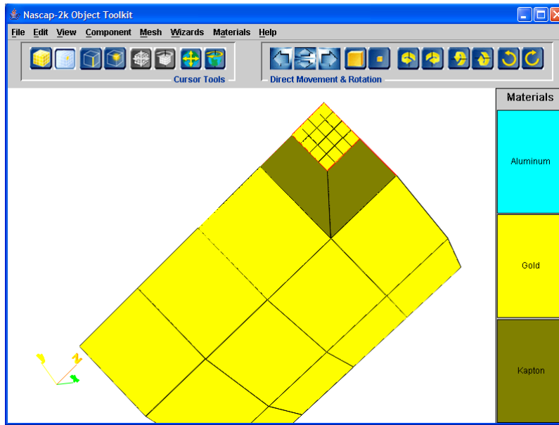
Figure 87. Result after Dividing the Corner Element and Then Dividing Each of the Newly Formed Elements.
