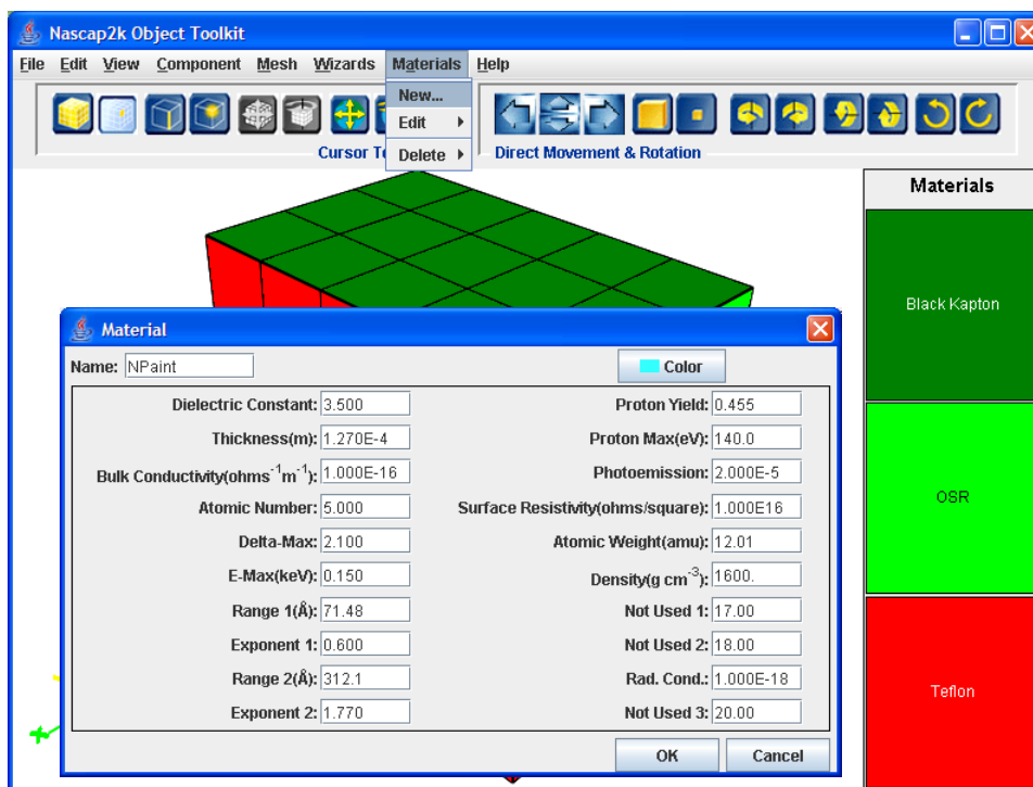
Figure 55. Defining a New Material, NPaint, Which Is Used to Cover the Omni-antenna.
