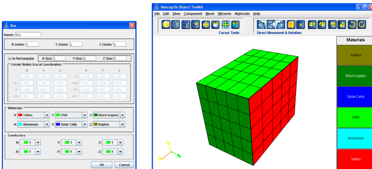
Figure 5. Definition of a 3 m by 4 m by 5 m Rectangular Box with a Different Material on Each Side.
