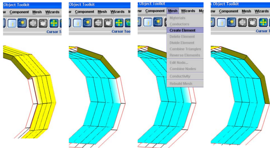
Figure 83. Creating an Element That Joins the Two Sides of the Sunshade. The Outlines of Elements with Normals Facing into the Screen Are Seen.
