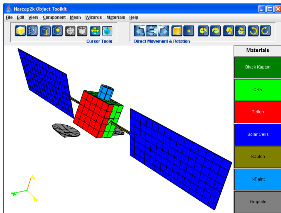
Figure 52. Object Toolkit Model of a Typical Geosynchronous Spacecraft to Be Built in this Example.
