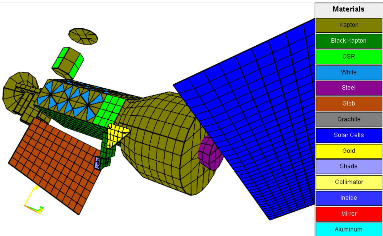
Figure 3. DMSP Spacecraft Model Constructed in Object Toolkit .
