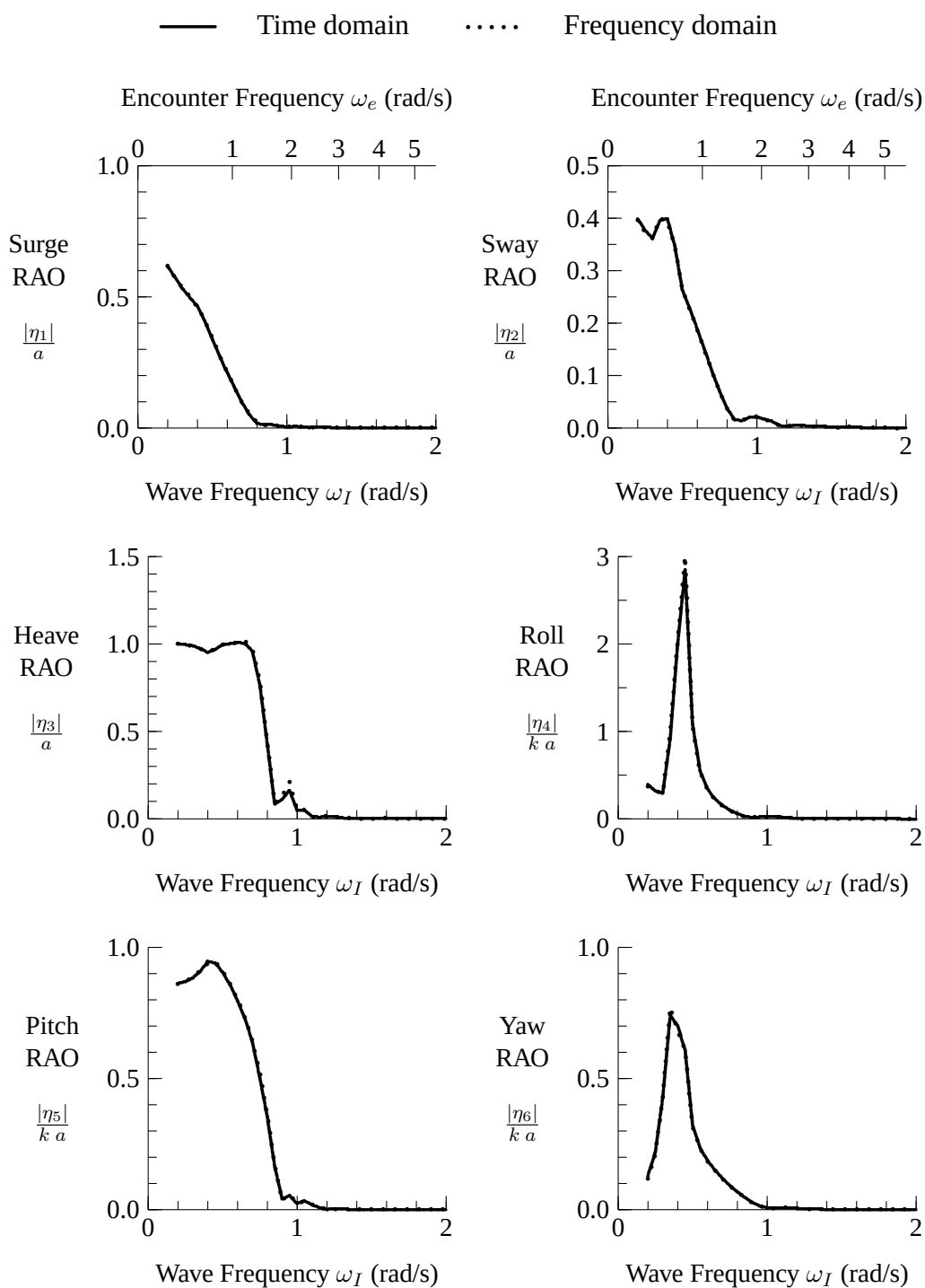
Figure 32: Motions for HALIFAX from Frequency Domain and Time Domain Computations, Medium Mesh, 20 knots, Bow Quartering Seas at 150 degrees
