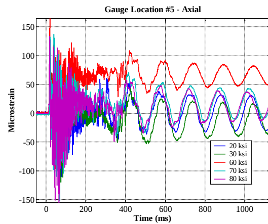
Figure 16. Axial Strains at Gauge Location #5
