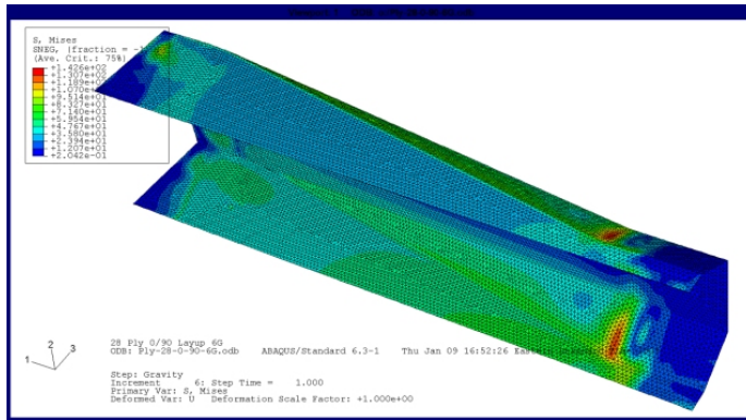
Figure 4. Stresses in the composite shell under a 6 g loading using smeared properties
