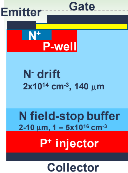
SiC N-IGBT Structure
