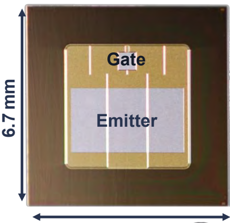
SiC N-IGBT Structure
