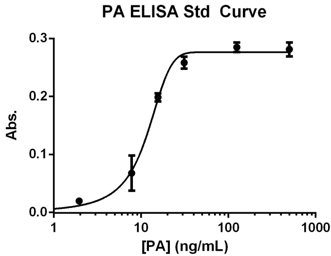
Figure 4. Standardized ELISA for HSA/PA detection in mouse tissues. Standard curve showing ability to assay PA by ELISA.
