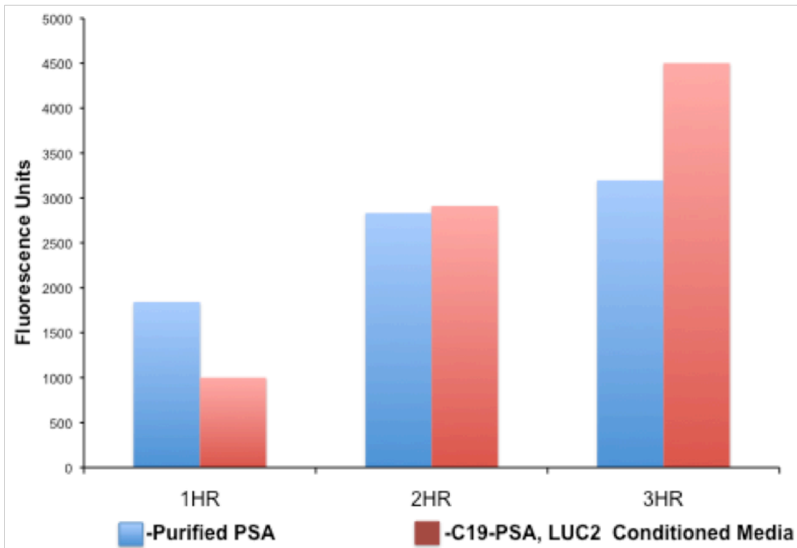
Figure 7. PSA activity assay. Conditioned media from C19 cells transduced to constitutively express PSA was collected and pooled. Activity of secreted PSA was determined using an AMC linked substrate specific for PSA. Activity of C19 secreted PSA is compared with 1ug of purified Human PSA.
