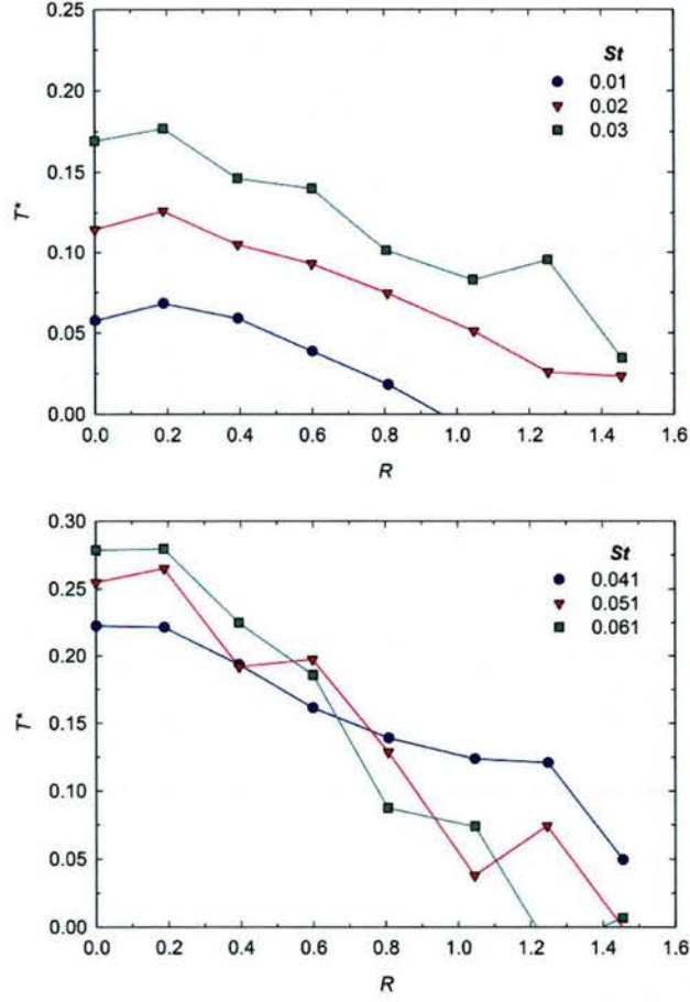
Fig. 13. Scaled thrust as a function of crossflow velocity ratio.
