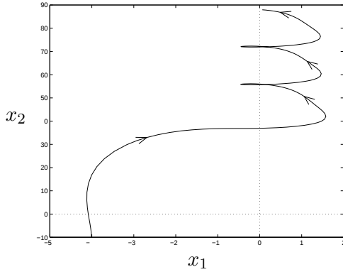
Figure 1.4: Nominal design.
