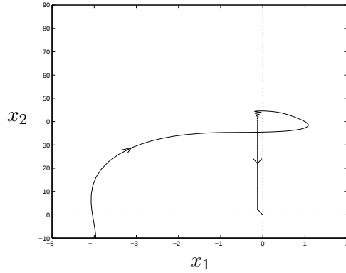
Figure 1.5: Robust redesign.
