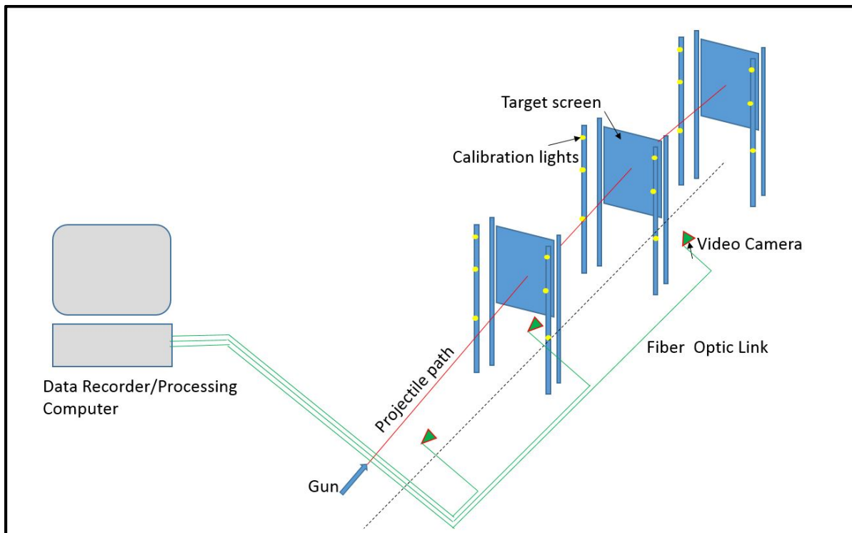
Figure 1. Multi-target setup.
