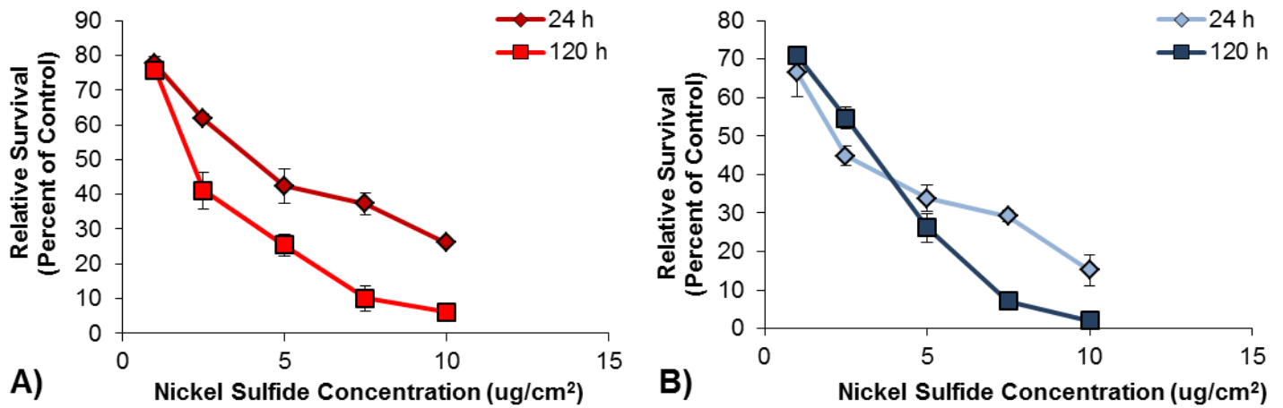
Figure 25. Cytotoxicity of Nickel Sulfide in Human Lung Fibroblast and Epithelial Cells. This figure shows that nickel subsulfide induced a concentration-dependent increase in cytotoxicity in human lung cells after a 24 or 120 h exposure. A) Human lung fibroblasts. B) Human lung epithelial cells. Data represent an average of 3-5 experiments +/- the standard error of the mean.
