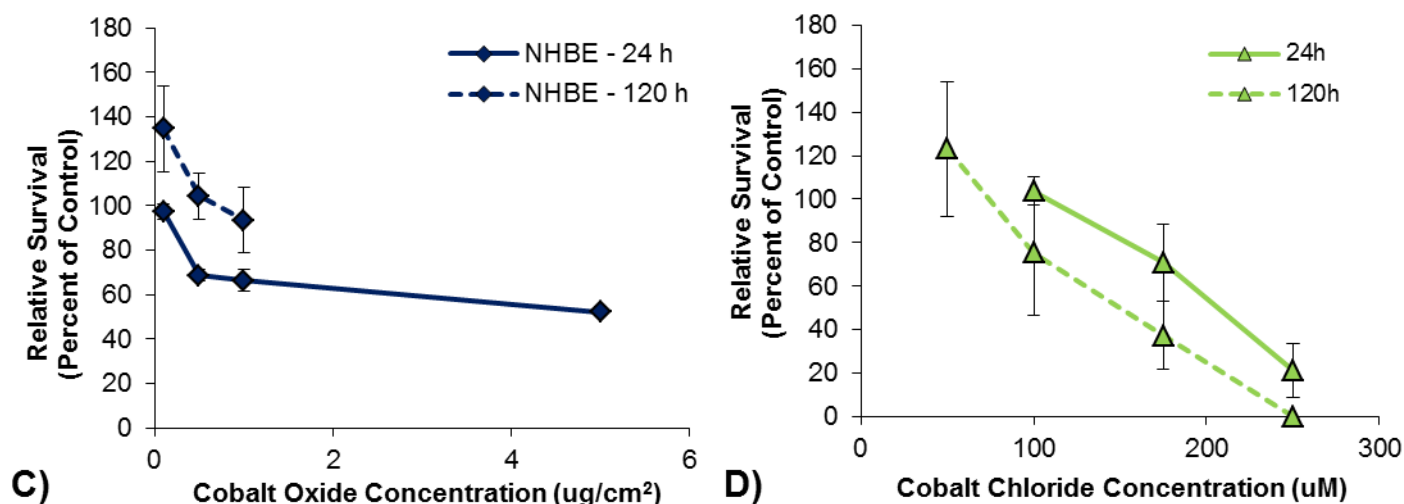
Figure 26. Cytotoxicity of Particulate and Soluble Cobalt in Human Lung Cells. This figure shows that cobalt induced a concentration-dependent increase in cytotoxicity in human lung cells. A) Cobalt oxide-induced cytotoxicity in human lung fibroblast cells after 24 or 120 h exposure. B) Cobalt chloride-induced cytotoxicity in human lung fibroblast cells after 24 or 120 h exposure. C) Cobalt oxide-induced cytotoxicity in human lung epithelial cells (NHBE) after 24 or 120 h exposure. D) Cobalt chloride-induced cytotoxicity in human lung epithelial cells (NHBE) after 24 or 120 h exposure. Data represent an average of 2-3 independent experiments +/- the standard error of the mean.
