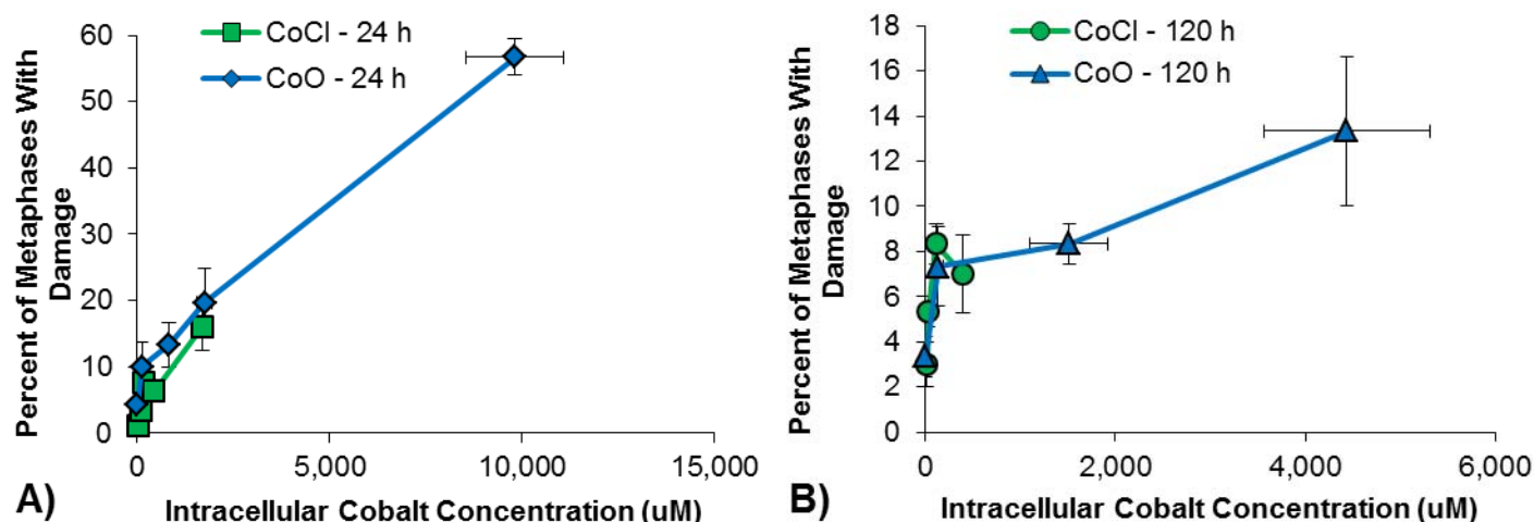
Figure 44. Comparison of Particulate and Soluble Cobalt-Induced Clastogenicity. Particulate and soluble cobalt induced similar levels of chromosome damage based on intracellular cobalt levels. Cell cycle arrest was observed at a lower intracellular cobalt level with cobalt chloride compared to cobalt oxide. A) 24 h. B) 120 h. Data represent an average of 3 independent experiments \pm the standard error of the mean.
