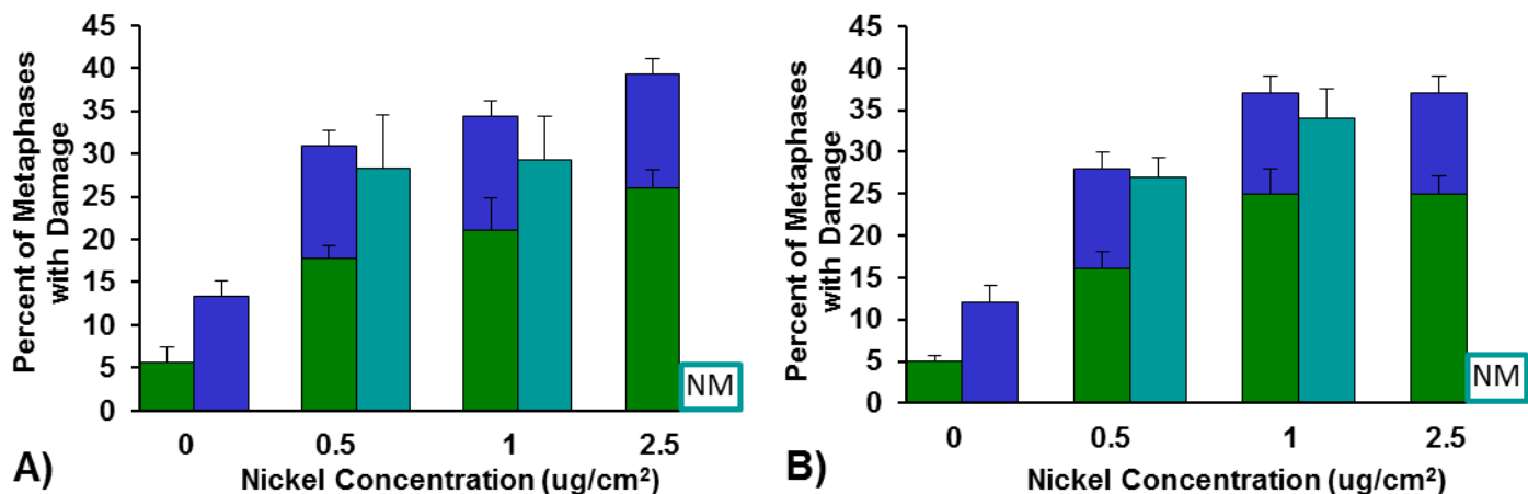
Figure 45. Clastogenicity of Nickel and Cobalt Co-Exposure in Human Lung Epithelial Cells. This figure shows the clastogenicity of nickel and cobalt co-treatments in human lung epithelial cells. A) 24 h. B) 120 h. NM = no metaphases. Data represent an average of 3 independent experiments +/- the standard error of the mean.
