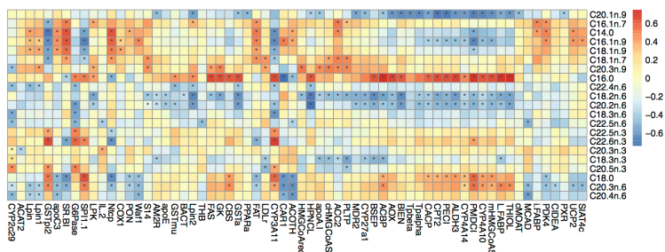
Figure 3: HALLA identifies validated and novel associations between mouse liver transcripts and fatty acid levels. Associations between hepatic fatty acids and gene expression in data from Martin et al (Hepatology 2007). '*' indicates significant associations identified by HALLA between corresponding genes and fatty acids, a strict superset of those previously reported.
