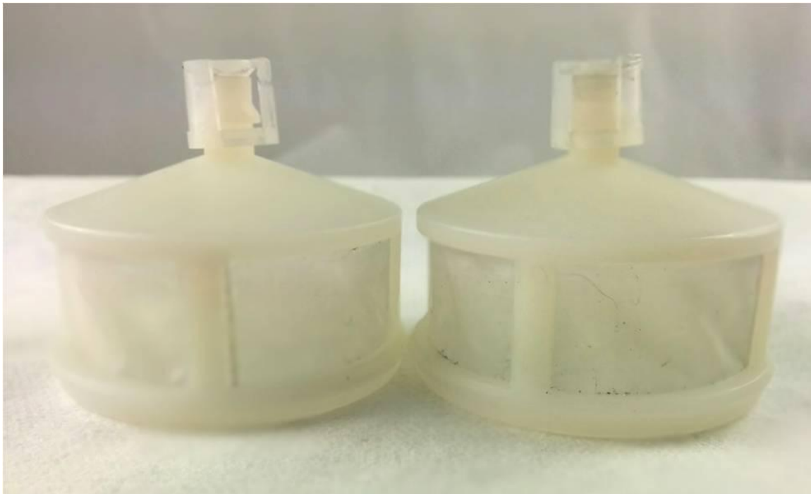
Figure 25. Two Filter Elements from 20,000-cycles of DOT III Fluid Testing
