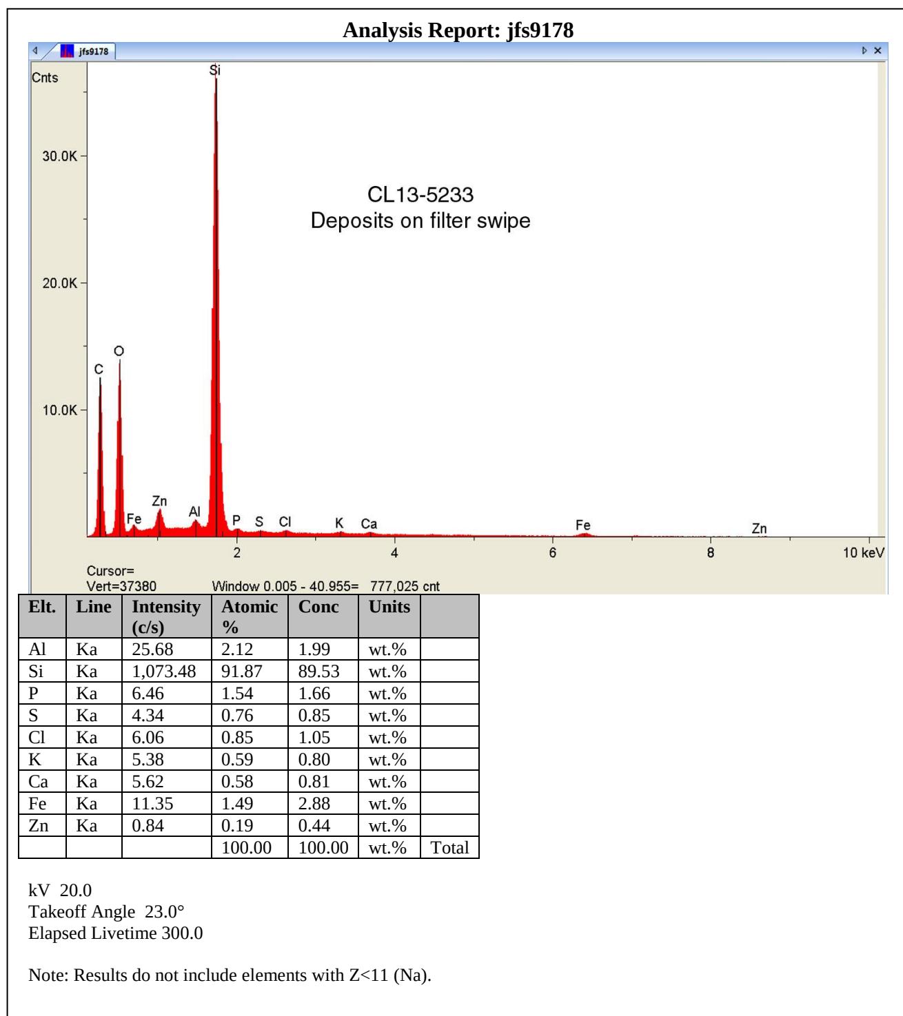
Figure 13. Surface Scan jfs9178 Elemental Analysis
