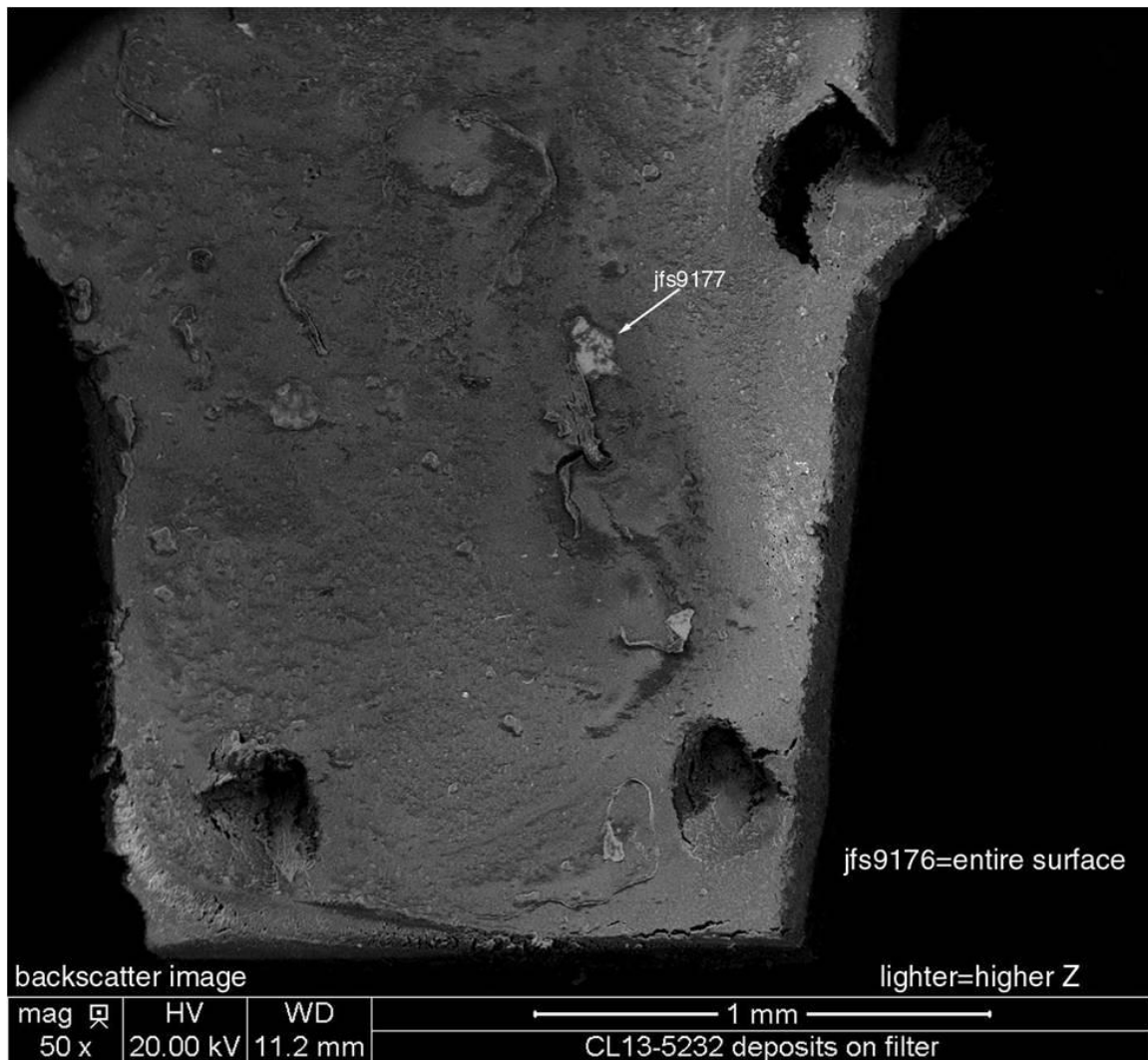
Figure 8. Backscatter SEM Image showing Elemental Analysis Scan Locations
