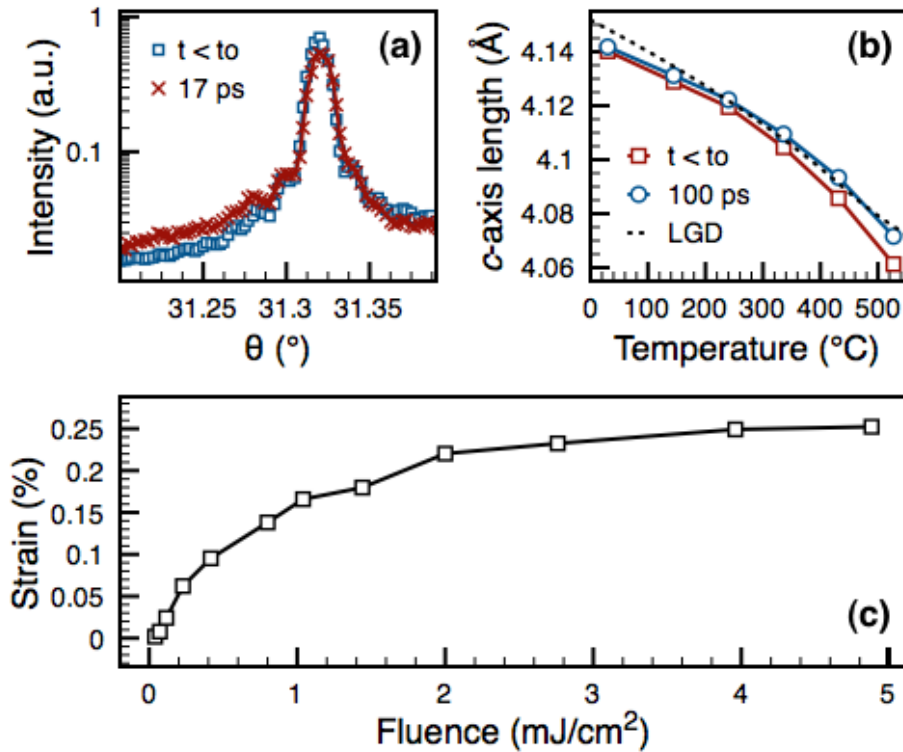
FIG. 4. Role of depolarization field in photovoltaic response. (a) PTO (003) on DSO in the paraelectric phase at 479° C, slightly above T_C (incident fluence = 5 mJ/cm 2 ). Only small \theta shifts are seen due to the centrosymmetric, paraelectric unit cell. (b) LGD theory calculation, comparing the observed c -axis lattice parameter of PTO on STO at t < t_0 and t = 100 ps (incident fluence = 4 mJ/cm 2 ) to the predicted zero-field c -axis parameter. (c) Strain in the c -axis parameter of monodomain PTO on STO at 550° C as a function of fluence, measured at t = 100 ps. Saturation behavior in the maximum drivable strain is seen.
