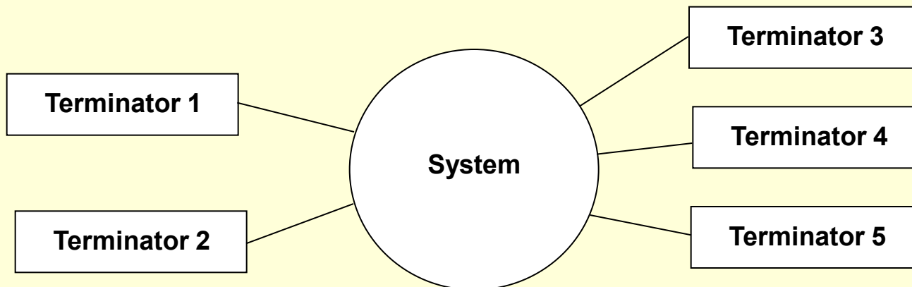
The Modern Structured Analysis View of a System The Context Diagram
