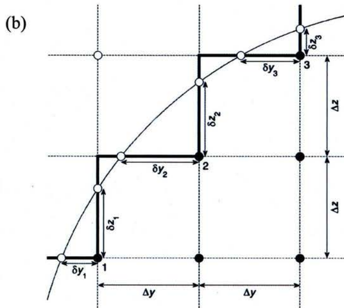
Figure 7. (a) The alternating direction implicit (ADI) method with a nonplanar surface, and (b) the boundary fitted grid for handling surface wave boundary conditions.
