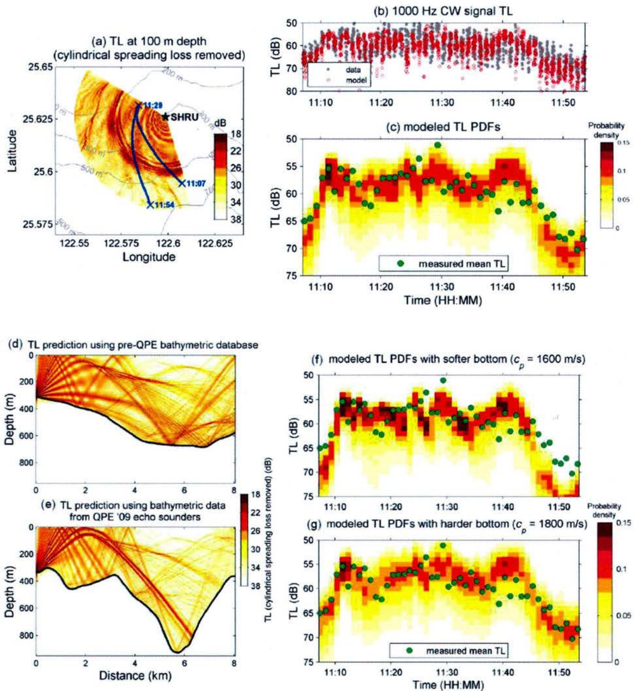
Figure 10. 3-D PE model TL and data comparison for the mobile source transmission in the QPE experiment over North Mein-Hua Canyon.
