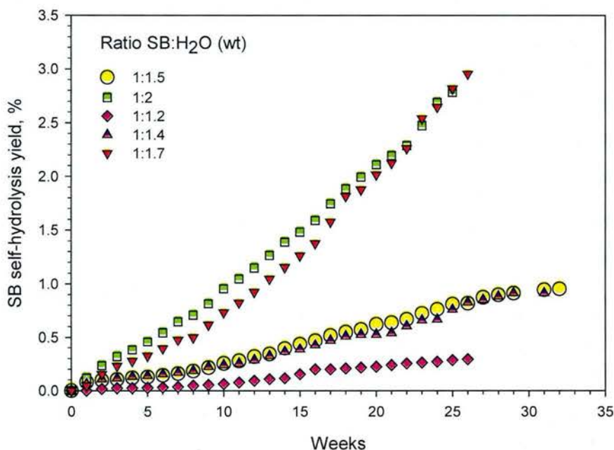
Fig. 11. Kinetics of \text{NaBH}_4 self-hydrolysis at different \text{NaBH}_4 : \text{H}_2\text{O} ratios in the stabilized slurry. Amount of NaOH stabilizer in the slurry: 7.3-8.8 wt.%. Room temperature.
