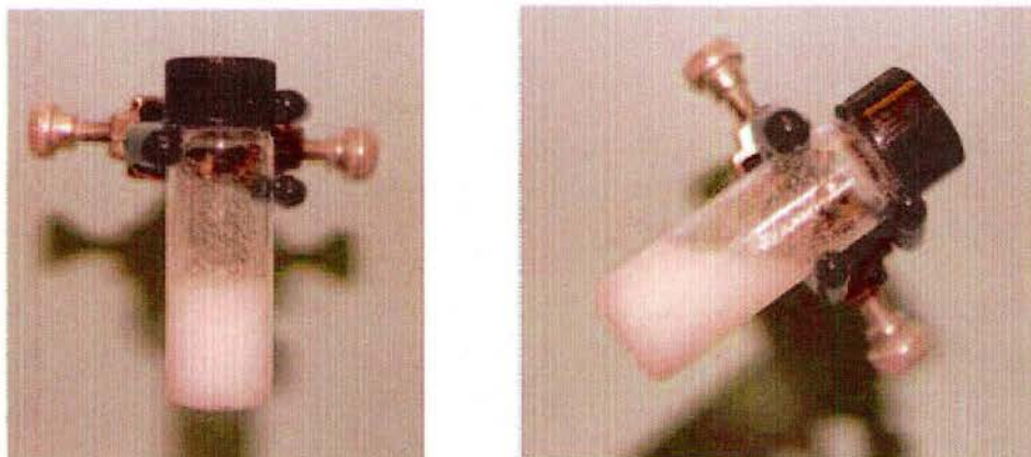
Fig. 12. NaBH 4 slurry in Tetra-EGDME. Ratio NaBH 4 : Tetra-EGDME=1:1.6 wt.
