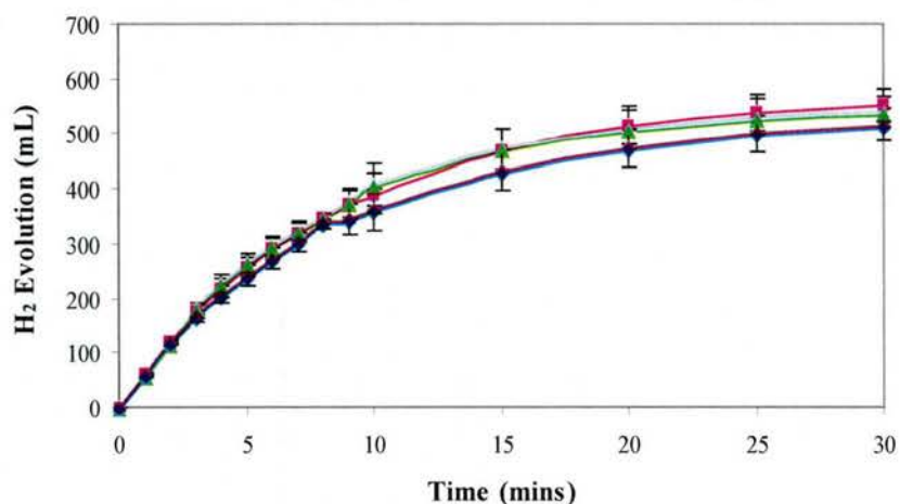
Fig. 30. Experimental margin of error in \text{H}_2 evolution measurements via Al- \text{NaBH}_4 hydrolysis
