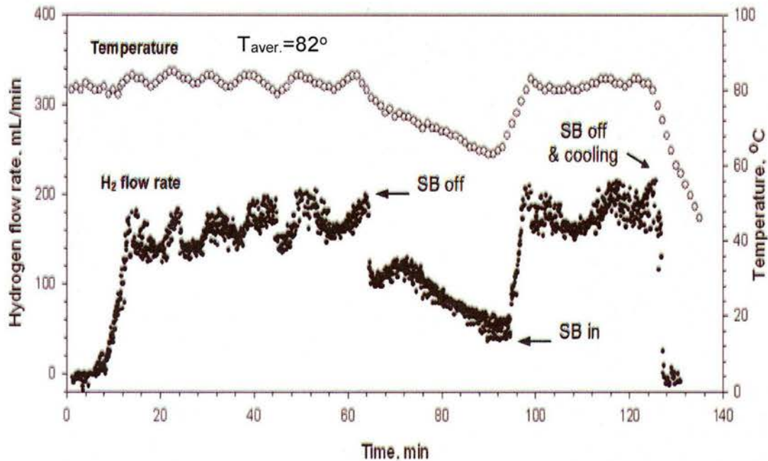
Fig. 23. Continuous production of hydrogen by Al- \text{NaBH}_4 hydrolysis at 82°C using a glass reactor.
