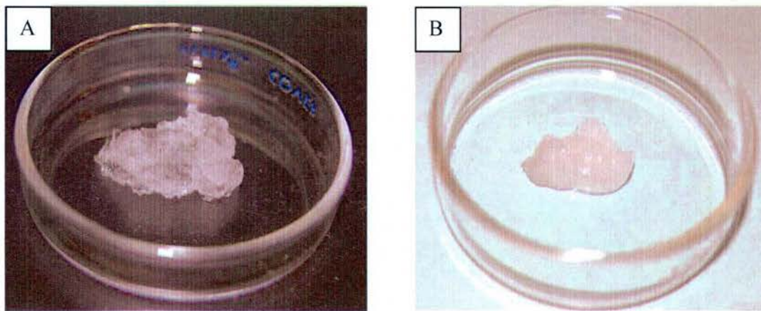
Fig. 7. NaBH 4 storage in gel form. A- a gel produced by adding 2% wt. of gelling polymer to deionized water. B- NaBH 4 gel produced by adding 3.5% wt. of gelling polymer to stabilized NaBH 4 :H 2 O=1:1.5 (wt) solution.
