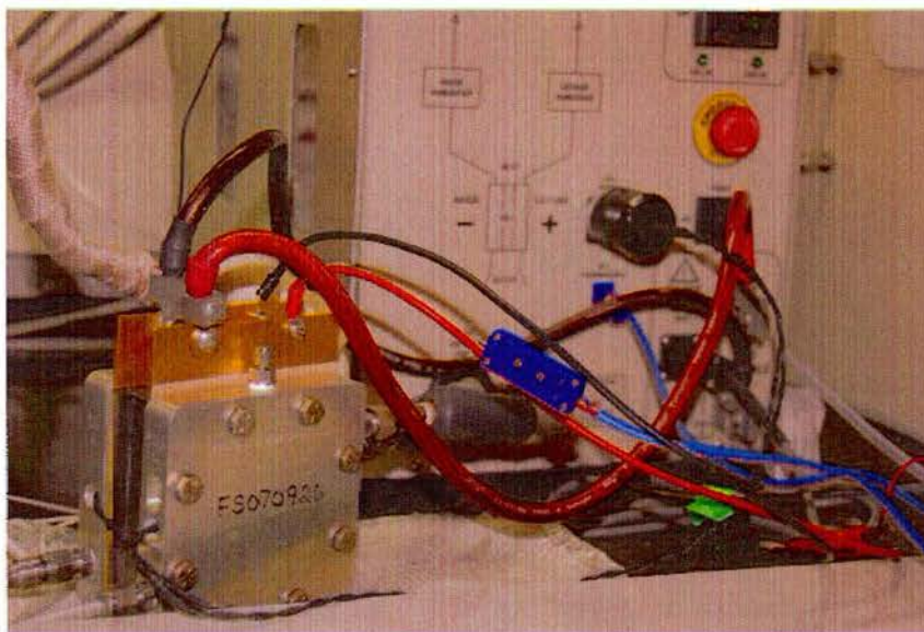
Fig. 27. A single-cell PEMFC and Scribner 850C testing station used in the experiments
