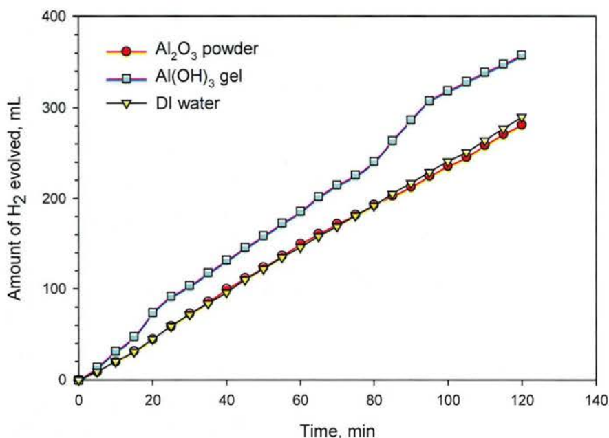
Fig. 19. Effect of Alumina (Al 2 O 3 ) powder and Al hydroxide gel on the kinetics of H 2 release from NaBH 4 solutions in DI water. Amount of Al oxide and hydroxide: 0.3 g. T= 80°C.
