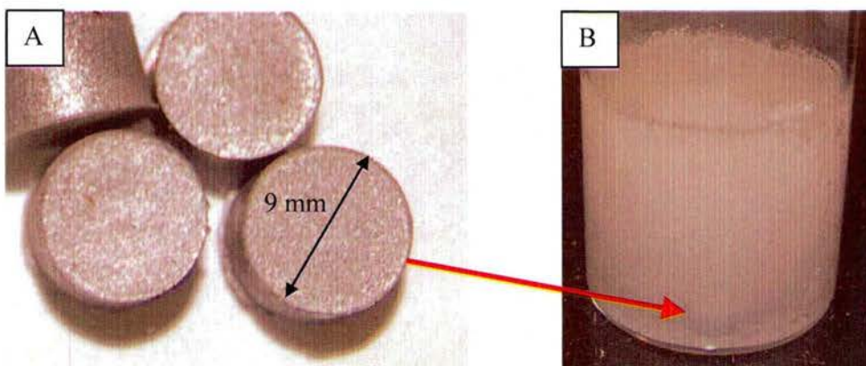
Fig. 5. Al-NaBH 4 tablets used for production of pure hydrogen from water. A- Tablets Al:NaBH 4 =1:2 (by wt). Tablets weigh 0.55-0.65 g. B- a tablet reacts with water after 3 months storage.
