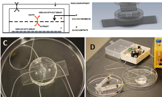
Figure 21 Miniaturized bioreactor. The reactor was made as described in the legend to the image.
