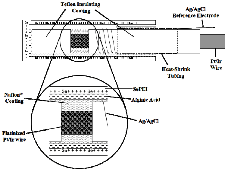
Figure 4. Schematic of needle type NO/RSNO sensor developed to measure NO/RSNO levels in SQ fluid.
