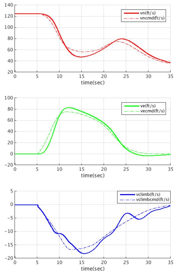
Figure 2. Velocity tracking
