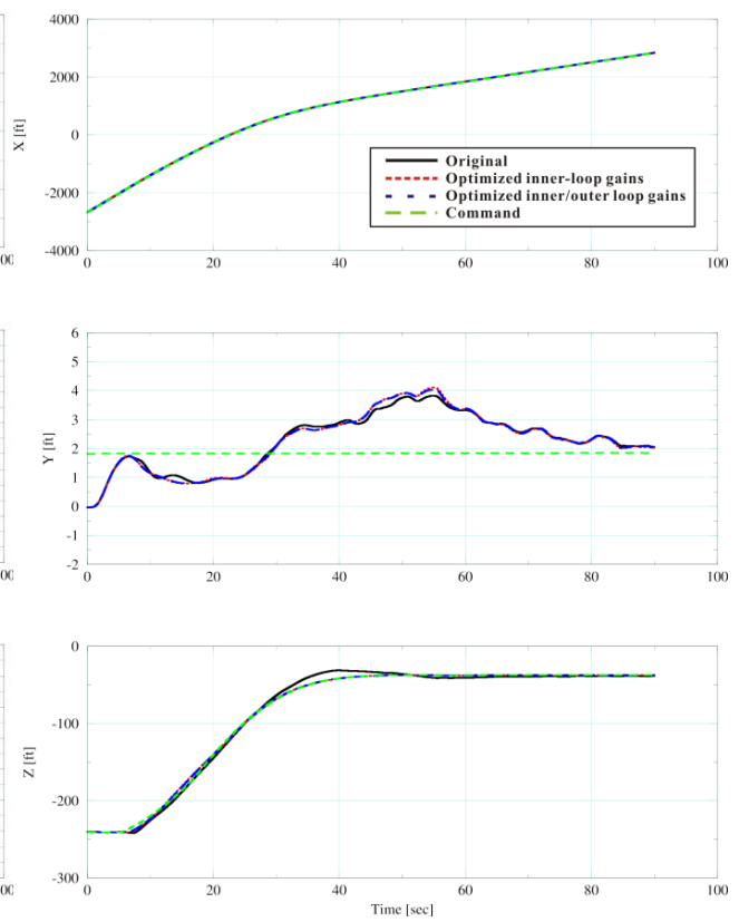
Figure 13 Aircraft position
