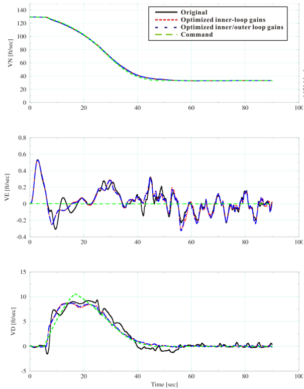
Figure 14 Aircraft velocity
