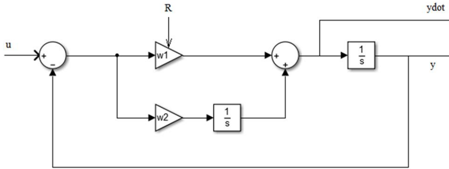
Figure 9. 2nd order low pass filter with tuned parameter
