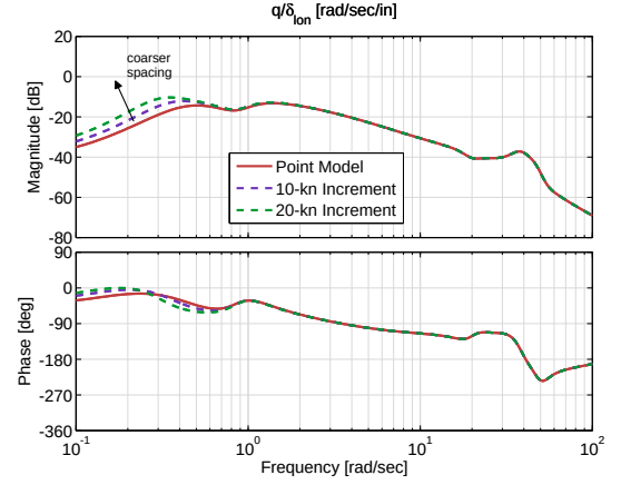
Figure 4.23: Pitch rate response to longitudinal cyclic input comparison for forward-flight trim data of 10- and 20-kn spacing, 40 kn.
