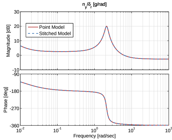
Figure 3.16: Case 1: lateral acceleration response to rudder input comparison.
