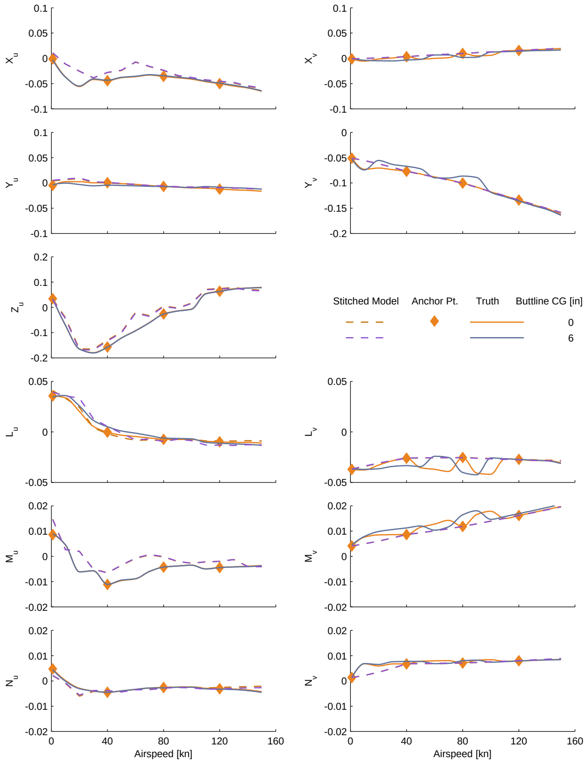
Figure C.15: Verification of off-nominal buttline CG extrapolation, UH-60 stitched model, stability derivatives.
