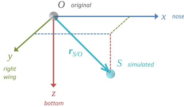
Figure 2.14: Simulated CG location axis convention.
