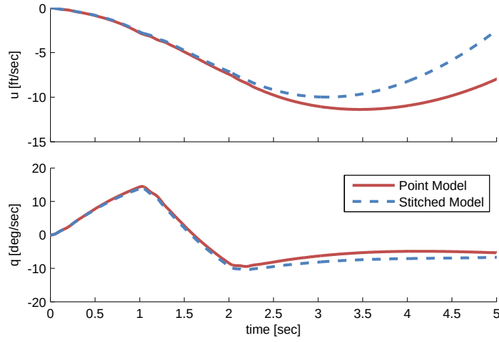
Figure 4.42: Case 1: short-term time history responses, longitudinal cyclic doublet.
