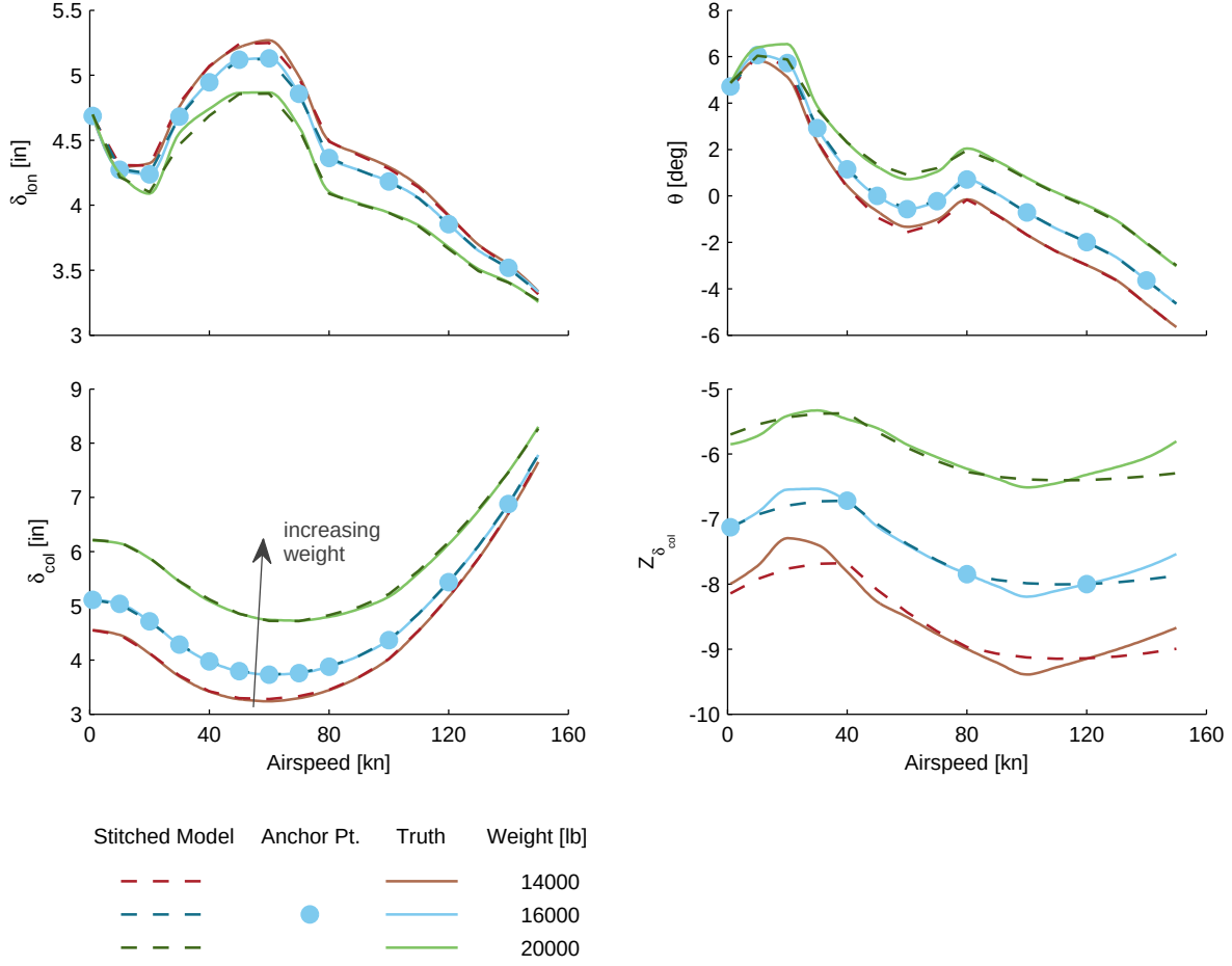
Figure 4.30: Verification of off-nominal weight extrapolation.
