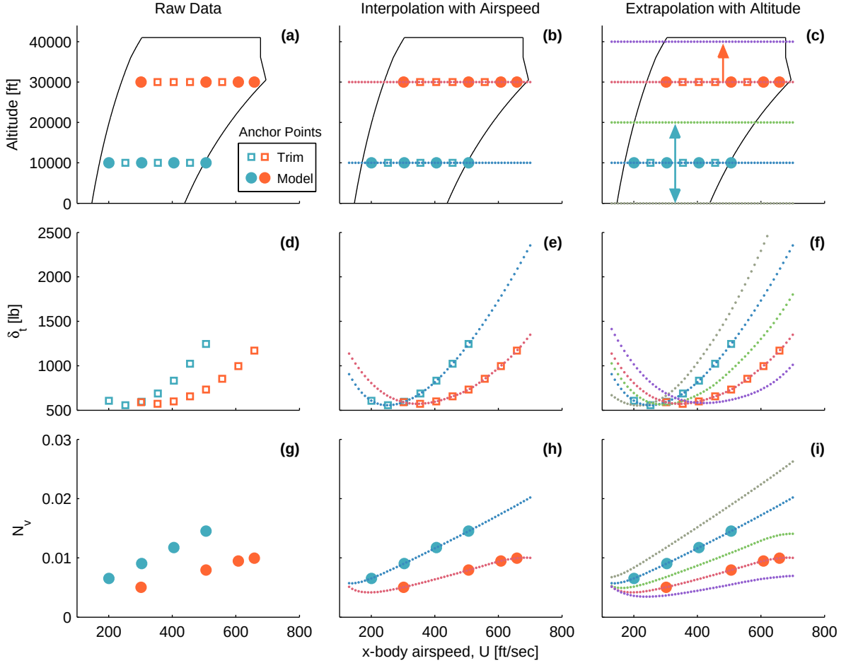
Figure 3.3: Spline-fit data and air density-ratio extrapolation to cover entire flight envelope.
