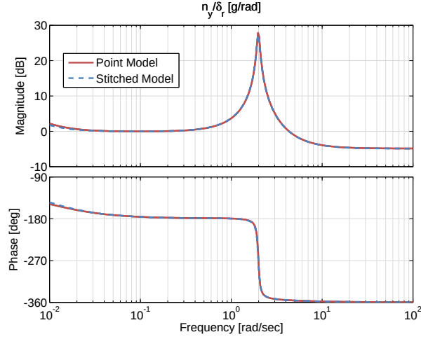
Figure 3.27: Case 2: lateral acceleration response to rudder input comparison.
