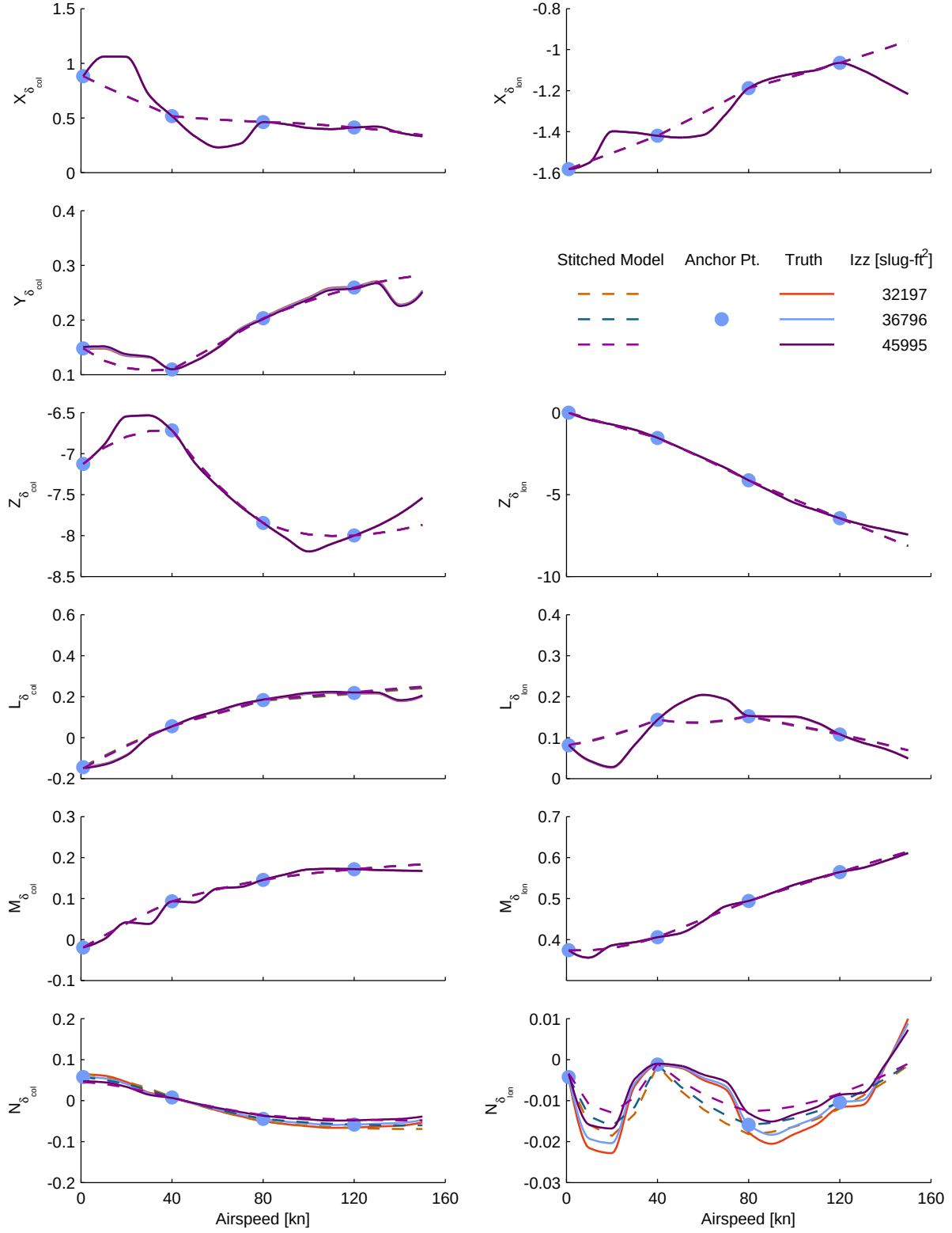
Figure C.10: Verification of off-nominal yaw inertia extrapolation, UH-60 stitched model, control derivatives.
