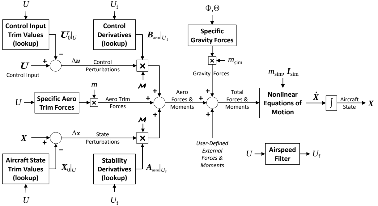
Figure 2.2: Model stitching simulation architecture – top level schematic.
