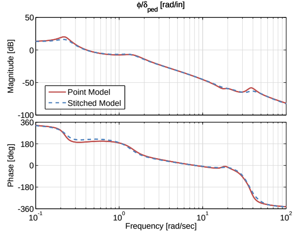
Figure 4.52: Case 2: bank angle response to pedal input comparison.
