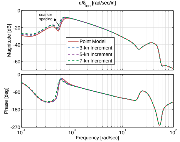
Figure 4.11: Pitch rate response to longitudinal cyclic input comparison for sideward trim data of various spacing, hover.
