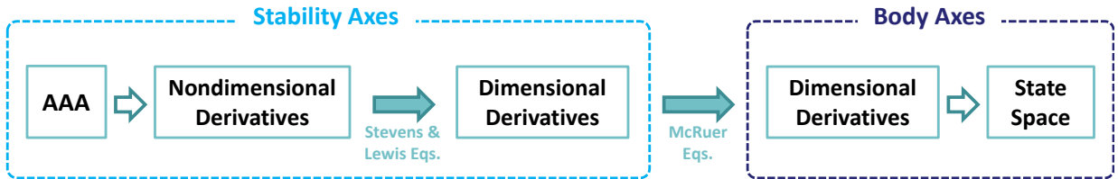
Figure 3.2: Transformation of stability and control derivatives from stability axes to body axes.
