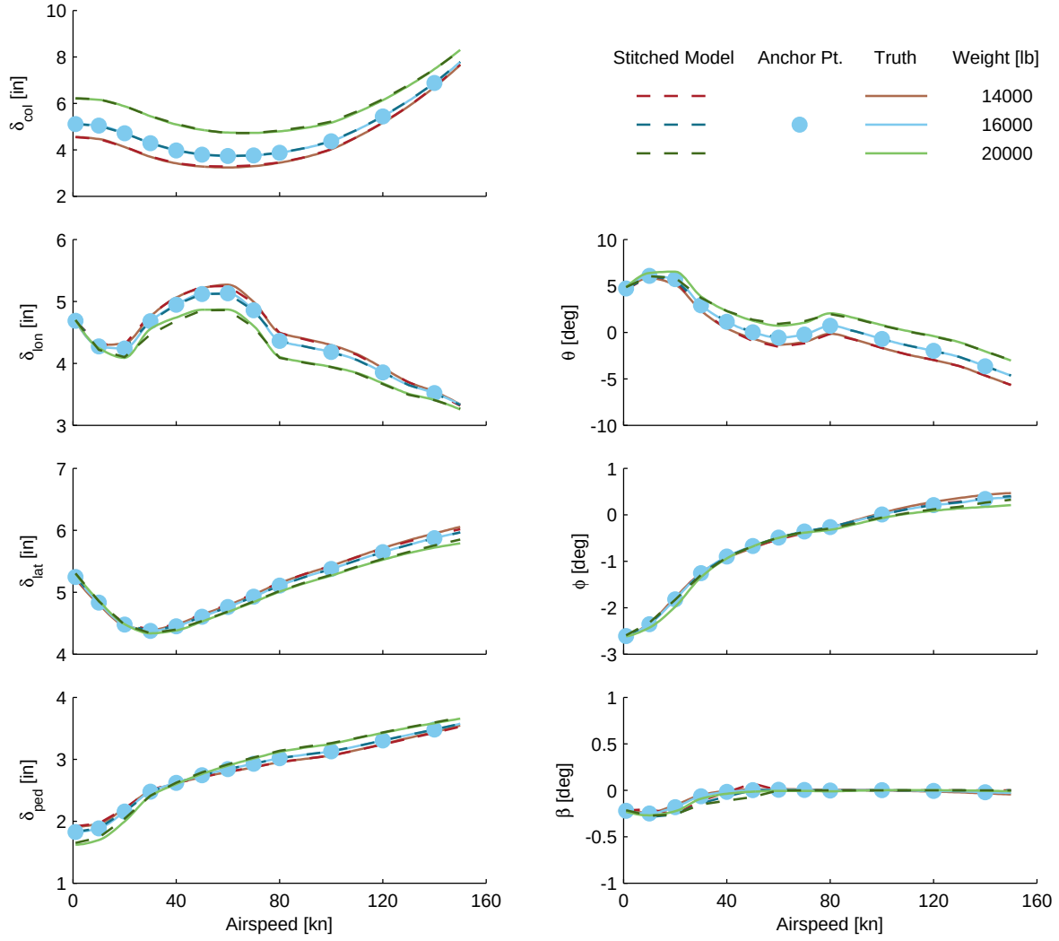
Figure C.1: Verification of off-nominal weight extrapolation, UH-60 stitched model, trim.
