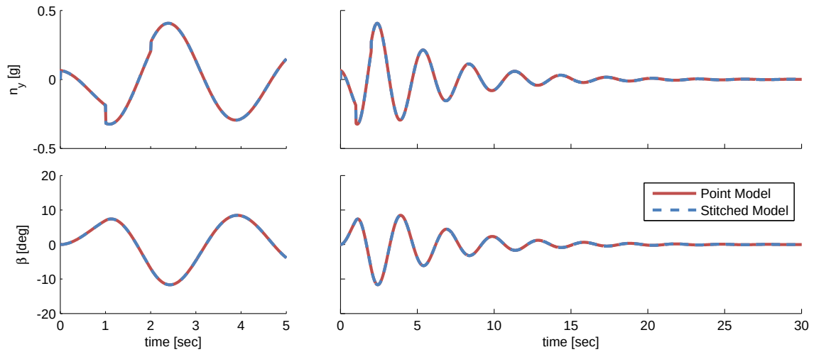
Figure 3.20: Case 1: short- and long-term time history responses, rudder doublet.
