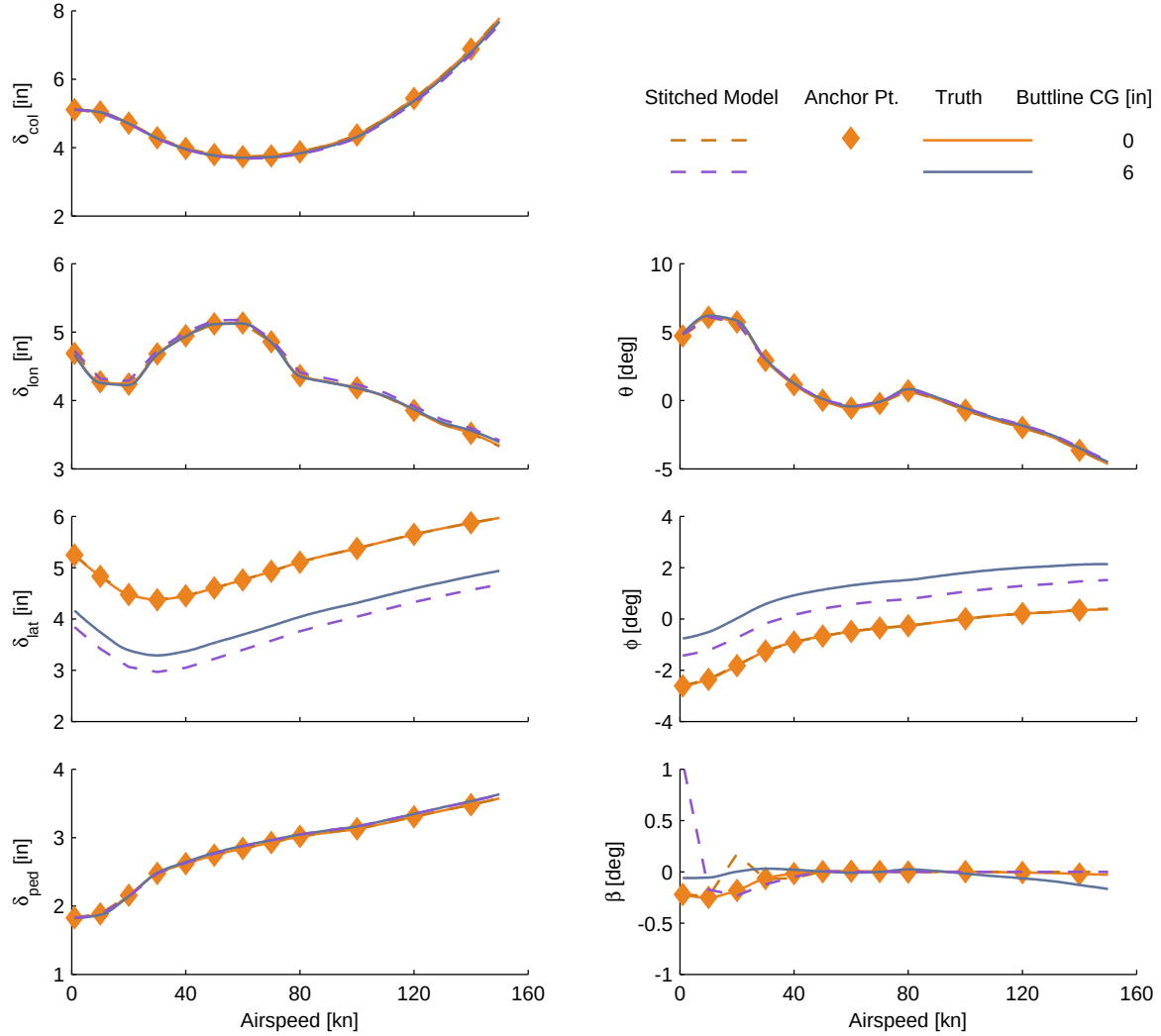
Figure C.14: Verification of off-nominal buttlane CG extrapolation, UH-60 stitched model, trim.
