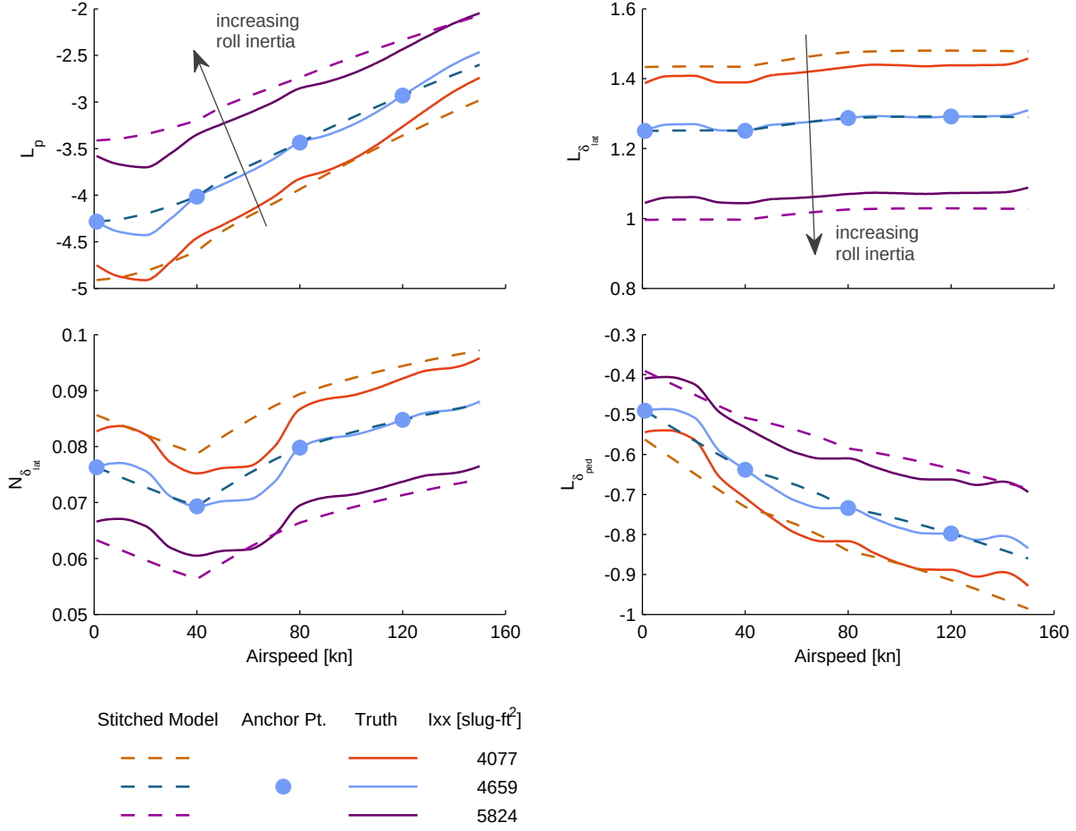
Figure 4.31: Verification of off-nominal inertia extrapolation, roll inertia I_{xx} .
