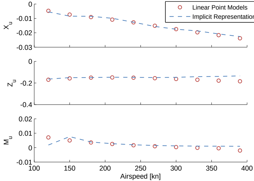
Figure 2.1: Implicit vs. explicit values of u -speed derivatives, CJ1 stitched model.
