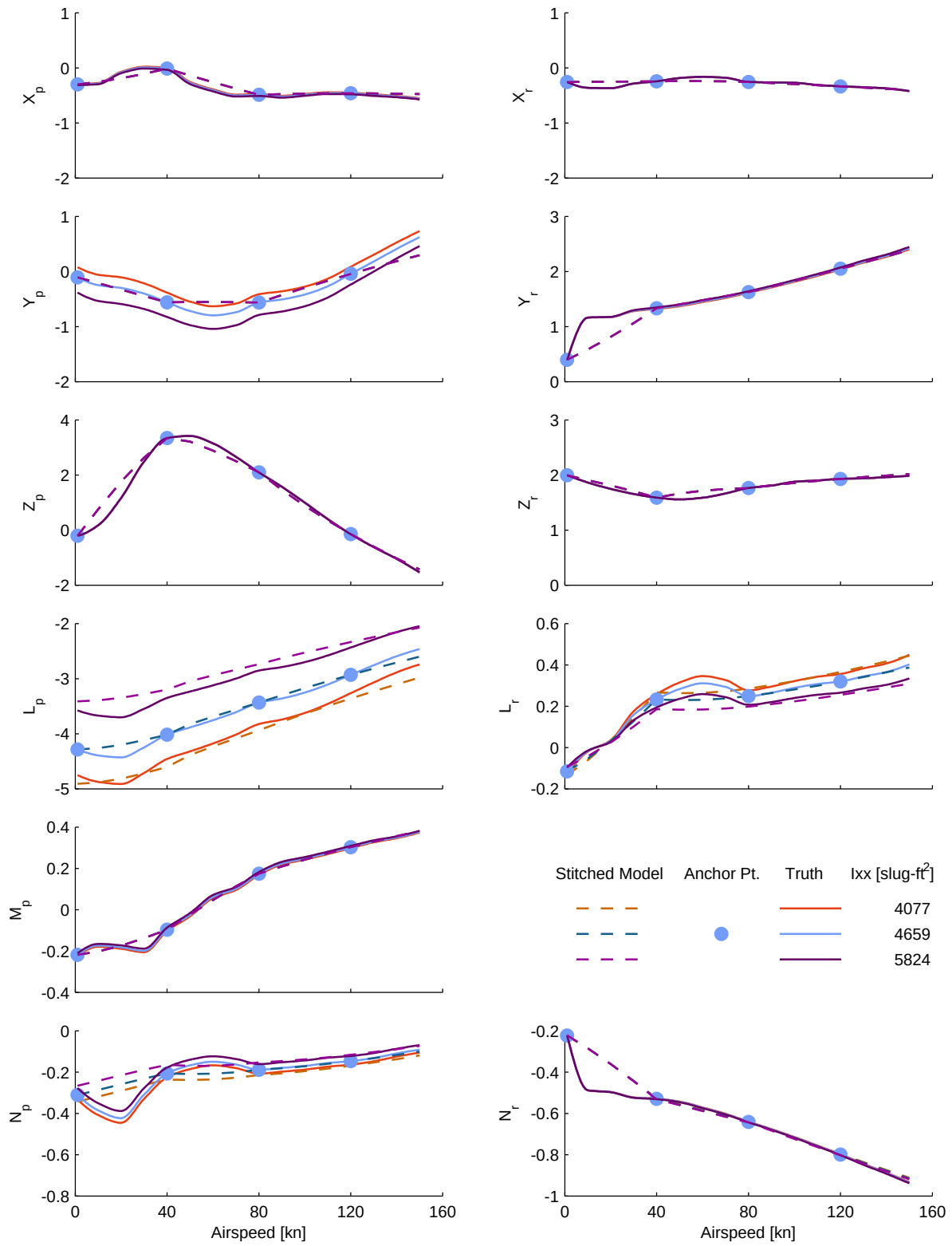
Figure C.5: Verification of off-nominal roll inertia extrapolation, UH-60 stitched model, stability derivatives (cont.)
