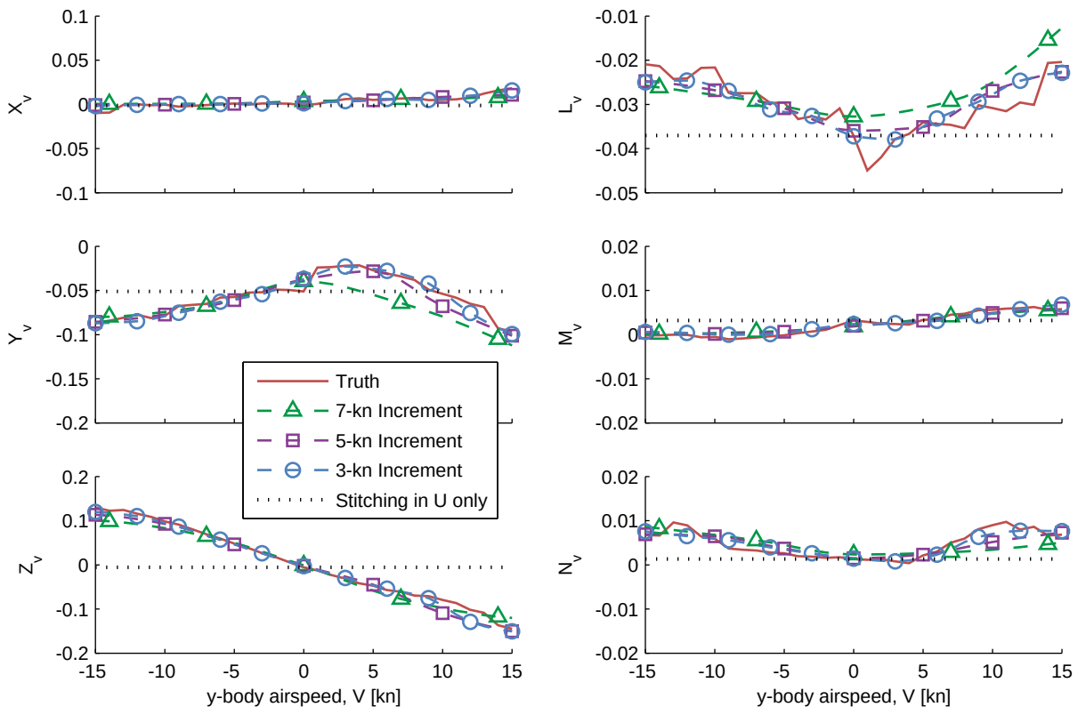
Figure 4.9: Implicit v -speed derivative values due to sideward flight trim data of various spacing.
