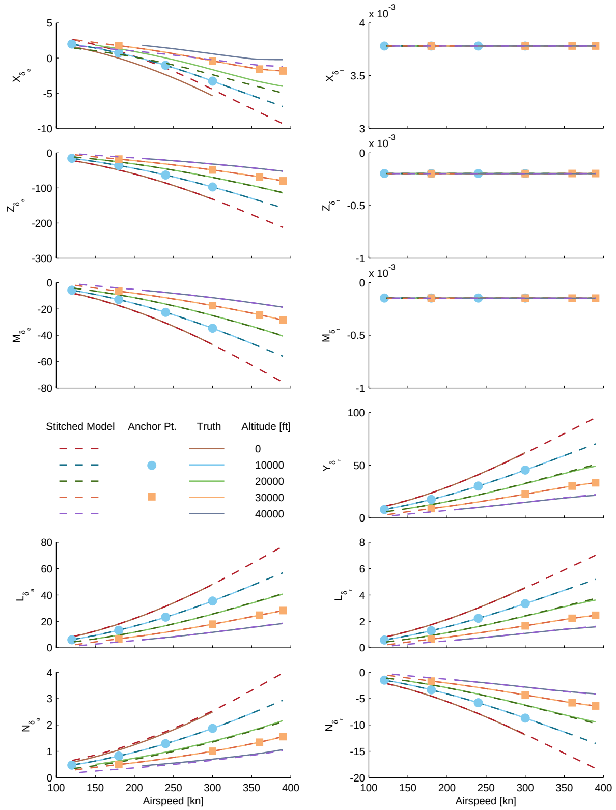
Figure B.25: Verification of altitude extrapolation, two altitudes, CJ1 stitched model, control derivatives.
