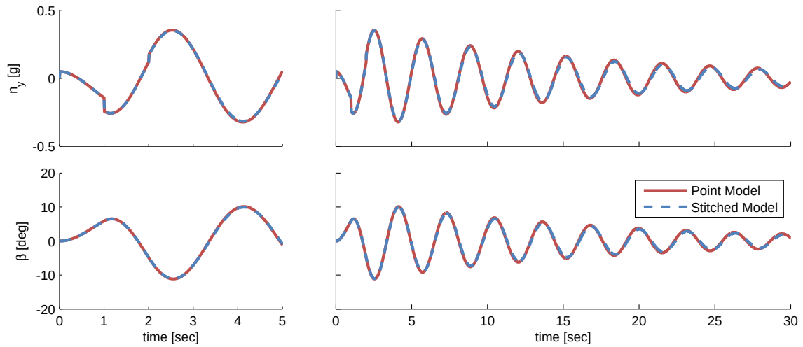
Figure 3.31: Case 2: short- and long-term time history responses, rudder doublet.
