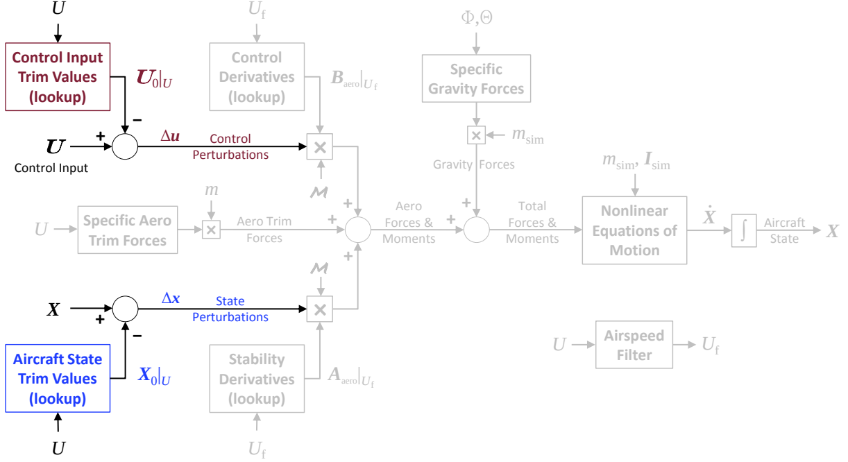
Figure 2.3: Model stitching simulation architecture – state and control perturbations.
