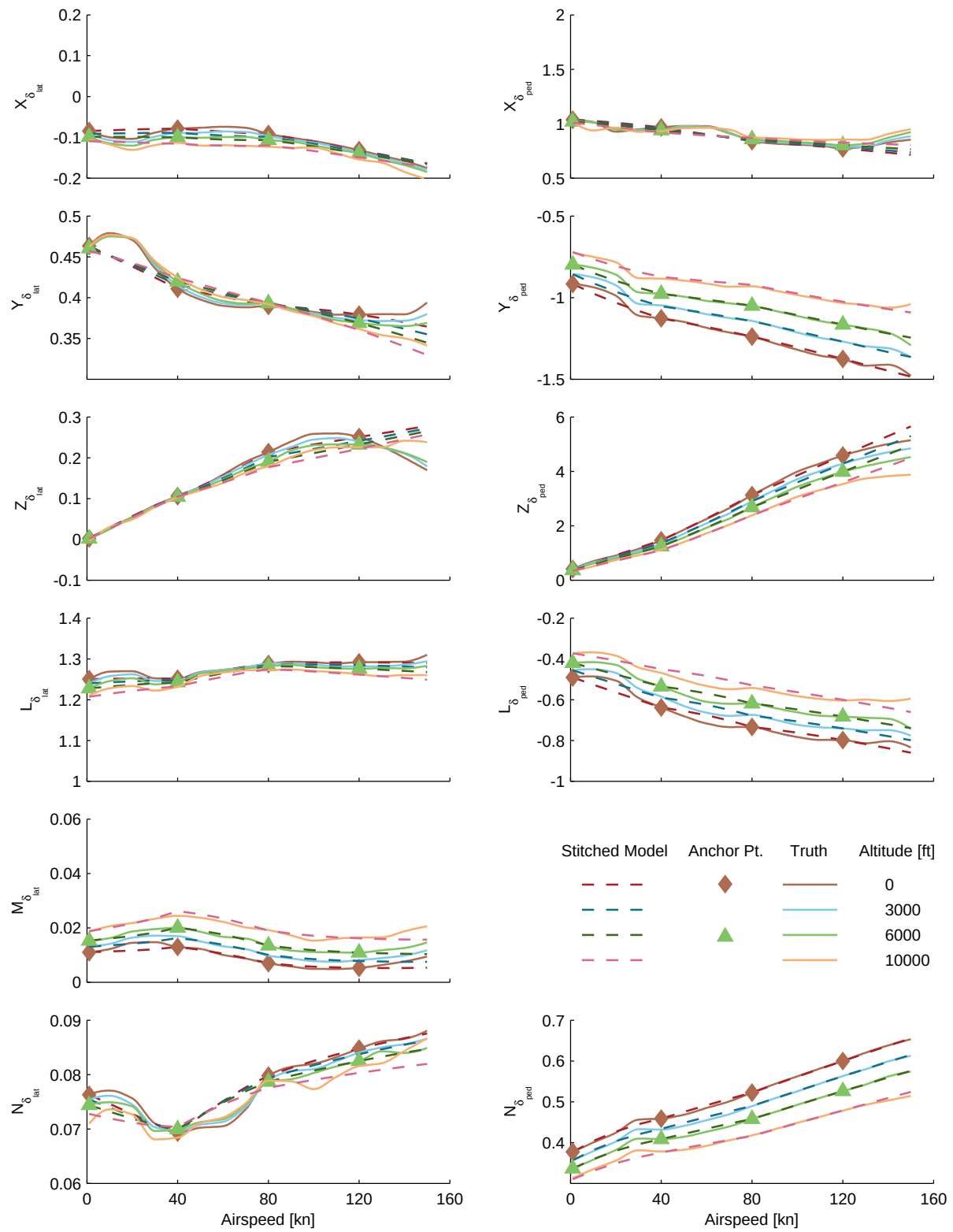
Figure C.19: Verification of altitude extrapolation, UH-60 stitched model, control derivatives (cont.)
