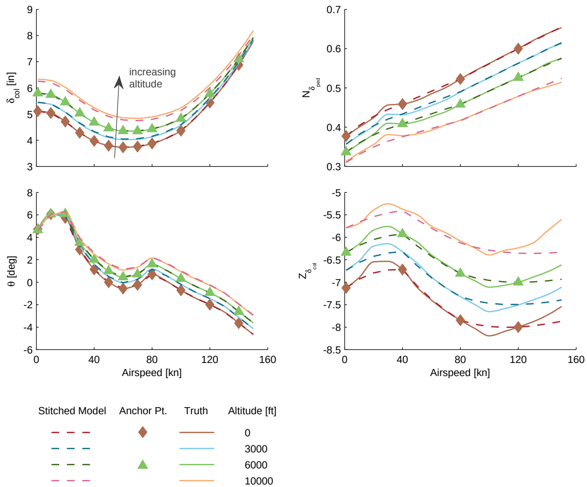
Figure 4.33: Verification of altitude extrapolation.
