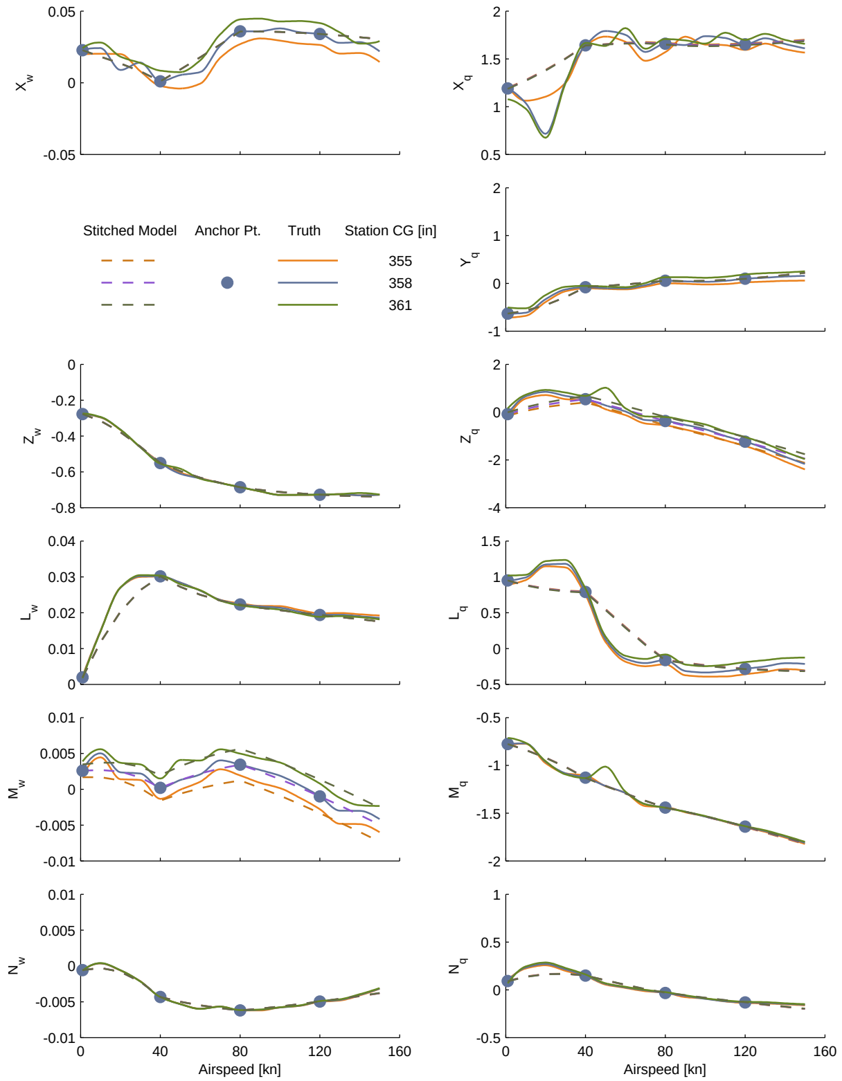
Figure C.12: Verification of off-nominal station CG extrapolation, UH-60 stitched model, stability derivatives (cont.)
