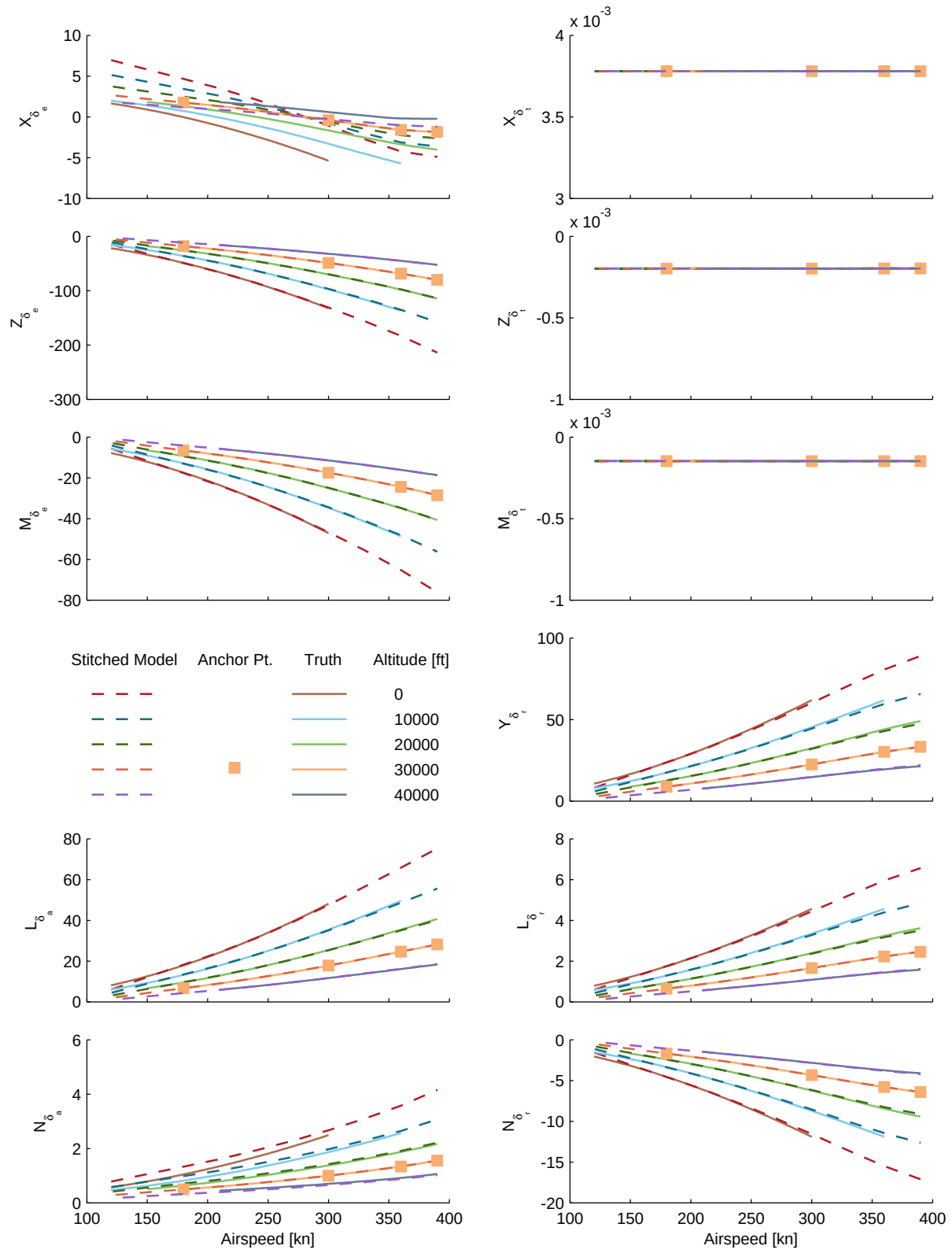
Figure B.22: Verification of single-altitude extrapolation, 30,000 ft, CJ1 stitched model, control derivatives.
