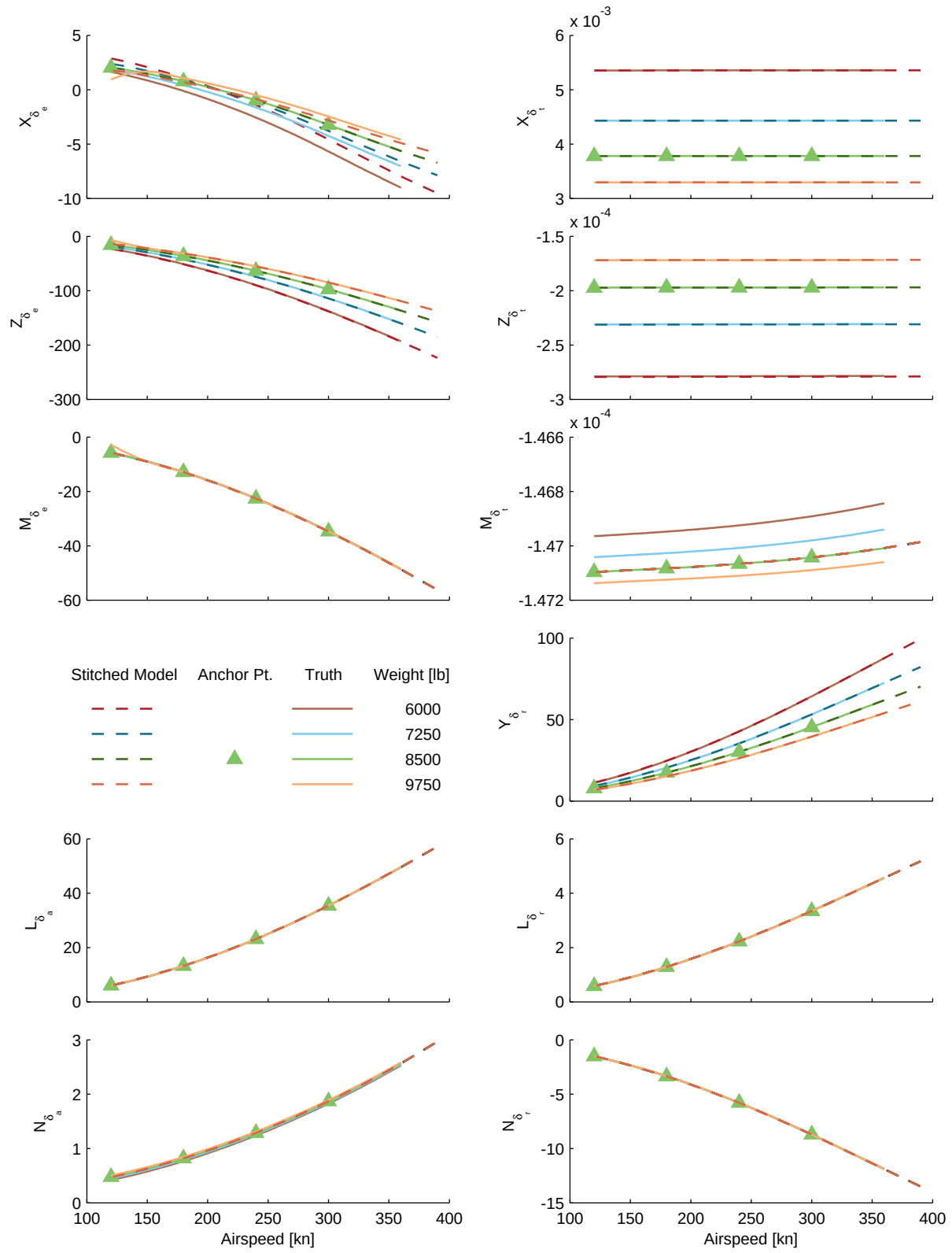
Figure B.3: Verification of off-nominal weight extrapolation, CJ1 stitched model, control derivatives.
