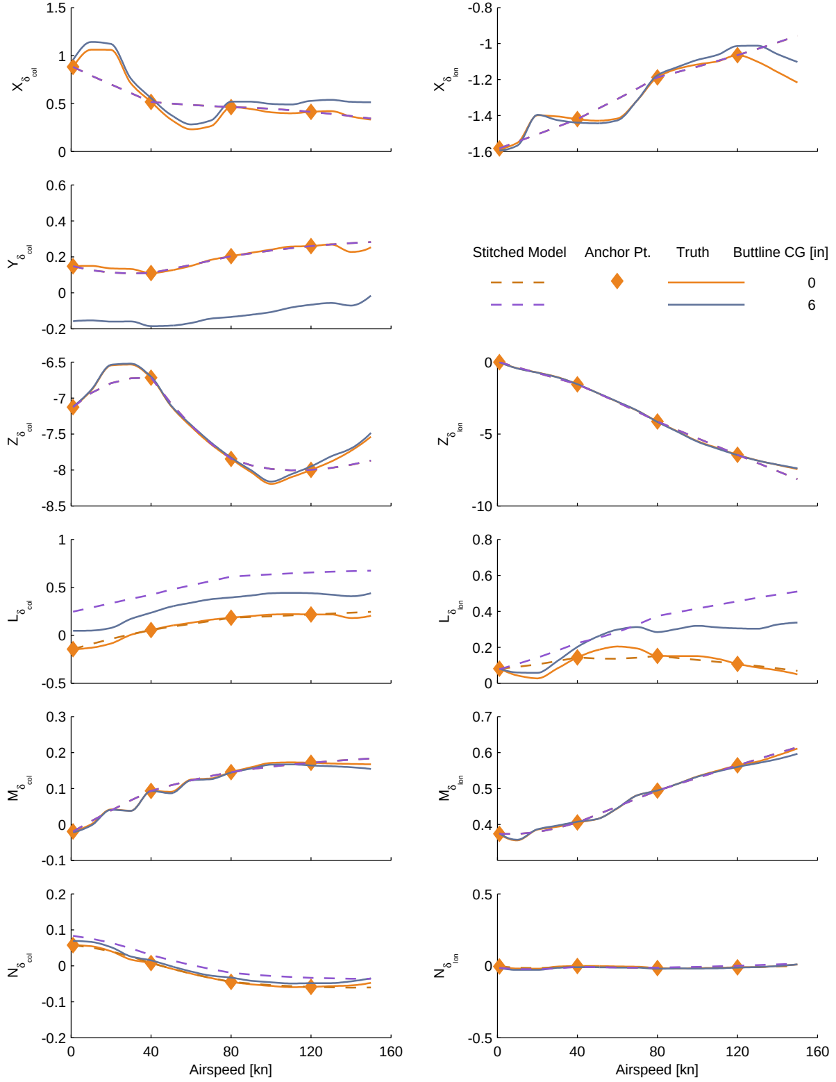
Figure C.16: Verification of off-nominal butto line CG extrapolation, UH-60 stitched model, control derivatives.
