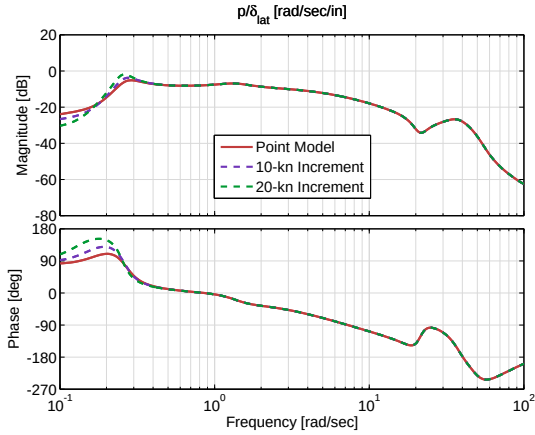
Figure 4.24: Roll rate response to lateral cyclic input comparison for forward-flight trim data of 10- and 20-kn spacing, 80 kn.
