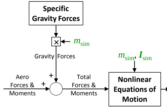
Figure 2.13: Simulation values of mass and inertia.
