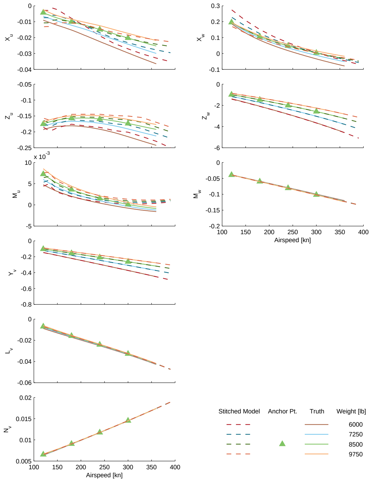
Figure B.2: Verification of off-nominal weight extrapolation, CJ1 stitched model, stability derivatives.
