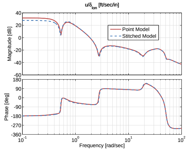
Figure 4.35: Case 1: x -body airspeed response to longitudinal cyclic input comparison.
