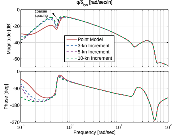
Figure 4.6: Pitch rate response to longitudinal cyclic input comparison for forward/rearward trim data of various spacing, hover.
