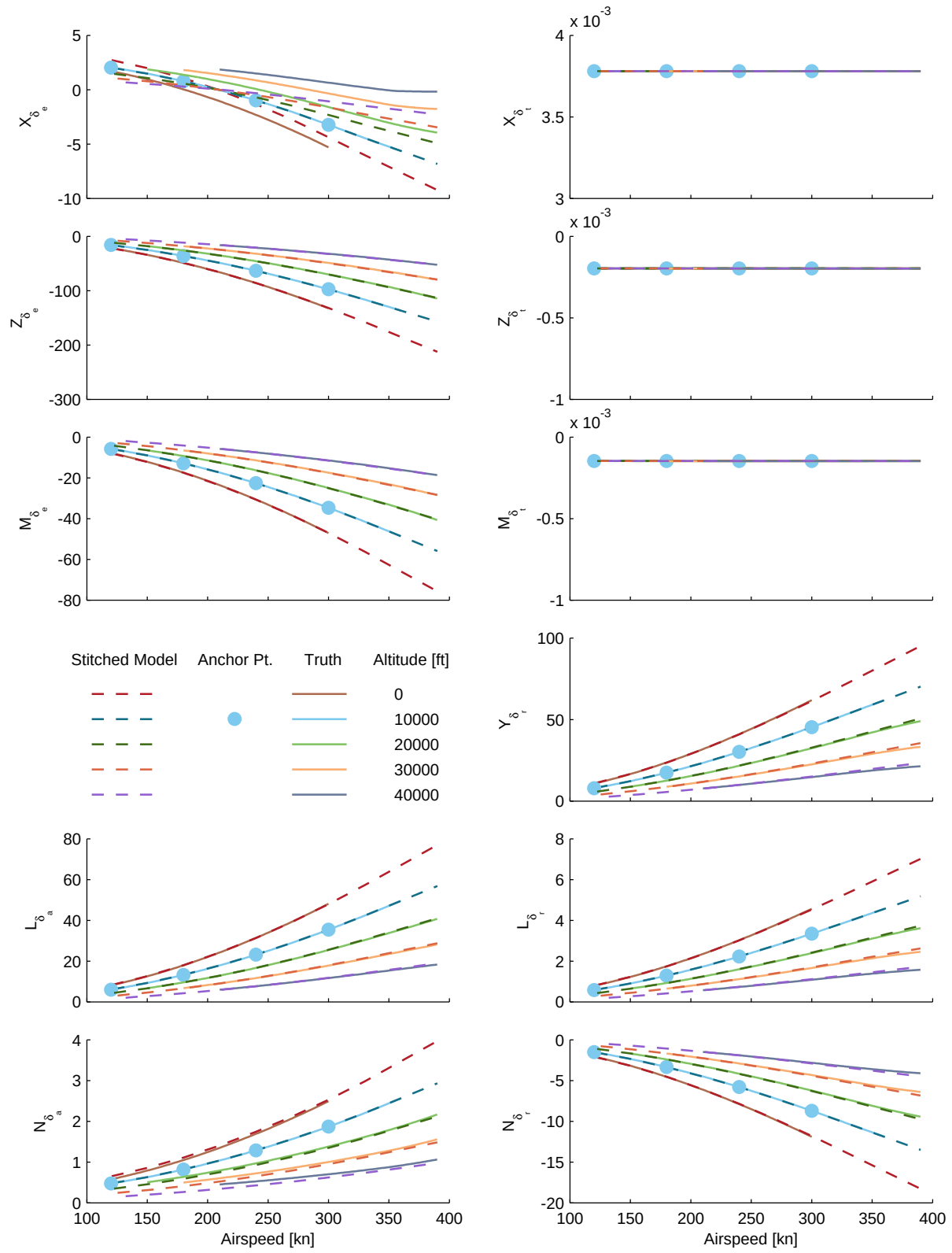
Figure B.19: Verification of single-altitude extrapolation, 10,000 ft, CJ1 stitched model, control derivatives.
