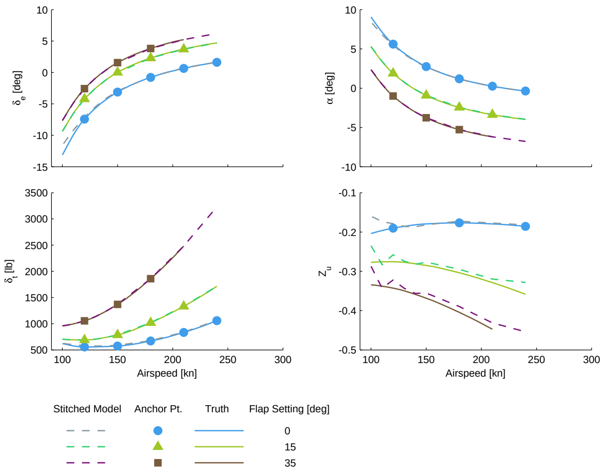
Figure 3.32: Alternate configuration verification, flap deflection.
