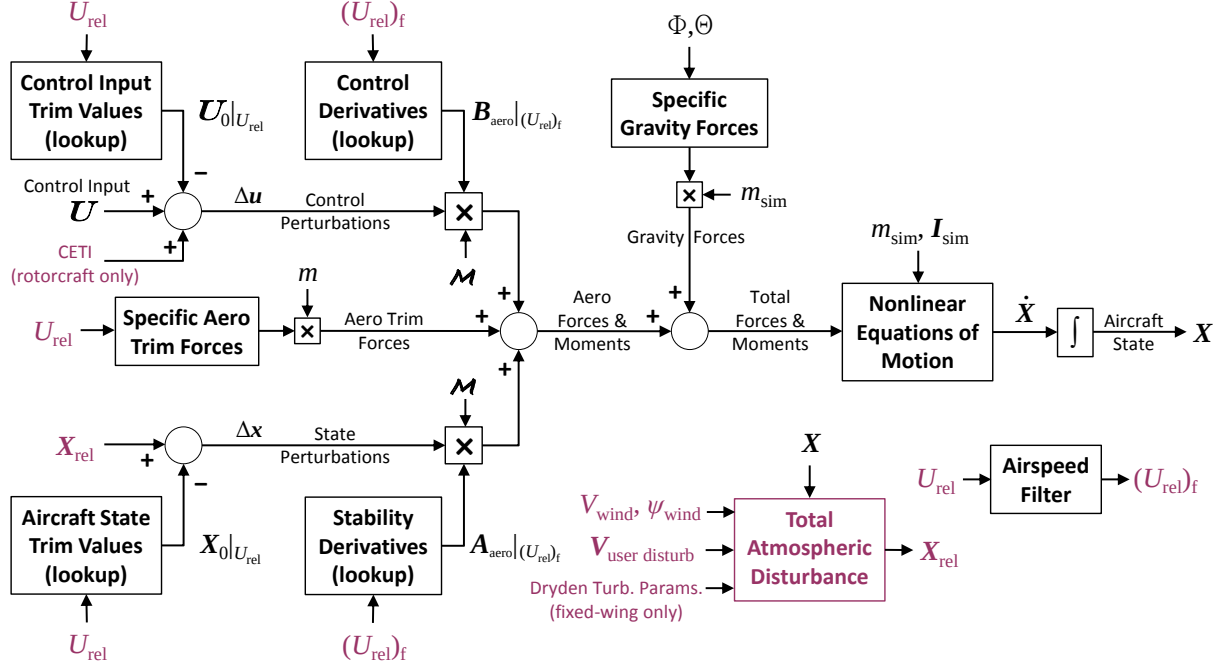
Figure 2.12: Model stitching simulation architecture – atmospheric disturbances.
