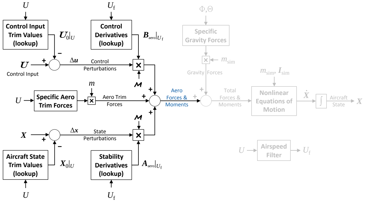
Figure 2.6: Model stitching simulation architecture – total aero forces and moments.
