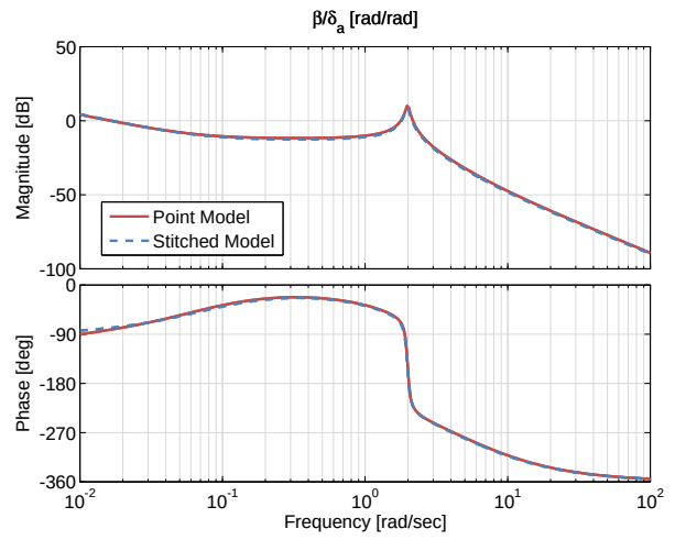
Figure 3.26: Case 2: sideslip response to aileron input comparison.
