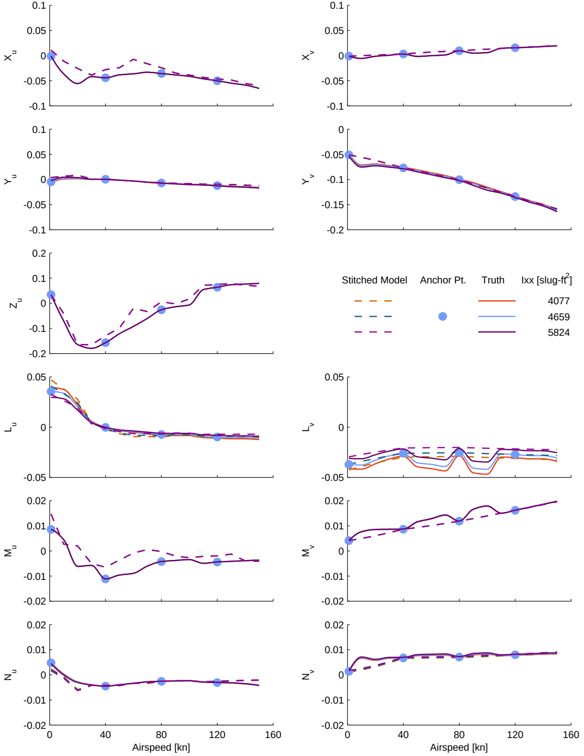
Figure C.5: Verification of off-nominal roll inertia extrapolation, UH-60 stitched model, stability derivatives.
