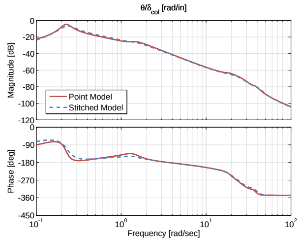
Figure 4.50: Case 2: pitch angle response to collective input comparison.
