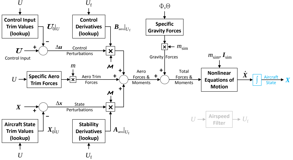
Figure 2.10: Model stitching simulation architecture – time integration.
