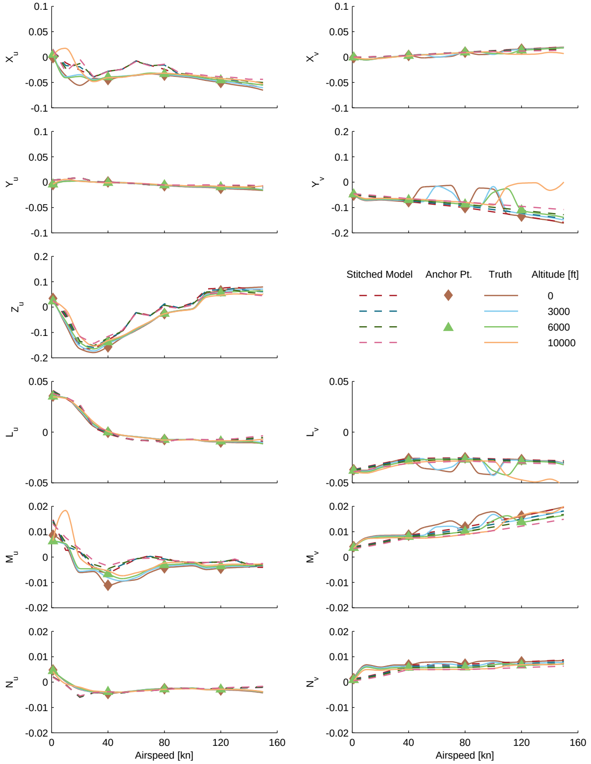
Figure C.18: Verification of altitude extrapolation, UH-60 stitched model, stability derivatives.
