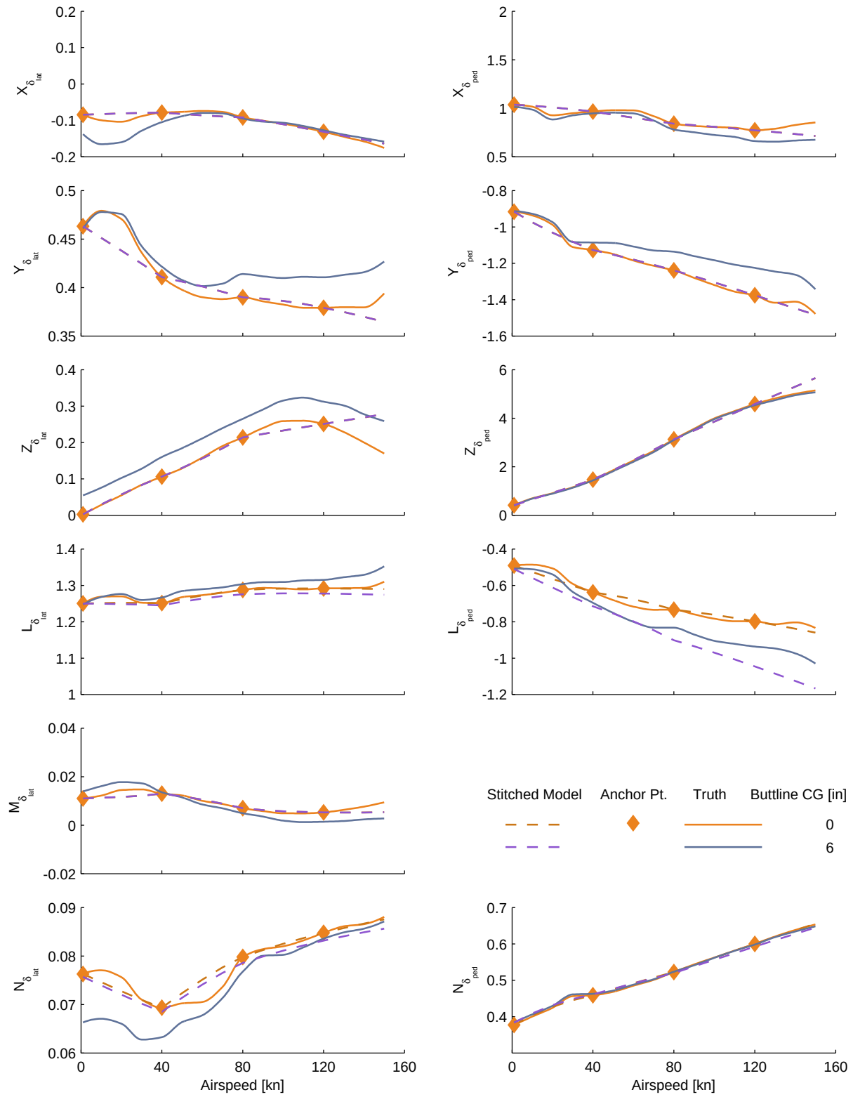
Figure C.16: Verification of off-nominal butto line CG extrapolation, UH-60 stitched model, control derivatives (cont.)
