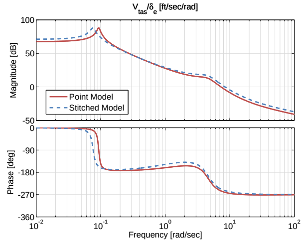
Figure 3.22: Case 2: true airspeed response to elevator input comparison.
