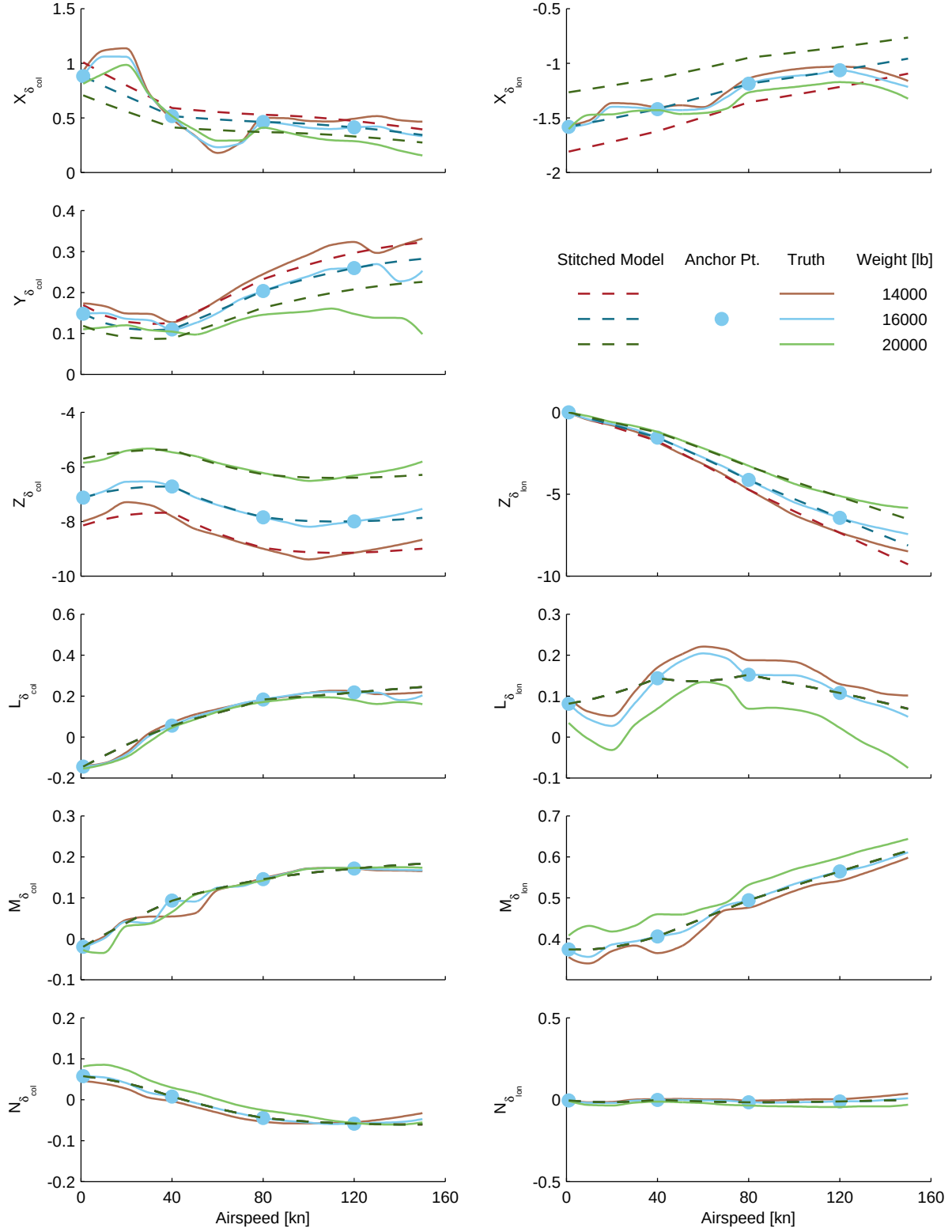
Figure C.3: Verification of off-nominal weight extrapolation, UH-60 stitched model, control derivatives.
