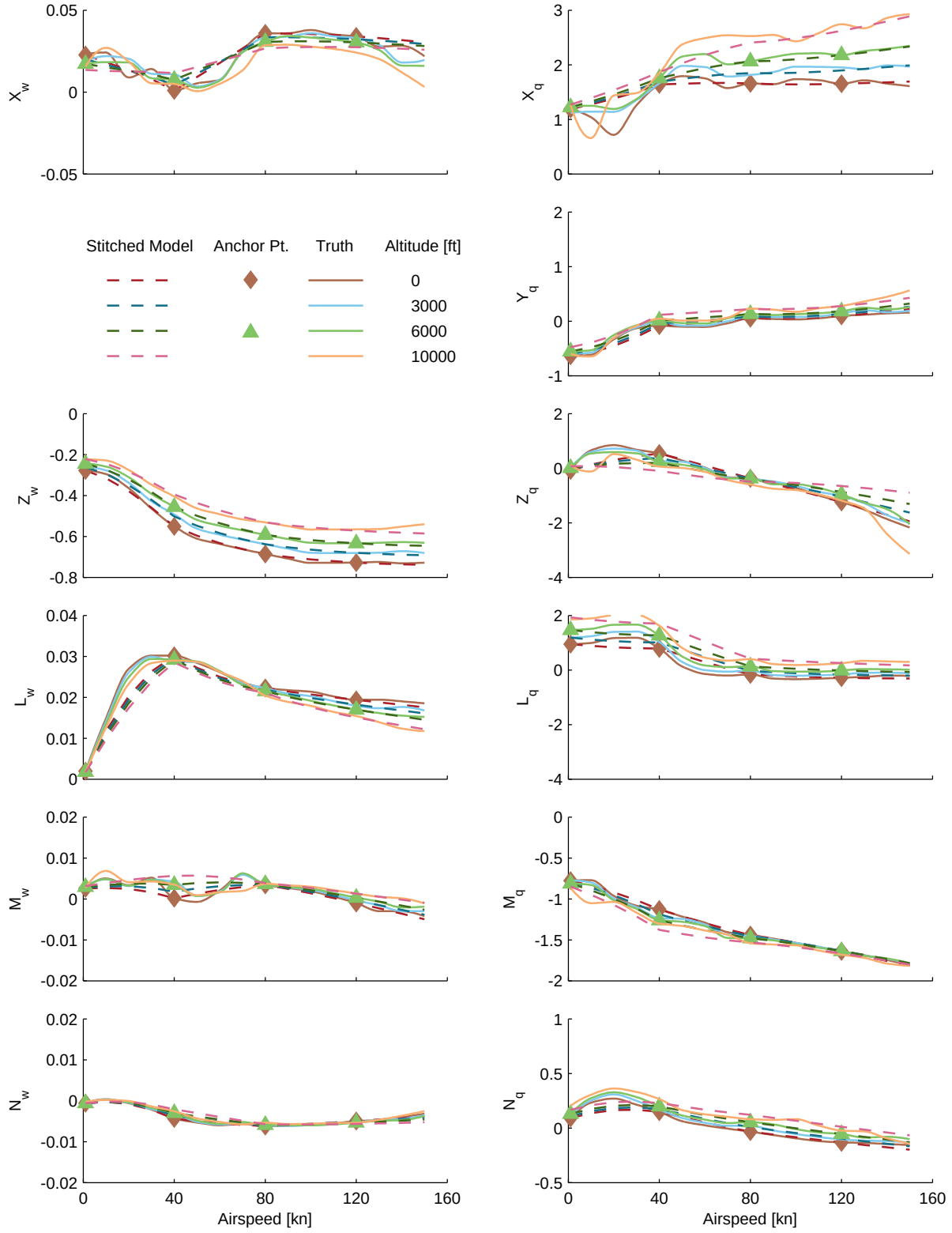
Figure C.18: Verification of altitude extrapolation, UH-60 stitched model, stability derivatives (cont.)
