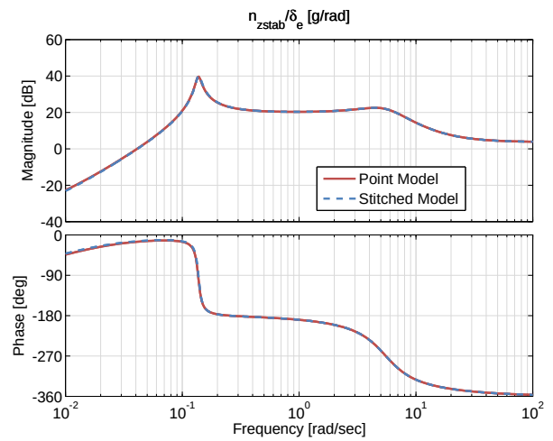
Figure 3.13: Case 1: normal acceleration response to elevator input comparison.
