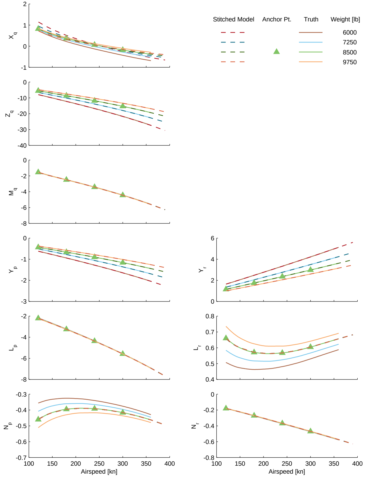
Figure B.2: Verification of off-nominal weight extrapolation, CJ1 stitched model, stability derivatives (cont.)
