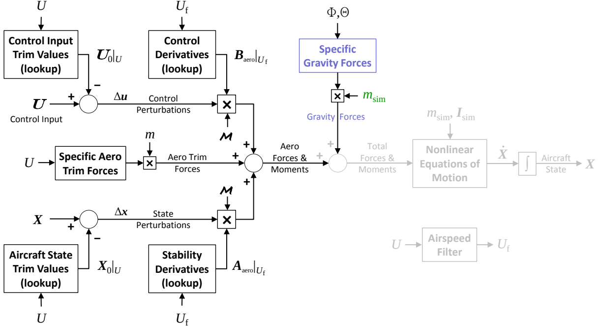
Figure 2.7: Model stitching simulation architecture – nonlinear gravitational forces.
