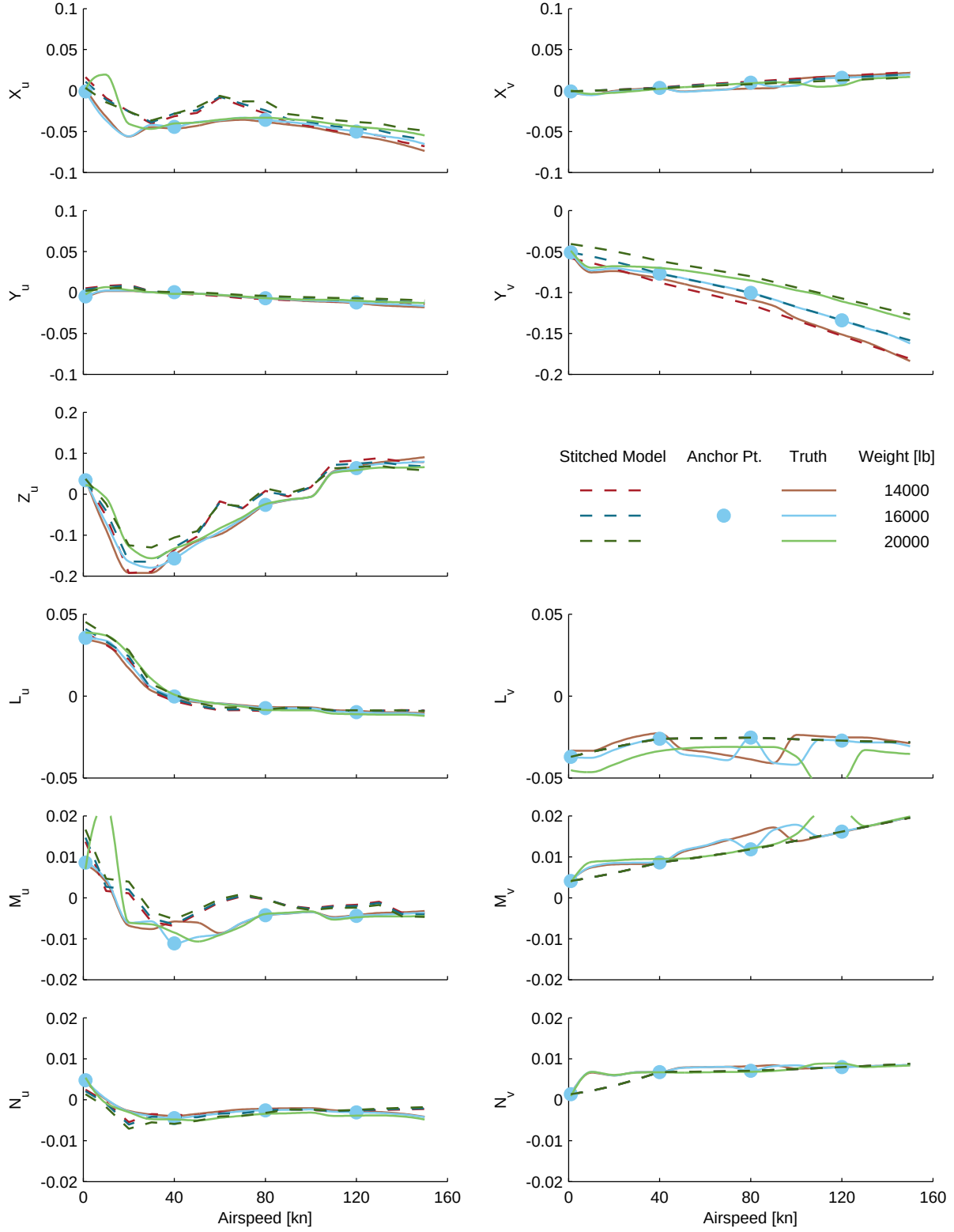
Figure C.2: Verification of off-nominal weight extrapolation, UH-60 stitched model, stability derivatives.
