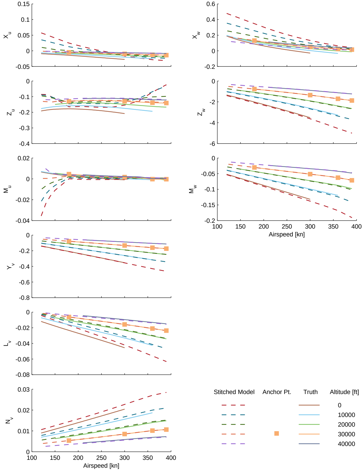
Figure B.21: Verification of single-altitude extrapolation, 30,000 ft, CJ1 stitched model, stability derivatives.
