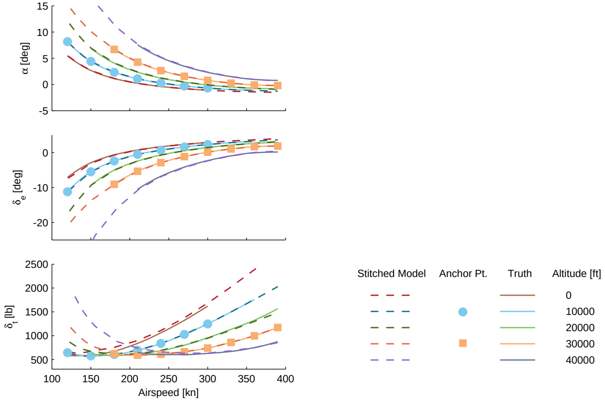
Figure B.23: Verification of altitude extrapolation, two altitudes, CJ1 stitched model, trim.
