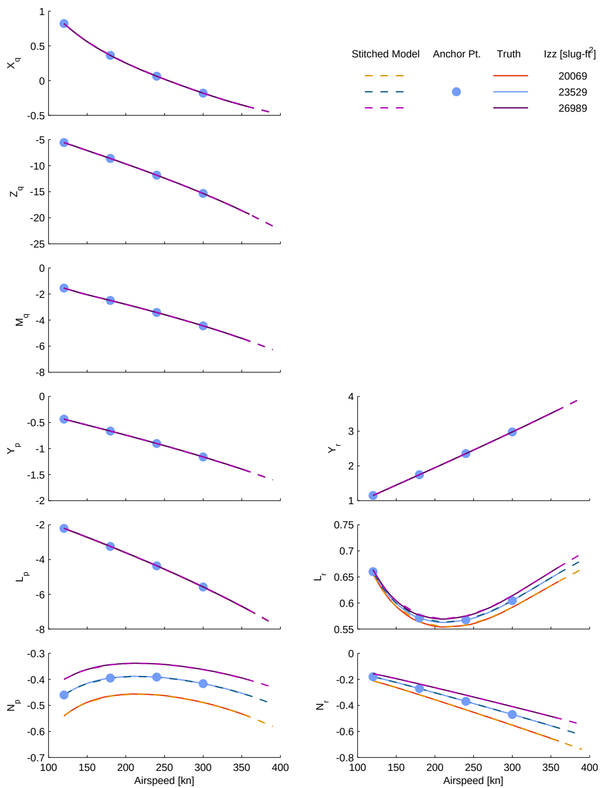
Figure B.9: Verification of off-nominal yaw inertia extrapolation, CJ1 stitched model, stability derivatives (cont.)
