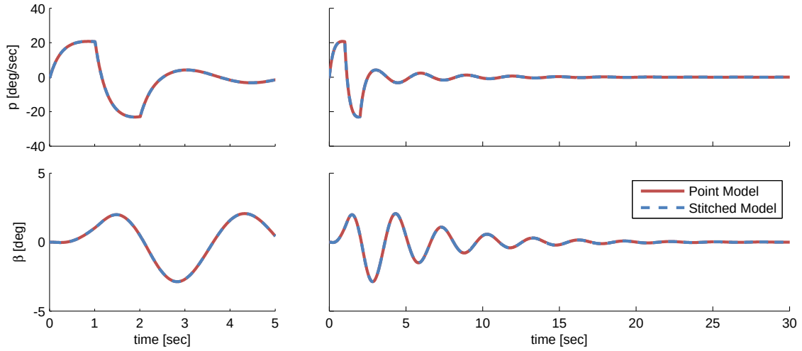
Figure 3.19: Case 1: short- and long-term time history responses, aileron doublet.
