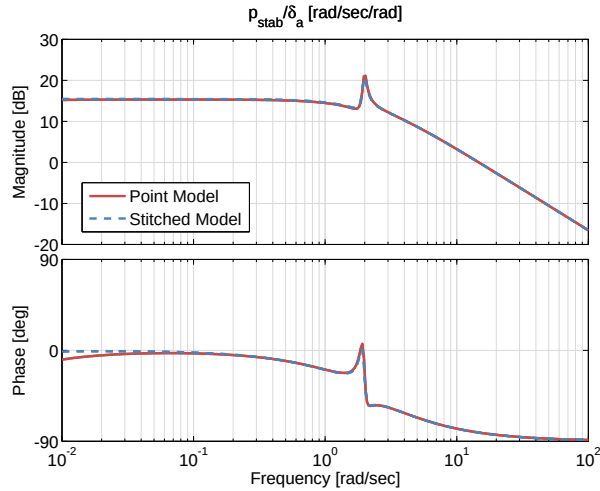
Figure 3.25: Case 2: roll rate response to aileron input comparison.
