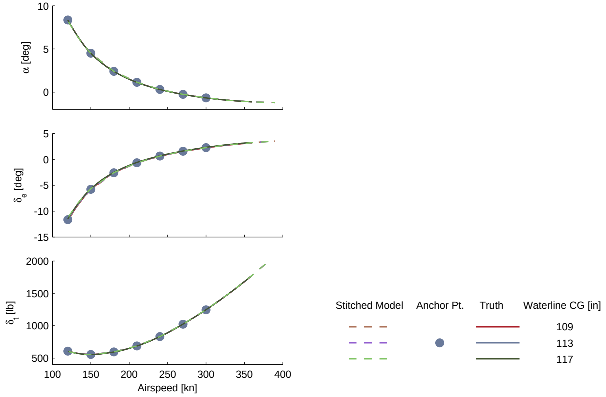
Figure B.14: Verification of off-nominal waterline CG extrapolation, CJ1 stitched model, trim.
