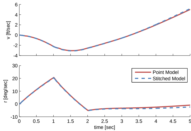
Figure 4.44: Case 1: short-term time history responses, pedal doublet.
