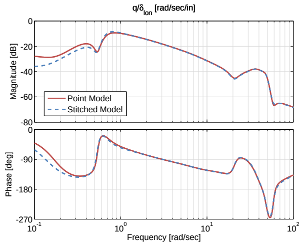
Figure 4.34: Case 1: pitch rate response to longitudinal cyclic input comparison.
