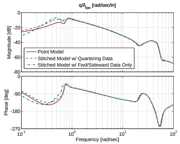
Figure 4.16: Pitch rate response to longitudinal cyclic input for 10-kn, 45-deg quartering flight.
