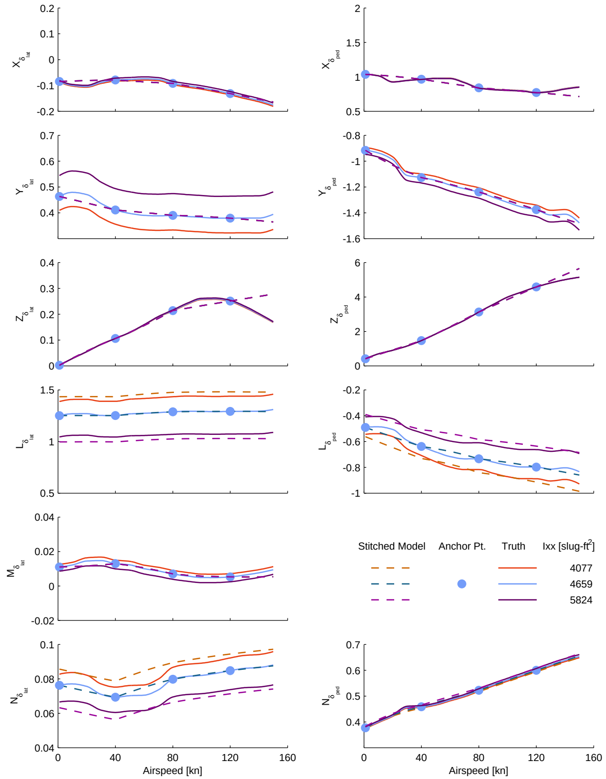
Figure C.6: Verification of off-nominal roll inertia extrapolation, UH-60 stitched model, control derivatives (cont.)
