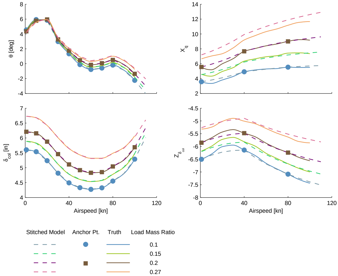
Figure 4.56: Alternate configuration verification, sling-load weight.
