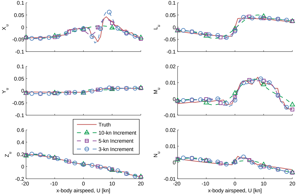
Figure 4.4: Implicit u -speed derivative values due to forward/rearward flight trim data of various spacing.
