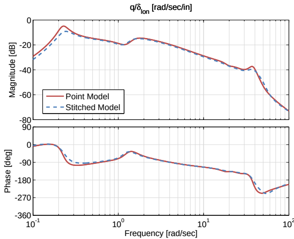
Figure 4.45: Case 2: pitch rate response to longitudinal cyclic input comparison.
