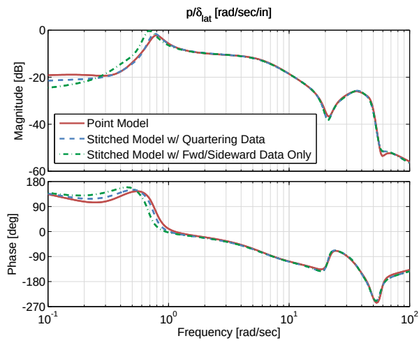
Figure 4.15: Roll rate response to lateral cyclic input for 10-kn, 45-deg quartering flight.
