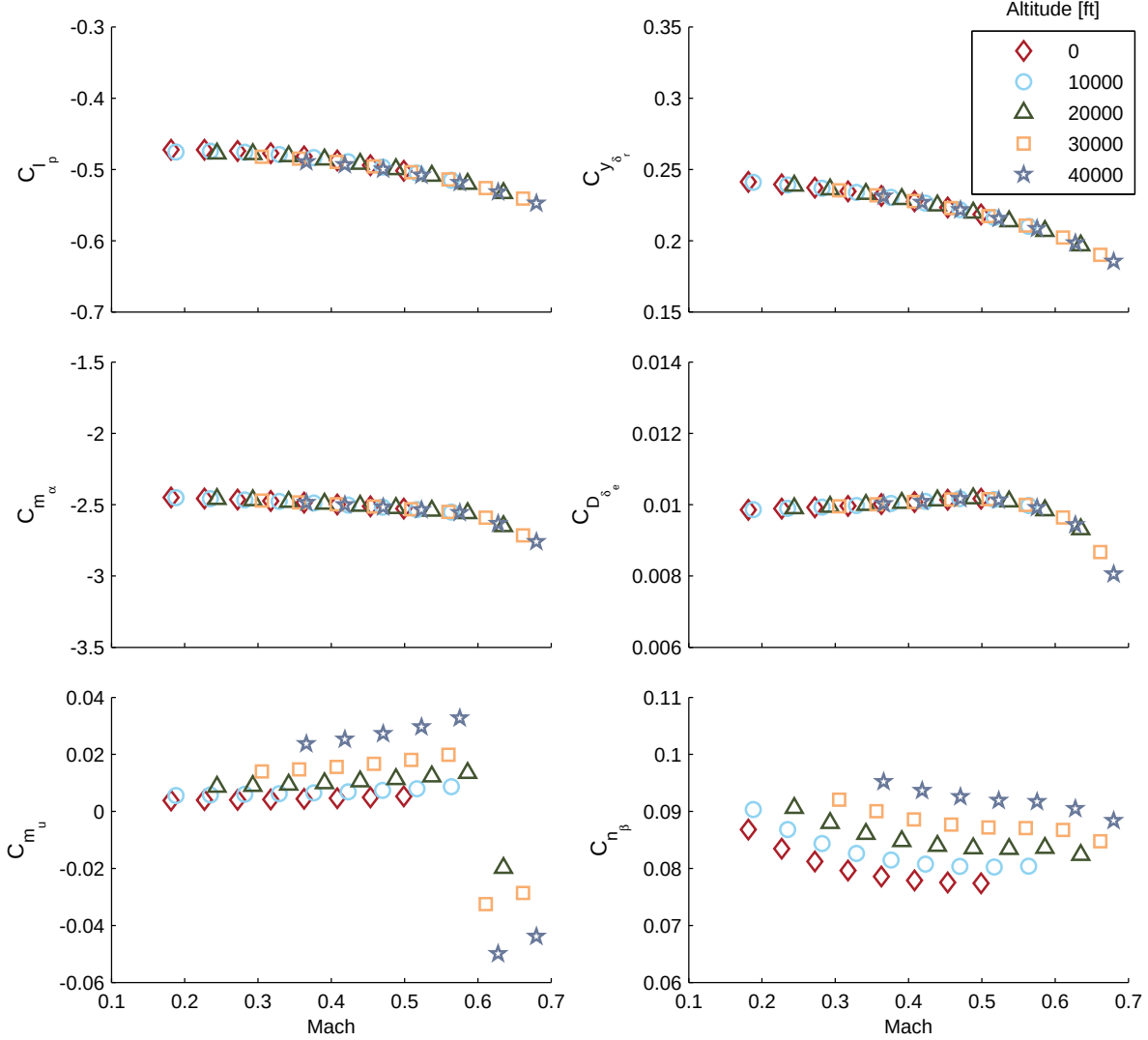
Figure 3.4: Nondimensional derivative values vs. Mach over flight envelope, AAA CJ1 model.
