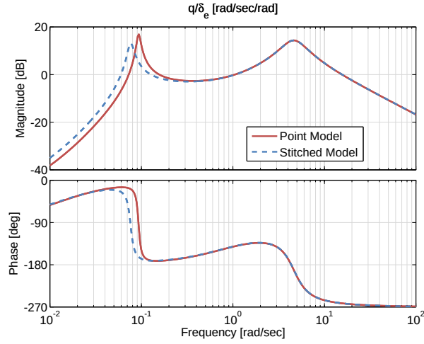
Figure 3.23: Case 2: pitch rate response to elevator input comparison.
