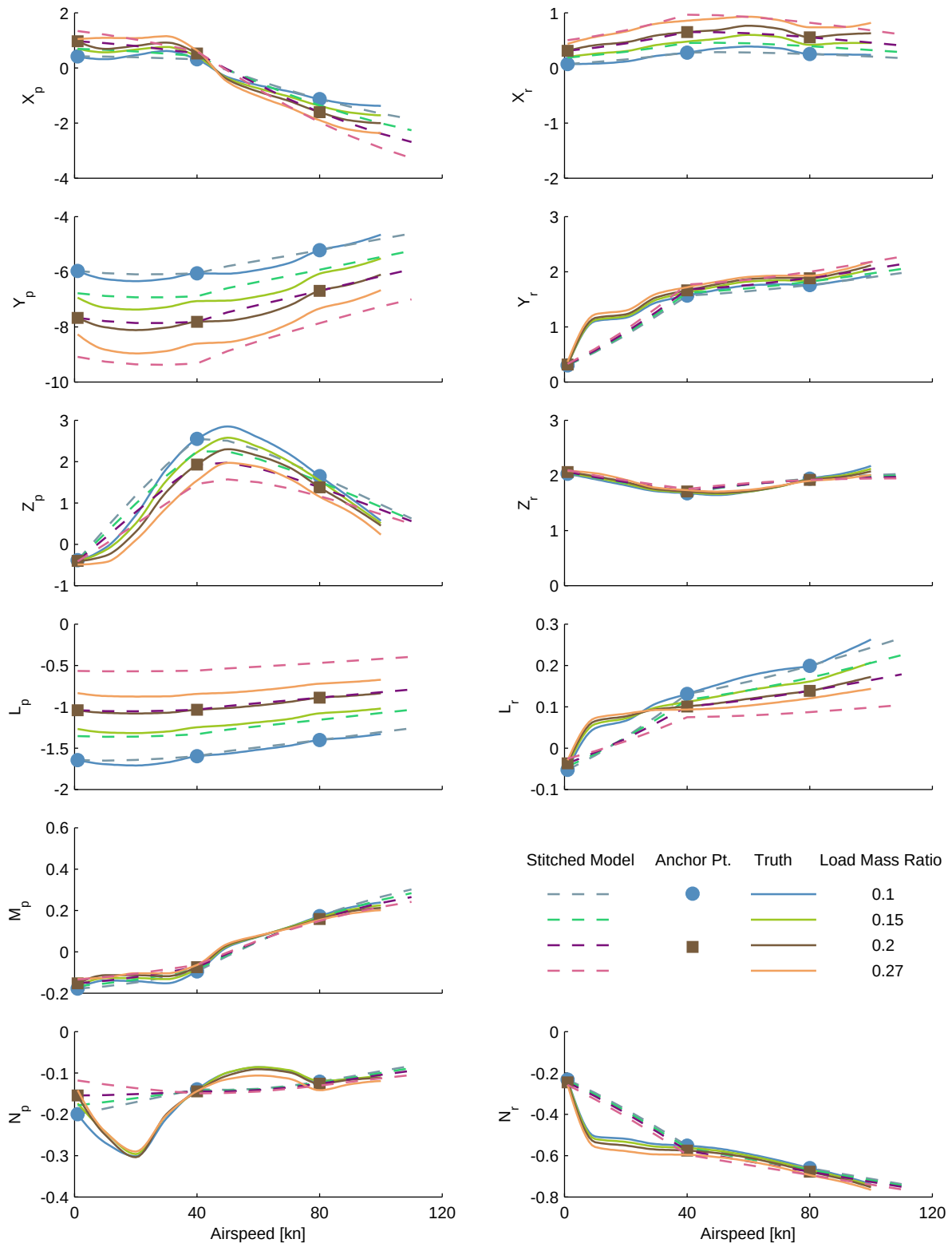
Figure C.21: Alternate configuration verification, sling-load weight, UH-60 stitched model, stability derivatives (cont.)
