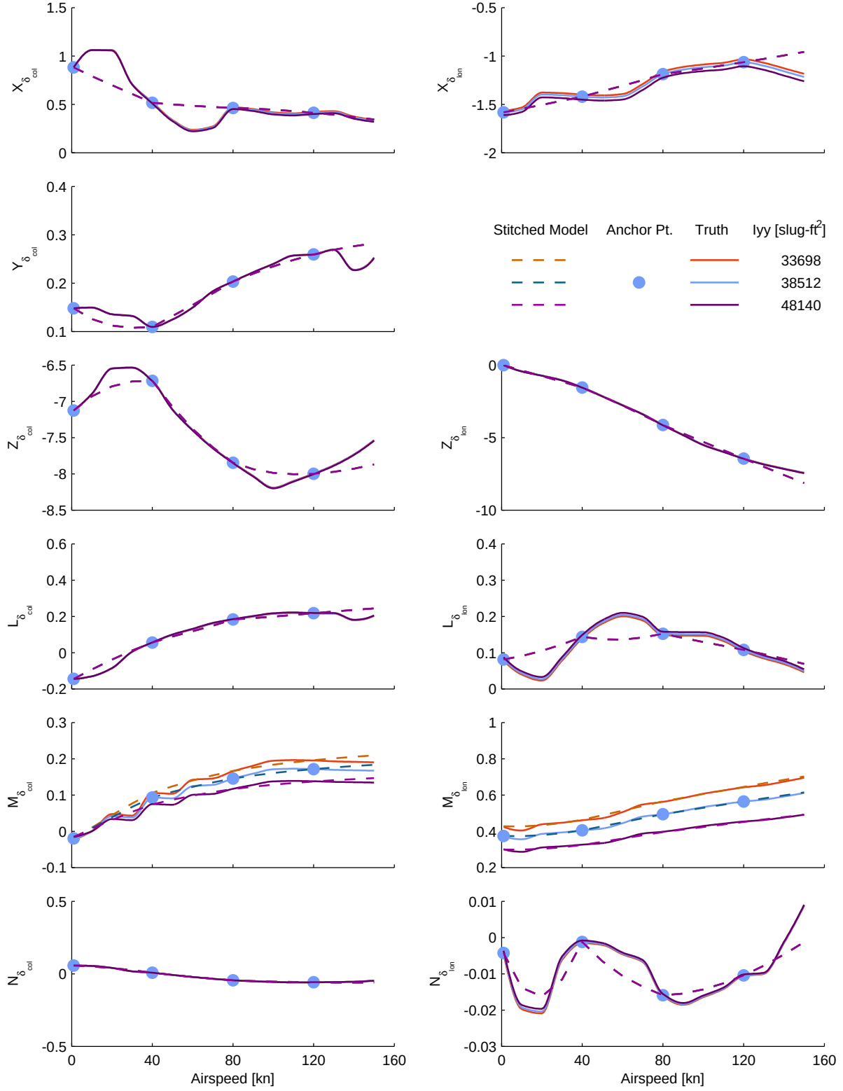
Figure C.8: Verification of off-nominal pitch inertia extrapolation, UH-60 stitched model, control derivatives.
