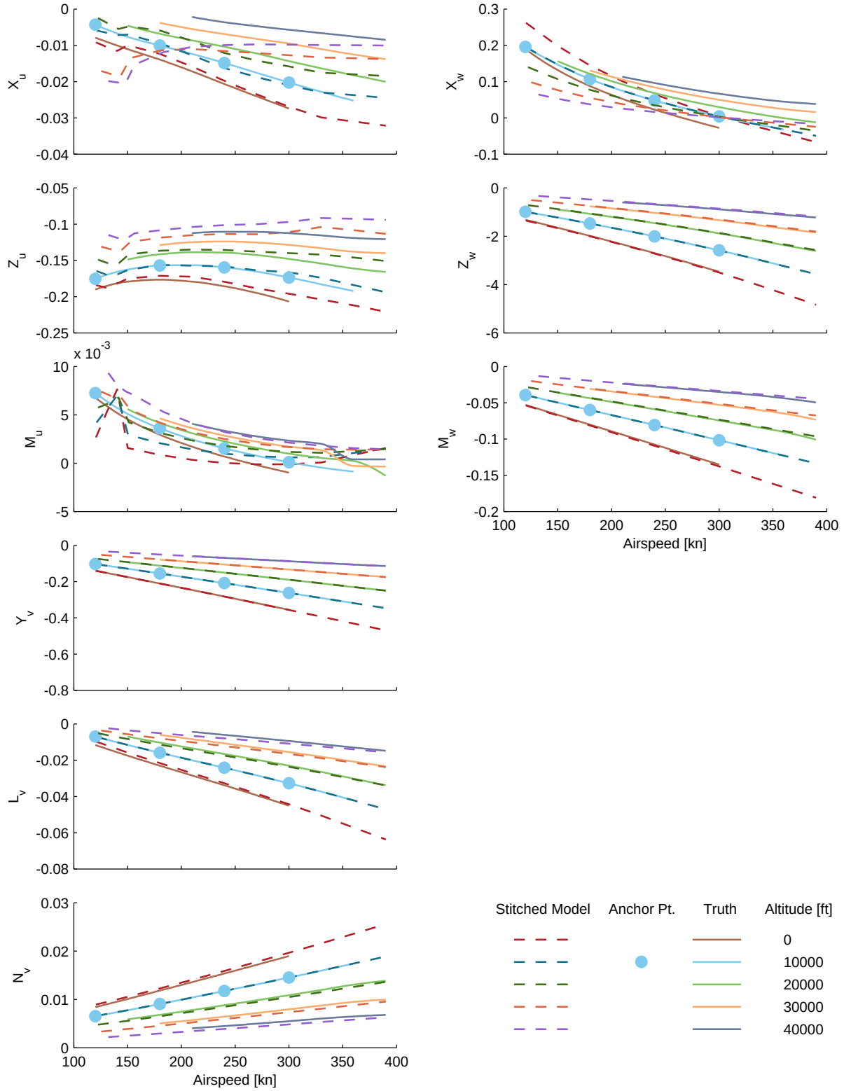
Figure B.18: Verification of single-altitude extrapolation, 10,000 ft, CJ1 stitched model, stability derivatives.
