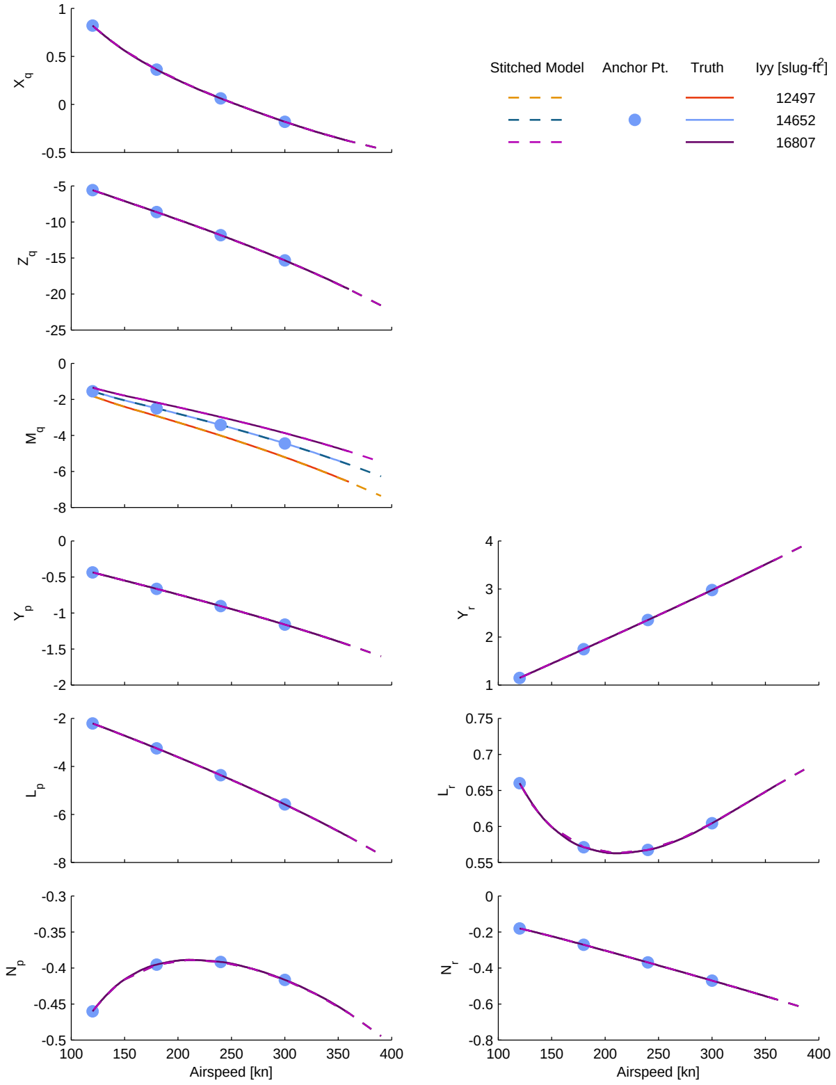
Figure B.7: Verification of off-nominal pitch inertia extrapolation, CJ1 stitched model, stability derivatives (cont.)
