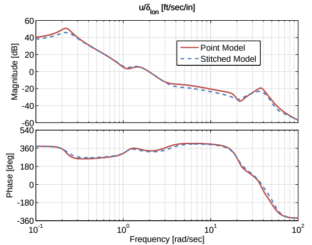
Figure 4.46: Case 2: x -body airspeed response to longitudinal cyclic input comparison.
