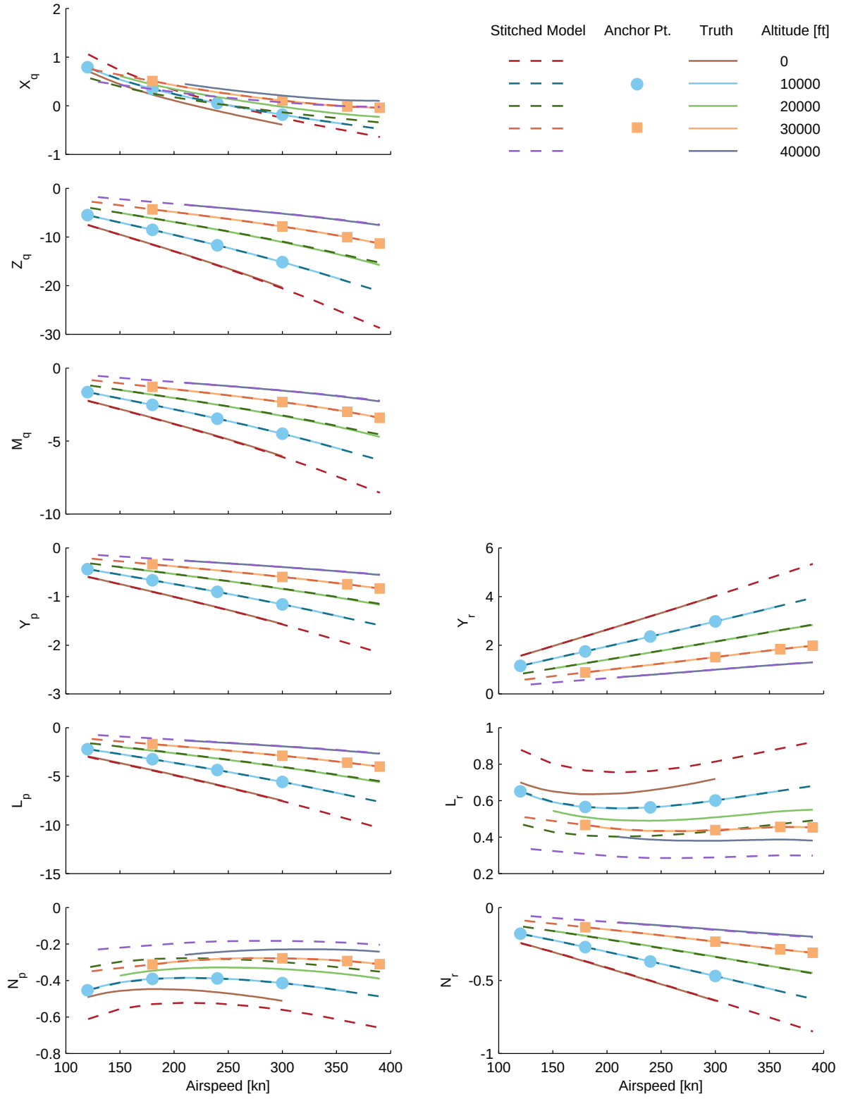
Figure B.24: Verification of altitude extrapolation, two altitudes, CJ1 stitched model, stability derivatives (cont.)
