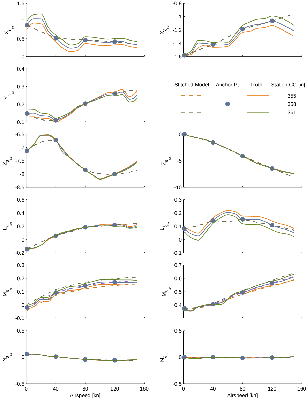
Figure C.13: Verification of off-nominal station CG extrapolation, UH-60 stitched model, control derivatives.
