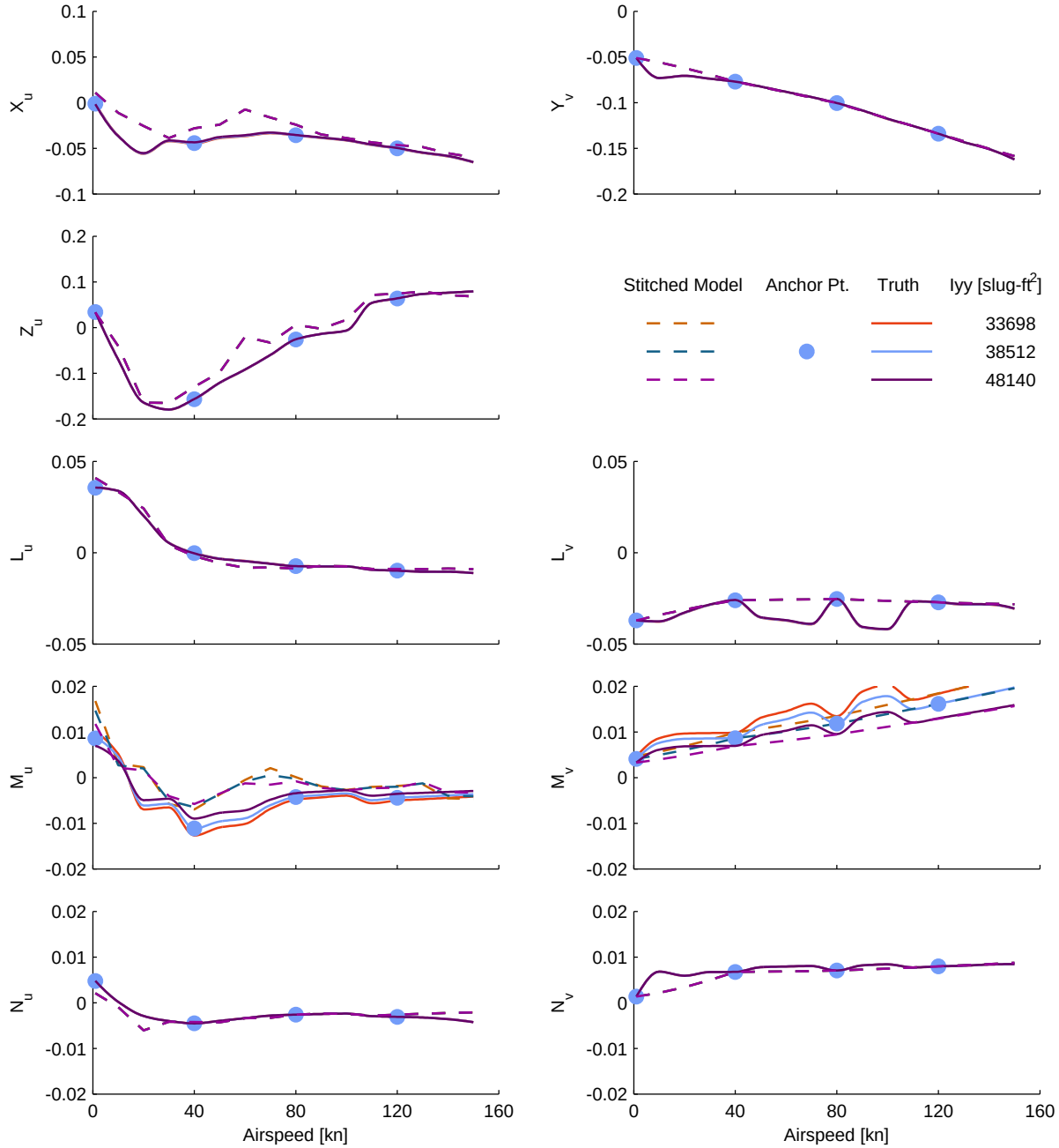
Figure C.7: Verification of off-nominal pitch inertia extrapolation, UH-60 stitched model, stability derivatives.
