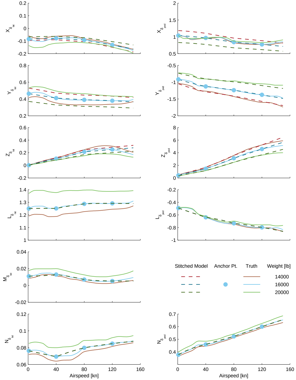
Figure C.3: Verification of off-nominal weight extrapolation, UH-60 stitched model, control derivatives (cont.)
