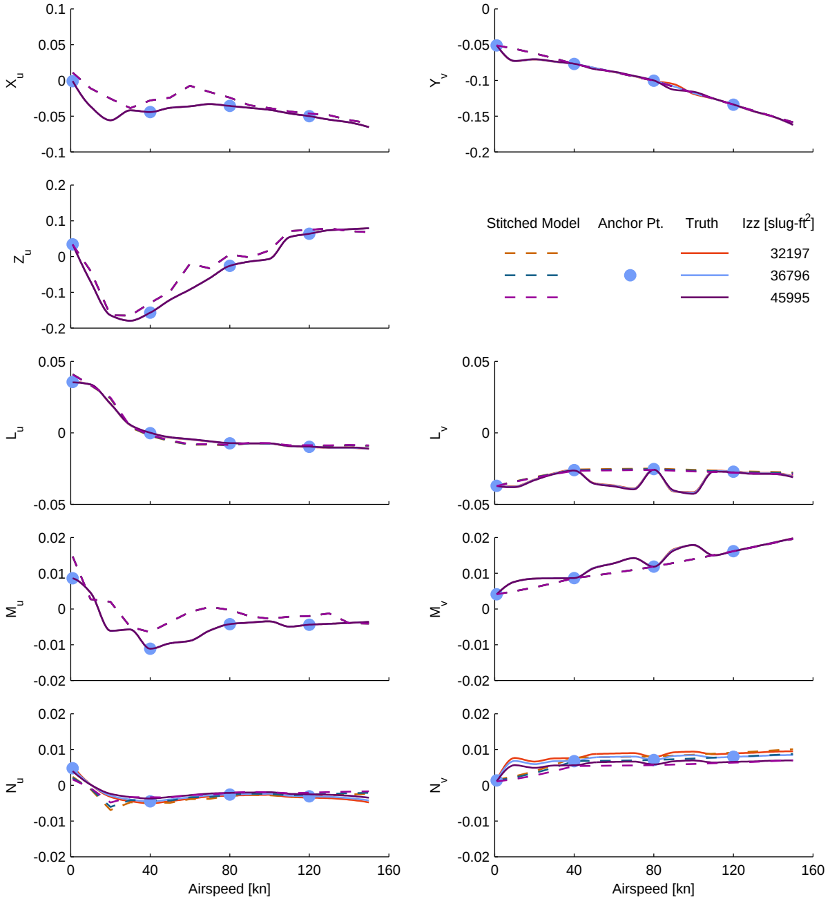
Figure C.9: Verification of off-nominal yaw inertia extrapolation, UH-60 stitched model, stability derivatives.
