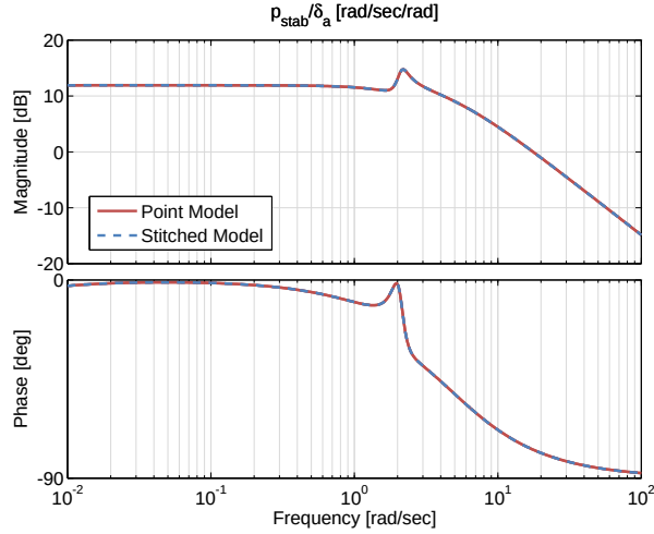
Figure 3.14: Case 1: roll rate response to aileron input comparison.
