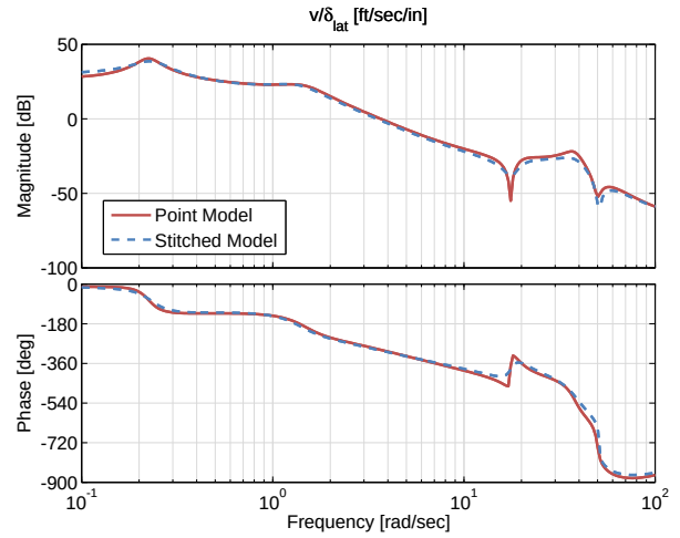
Figure 4.48: Case 2: y -body airspeed response to lateral cyclic input comparison.
