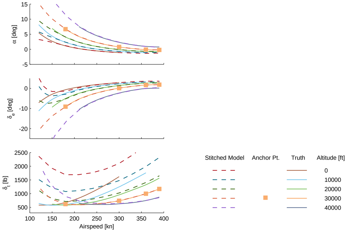
Figure B.20: Verification of single-altitude extrapolation, 30,000 ft, CJ1 stitched model, trim.
