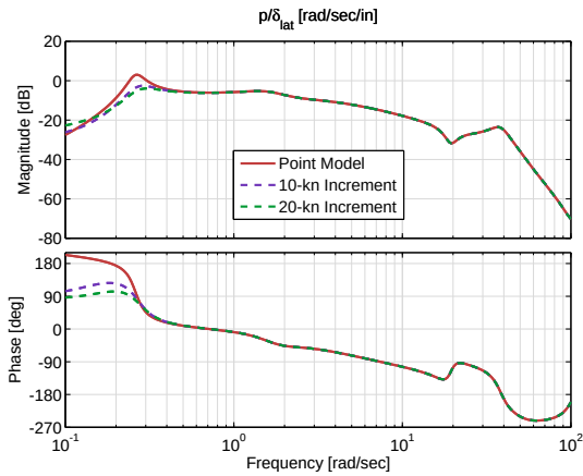
Figure 4.26: Roll rate response to lateral cyclic input comparison for forward-flight trim data of 10- and 20-kn spacing, 120 kn.
