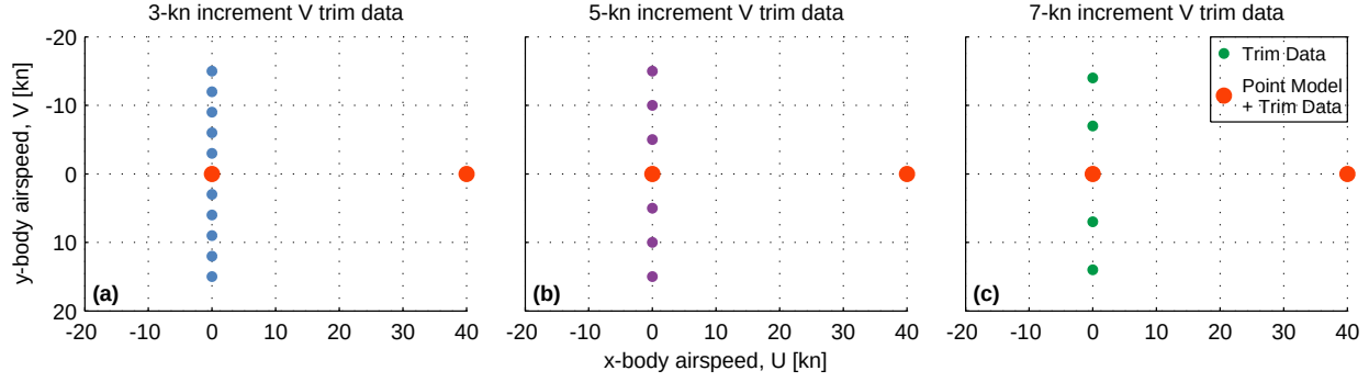
Figure 4.7: Sideward flight trim data points at 3-, 5-, and 7-kn y -body airspeed V increments, and point models at hover and 40 kn.
