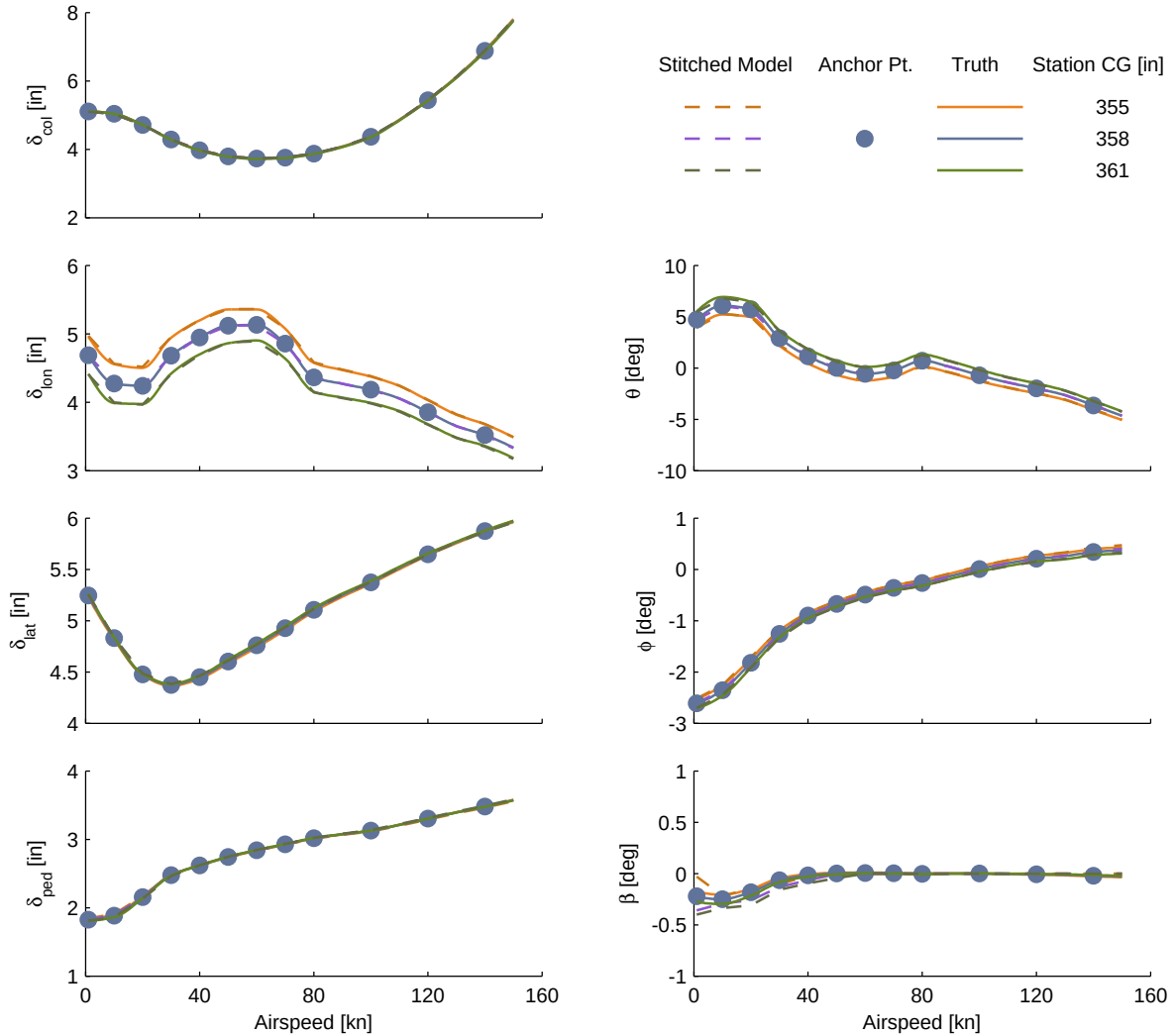
Figure C.11: Verification of off-nominal station CG extrapolation, UH-60 stitched model, trim.
