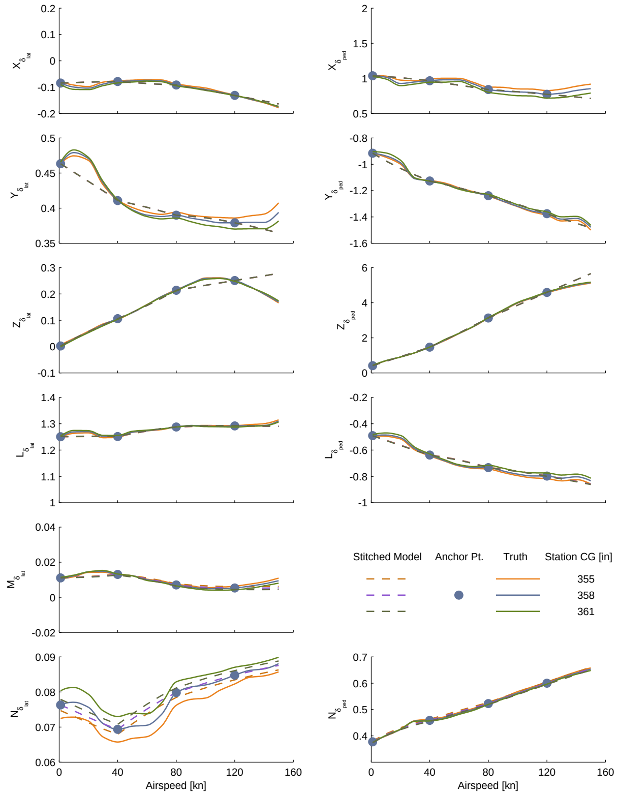
Figure C.13: Verification of off-nominal station CG extrapolation, UH-60 stitched model, control derivatives (cont.)
