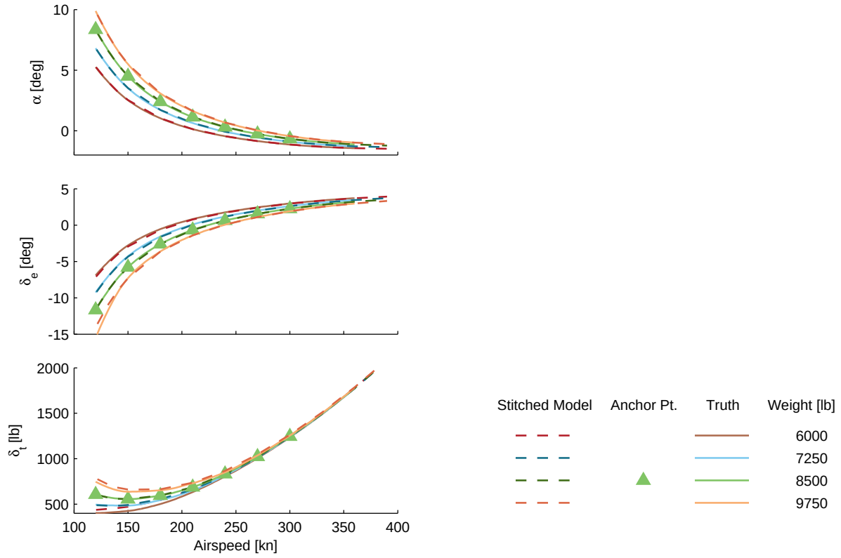
Figure B.1: Verification of off-nominal weight extrapolation, CJ1 stitched model, trim.
