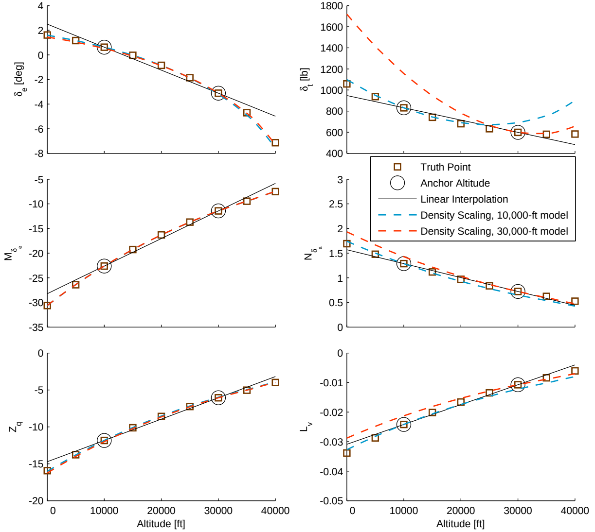
Figure 3.8: Altitude density-ratio scaling vs. linear interpolation, 240-kn point models.
