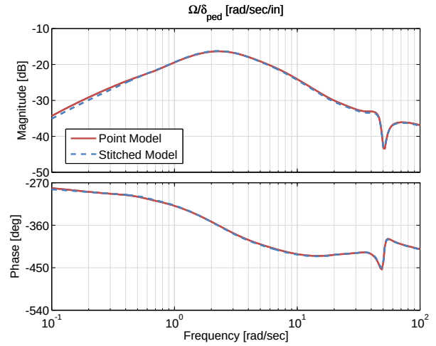
Figure 4.41: Case 1: main rotor rotational speed to pedal input comparison.
