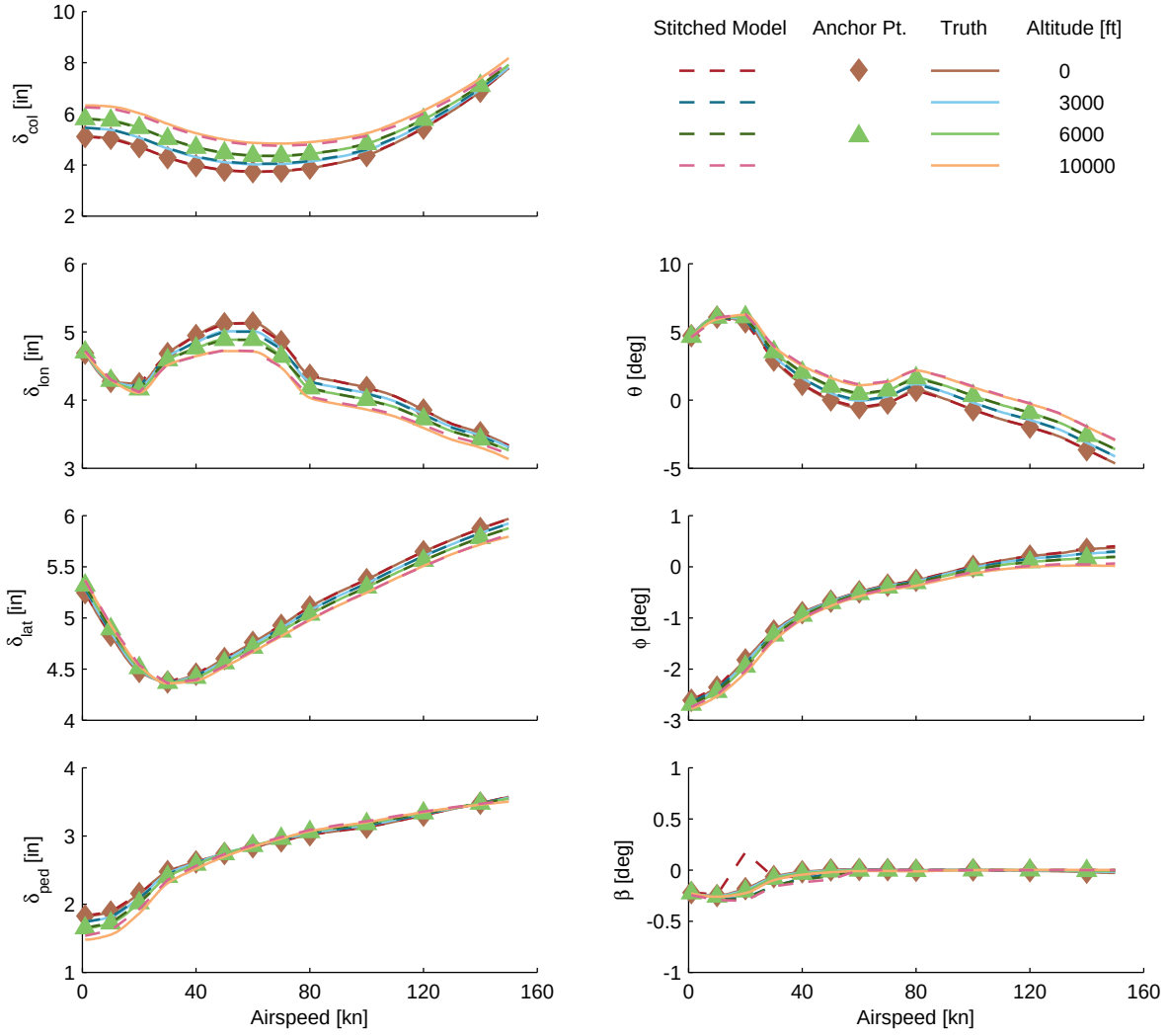
Figure C.17: Verification of altitude extrapolation, UH-60 stitched model, trim.
