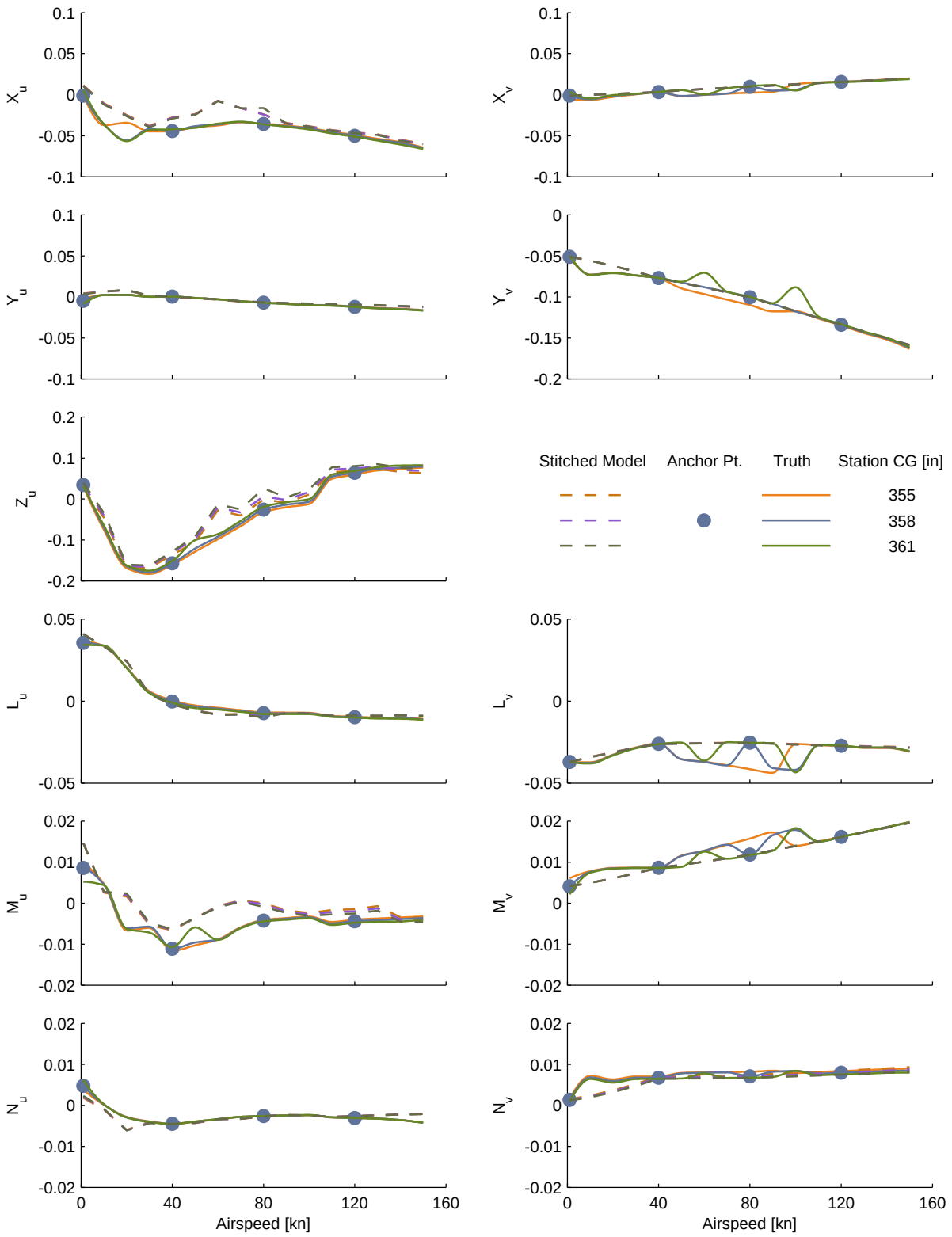
Figure C.12: Verification of off-nominal station CG extrapolation, UH-60 stitched model, stability derivatives.
