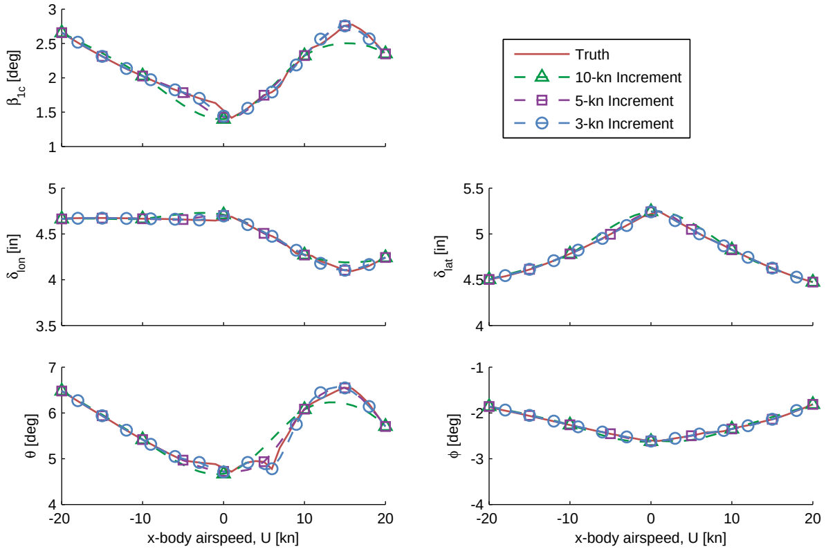
Figure 4.3: Spline-fit forward/rearward flight trim values with various spacing.
