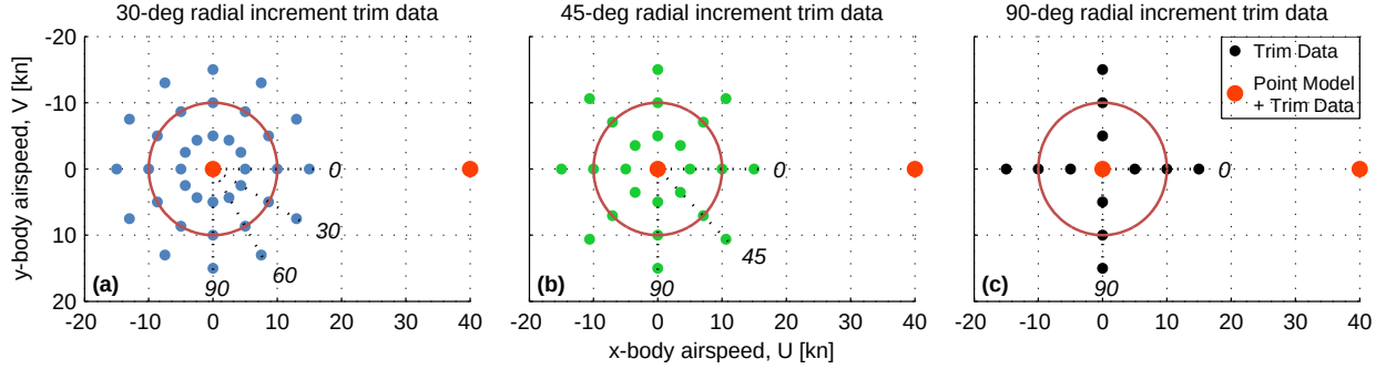
Figure 4.17: Trim data points at 30-, 45-, and 90-deg radial increments, with 10-kn magnitude indicated, and point models at hover and 40 kn.
