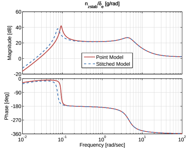
Figure 3.24: Case 2: normal acceleration response to elevator input comparison.
