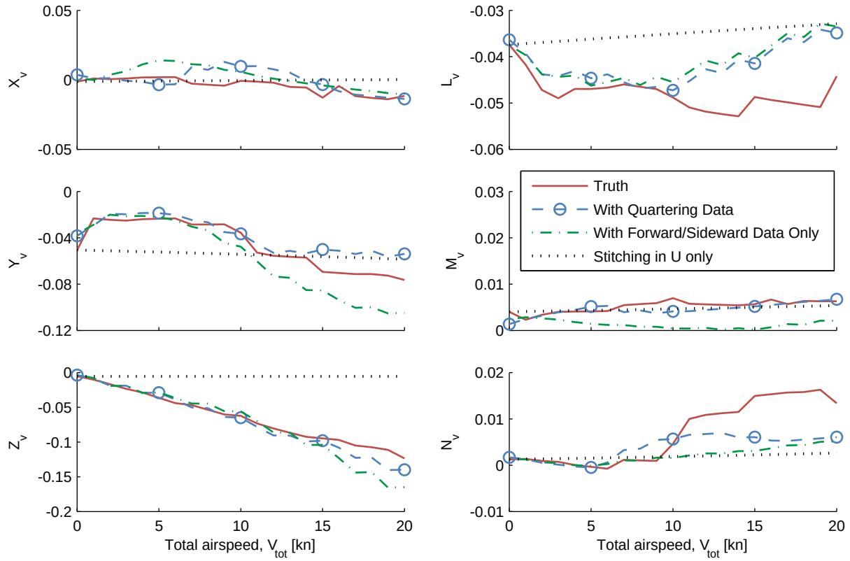
Figure 4.14: Implicit v -speed derivative values for 45-deg quartering flight up to 20 kn.
