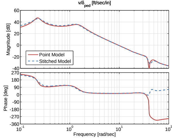
Figure 4.51: Case 2: y -body airspeed response to pedal input comparison.
