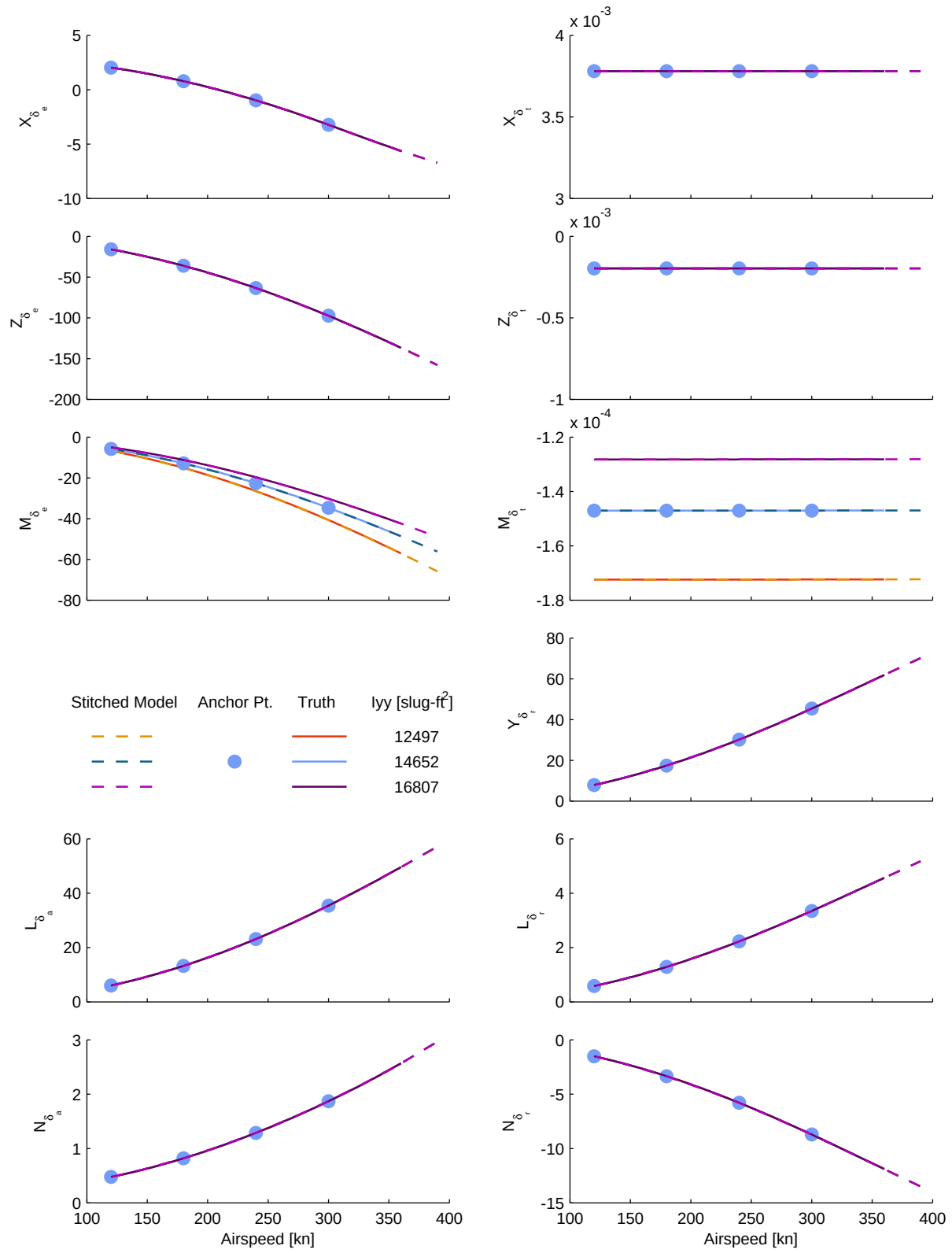
Figure B.8: Verification of off-nominal pitch inertia extrapolation, CJ1 stitched model, control derivatives.
