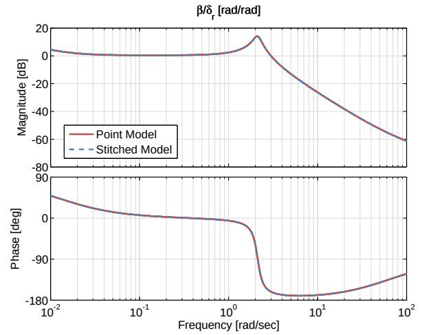
Figure 3.17: Case 1: sideslip response to rudder input comparison.
