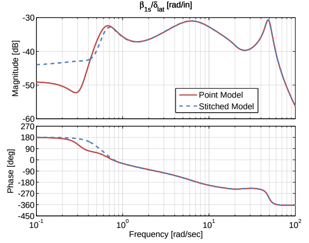
Figure 4.37: Case 1: lateral flapping angle to lateral cyclic input comparison.
