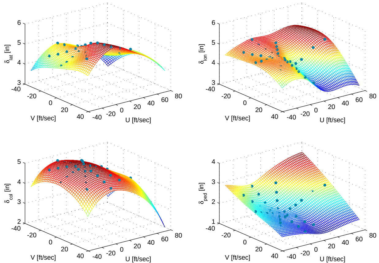
Figure 4.29: Two-dimensional interpolation of trim control values to U, V airspeed full rectangular grid – hover/low-speed regime.
