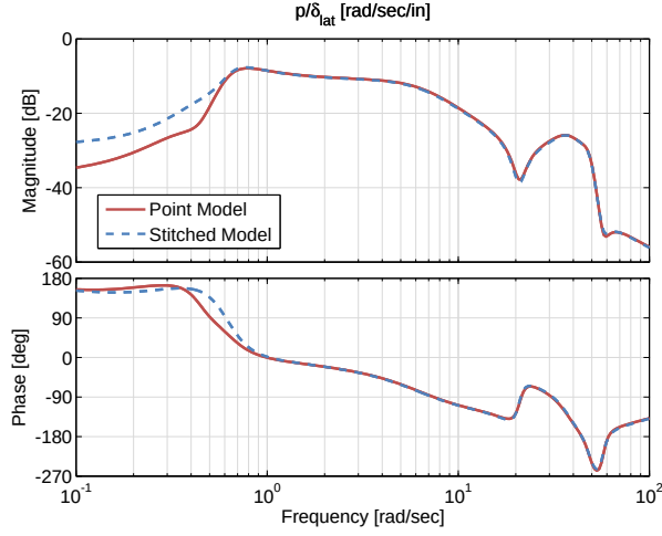
Figure 4.36: Case 1: roll rate response to lateral cyclic input comparison.
