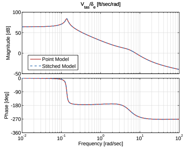
Figure 3.11: Case 1: true airspeed response to elevator input comparison.
