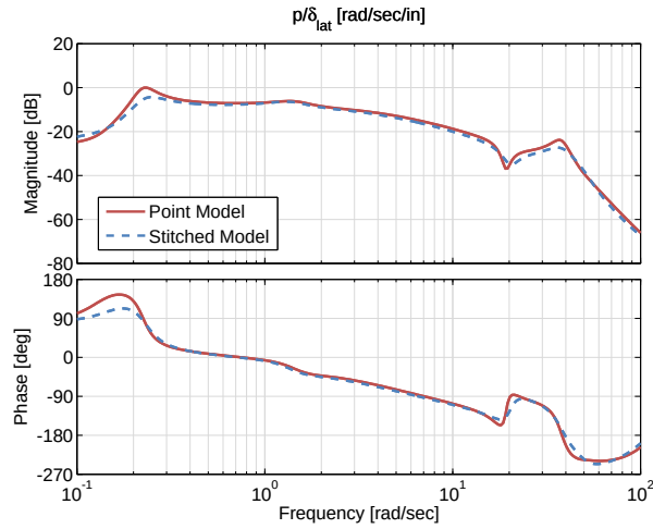
Figure 4.47: Case 2: roll rate response to lateral cyclic input comparison.
