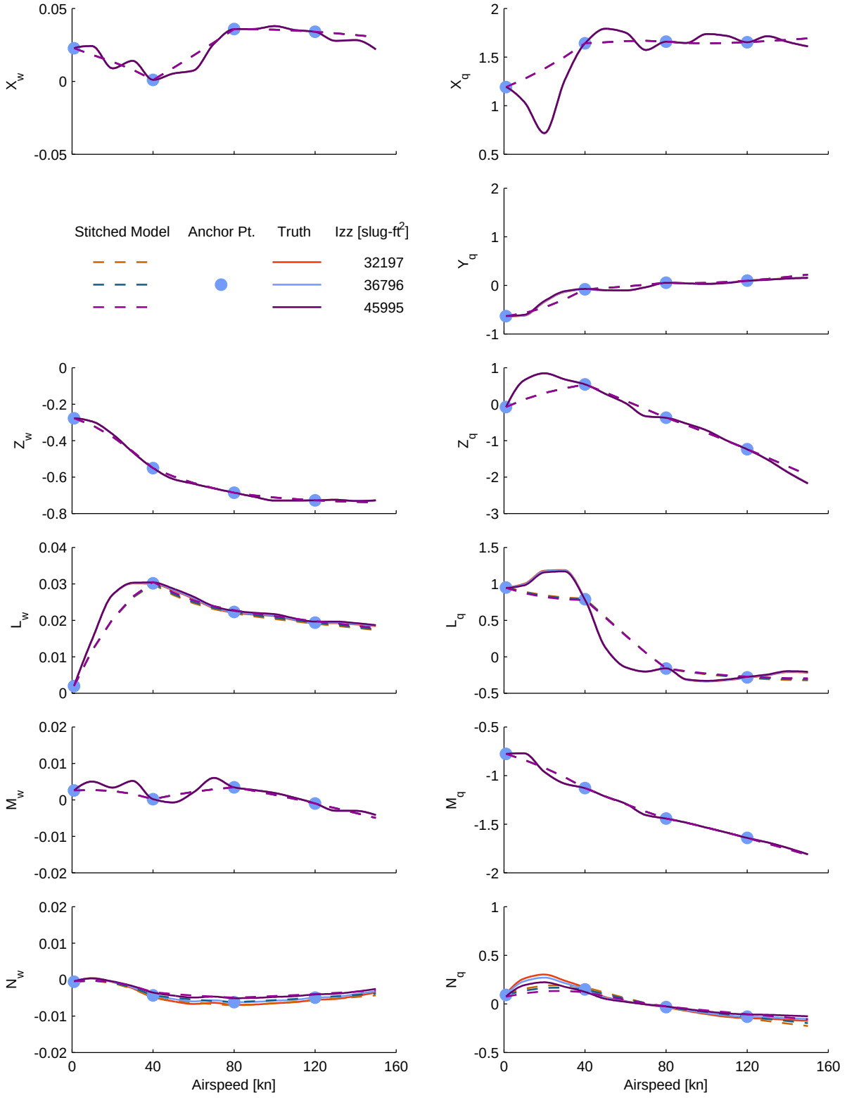
Figure C.9: Verification of off-nominal yaw inertia extrapolation, UH-60 stitched model, stability derivatives (cont.)
