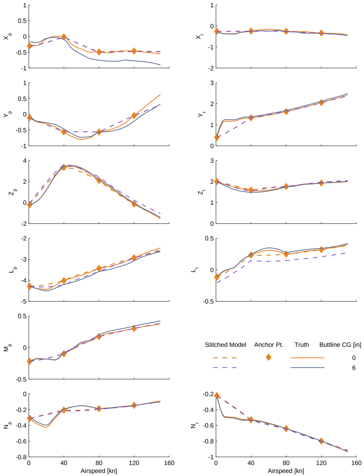
Figure C.15: Verification of off-nominal buttline CG extrapolation, UH-60 stitched model, stability derivatives (cont.)
