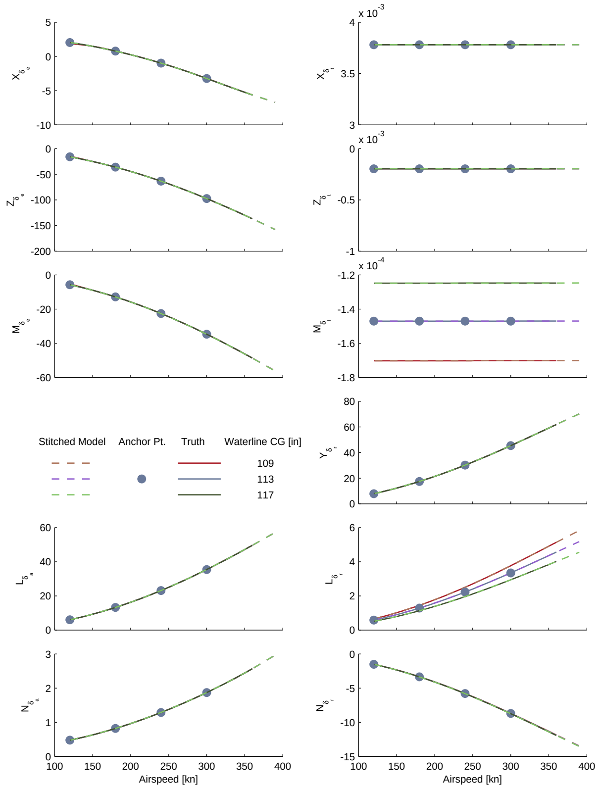
Figure B.16: Verification of off-nominal waterline CG extrapolation, CJ1 stitched model, control derivatives.
