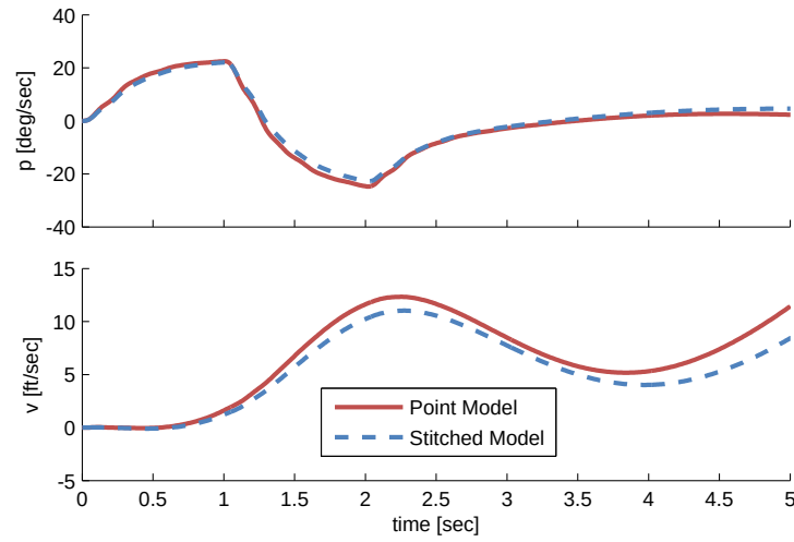
Figure 4.54: Case 2: short-term time history responses, lateral cyclic doublet.
