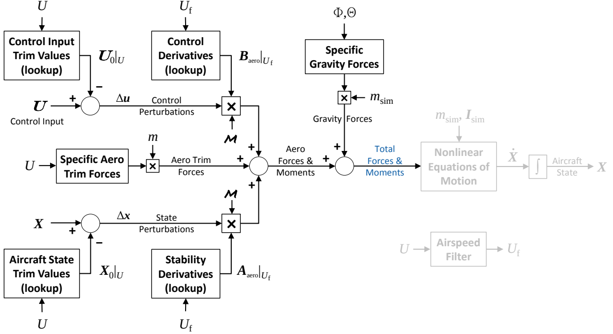
Figure 2.8: Model stitching simulation architecture – total forces and moments.
