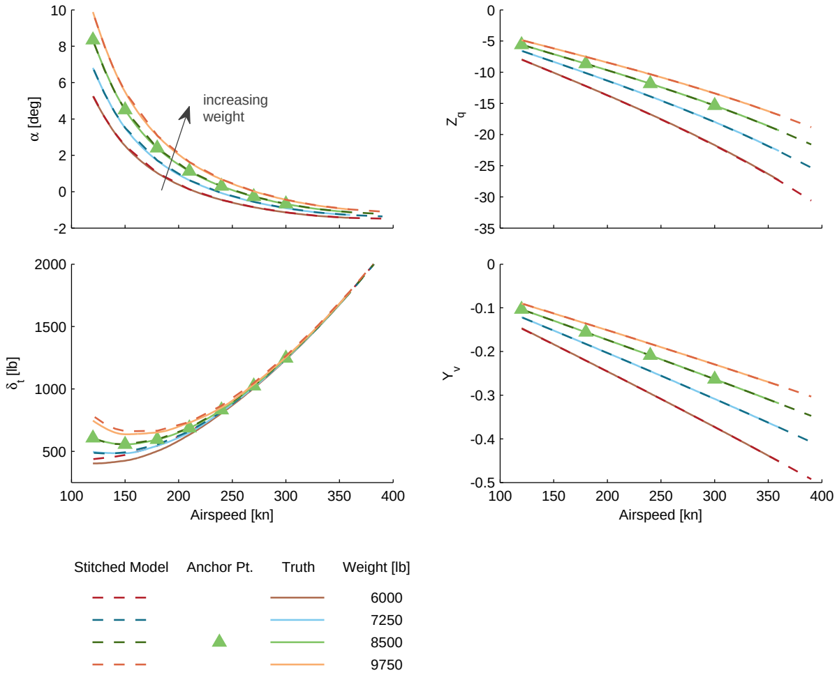
Figure 3.5: Verification of off-nominal weight extrapolation.
