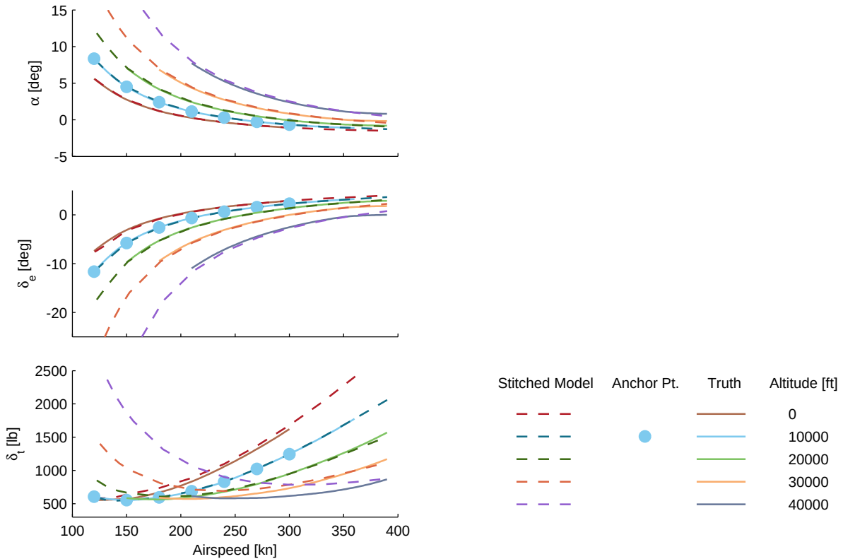
Figure B.17: Verification of single-altitude extrapolation, 10,000 ft, CJ1 stitched model, trim.
