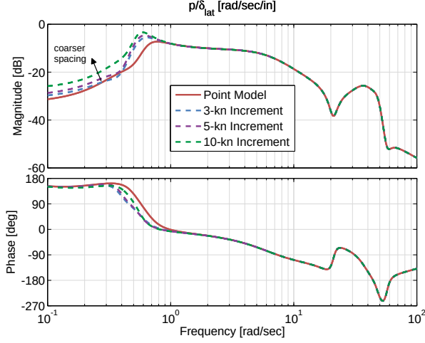
Figure 4.5: Roll rate response to lateral cyclic input comparison for forward/rearward trim data of various spacing, hover.
