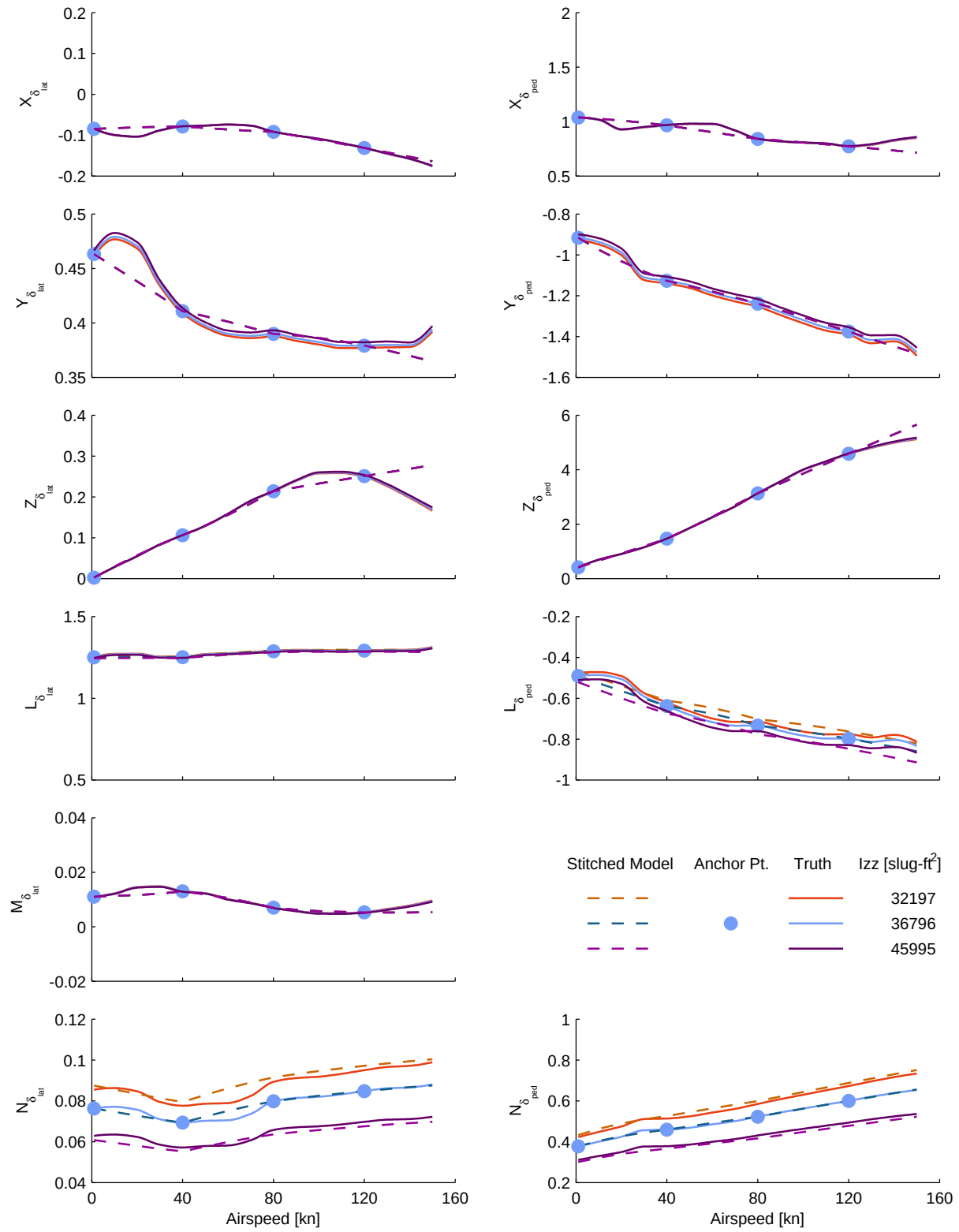
Figure C.10: Verification of off-nominal yaw inertia extrapolation, UH-60 stitched model, control derivatives (cont.)
