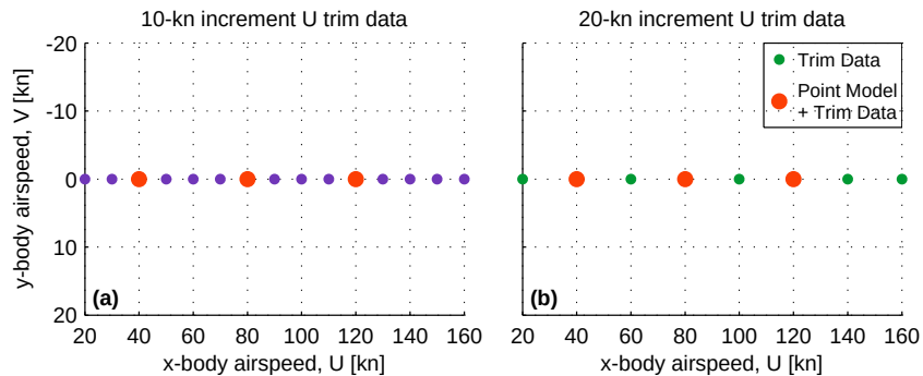
Figure 4.19: Forward-flight trim data points at 10- and 20-kn x -body airspeed U increments, and point models at 40, 80, and 120 kn.
