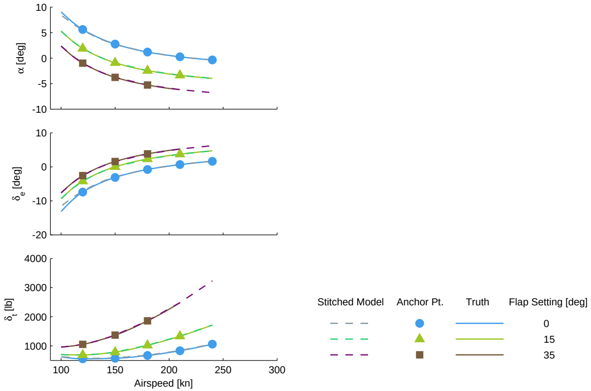
Figure B.26: Alternate configuration verification, flap setting, CJ1 stitched model, trim.
