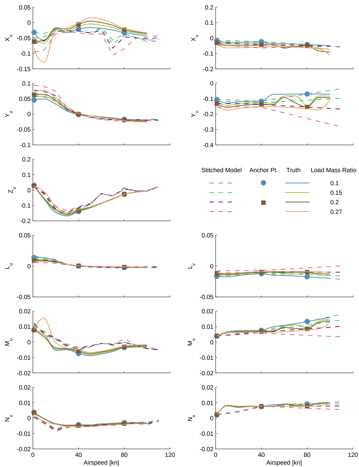
Figure C.21: Alternate configuration verification, sling-load weight, UH-60 stitched model, stability derivatives.
