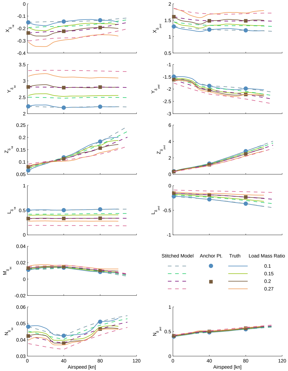
Figure C.22: Alternate configuration verification, sling-load weight, UH-60 stitched model, control derivatives (cont.)
