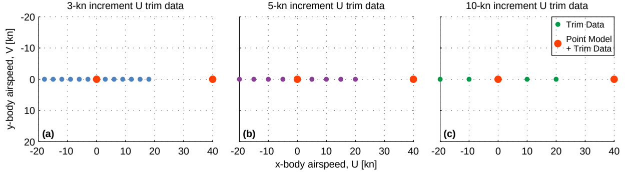
Figure 4.2: Forward/rearward flight trim data points at 3-, 5-, and 10-kn x -body airspeed U increments, and point models at hover and 40 kn.
