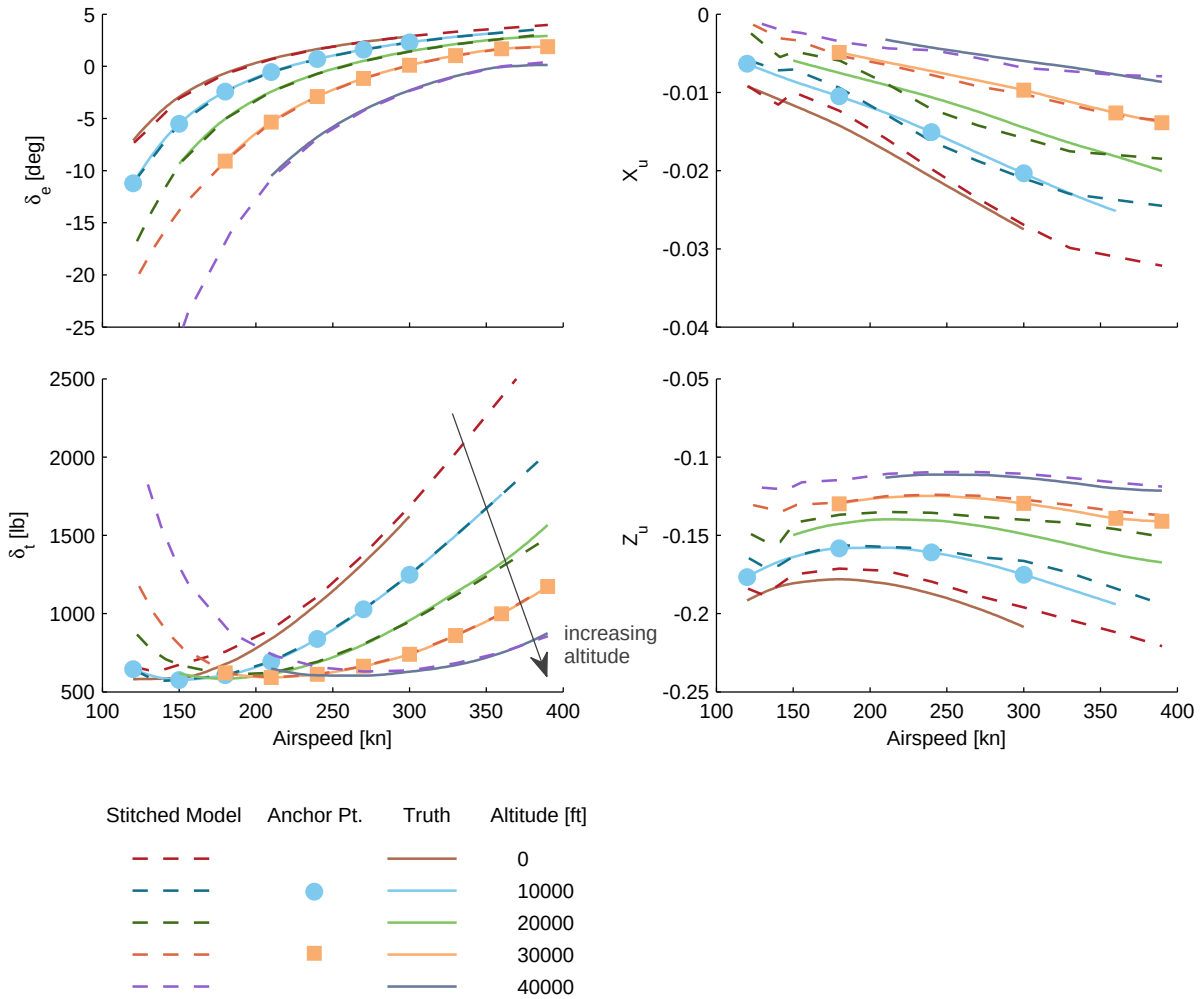
Figure 3.9: Verification of altitude extrapolation.
