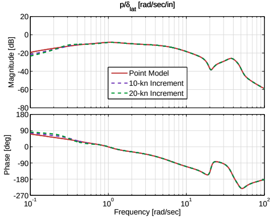
Figure 4.22: Roll rate response to lateral cyclic input comparison for forward-flight trim data of 10- and 20-kn spacing, 40 kn.
