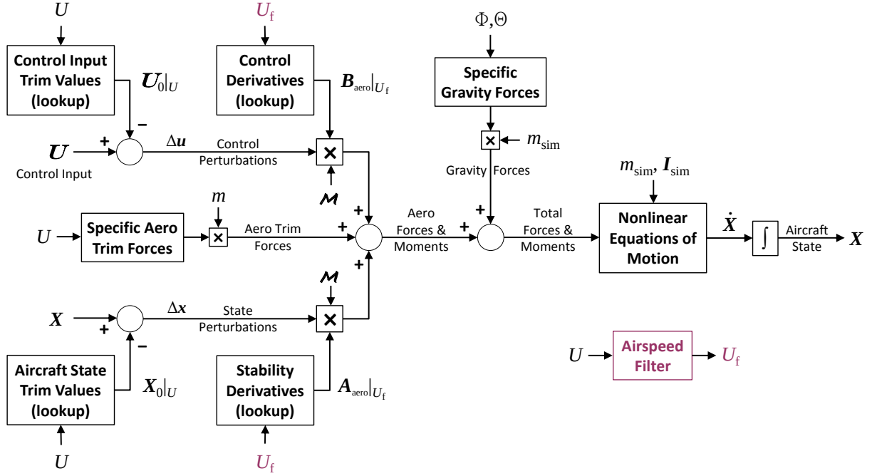
Figure 2.11: Model stitching simulation architecture – airspeed filter.
