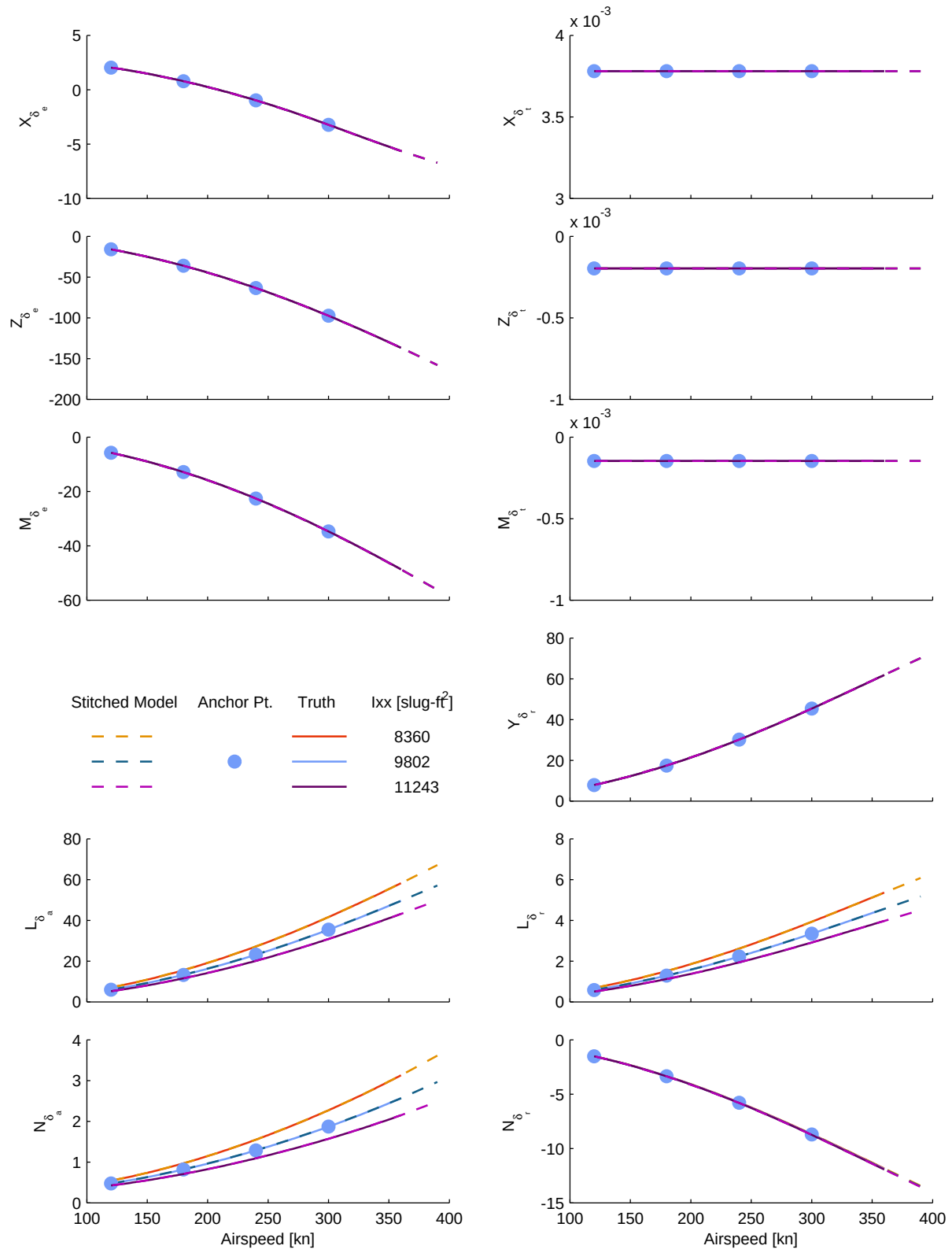
Figure B.6: Verification of off-nominal roll inertia extrapolation, CJ1 stitched model, control derivatives.
