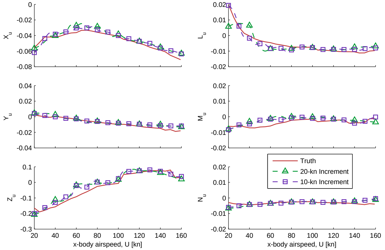
Figure 4.21: Implicit u -speed derivative values due to forward-flight trim data of 10- and 20-kn spacing.
