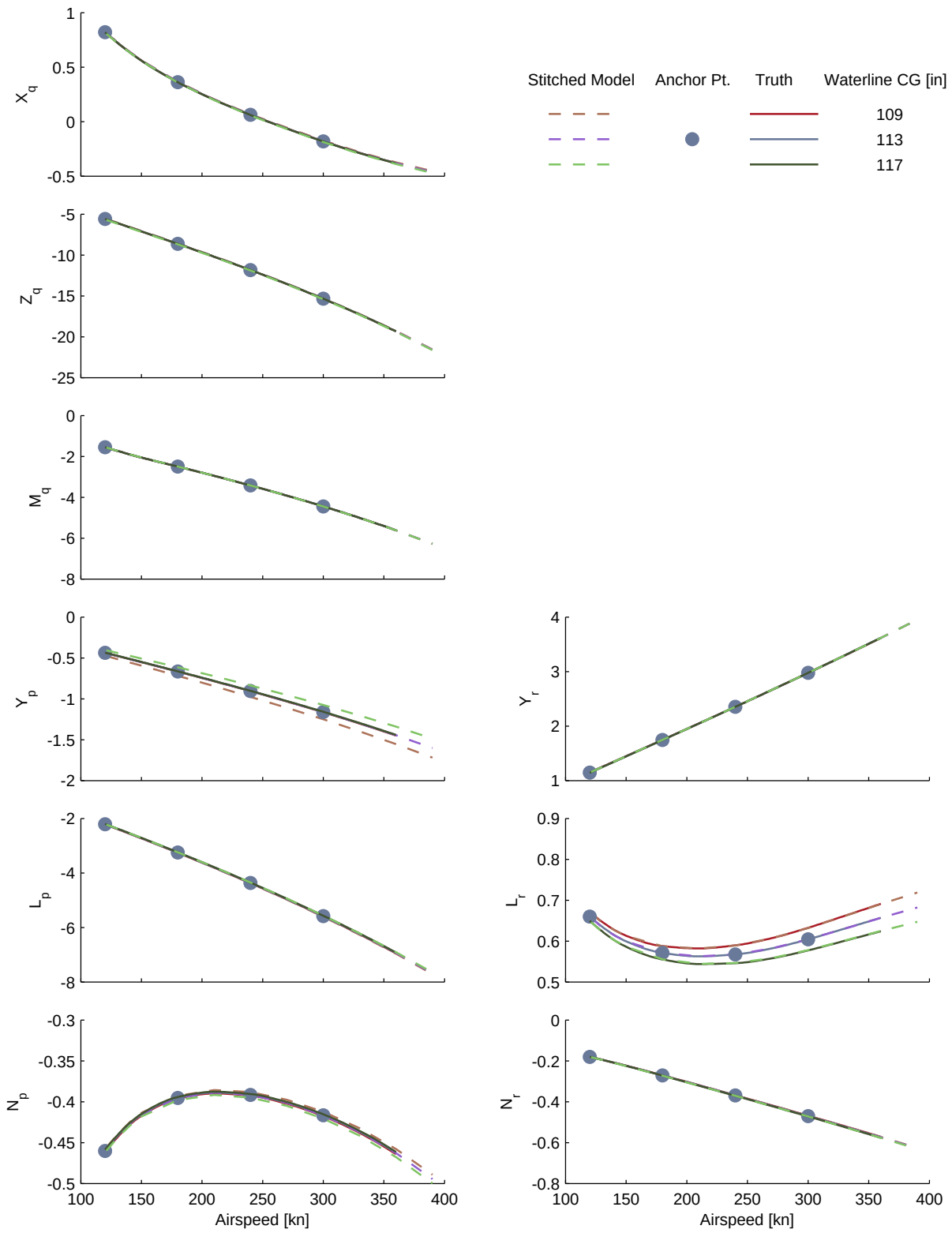
Figure B.15: Verification of off-nominal waterline CG extrapolation, CJ1 stitched model, stability derivatives (cont.)
