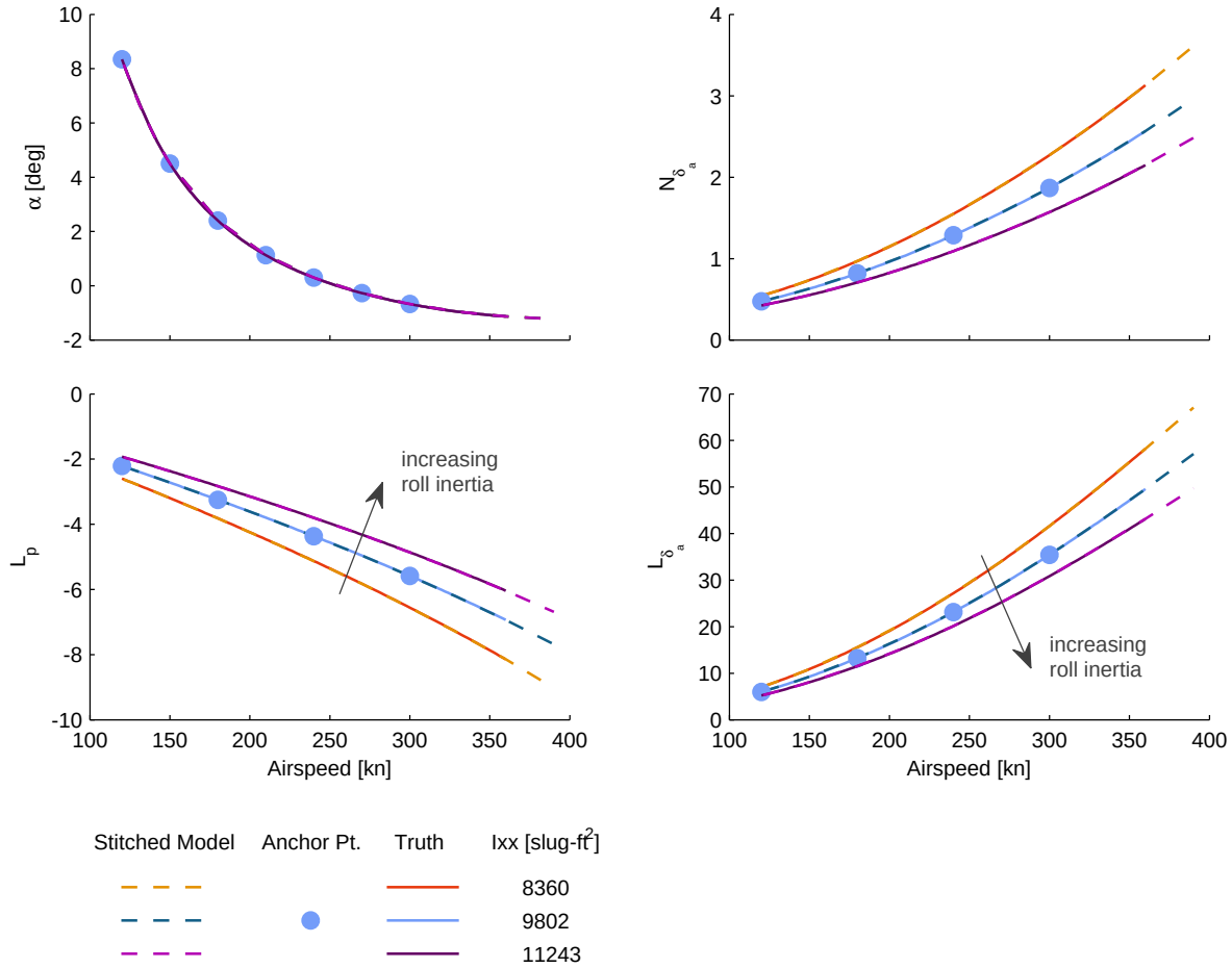
Figure 3.6: Verification of off-nominal inertia extrapolation, roll inertia I_{xx} .
