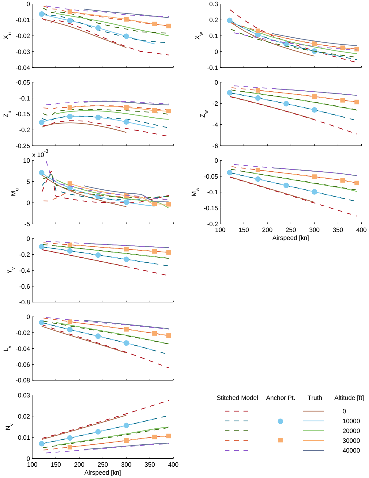
Figure B.24: Verification of altitude extrapolation, two altitudes, CJ1 stitched model, stability derivatives.
