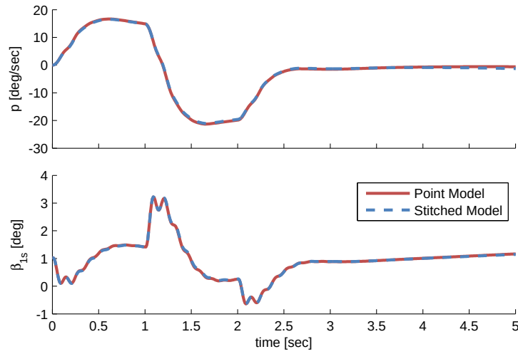
Figure 4.43: Case 1: short-term time history responses, lateral cyclic doublet.
