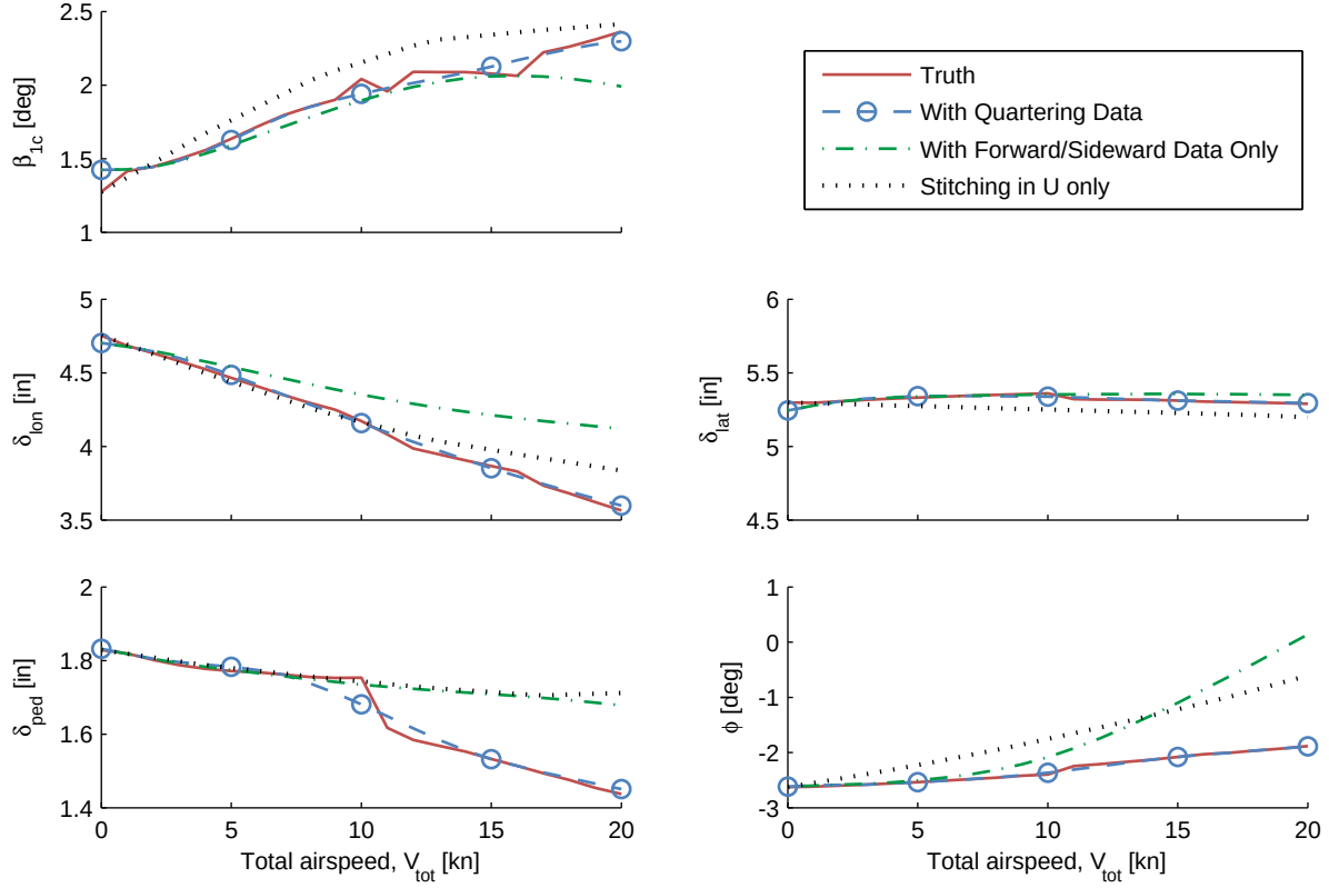
Figure 4.13: Trim values for 45-deg quartering flight up to 20 kn.
