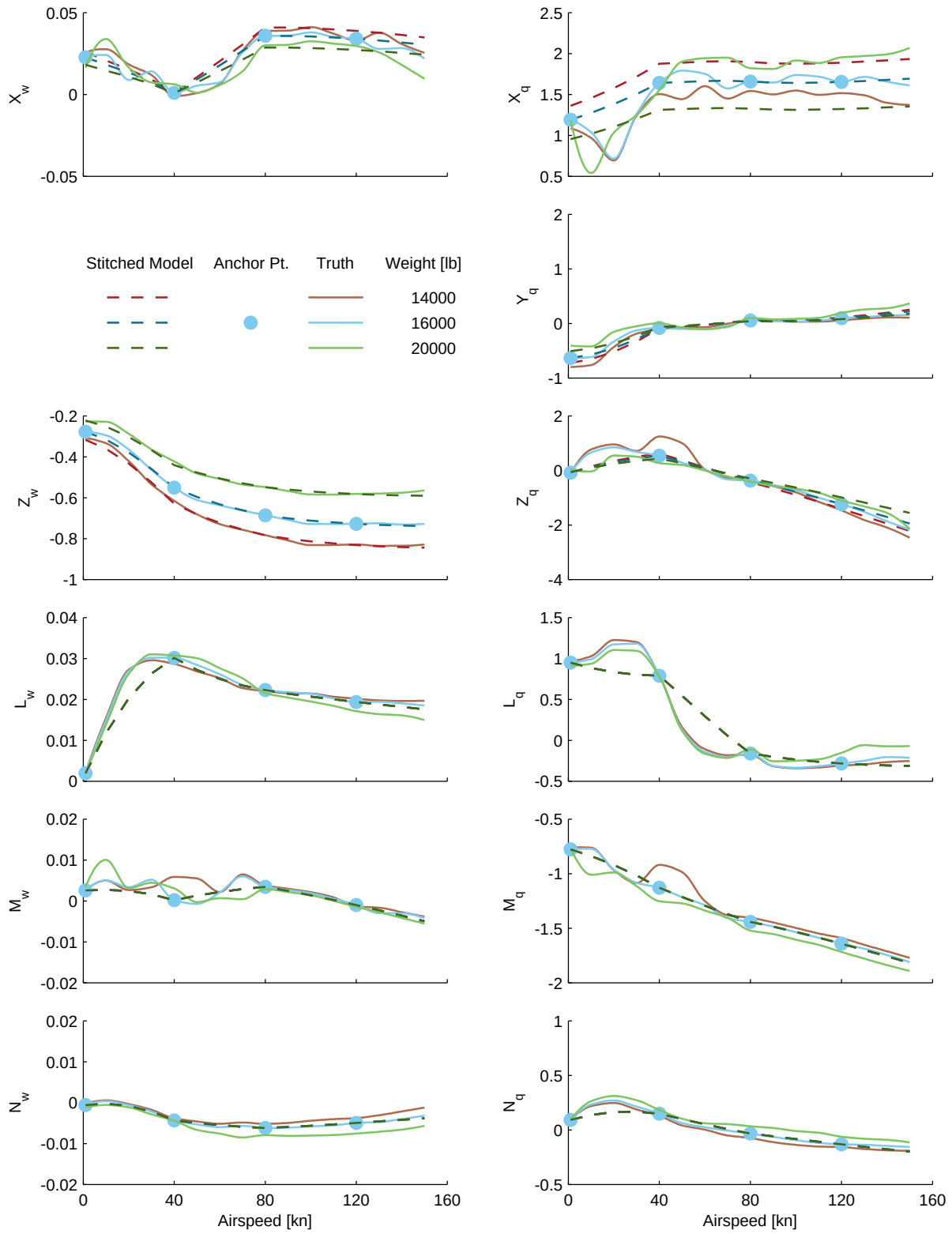
Figure C.2: Verification of off-nominal weight extrapolation, UH-60 stitched model, stability derivatives (cont.)
