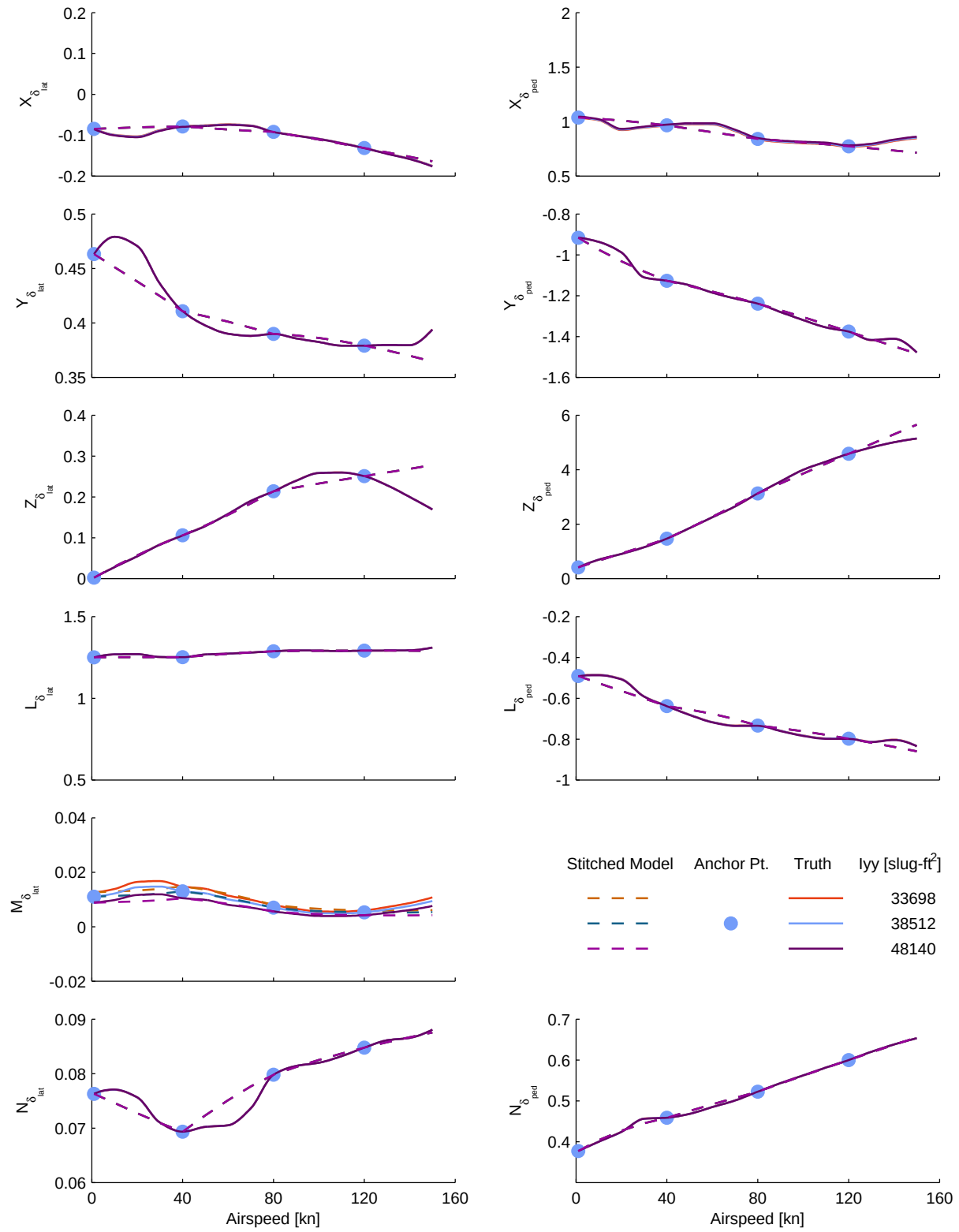
Figure C.8: Verification of off-nominal pitch inertia extrapolation, UH-60 stitched model, control derivatives (cont.)
