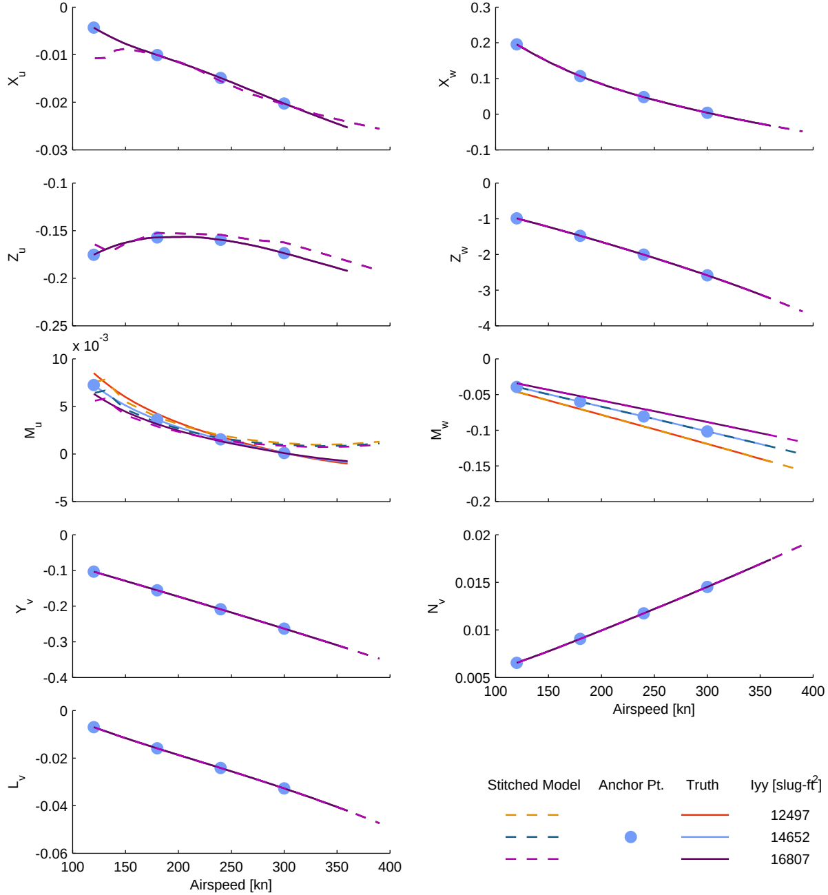
Figure B.7: Verification of off-nominal pitch inertia extrapolation, CJ1 stitched model, stability derivatives.
