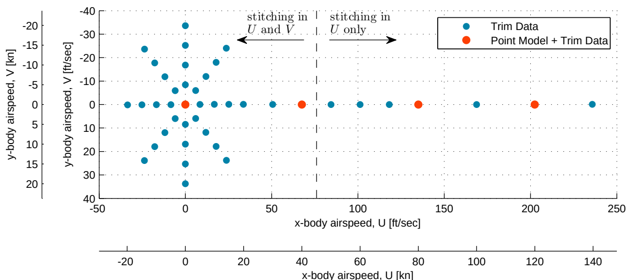
Figure 4.28: U, V airspeed points for anchor trim data and point models included in the stitched model.
