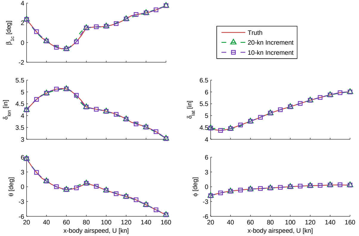
Figure 4.20: Spline-fit forward-flight trim values with 10- and 20-kn spacing.
