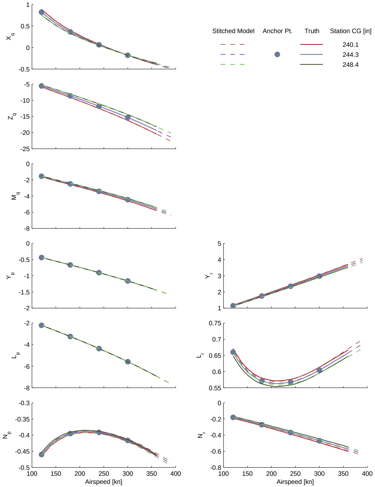
Figure B.12: Verification of off-nominal station CG extrapolation, CJ1 stitched model, stability derivatives (cont.)
