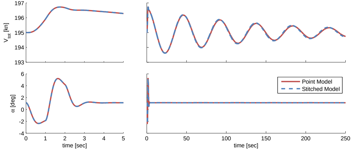
Figure 3.18: Case 1: short- and long-term time history responses, elevator doublet.
