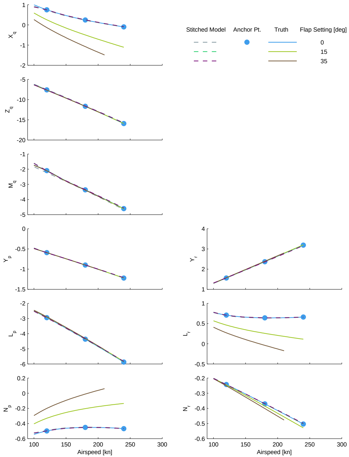
Figure B.27: Alternate configuration verification, flap setting, CJ1 stitched model, stability derivatives (cont.)
