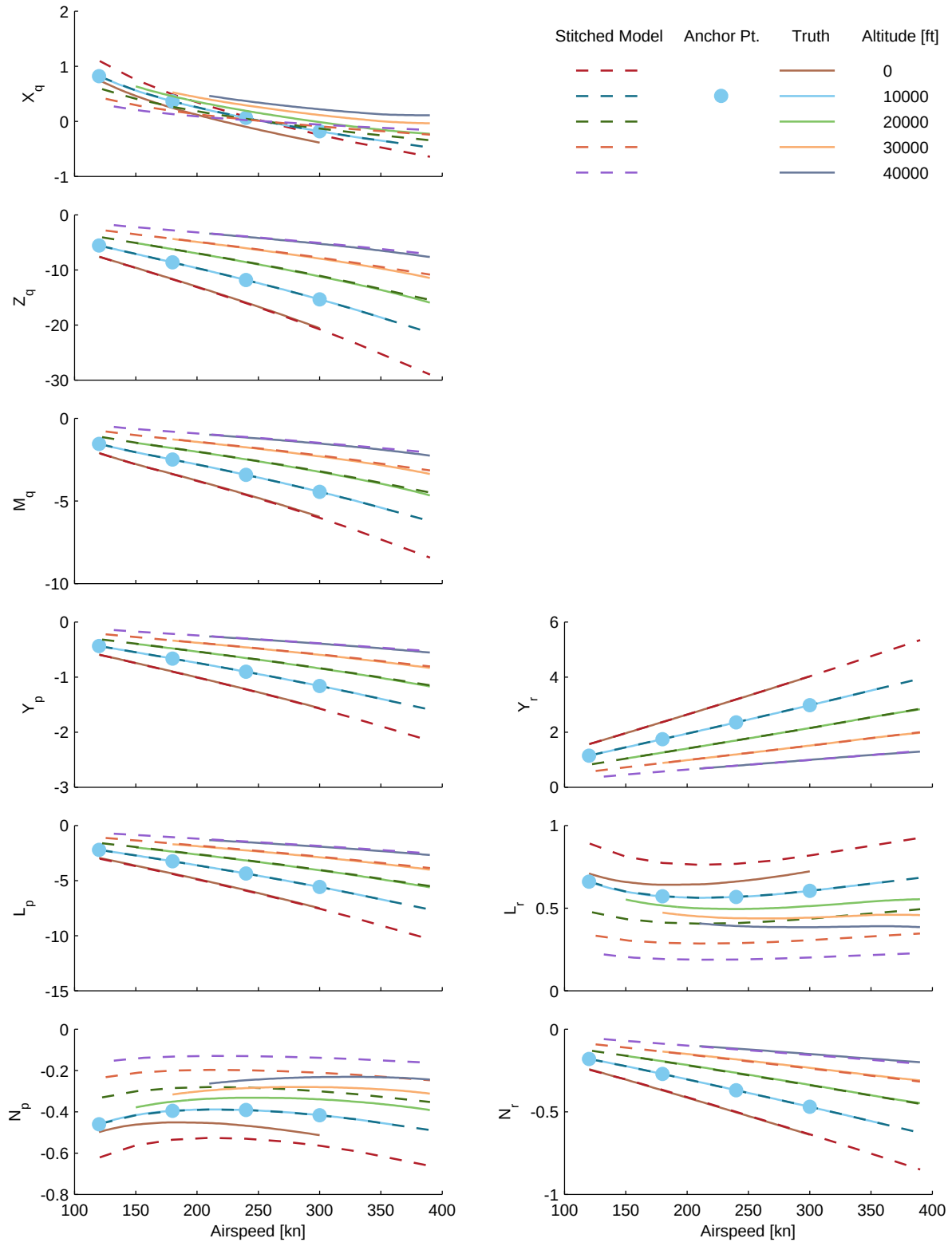
Figure B.18: Verification of single-altitude extrapolation, 10,000 ft, CJ1 stitched model, stability derivatives (cont.)
