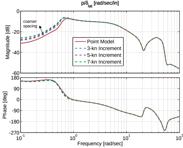
Figure 4.10: Roll rate response to lateral cyclic input comparison for sideward trim data of various spacing, hover.
