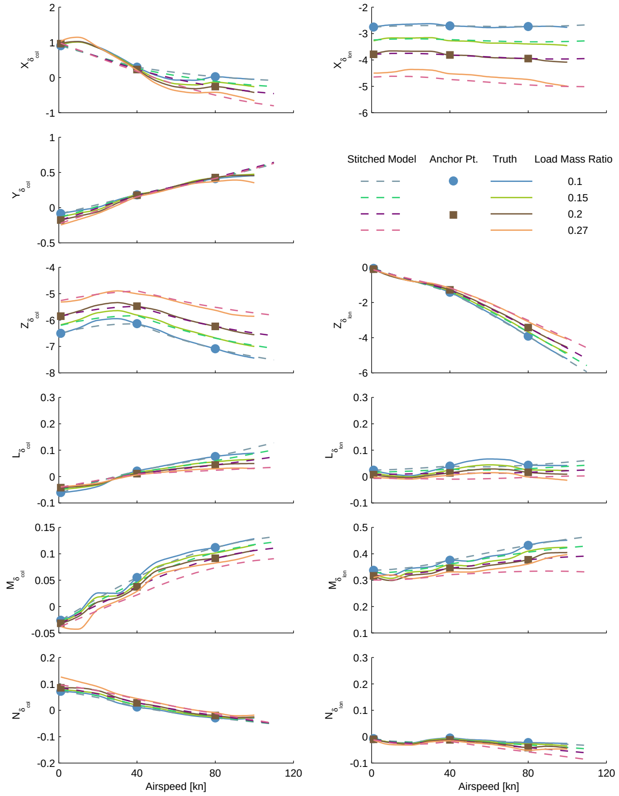
Figure C.22: Alternate configuration verification, sling-load weight, UH-60 stitched model, control derivatives.
