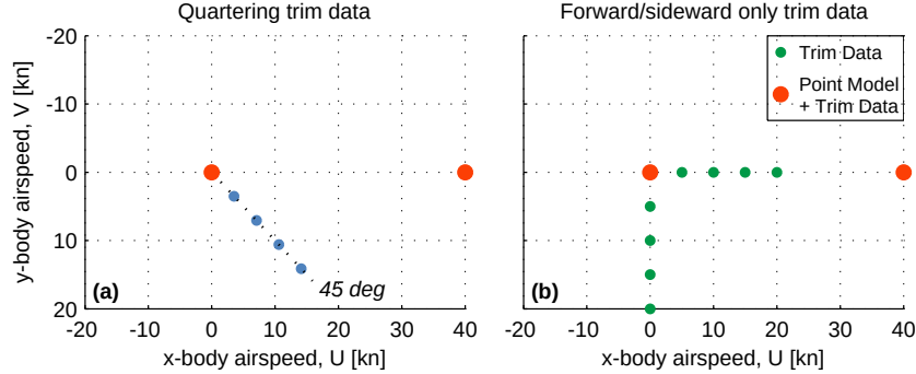
Figure 4.12: Quartering and pure forward/sideward flight trim data points at 5-kn airspeed V_{\text{tot}} increments, and point models at hover and 40 kn.
