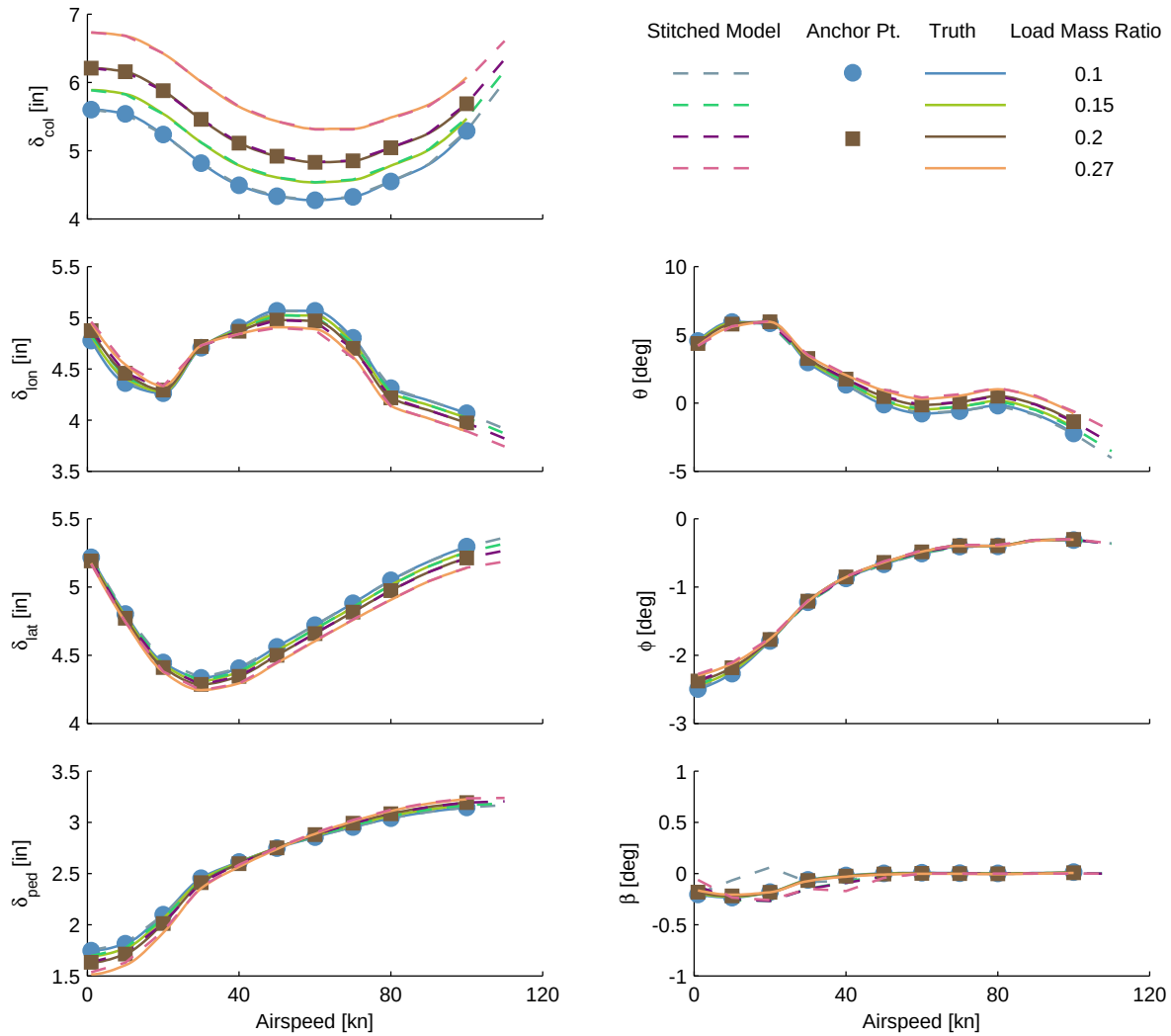
Figure C.20: Alternate configuration verification, sling-load weight, UH-60 stitched model, trim.
