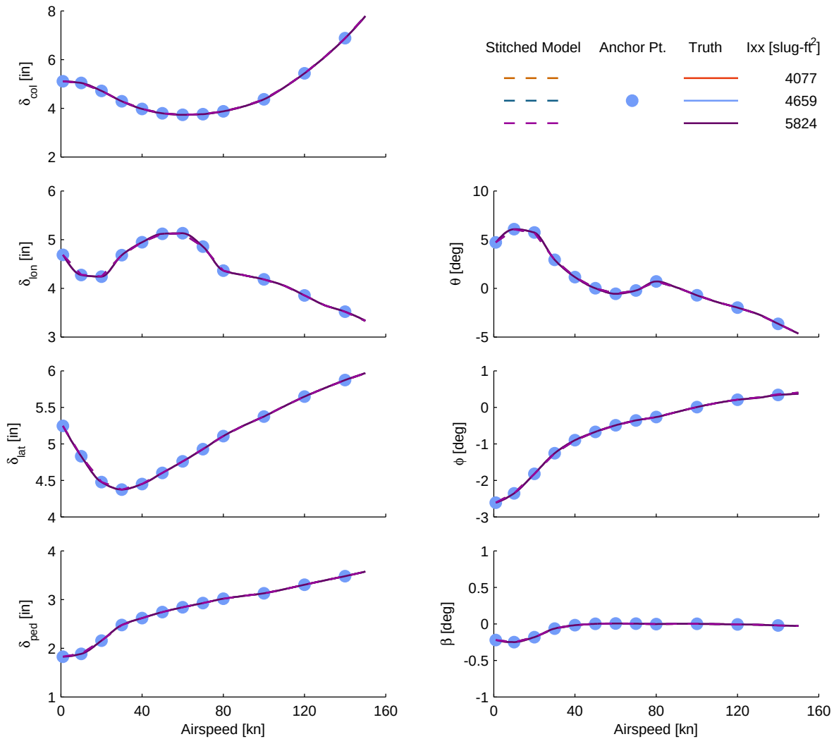
Figure C.4: Verification of off-nominal roll inertia extrapolation, UH-60 stitched model, trim.
