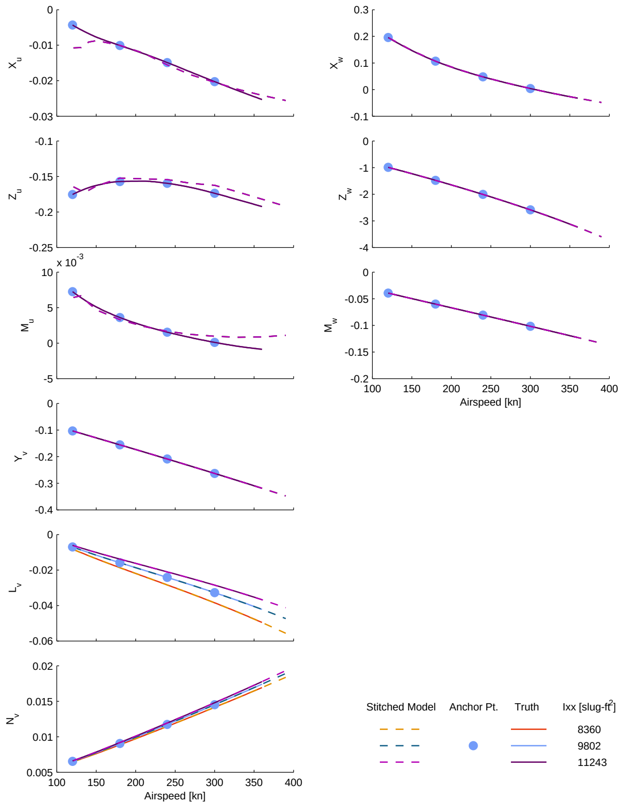
Figure B.5: Verification of off-nominal roll inertia extrapolation, CJ1 stitched model, stability derivatives.
