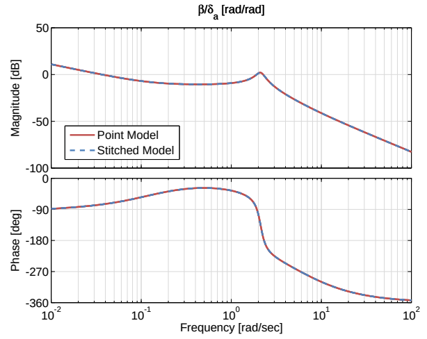
Figure 3.15: Case 1: sideslip response to aileron input comparison.
