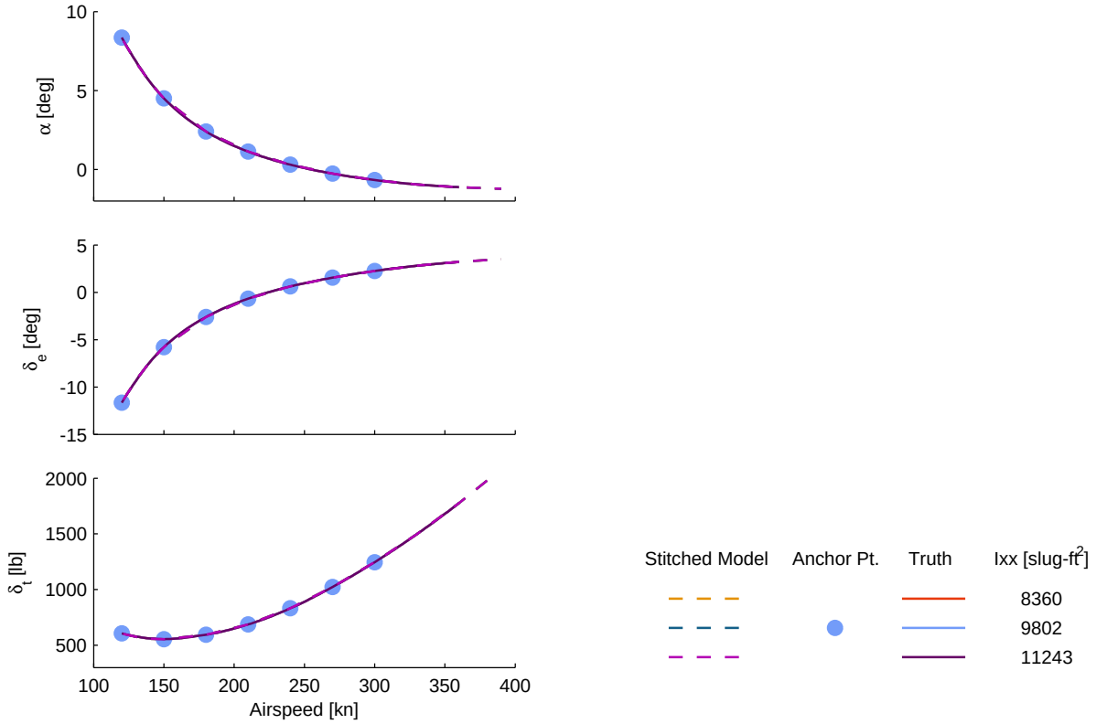
Figure B.4: Verification of off-nominal roll inertia extrapolation, CJ1 stitched model, trim.
