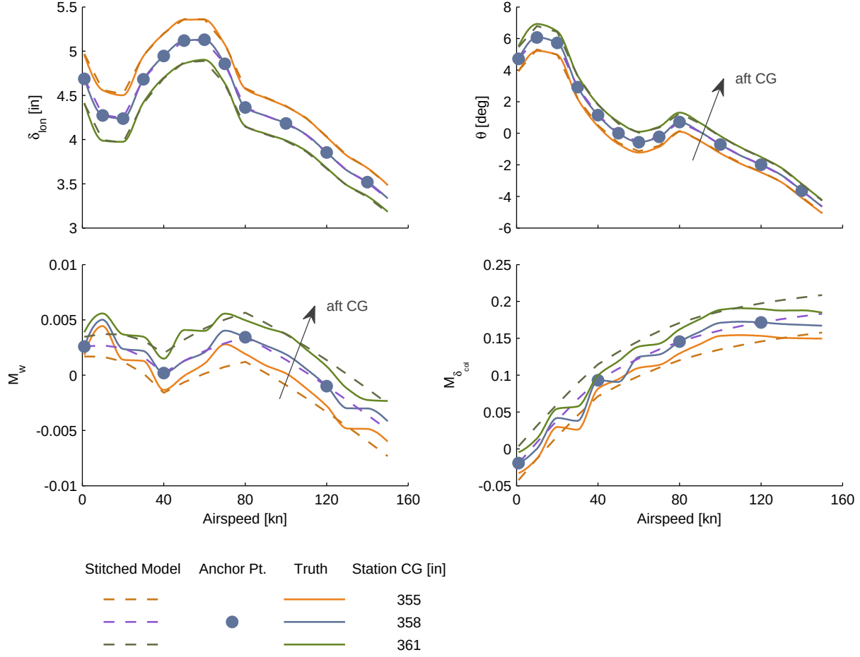
Figure 4.32: Verification of off-nominal CG extrapolation, fuselage station.
