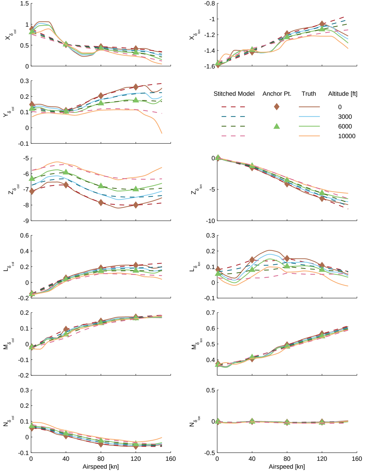
Figure C.19: Verification of altitude extrapolation, UH-60 stitched model, control derivatives.
