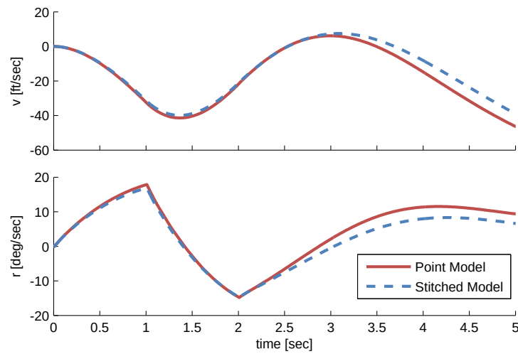
Figure 4.55: Case 2: short-term time history responses, pedal doublet.
