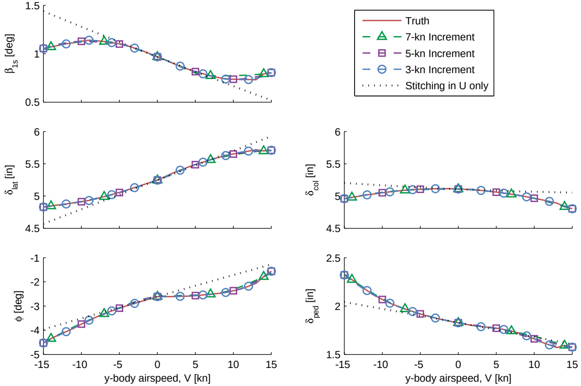
Figure 4.8: Spline-fit sideward flight trim values with various spacing.
