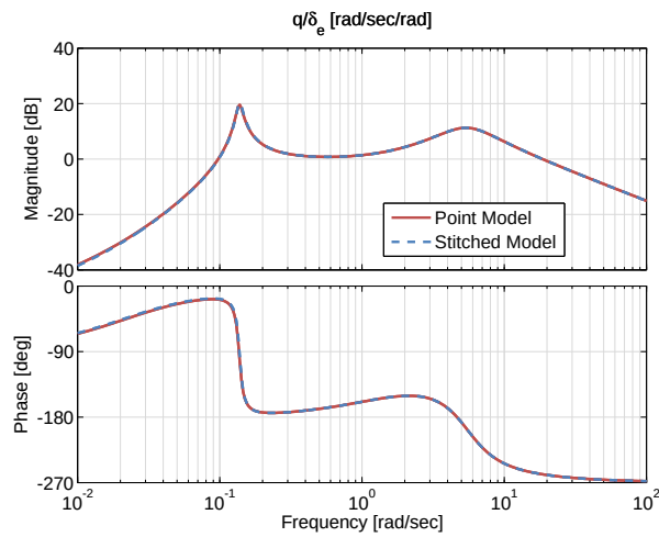
Figure 3.12: Case 1: pitch rate response to elevator input comparison.
