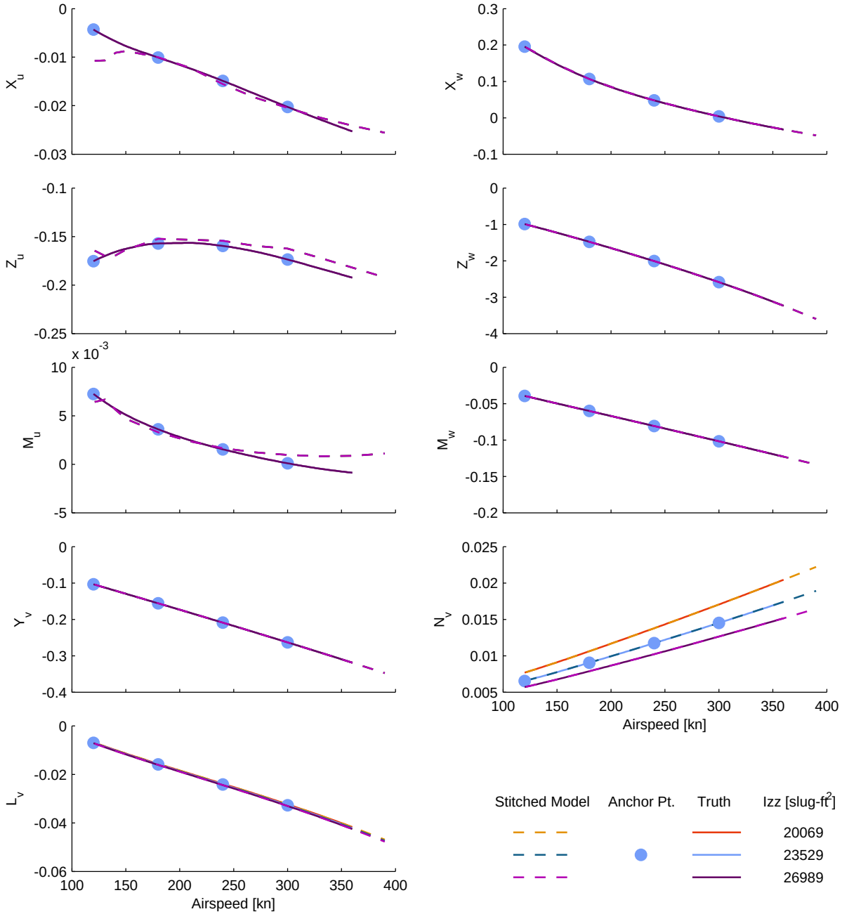
Figure B.9: Verification of off-nominal yaw inertia extrapolation, CJ1 stitched model, stability derivatives.
