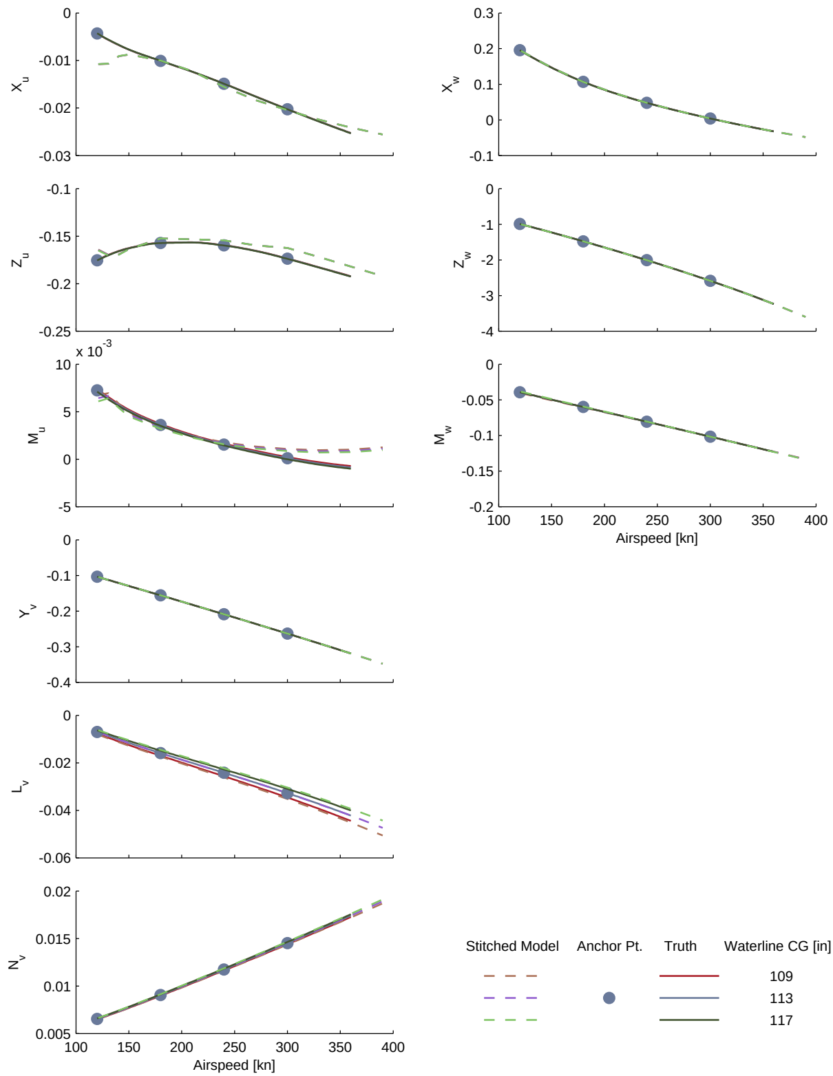
Figure B.15: Verification of off-nominal waterline CG extrapolation, CJ1 stitched model, stability derivatives.
