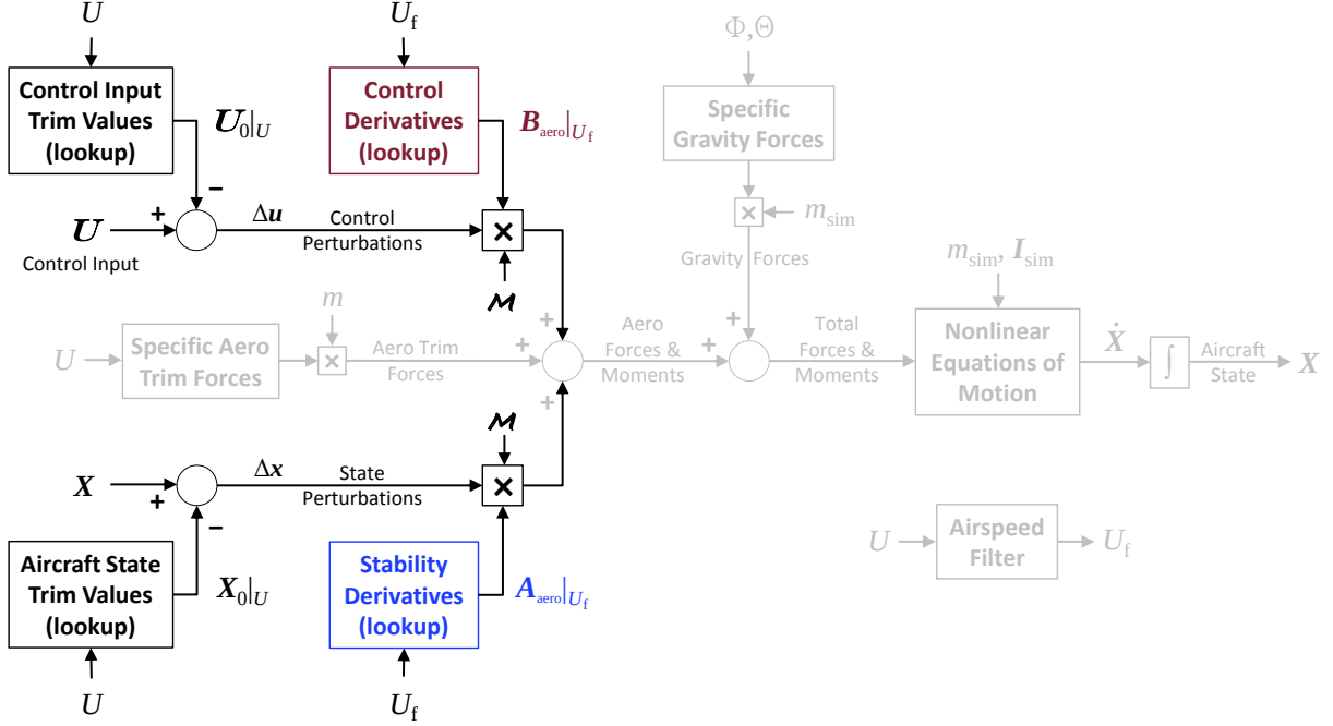
Figure 2.4: Model stitching simulation architecture – aero perturbation forces and moments.
