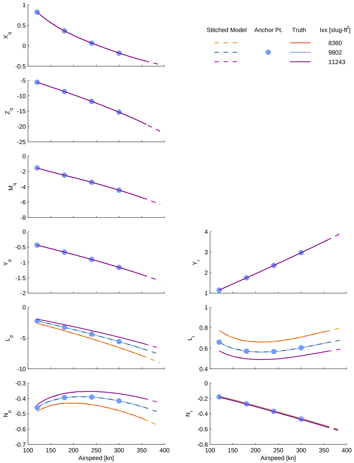
Figure B.5: Verification of off-nominal roll inertia extrapolation, CJ1 stitched model, stability derivatives (cont.)
