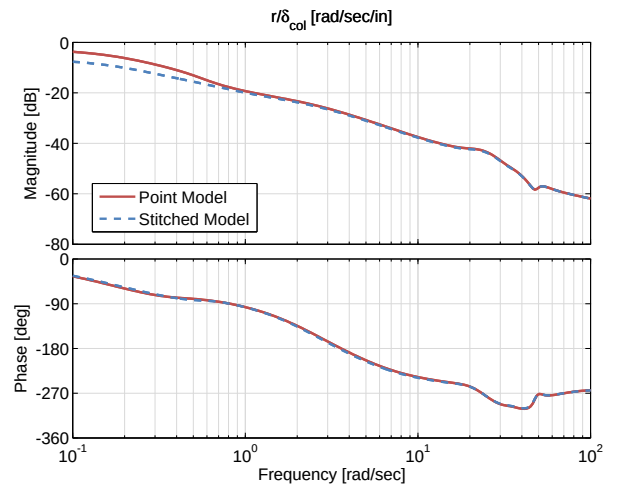
Figure 4.39: Case 1: yaw rate response to collective input comparison.
