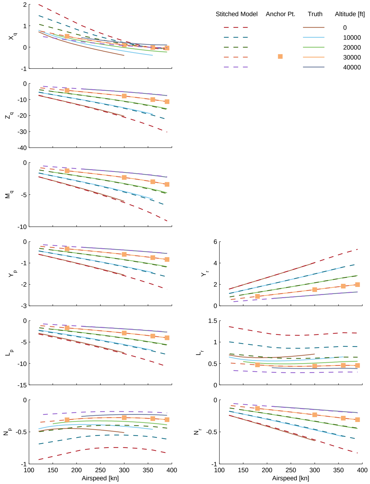
Figure B.21: Verification of single-altitude extrapolation, 30,000 ft, CJ1 stitched model, stability derivatives (cont.)
