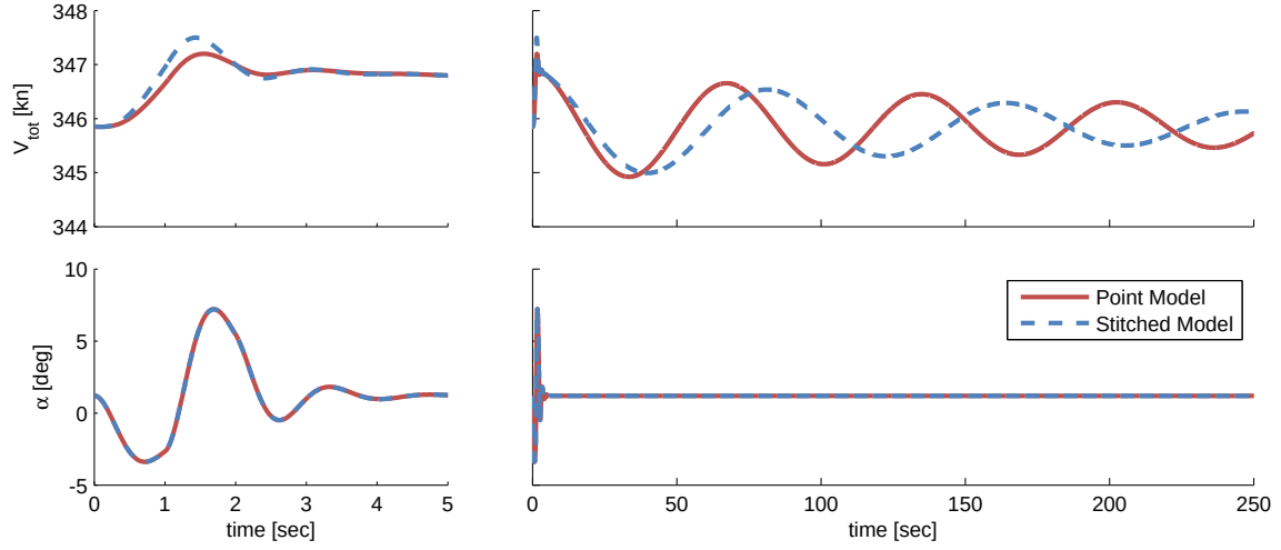
Figure 3.29: Case 2: short- and long-term time history responses, elevator doublet.
