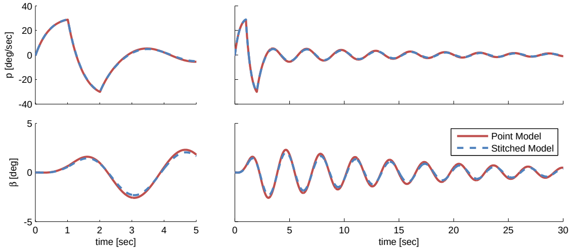
Figure 3.30: Case 2: short- and long-term time history responses, aileron doublet.
