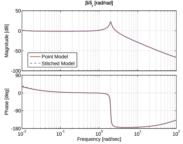
Figure 3.28: Case 2: sideslip response to rudder input comparison.
