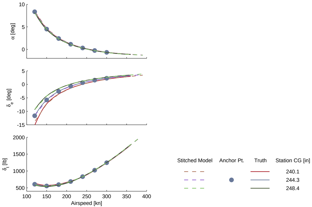
Figure B.11: Verification of off-nominal station CG extrapolation, CJ1 stitched model, trim.
