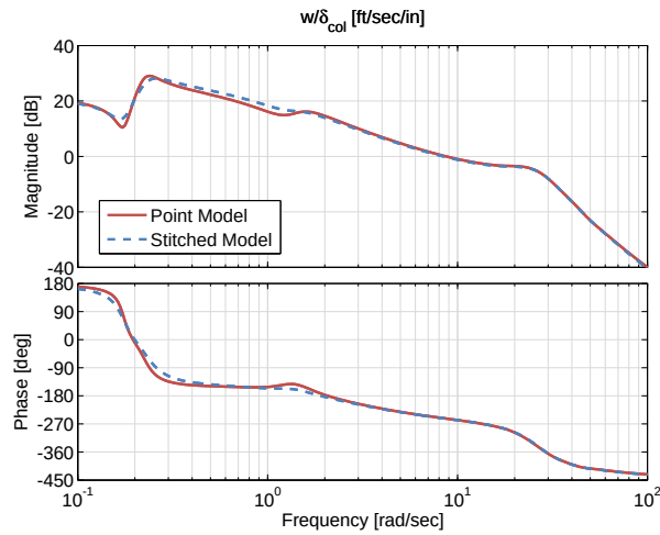
Figure 4.49: Case 2: z -body airspeed response to collective input comparison.
