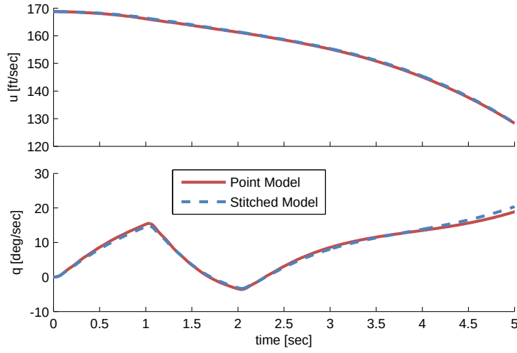
Figure 4.53: Case 2: short-term time history responses, longitudinal cyclic doublet.
