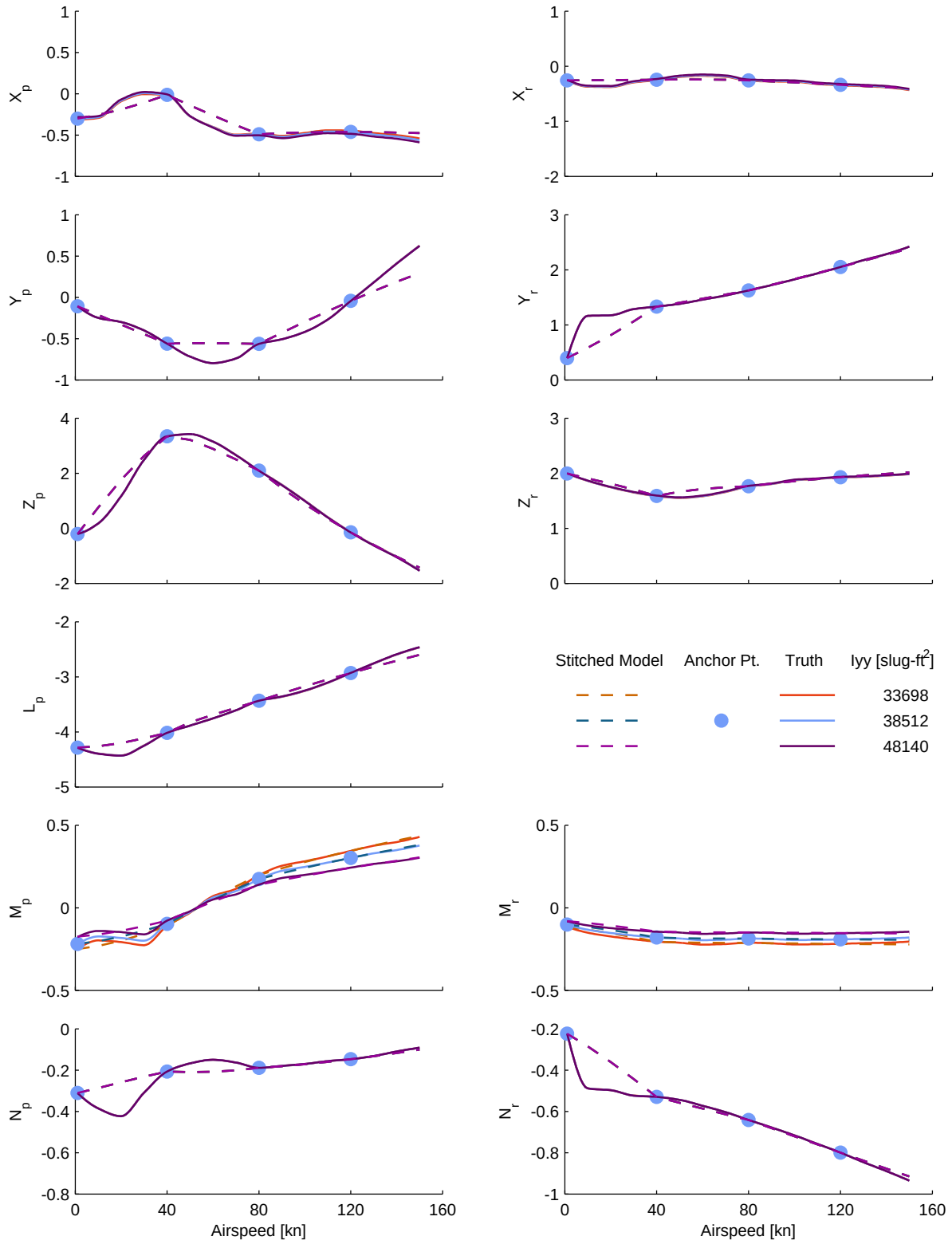
Figure C.7: Verification of off-nominal pitch inertia extrapolation, UH-60 stitched model, stability derivatives (cont.)
