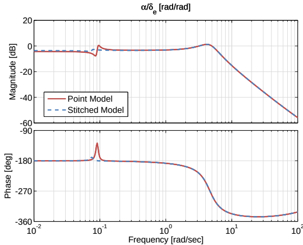
Figure 3.21: Case 2: angle of attack response to elevator input comparison.
