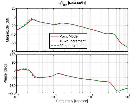
Figure 4.25: Pitch rate response to longitudinal cyclic input comparison for forward-flight trim data of 10- and 20-kn spacing, 80 kn.
