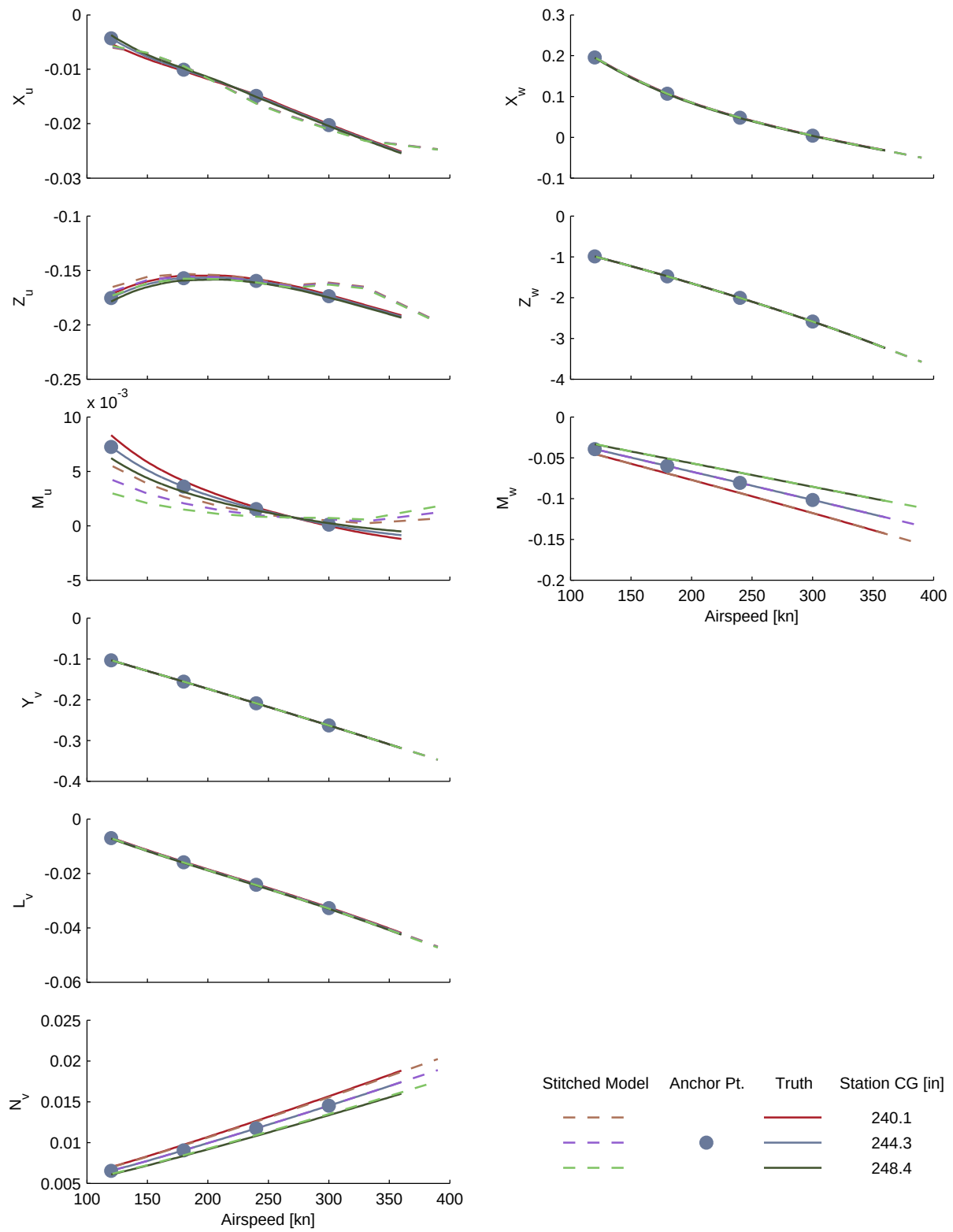
Figure B.12: Verification of off-nominal station CG extrapolation, CJ1 stitched model, stability derivatives.
