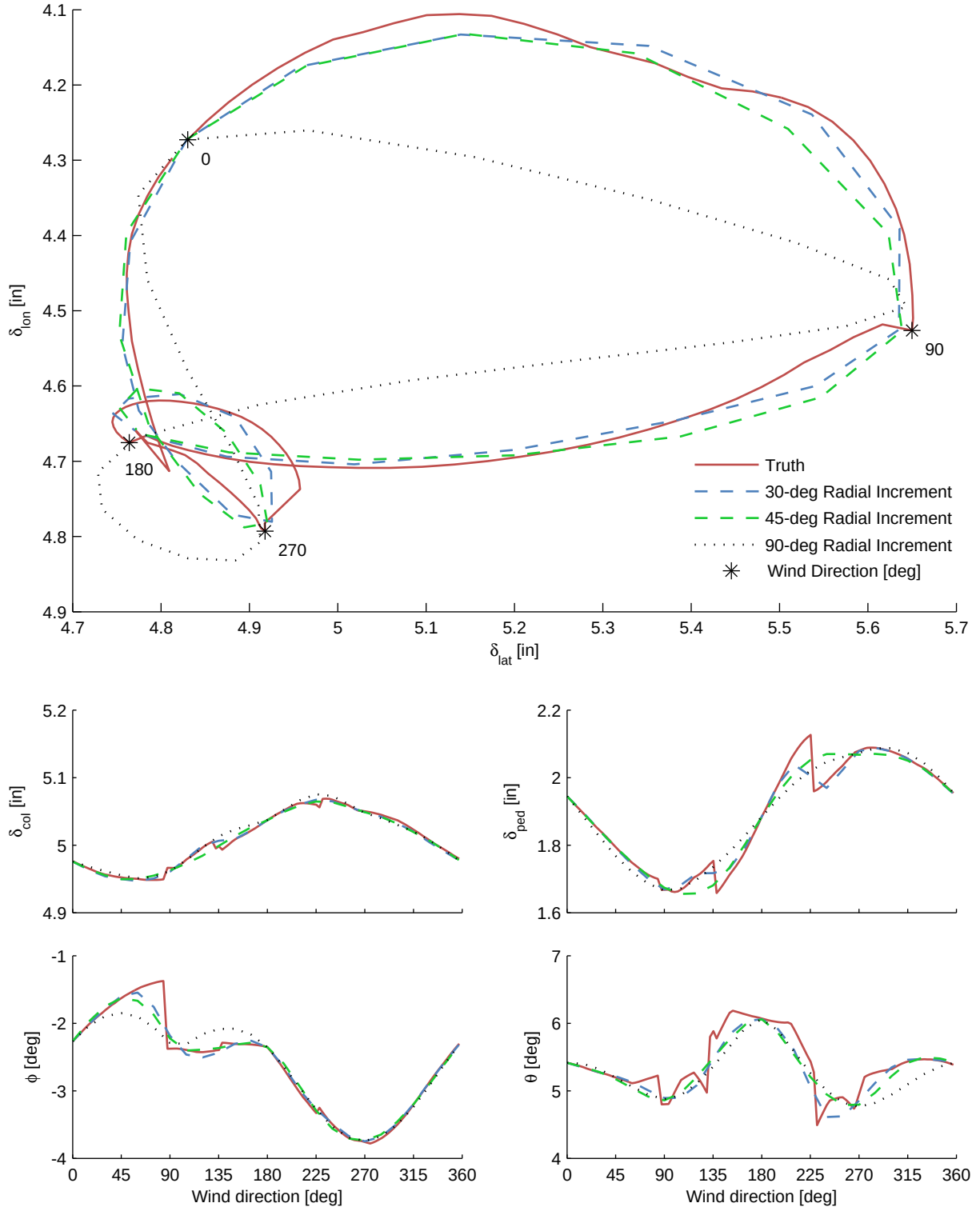
Figure 4.18: Stitched model trim results of position-held/heading-held hovering flight in the presence of a rotating 10-knot wind through 360 degrees.
