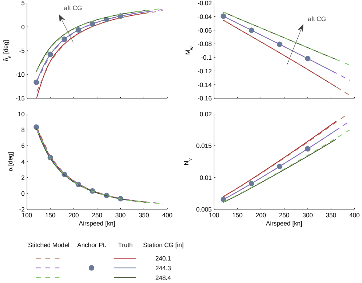
Figure 3.7: Verification of off-nominal CG extrapolation, fuselage station.
