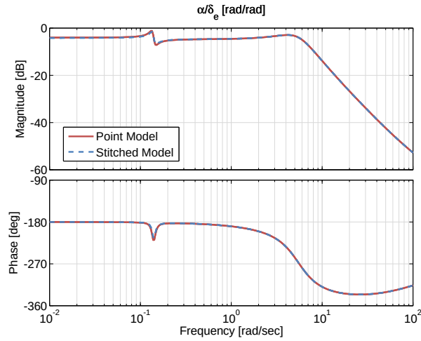
Figure 3.10: Case 1: angle of attack response to elevator input comparison.
