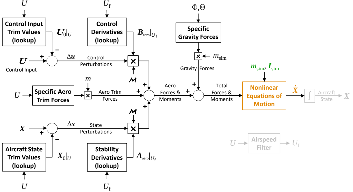
Figure 2.9: Model stitching simulation architecture – nonlinear equations of motion.
