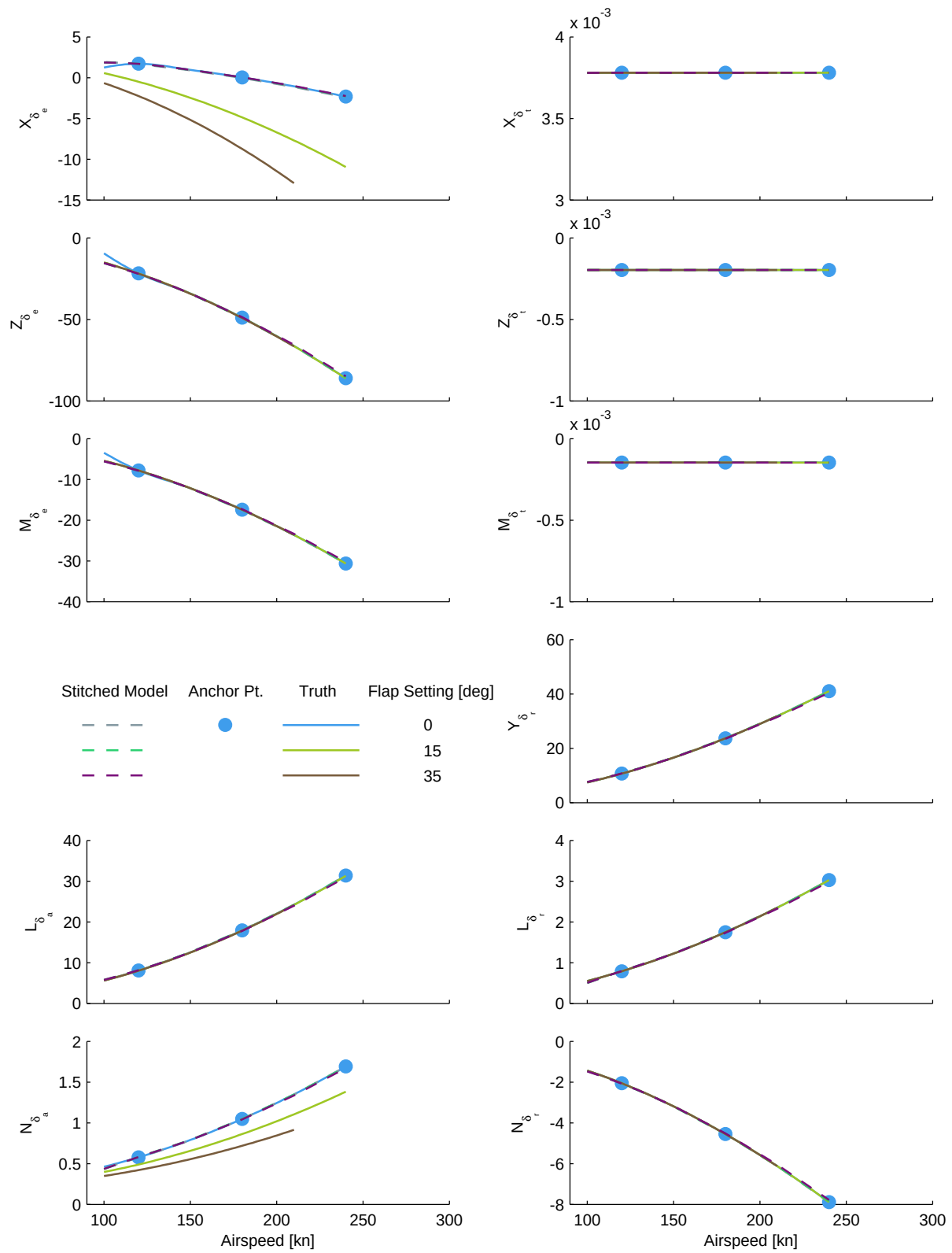
Figure B.28: Alternate configuration verification, flap setting, CJ1 stitched model, control derivatives.
