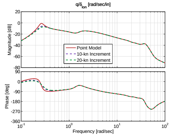
Figure 4.27: Pitch rate response to longitudinal cyclic input comparison for forward-flight trim data of 10- and 20-kn spacing, 120 kn.
