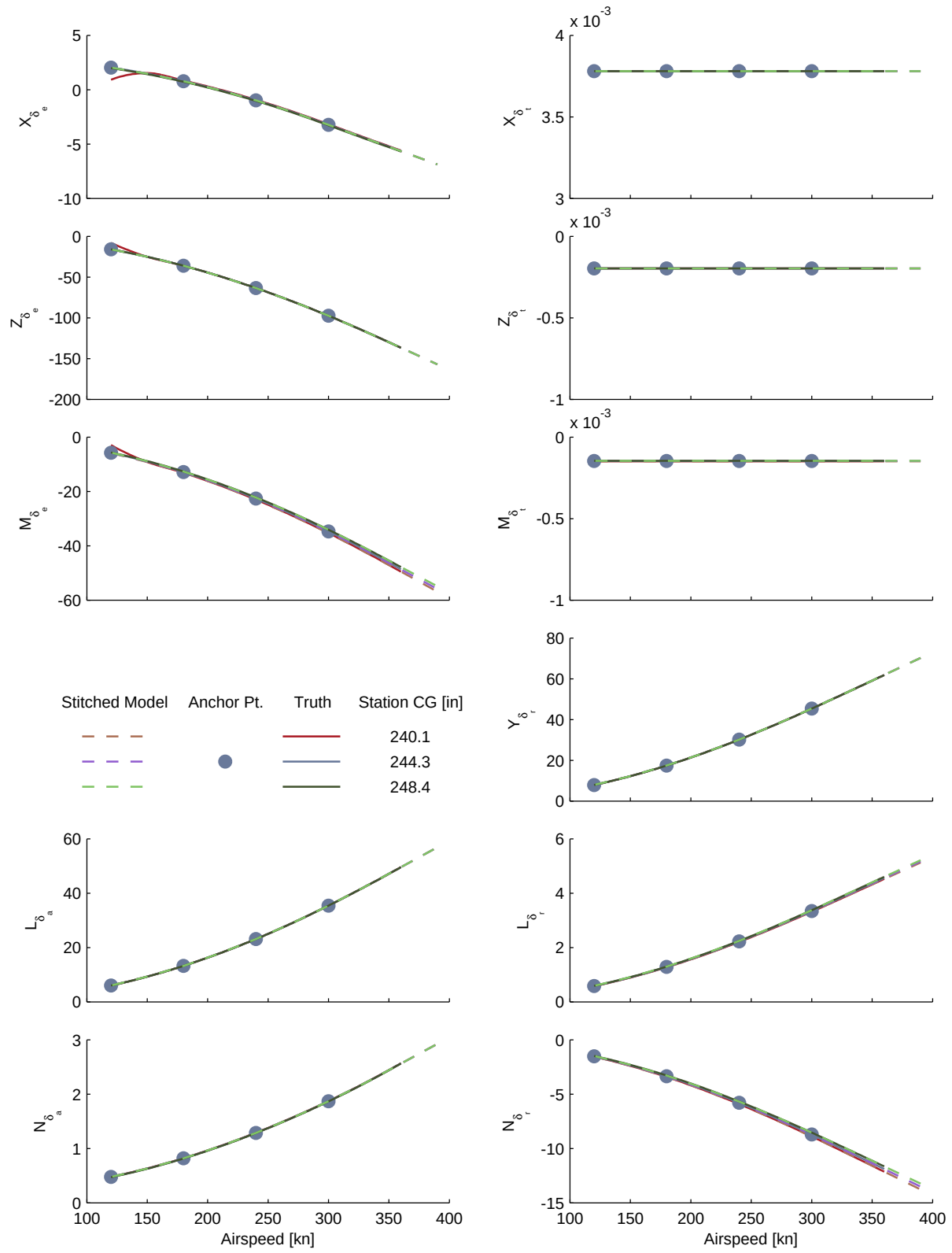
Figure B.13: Verification of off-nominal station CG extrapolation, CJ1 stitched model, control derivatives.
