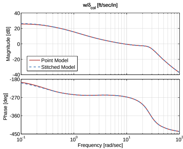
Figure 4.38: Case 1: z -body airspeed response to collective input comparison.
