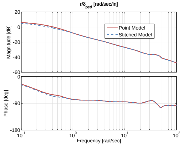
Figure 4.40: Case 1: yaw rate response to pedal input comparison.
