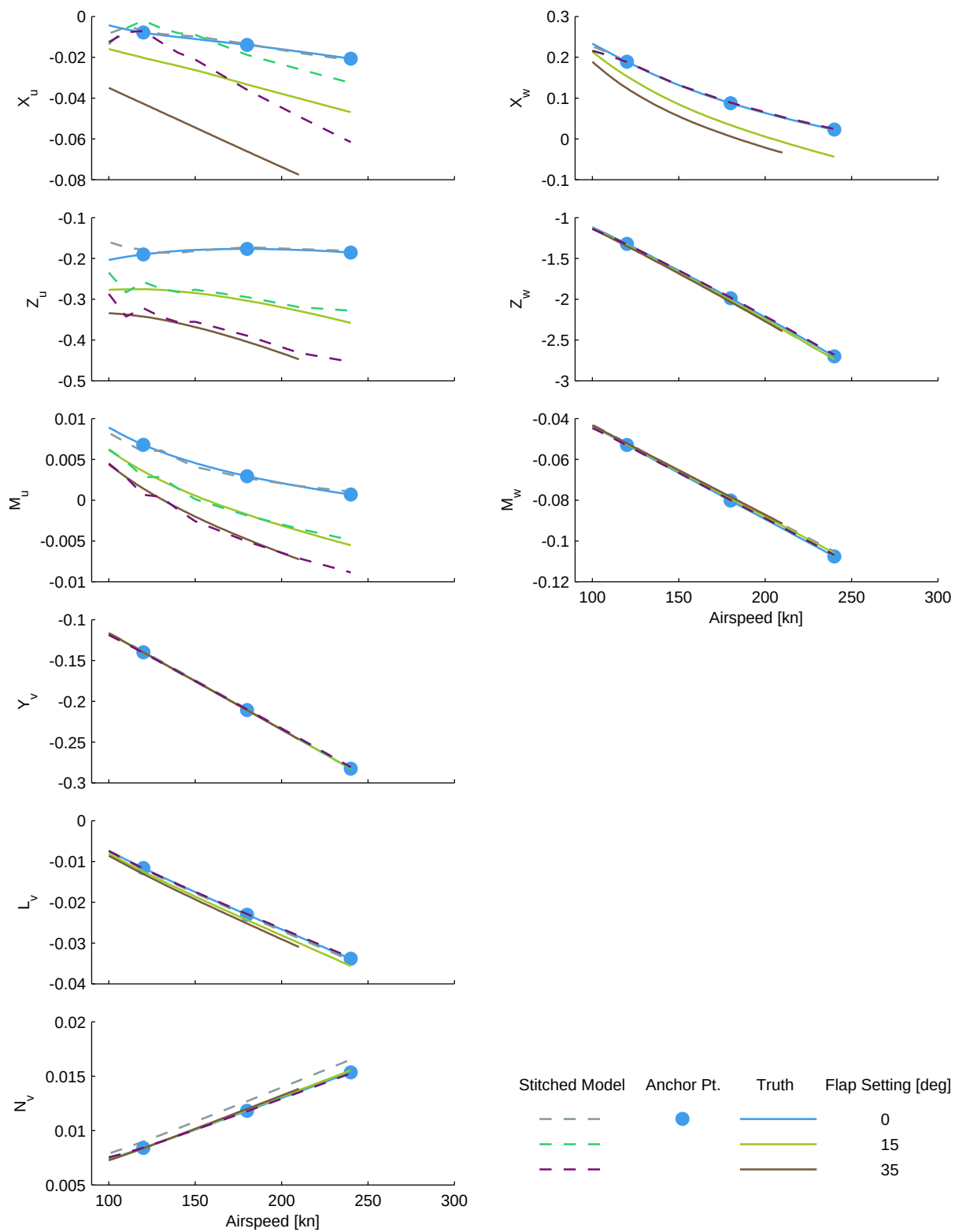
Figure B.27: Alternate configuration verification, flap setting, CJ1 stitched model, stability derivatives.
