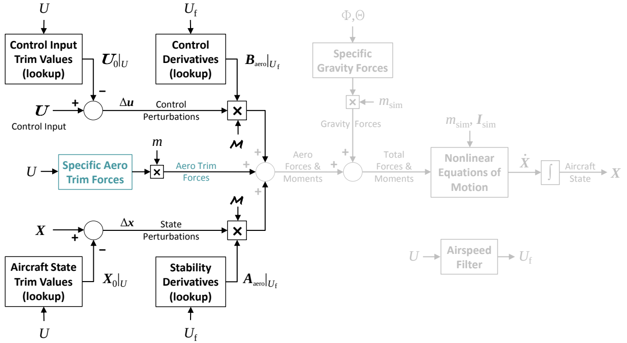
Figure 2.5: Model stitching simulation architecture – aero trim forces.
