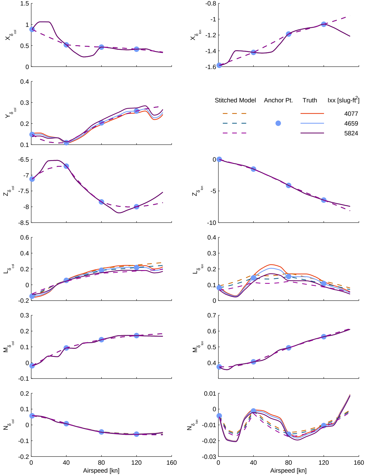
Figure C.6: Verification of off-nominal roll inertia extrapolation, UH-60 stitched model, control derivatives.
