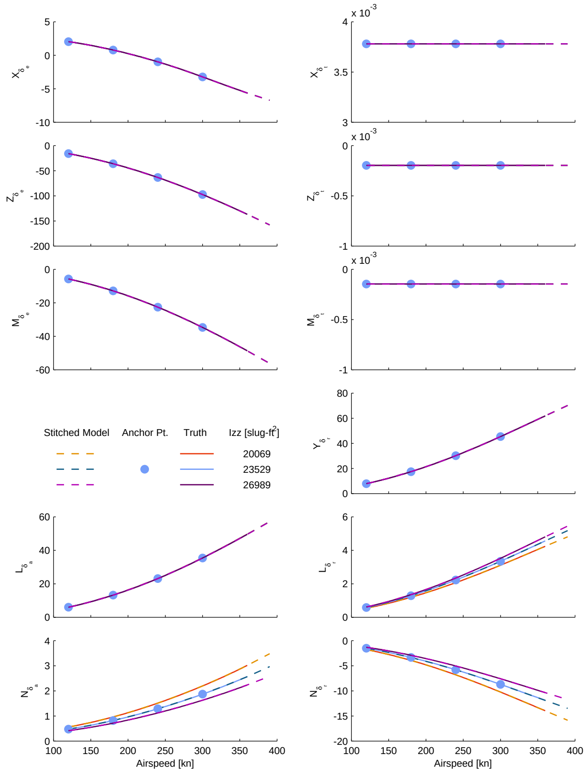
Figure B.10: Verification of off-nominal yaw inertia extrapolation, CJ1 stitched model, control derivatives.
