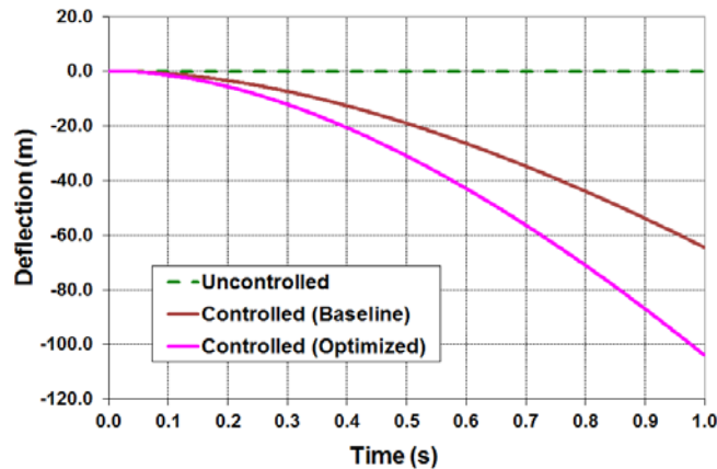
Fig. 14 Flight dynamic results showing trajectory deflection control due to microflaps; initial M = 2.5
