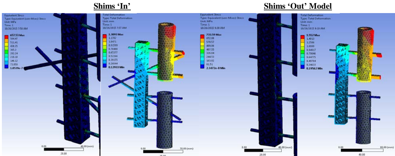
Figure 6 Finite Element Analysis (FEA) model developed through ANSYS 16. Stresses and total deformation suffered shown in shims in configuration (left) and shims out configuration (right). Shims out model simplified by removal of 'diagonal' pins for ease of computation (not in contact with fixator without shim addition).
