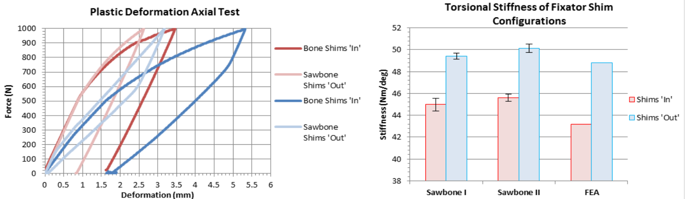
Figure 5 Axial Plastic Deformation Compressive testing (Left) and Elastic Torsional Stiffness of Fixator (Right)
