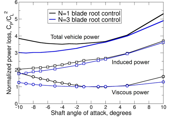
FIGURE 2.7: Power loss of a coaxial rotor with pusher propeller using N = 1 and N = 3 blade root control divided into induced and viscous components .
