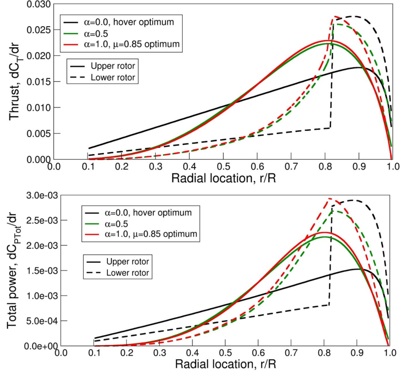
FIGURE 5.16: Radial thrust and total power distributions for the optimal N = 1 coaxial rotor in hover with varying values of \alpha .
