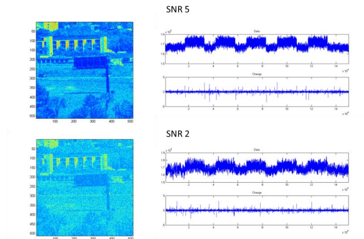
Figure 3-25. Simulation results to test when the anomaly detection using FPA fails under different noise level
