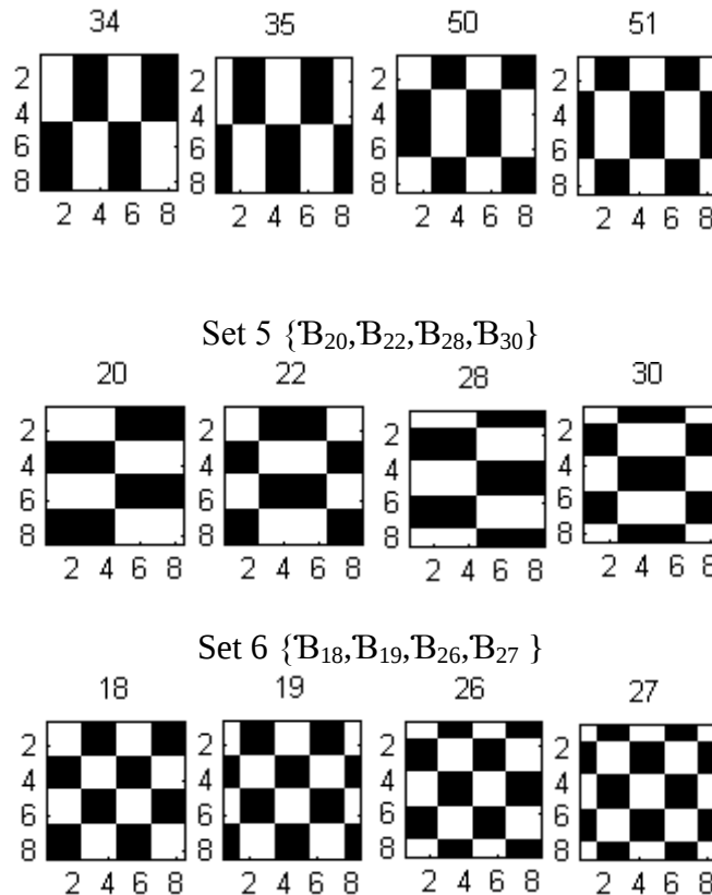
Fig. 2-8. Signature tiles of complementary Hadamard block sets corresponding to different anomaly sizes (e.g., for size 2×2, we would choose measurements from group { B_{18}, B_{19}, B_{26}, B_{27} }).
