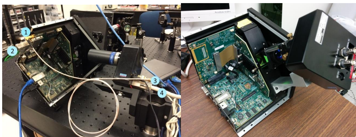
Figure 3-1. Compressive camera with multi-pixel optics and electronics modifications used in our experiments. Parts labeled are: (1) pattern generator BNC connection; (2) pattern generator PCIe connection; (3) sensor array BNC connection; (4) CameraLink connection to the Hamamatsu 64 x 64 sensor array.
