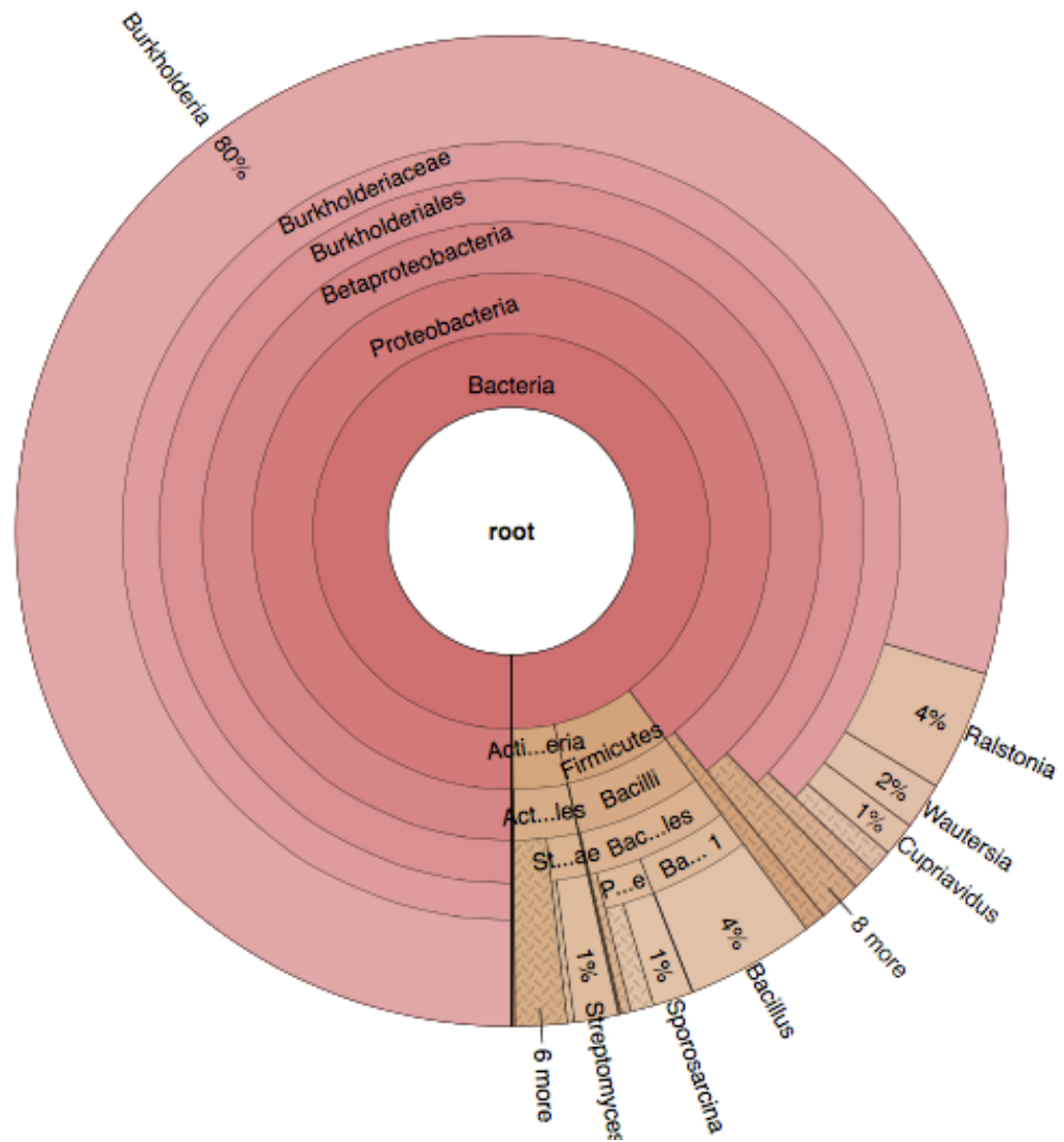
Figure 22 Microbiome of termite hindgut from the Appomattox River cultured in selective cellulose media from the phylum to the genus level
