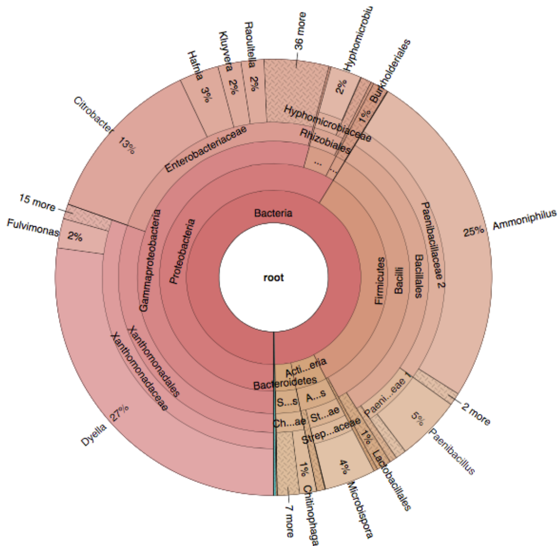
Figure 24 Microbiome of soil sample from the East Woods of VSU cultured in selective cellulose media from the phylum to the genus level
