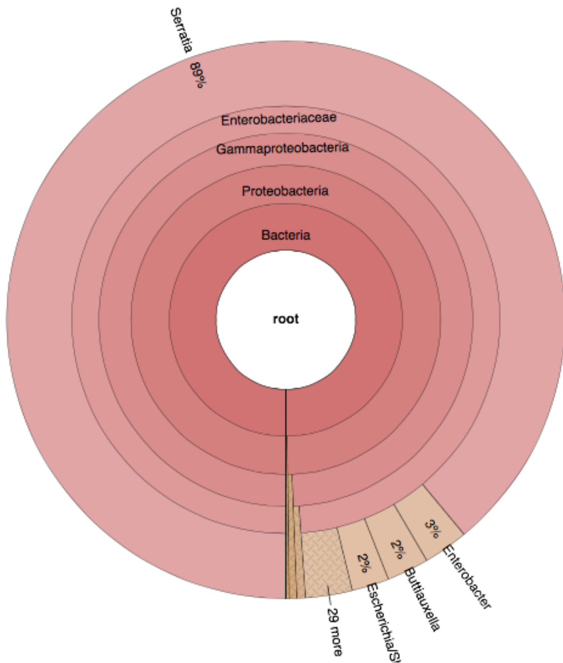
Figure 13 Microbiome of leaf sample #1 from the Bear Creek State Park cultured in selective cellulose media from the phylum to the genus level
