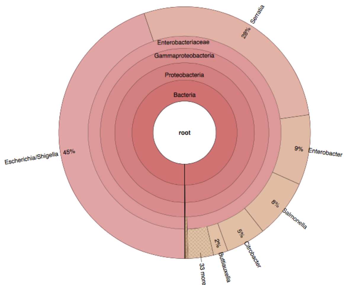
Figure 15 Microbiome of twig sample #2 from the Bear Creek State Park cultured in selective cellulose media from the phylum to the genus level
