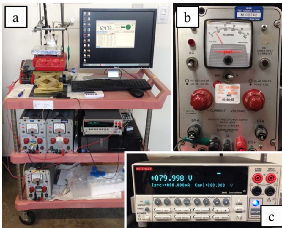
Figure 18. (a) Anodization workstation with DC voltage power supplies, digital voltmeter, digital ammeter with computer interface, and electrochemical cell; (b) one of three power supplies used as a DC voltage source to anodize titanium; and (c) Keithley 2400 Source Meter used to monitor applied anodization potential.
