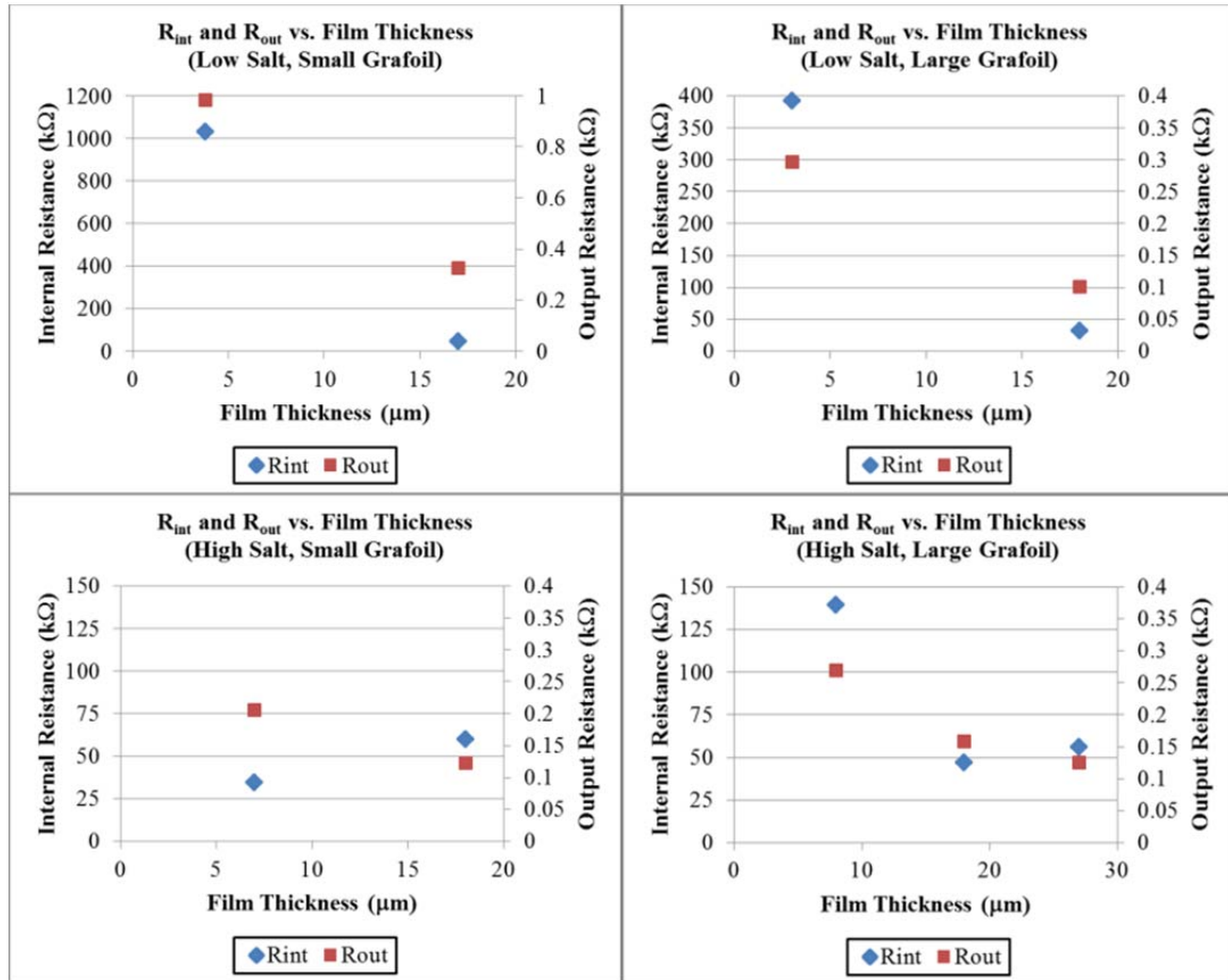
Figure 105. NTSDM capacitor leakage resistances (internal and output) vs. film thickness for varying salt concentrations and electrode surface areas.
