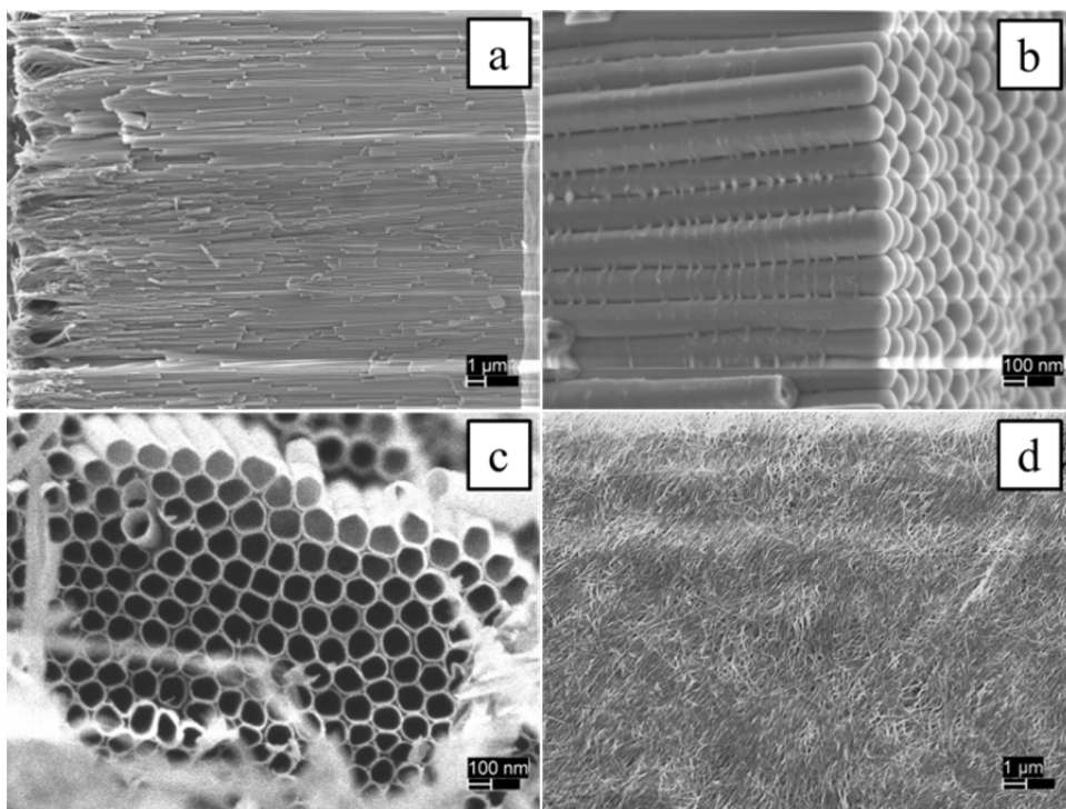
Figure 55. SEM images of 50 volt, 4-hour anodic film capturing 27 \mu\text{m} (a), familiar tubular morphology at tube bases (b), clean tube structure just below grassing (c), and grassing at the surface (d).
