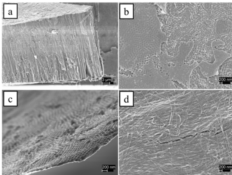
Figure 60. SEM images of 50 volt, 4-hour (reused electrolyte) anodic film capturing 26 \mu\text{m} nanotubes (a), tube bottoms with non-anodized substrate remnants (b), remnant of titanium substrate (c) and grassing (d).
