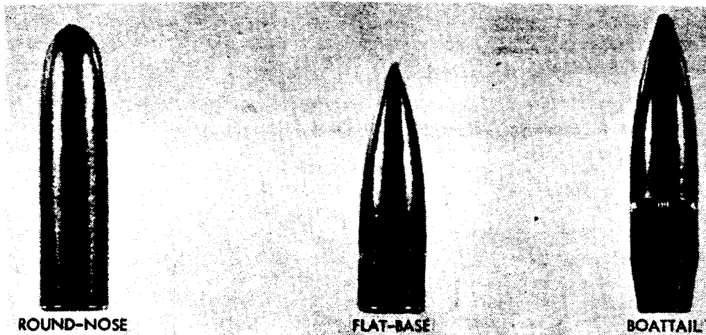
Figure 8. Typical Bullet Shapes
