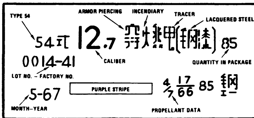
Figure 21. Chinese Sheet-Metal Container Markings, 12.7x108 API-T, Type 54 Cartridges
