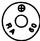
A335 UNITED STATES Also found with "9 MM" in place of NATO mark. On 9x19-mm and 7.62x51-mm cartridges. 1900-1968.
