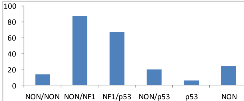
Graph 2: Percentages of blue cells obtained after performing \beta -Gal Assay of infected cells
