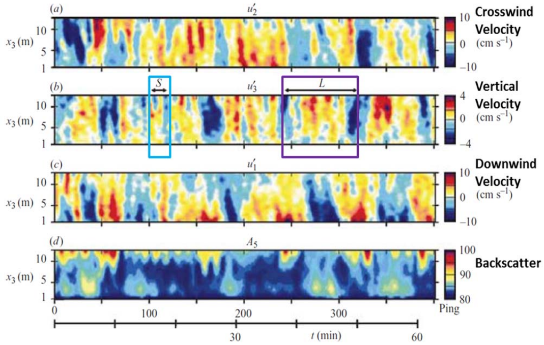
Figure 10. Examples of LSC Spatial and Time Scale of Variability
