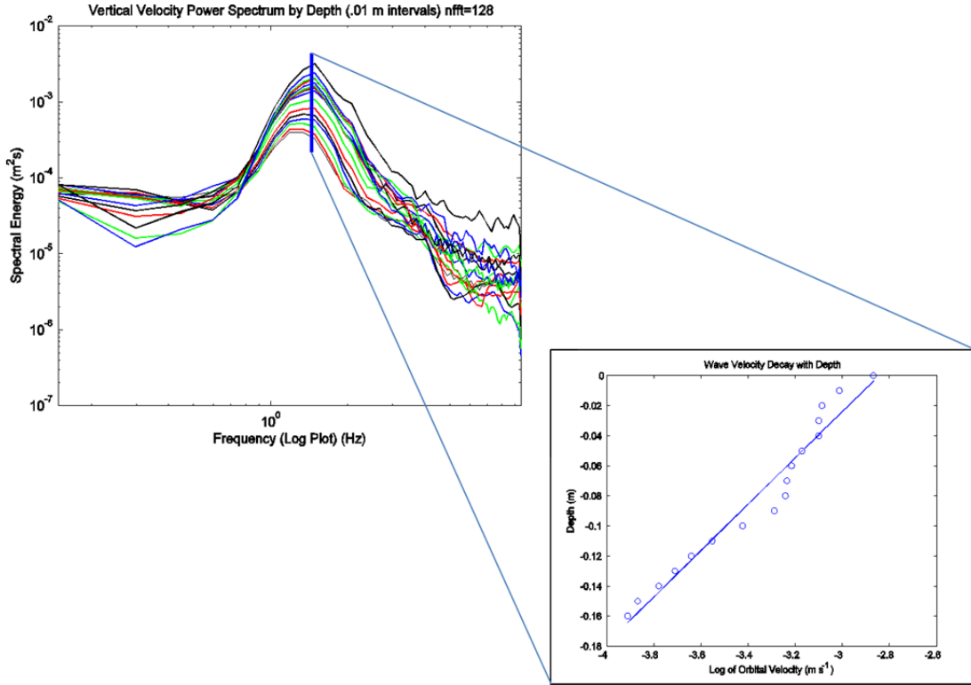
Figure 22. Decay of Wave Orbital Velocity with Depth
