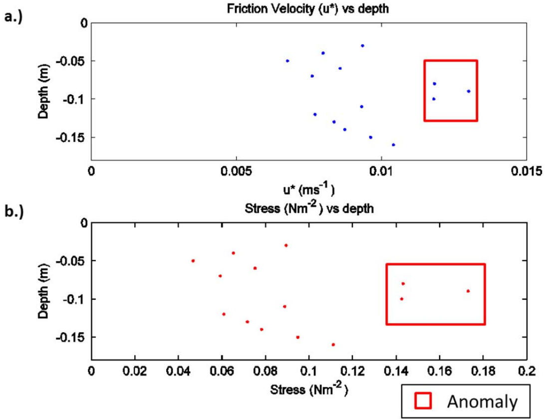
Figure 27. Friction Velocity and Stress
