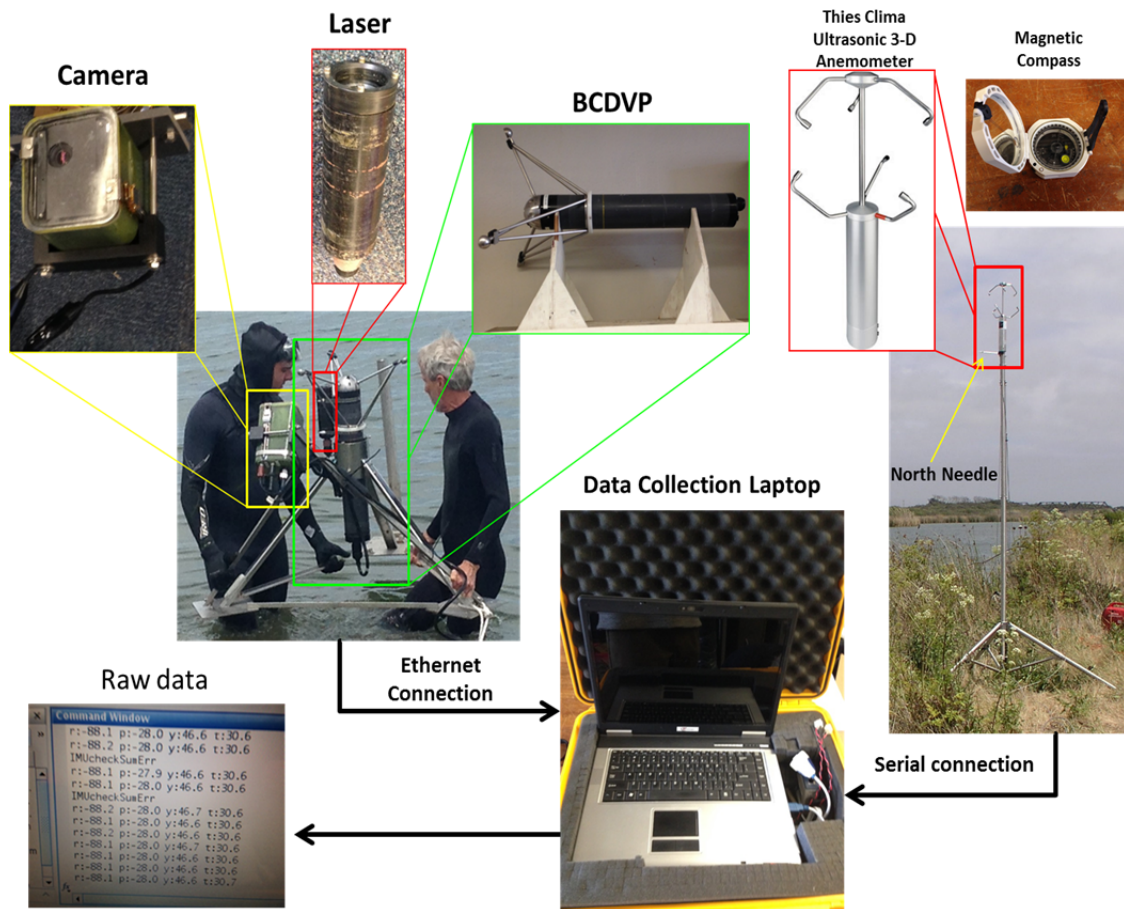
Figure 17. Sensors Network Setup
