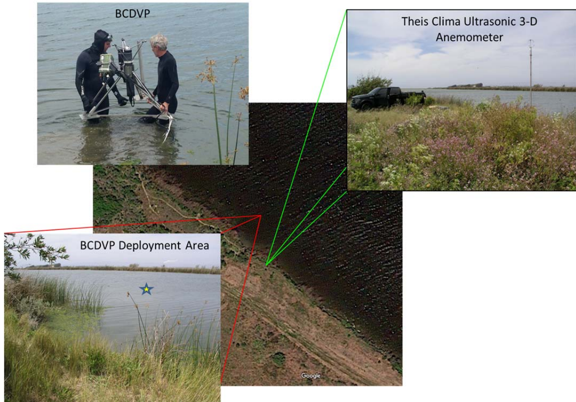
Figure 18. Sensor Deployment Locations
