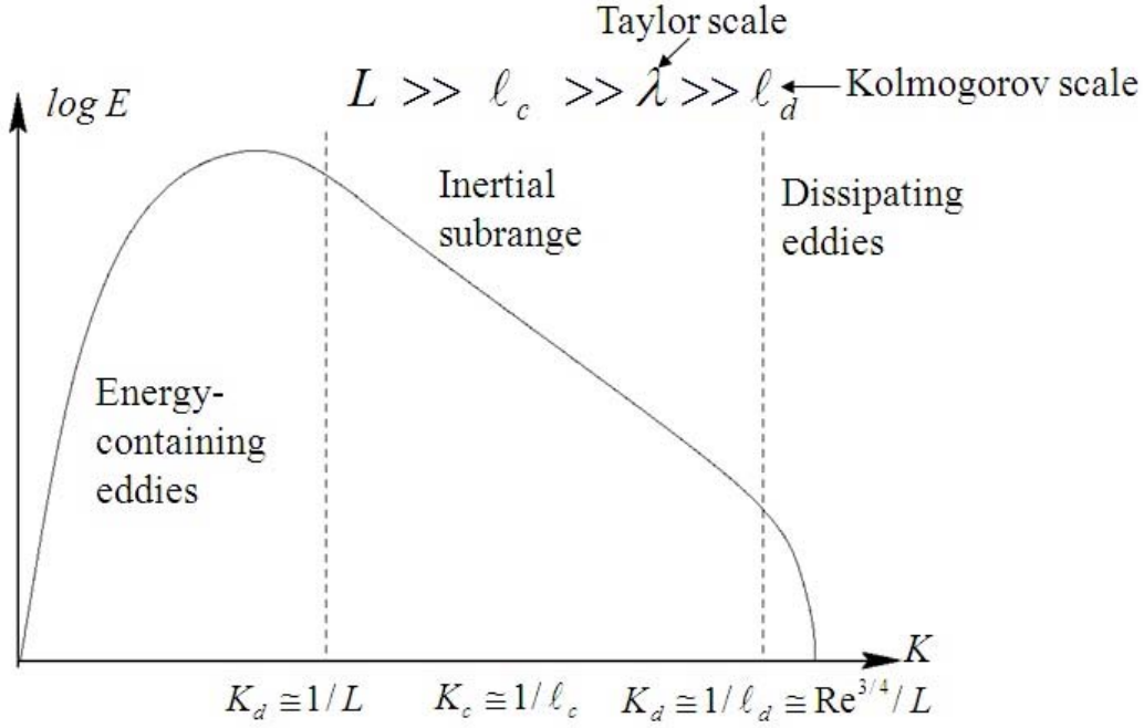
Figure 1. Energy Spectrum Breakdown and Distribution Based on the Kolmogorov Scale
