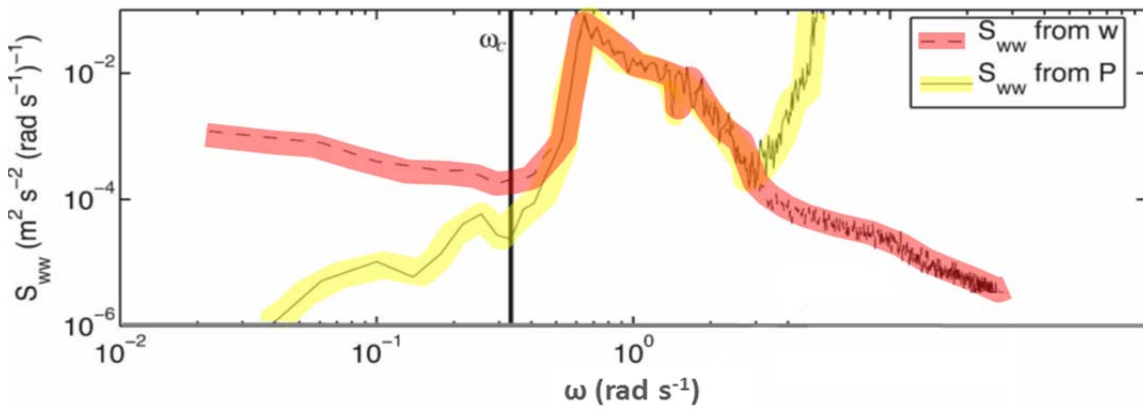
Figure 2. Example Autospectra of Vertical Velocity Fluctuations
