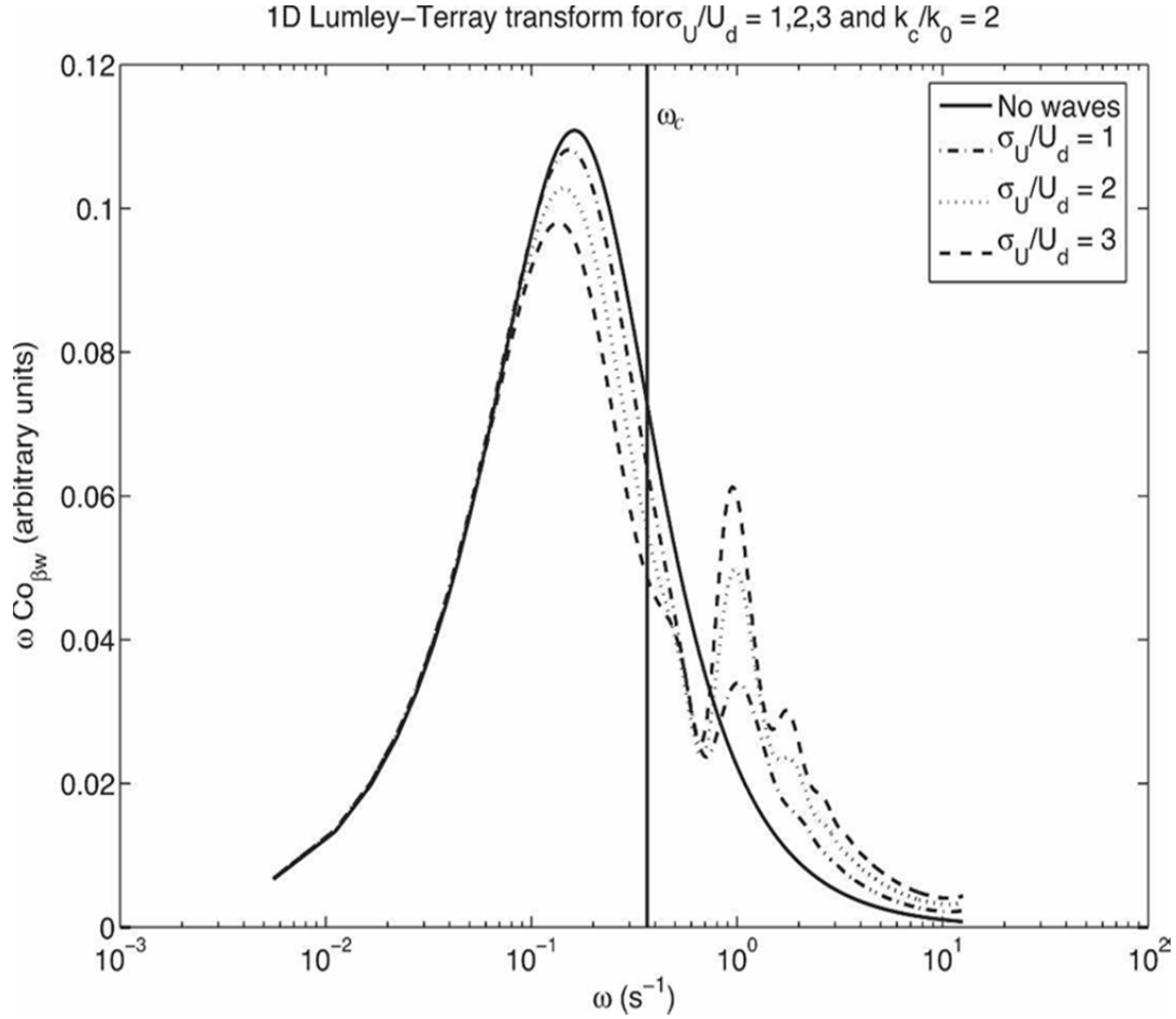
Figure 3. Unsteady Frozen Turbulence Spectrum Affected by Wave Energy
