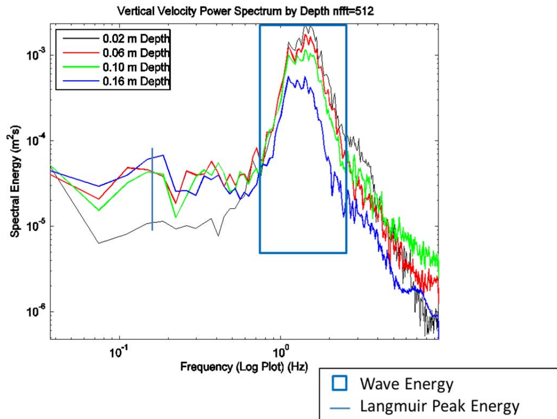
Figure 30. Wave Energy and Langmuir Energy
