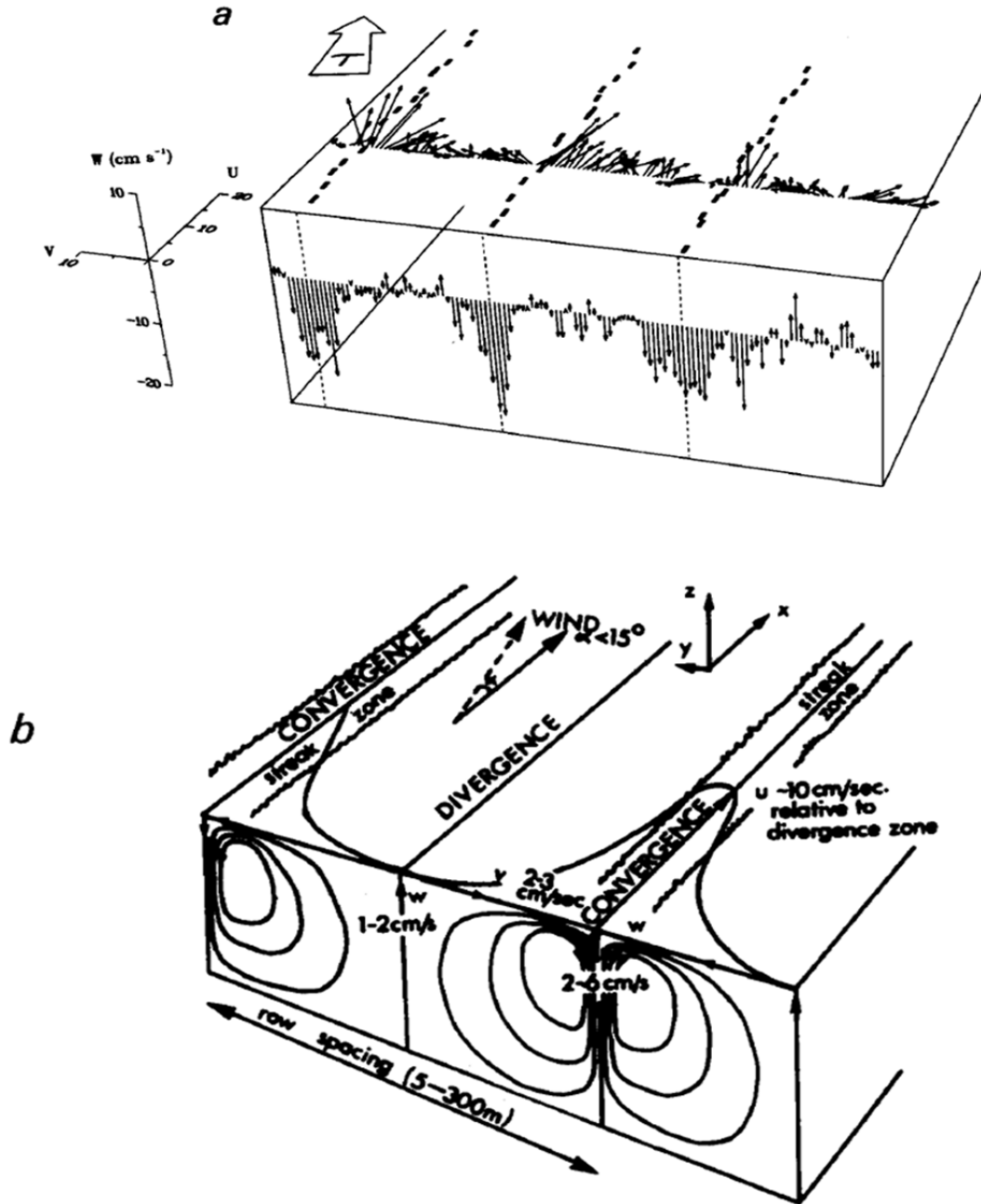
Figure 6. Langmuir Circulations and December 1982 RTP Data
