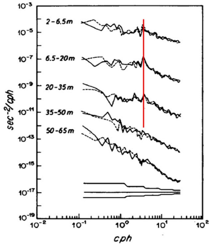
Figure 7. Rotary Autospectra of the Vertical Shear November 9, 1983
