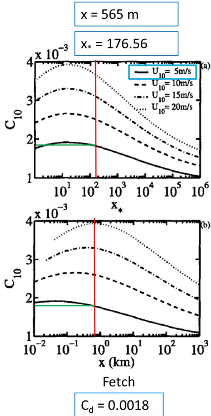
Figure 23. Drag Coefficient Curves
