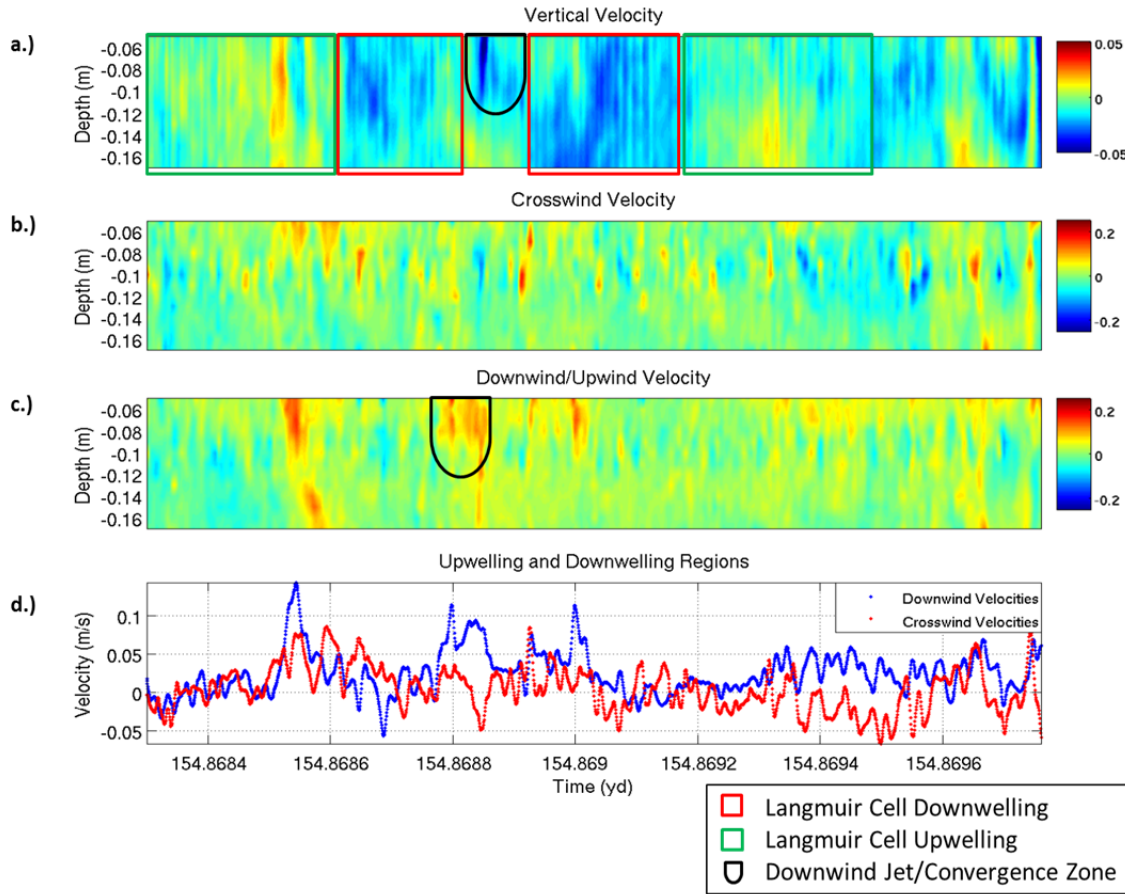
Figure 29. BCDVP Velocity Data
