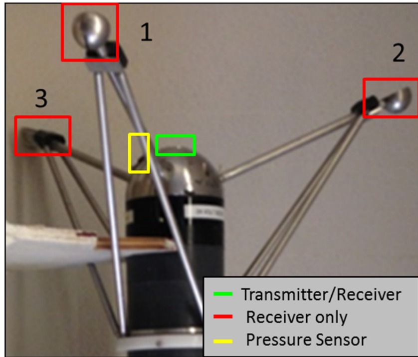
Figure 19. BCDVP Probe Diagram
