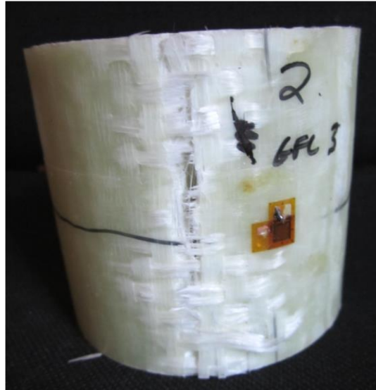
Figure 50. Glass Fiber Composite #3 Failure Location.
