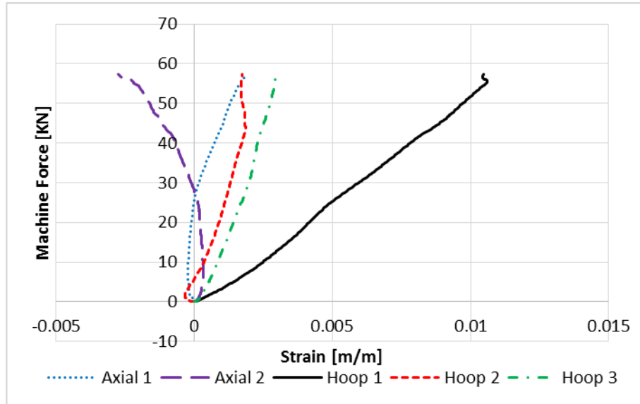
Figure 59. Carbon Fiber Composite #4 Test Results.
