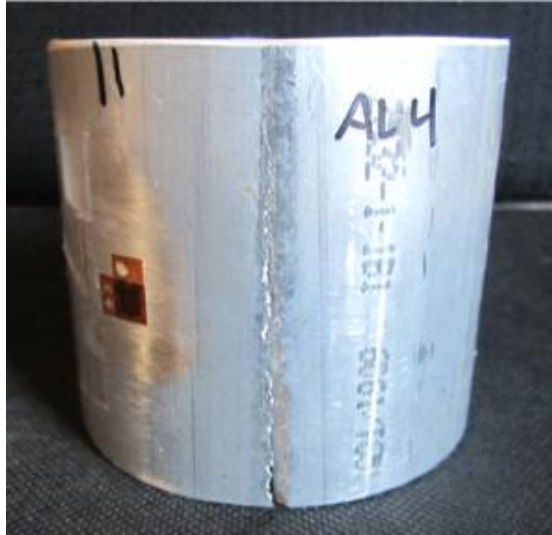
Figure 37. Failure Location of Thin Aluminum #4 Near Strain Channel 2.
