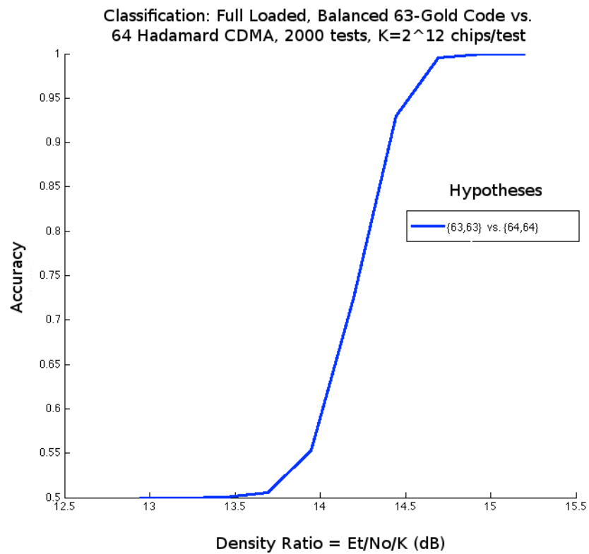
Fig. 32 Classification of {63,63}-Gold Code versus {64,64}-Hadamard
