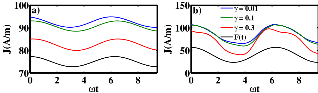
Figure 3.2: (Color online) Current density for three different values of the damping \gamma at resonance ( \omega \approx 0.56\omega_F ). (a) F_1/F_o = 0.1 ; (b) F_1/F_o = 0.8 .
