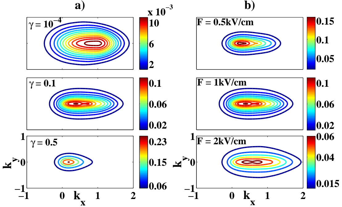
Figure 2.2: (Color online) (a) Contour plot of the distribution functions for different damping parameters ( F = 1 kV/cm) and (b) different applied fields ( \gamma = 0.1 ).
