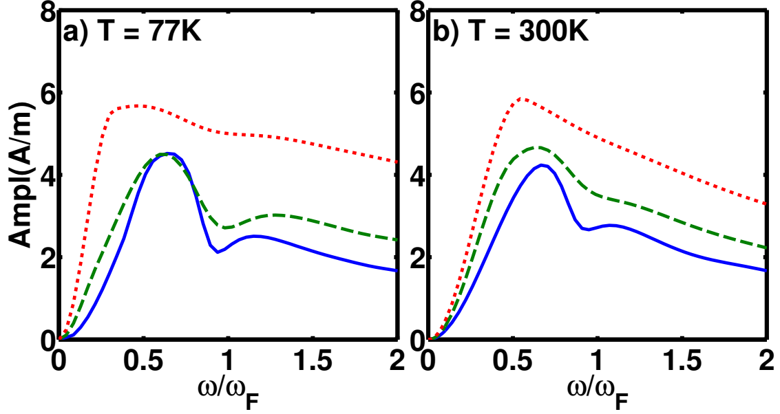
Figure 4.5: (Color online) Current density amplitude vs frequency for different values of \gamma . (a) T = 77 K and (b) T = 300 K. F_1/F_o = 0.1 , and F_o = 0.5 kV/cm. Solid lines ( \gamma = 0.01 ), dashed lines ( \gamma = 0.1 ), and dotted lines ( \gamma = 0.3 ).
