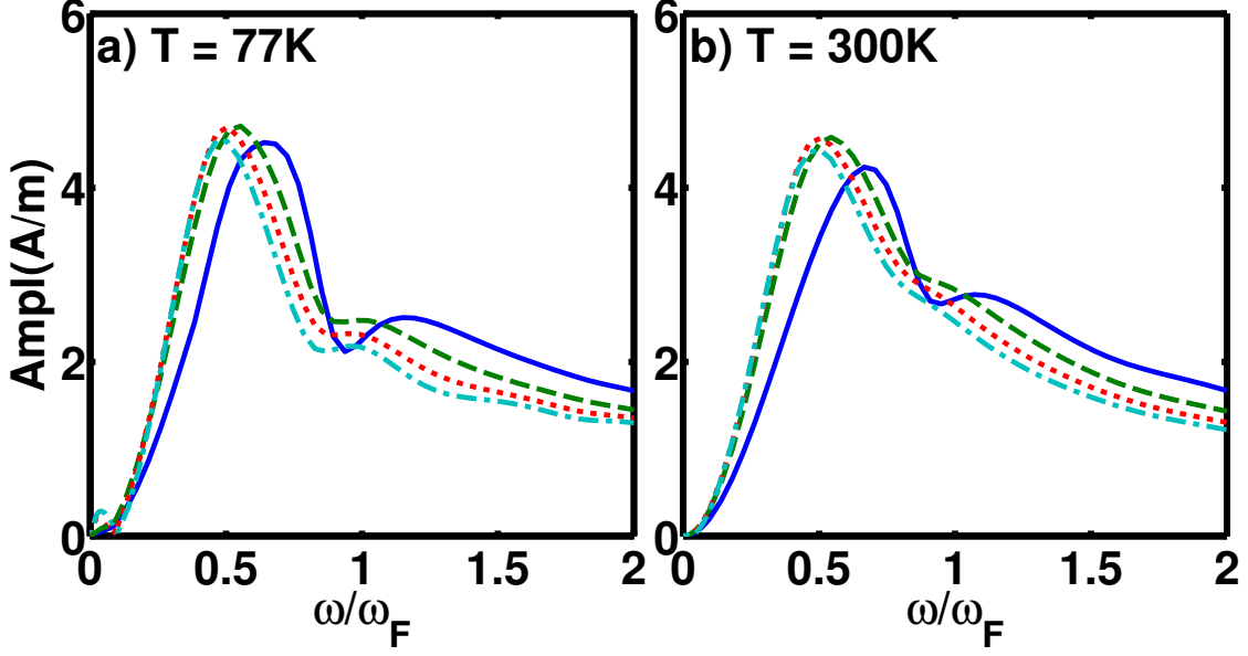
Figure 4.3: (Color online) Current density amplitude vs applied frequency for different values of F_o . (a) T = 77 K. (b) T = 300 K. F_1/F_o = 0.1 , and \gamma = 0.01 . Solid line ( F_o = 0.5 kV/cm), dashed lines ( F_o = 1 kV/cm), dotted lines ( F_o = 1.5 kV/cm), and dashed-dotted lines ( F_o = 2 kV/cm).
