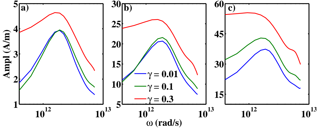
Figure 3.3: (Color online) Current density amplitude vs frequency for three different values of the damping parameter \gamma . (a) F_1/F_0 = 0.1 ; (b) F_1/F_0 = 0.5 ; (c) F_1/F_0 = 0.8 .
