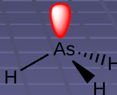
Arsine
