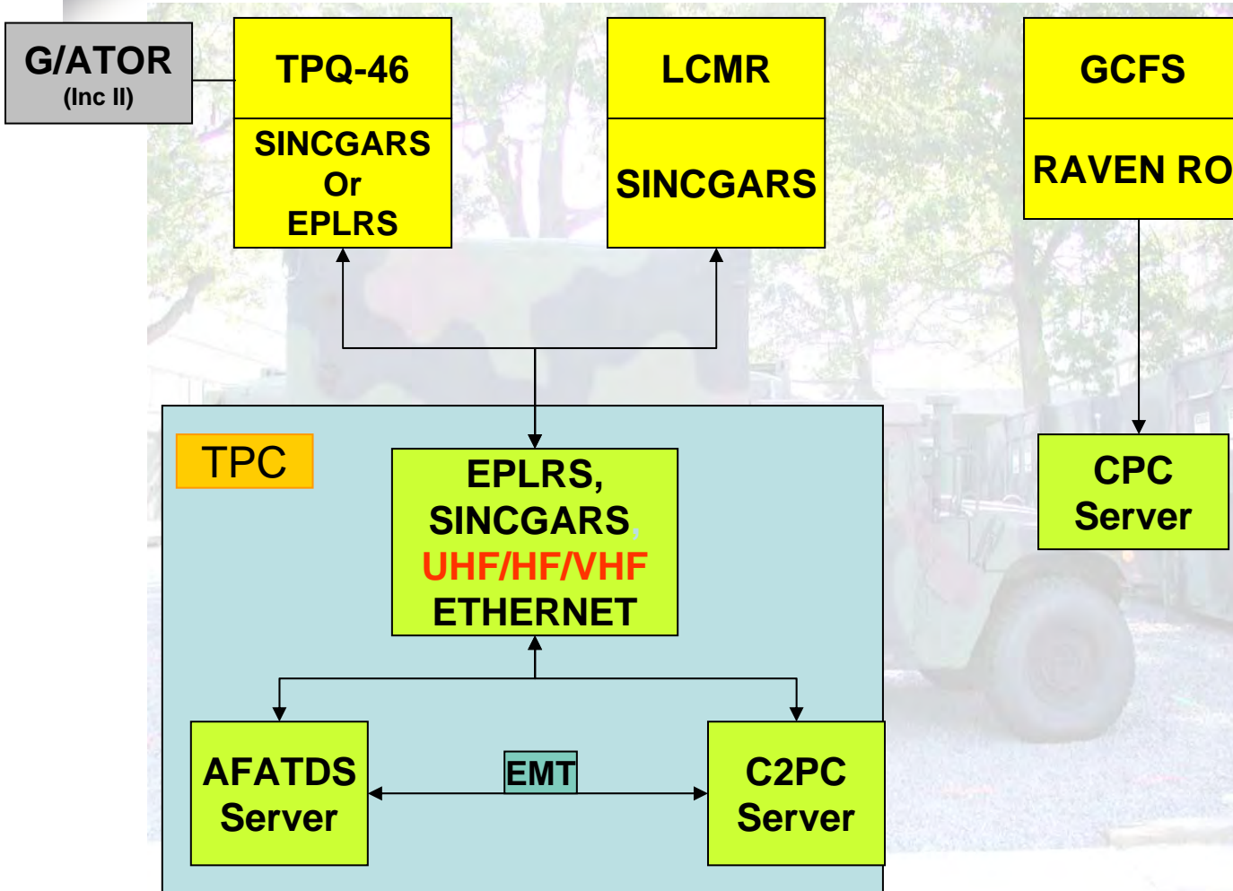
TPC – GWLR, LCMR, GCFS Architecture using fielded H/W
