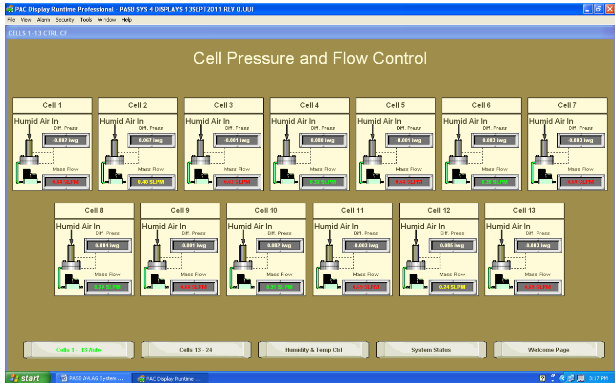
Figure 1. Example of the AVLAG environmental control system screen display for flow control.
