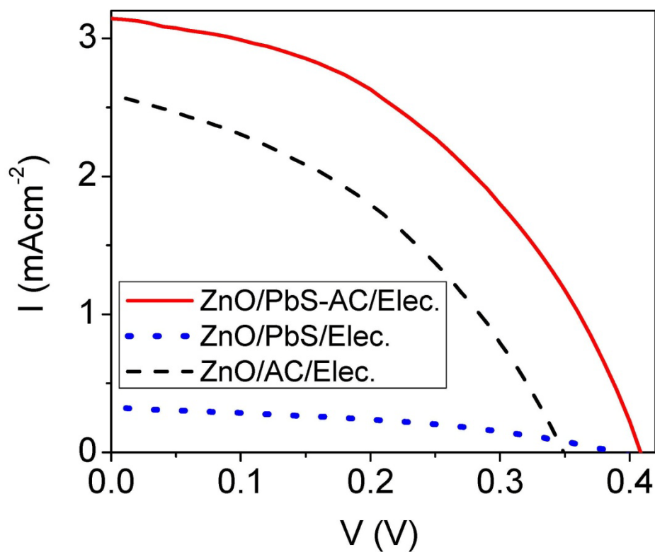
Figure 9-5: The IV characteristics of the three device structures (i.e., ZnO/Dye, ZnO/PbS, and ZnO/PbS-Dye) under illuminated with \sim 100 \text{ mW/cm}^2 light source.
