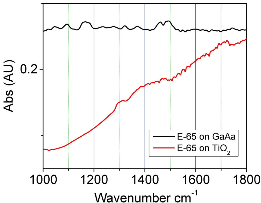
Figure 8-2: The FTIR spectrum of the dye deposited on GaAs wafer, nanocrystalline TiO 2 film are shown in the Fig.4 below. The annihilation of absorption peaks in the range 1000 cm -1 to 1250 cm -1 with E-65 adsorbed on TiO 2 implies bidentate bonding of E-65 on to TiO 2 .
