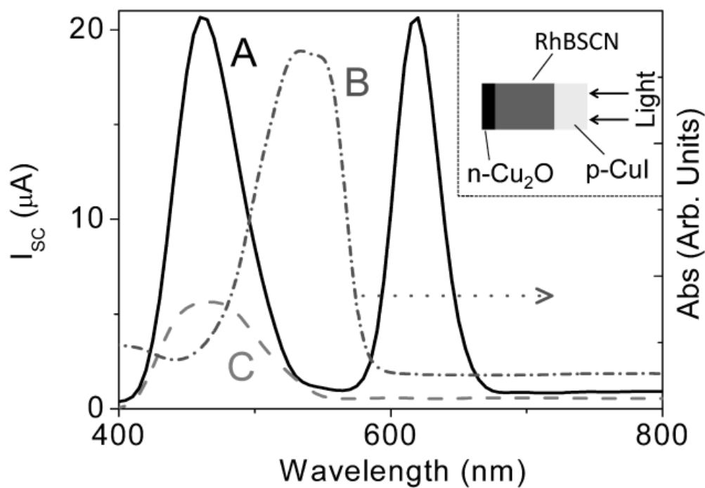
Figure 7-4: A-Photocurrent action spectrum of a n-Cu 2 O/J-aggregated RhBSCN/p-CuI heterojunction shined with light as indicated in the inset (for clarity contacts to cell are not shown). The narrow peak to left in the curve A originate from light absorption by the dye and the broad peak is Cu 2 O band gap excitation. B - Absorption spectrum of aqueous RhBSCN. C - Photocurrent action spectrum of n-Cu 2 O/p-CuI.
