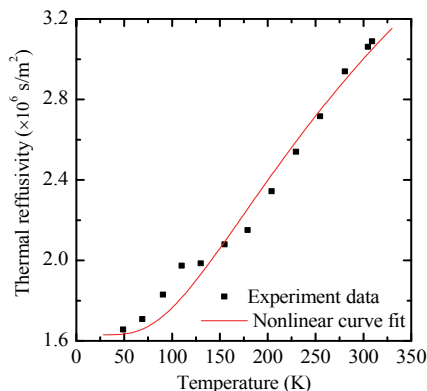
Figure 8. Thermal reffusivity of silkworm silk against temperature. The residual thermal reffusivity and Debye temperature are fitted to be 1.63 \times 10^6 \text{ s/m}^2 and 696.5 K. When the average phonon velocity is estimated as 630 m/s, the mean free path of defect-phonon scattering is determined to be 2.92 nm. This value is very close to the crystallite size uncovered by XRD.
