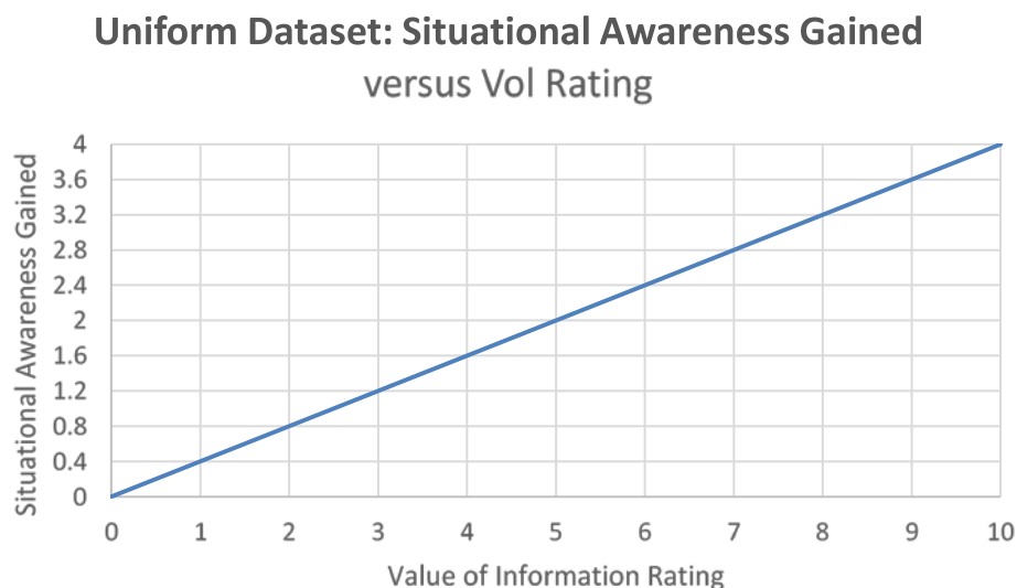
Fig. 1 Relationship between VoI and SA in the uniform data set
