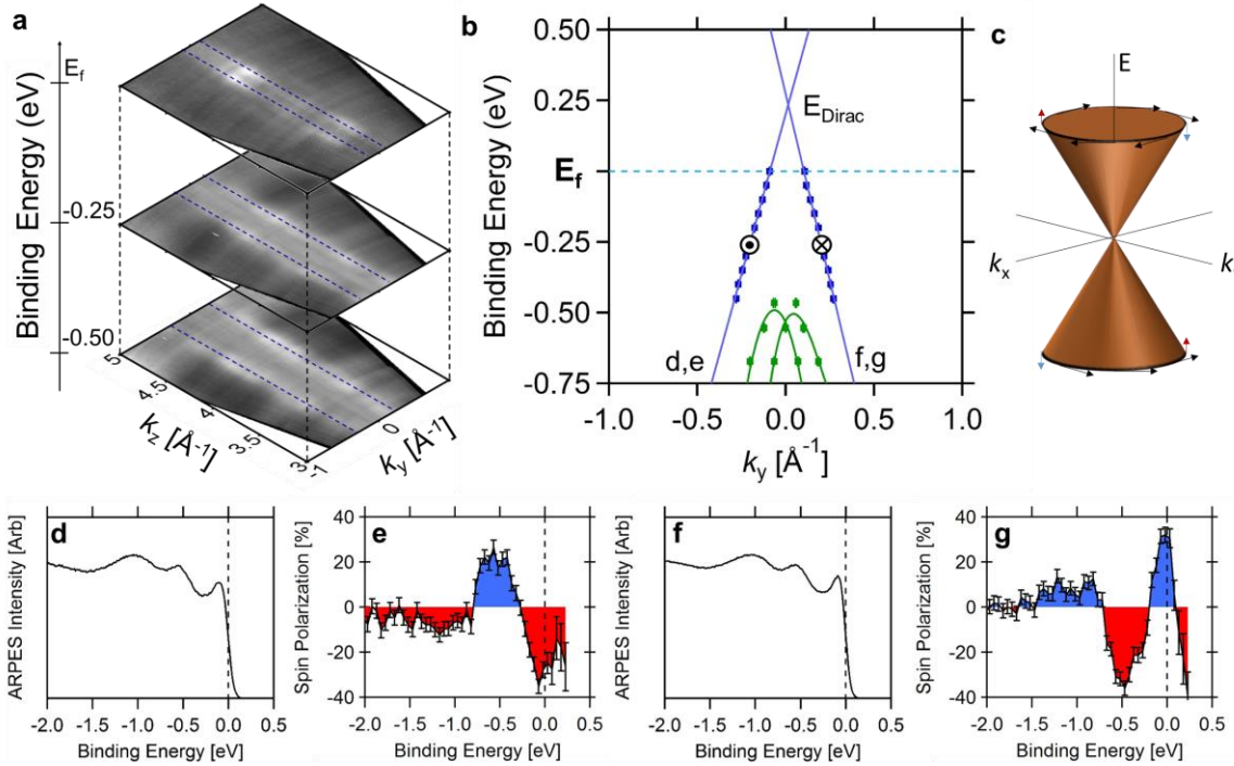
Figure 11 (a) Out-of-plane momentum dependence for various binding energies. An absence of k_z dispersion is observed, consistent with the behavior of a surface state. (b) By tracking this state's position as a function of binding energy, a Dirac-like behavior can be seen with a crossing point approximately 235 meV above the Fermi level. Spin-ARPES spin polarization directions are marked. (c) Schematic diagram of a topological surface state with helical spin texture. (d-e,f-g) ARPES intensity and corresponding spin polarization for the left and right side of the linearly dispersing surface state, respectively. A counter-clockwise helical spin texture, consistent with theory, is observed. Furthermore, a Rashba-like split hole band can be seen at lower binding energies.
