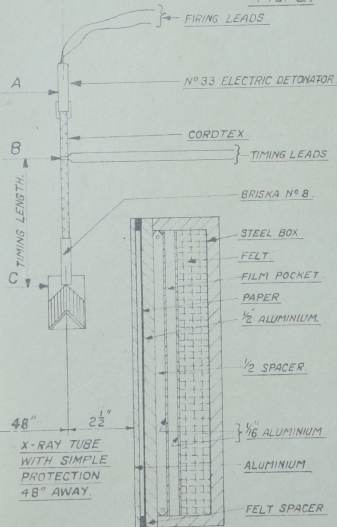
FLASH RADIOGRAPHY OF SHAPED CHARGES.
