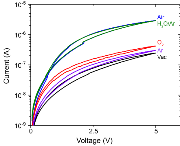
Figure 3. Representative positive voltage I-V curves showing the atmospheric dependence of P:GeH using top contact geometry. Samples were exposed to air (blue), water/argon mixture (green), oxygen (red), argon (violet), and vacuum (black). The sample was pumped down to a base vacuum of 5 \times 10^{-4} mbar between measurements.
