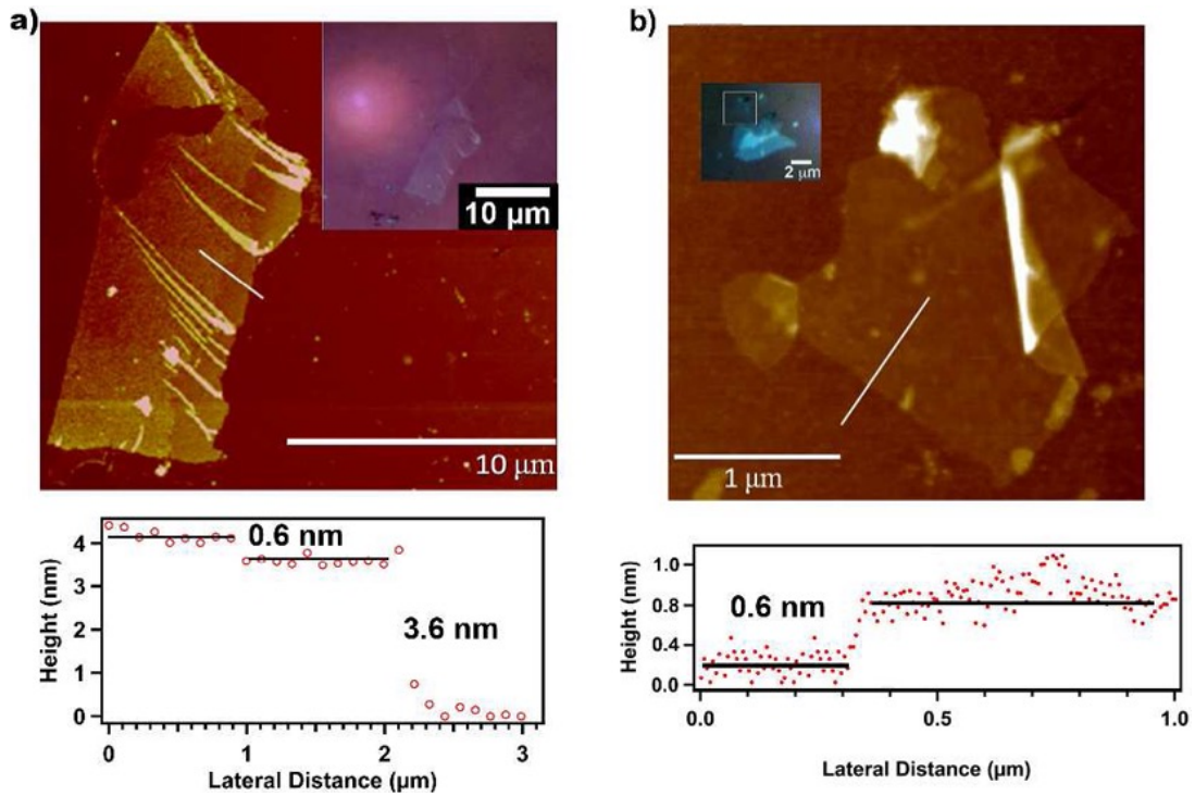
Figure 2.2. (a) AFM image (top), optical image (inset) and height profile of few-layer GeH flake on SiO 2 /Si. (b) AFM image (top), optical image (inset) and height profile of single-atom-thick GeH flake. 18
