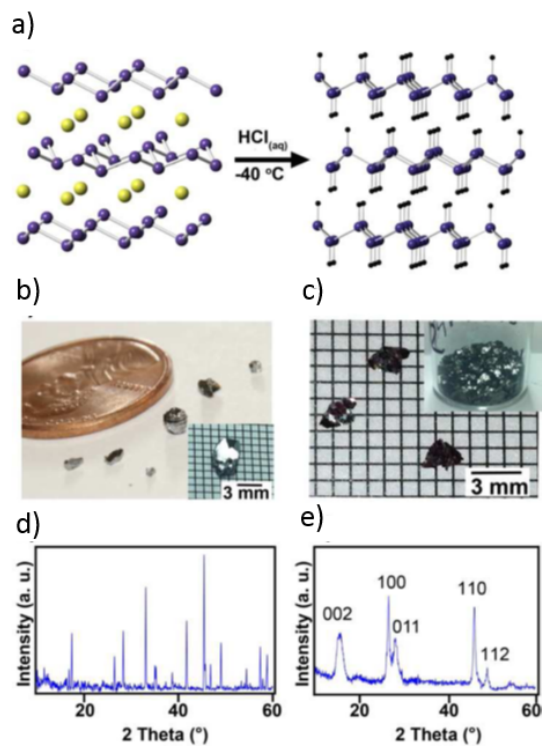
Figure 3.1 (a) Schematic illustration of the GeH preparation. (b) Optical image of CaGe 2 crystal. (c) Optical image of GeH crystal. (d) XRD diagram of (b). (e) XRD diagram of GeH. 18
