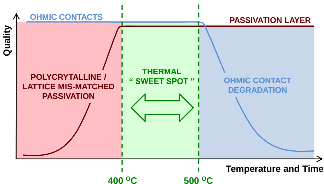
Figure 1.2: Thermal "sweet-spot"
