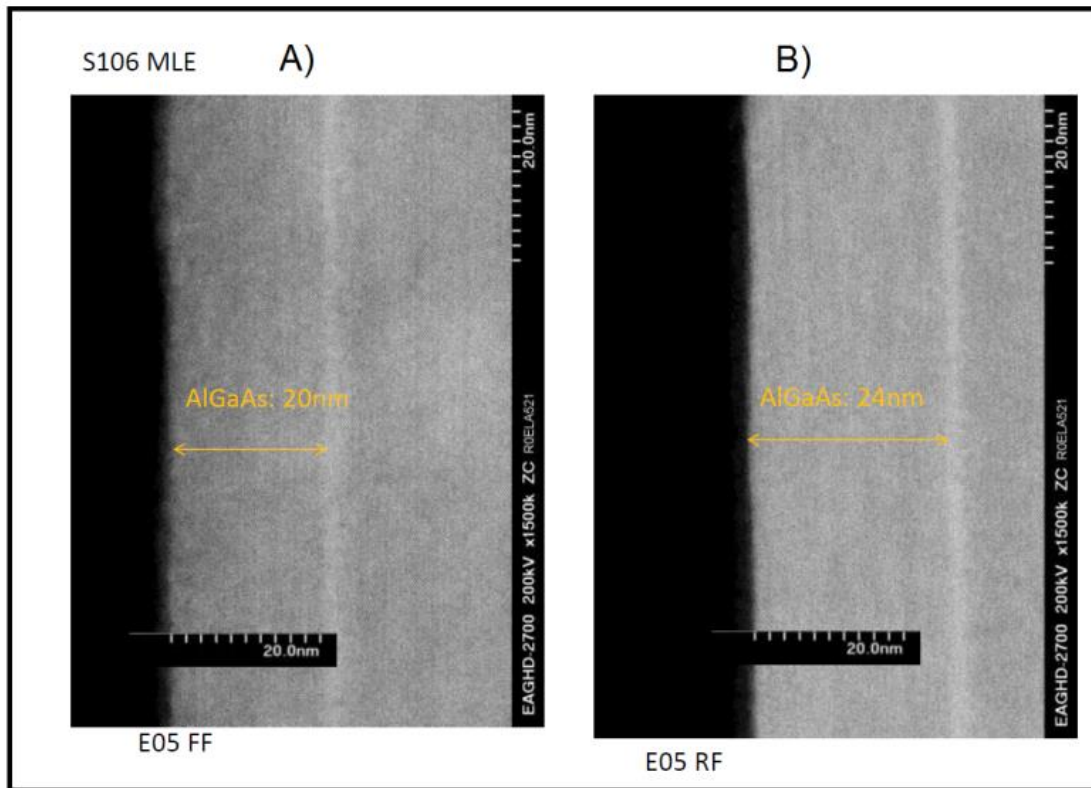
Figure 4.10 Cross section of laser diode A) front facet and B) rear facet showing the epitaxial passivation GaAs/AlGaAs layers grown by MBE.
