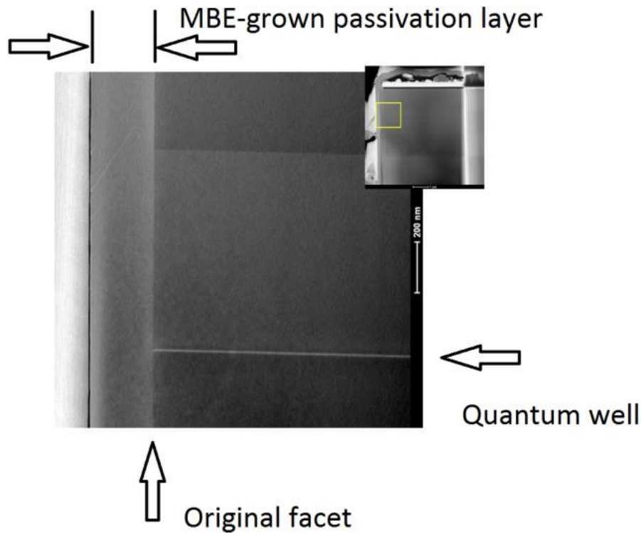
Figure 4.8 TEM image of \text{Al}_x\text{Ga}_{(1-x)}\text{As} ( \sim 237\text{nm} thick) layer grown by MBE at 500^\circ\text{C} on the facet of a processed 980 LD-bar.
